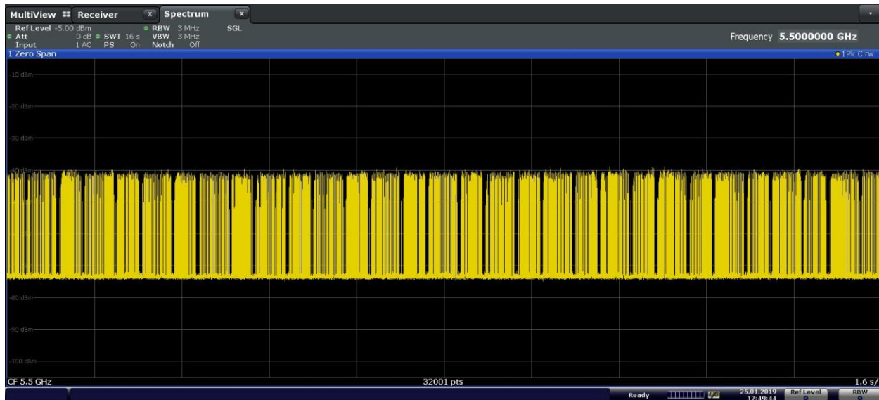
Figure 9-7. 5500MHz - Channel Loading - Mode 2 (20MHz)
