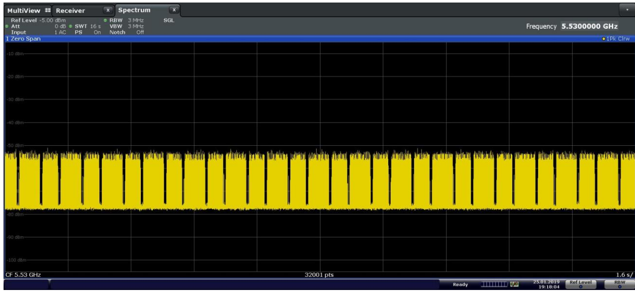
Figure 9-17. 5530MHz - Channel Loading - Mode 3 (80MHz)
