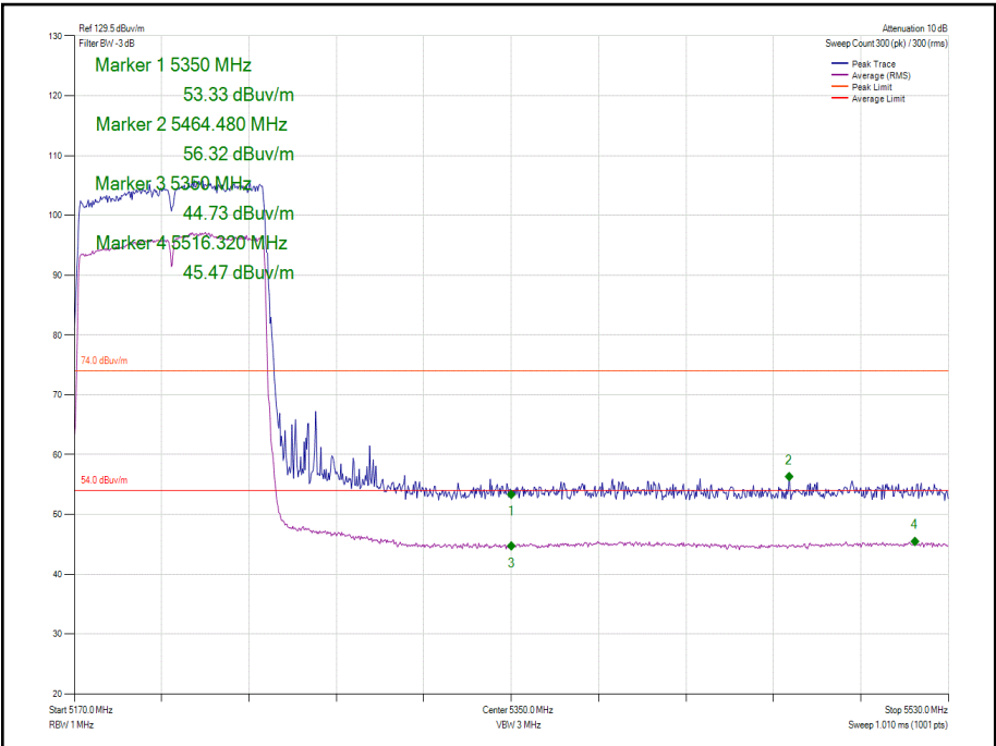
Figure 1132 - 802.11ac VHT80 TxBF Cores 0-1-2 - 5210 MHz Band Edge Frequency 5350 MHz
