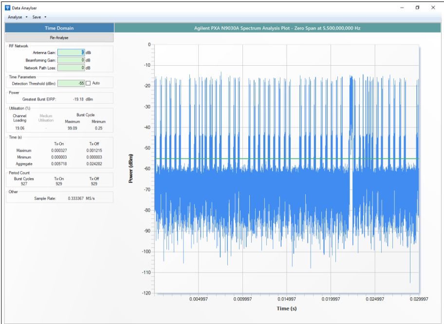
Figure 1165 - Channel Loading
