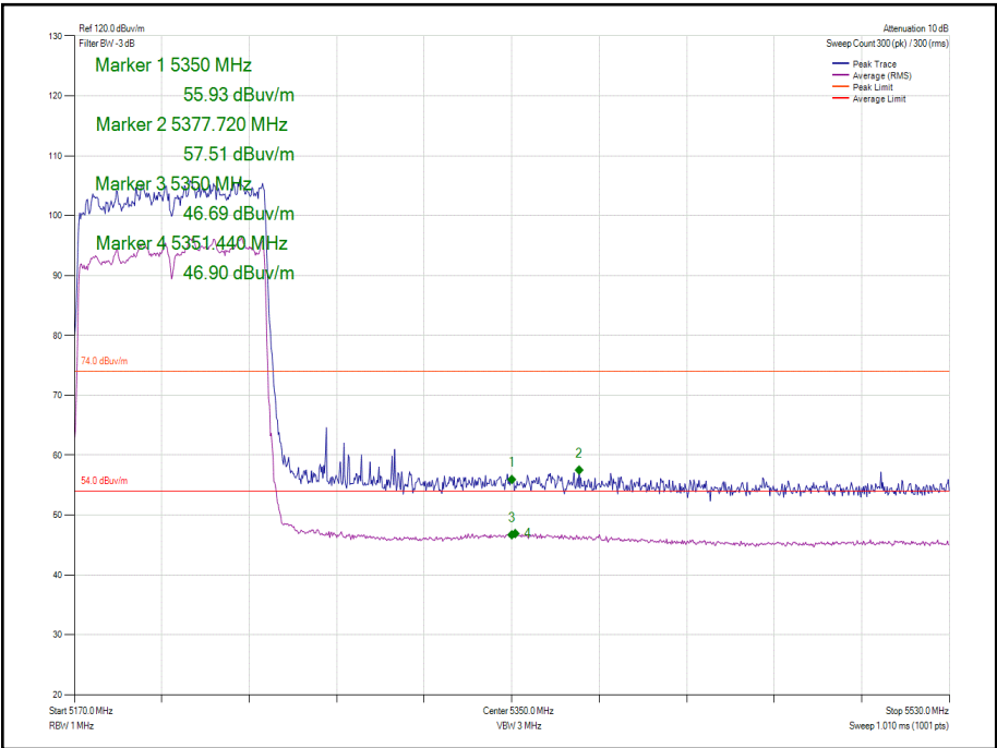
Figure 1131 - 802.11ac VHT80 SDM Cores 0-1-2 - 5210 MHz Band Edge Frequency 5350 MHz
