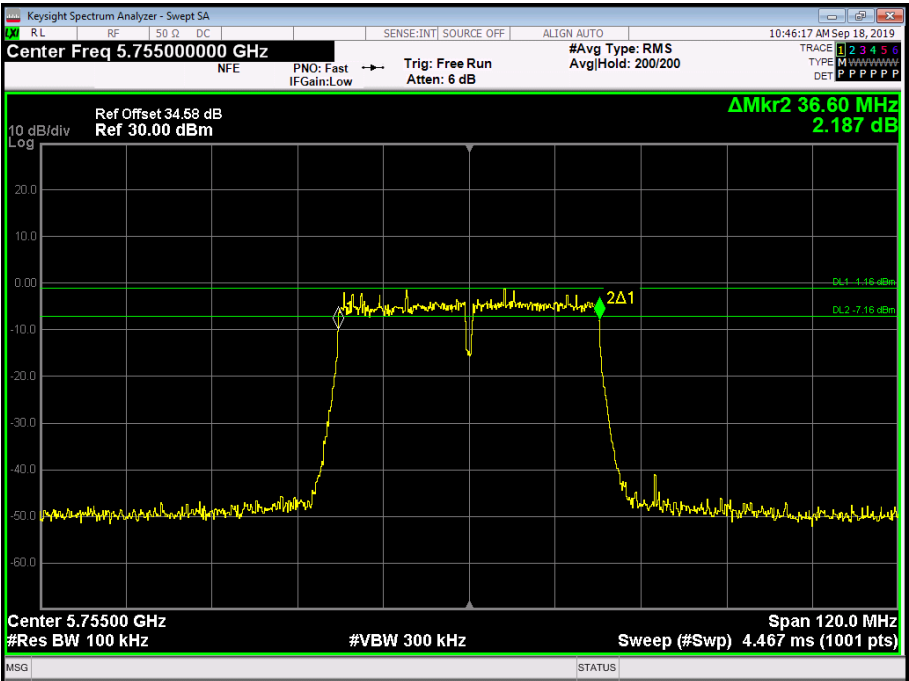
Figure 761 - 5755 MHz - 6 dB DTS Bandwidth
