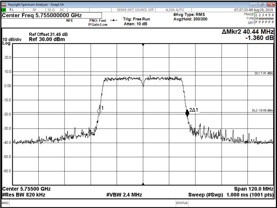
Figure 762 - 5755 MHz - 26 dB Emission Bandwidth
