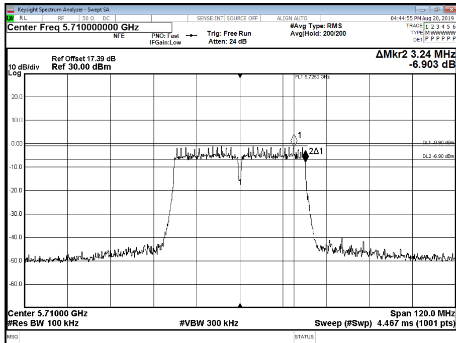
Figure 689 - 5710 MHz - 6 dB DTS Bandwidth
