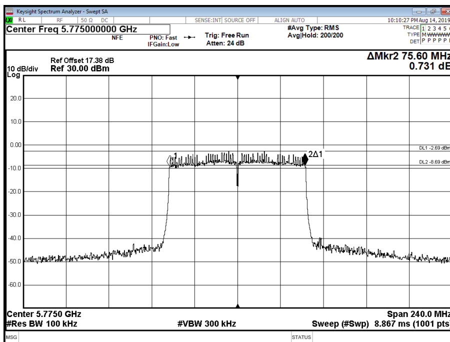
Figure 803 - 5775 MHz - 6 dB DTS Bandwidth
