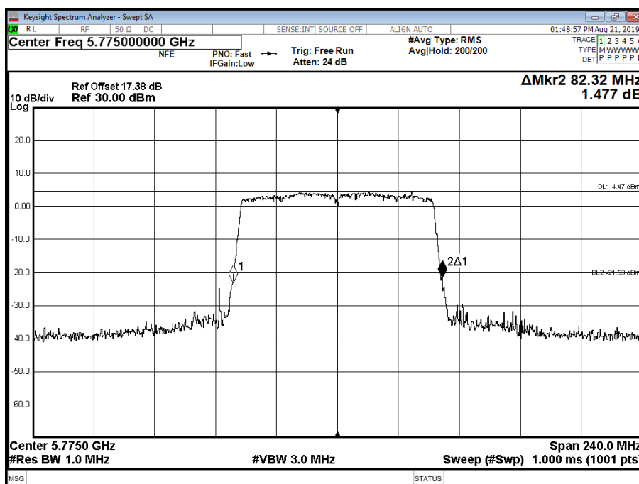
Figure 804 - 5775 MHz - 26 dB Emission Bandwidth
