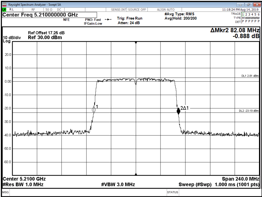
Figure 235 - 5210 MHz - 26 dB Emission Bandwidth
