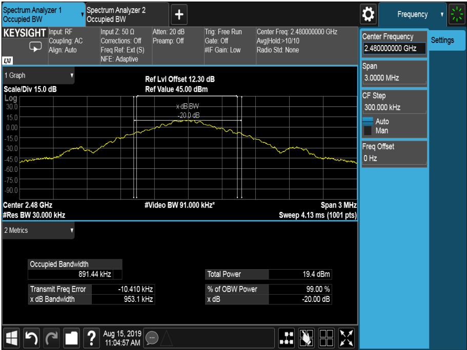
Figure 22 - 2480 MHz - GFSK
