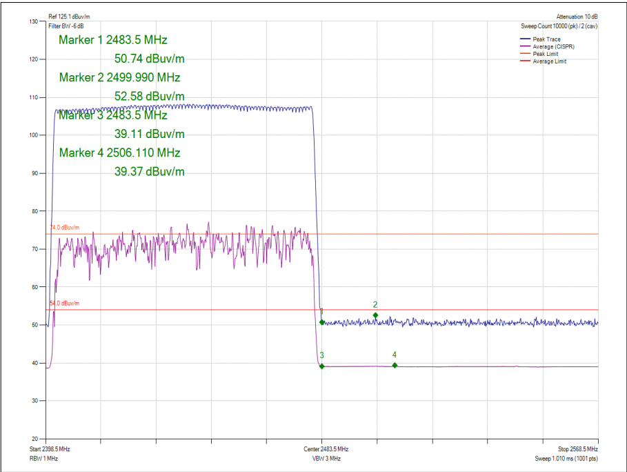
Figure 41 - Hopping - \pi/4 DQPSK/2DH5 - Band Edge Frequency 2483.5 MHz
