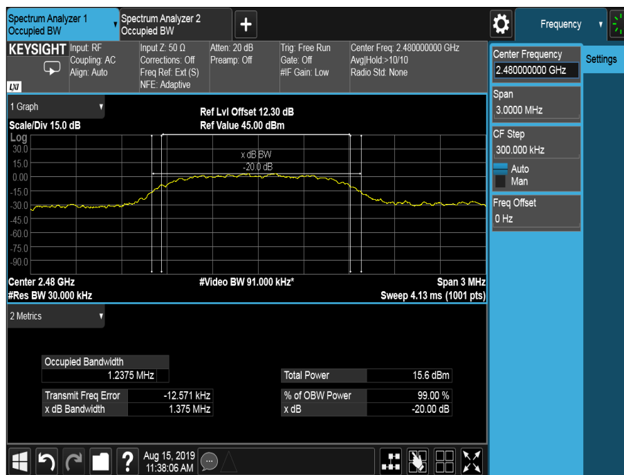
Figure 24 - 2480 MHz - 8-DPSK
