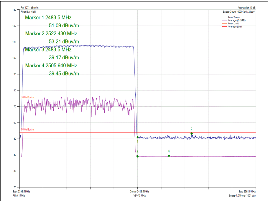
Figure 42 - Hopping - 8-DPSK/3DH5 - Band Edge Frequency 2483.5 MHz
