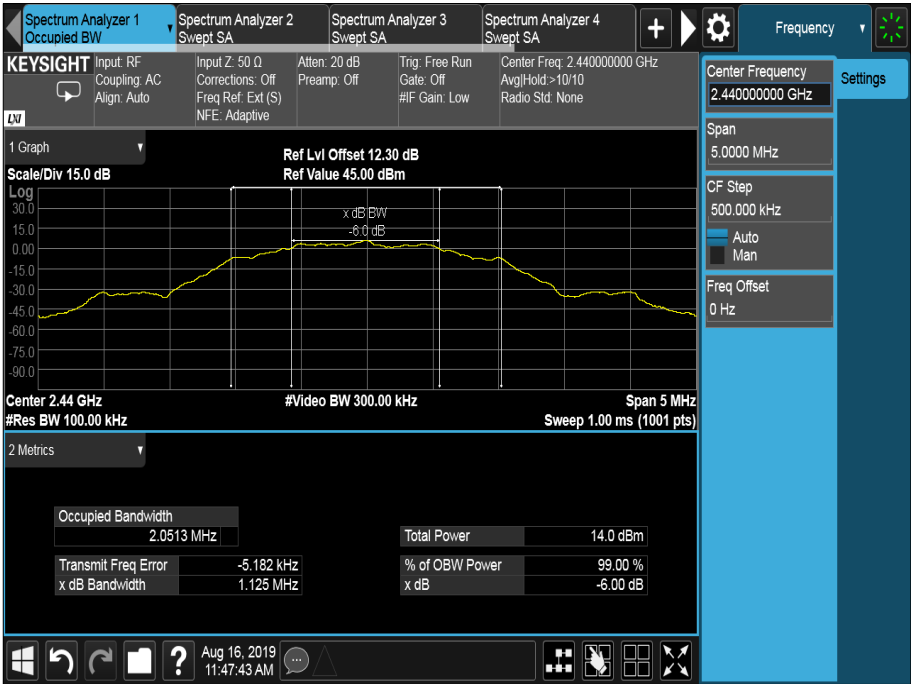
Figure 13 - 2440 MHz
