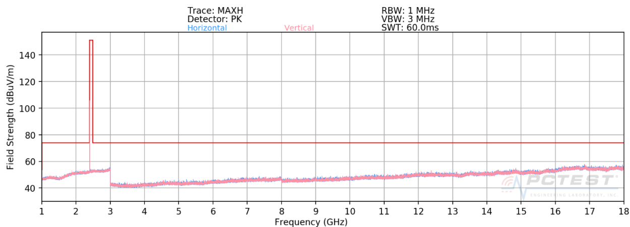
Plot 7-106. Radiated Spurious Plot above 1GHz ANT 1 (BT GFSK ePA – Ch. 0)
