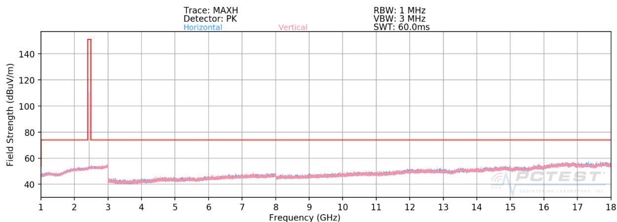
Plot 7-107. Radiated Spurious Plot above 1GHz ANT 1 (BT GFSK ePA – Ch. 39)
