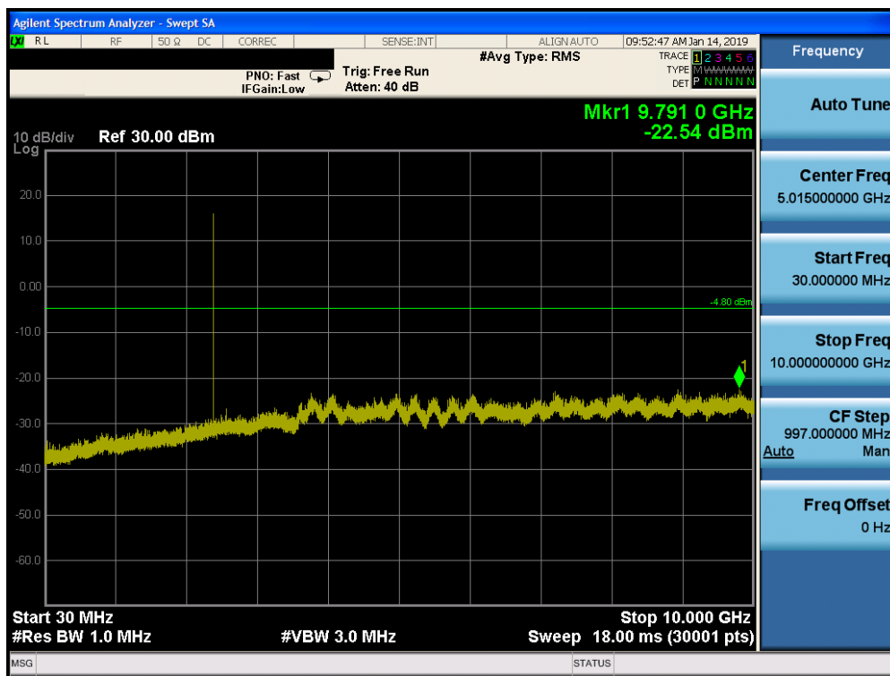
Plot 7-91. Conducted Spurious Plot ANT 2 (Bluetooth, GFSK, ePA – Ch. 0)
