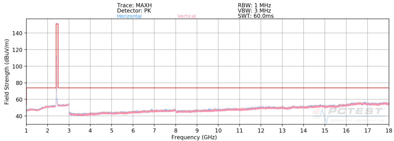
Plot 7-139. Radiated Spurious Plot above 1GHz SISO CORE 1 (802.11b – Ch. 1)
