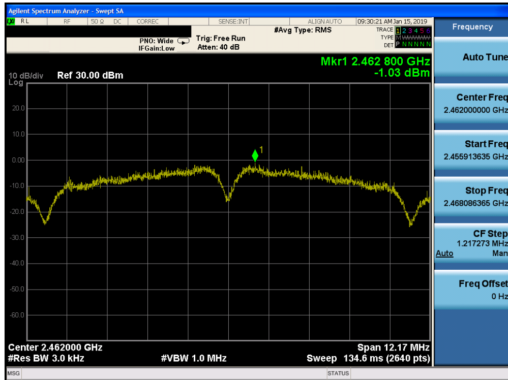
Plot 7-30. Power Spectral Density Plot SISO CORE 0 PRIMARY (802.11b – Ch. 11)
