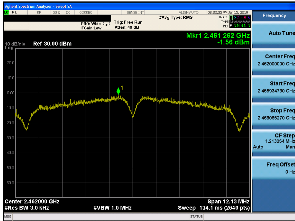
Plot 7-48. Power Spectral Density Plot SISO CORE 1 (802.11b – Ch. 11)
