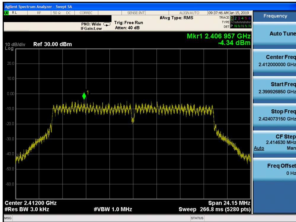
Plot 7-31. Power Spectral Density Plot SISO CORE 0 PRIMARY (802.11g – Ch. 1)
