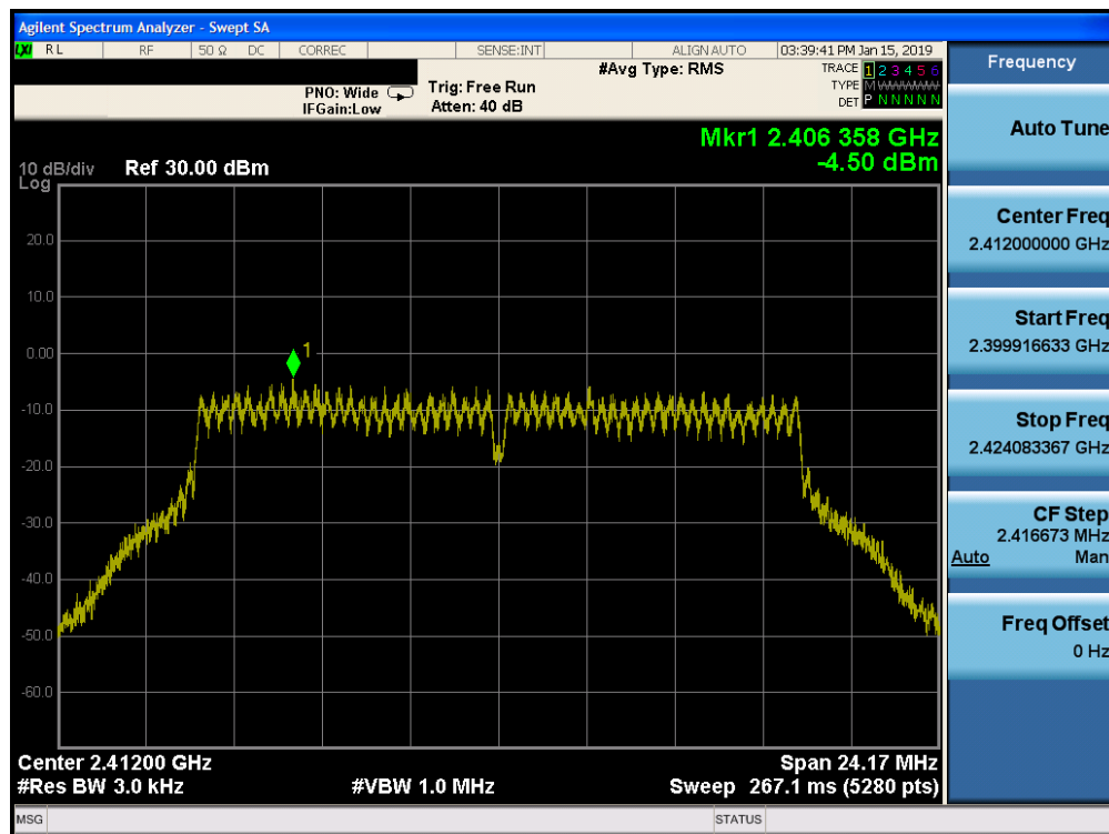
Plot 7-49. Power Spectral Density Plot SISO CORE 1 (802.11g – Ch. 1)
