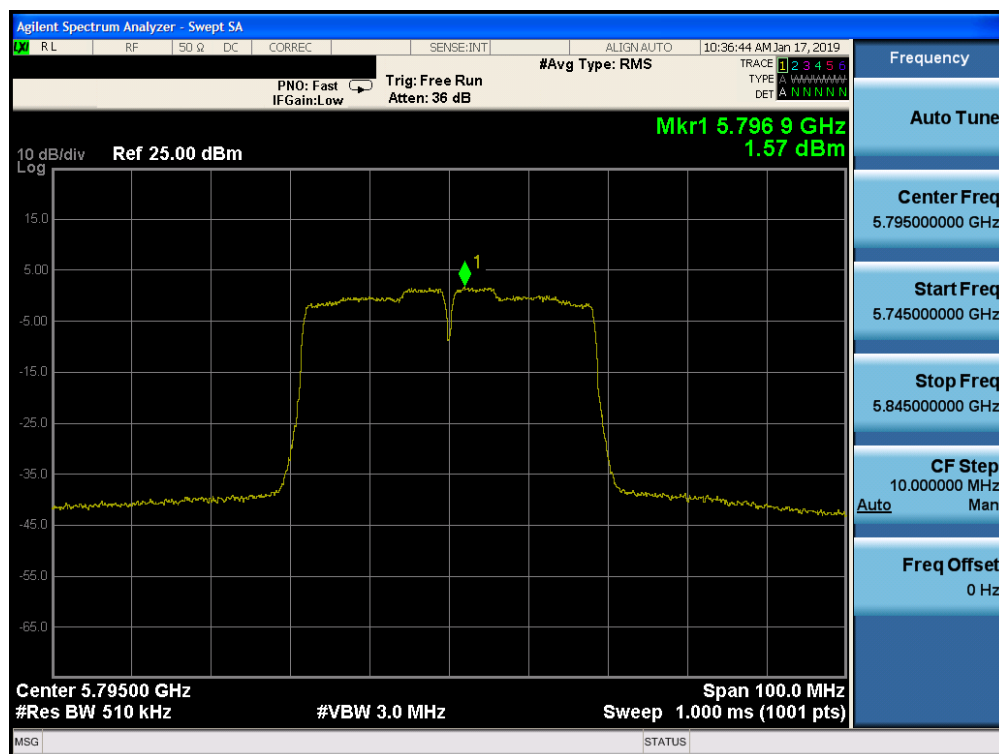
Plot 7-154. Power Spectral Density Plot MIMO/CDD CORE 1 (40MHz BW 802.11n (UNII Band 3) – Ch. 159)
