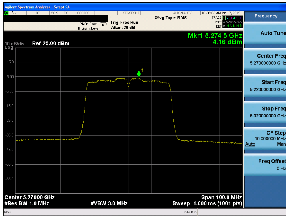
Plot 7-124. Power Spectral Density Plot MIMO/CDD CORE 1 (40MHz BW 802.11n (UNII Band 2A) – Ch. 54)
