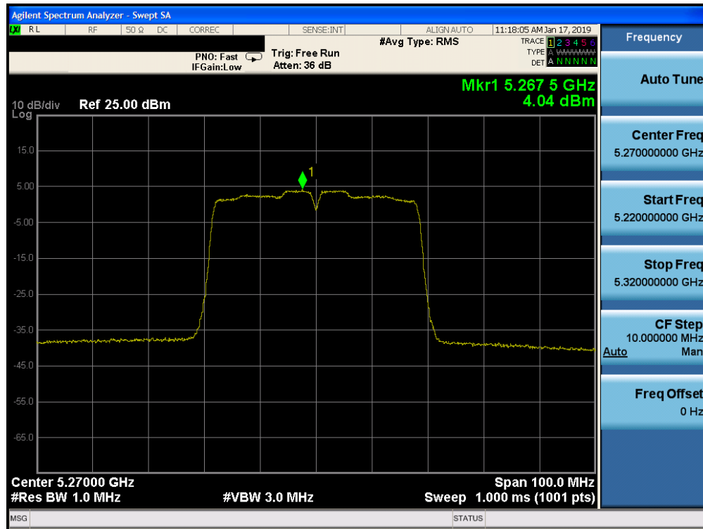
Plot 7-123. Power Spectral Density Plot MIMO/CDD CORE 0 (40MHz BW 802.11n (UNII Band 2A) – Ch. 54)
