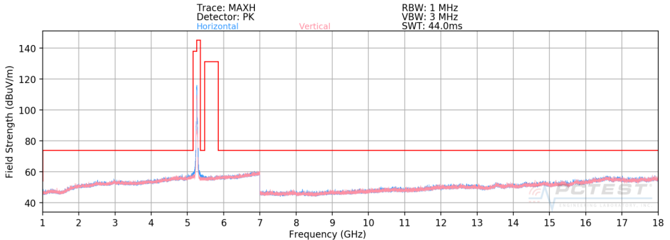
Plot 7-172. Radiated Spurious Plot above 1GHz SISO CORE 1 (802.11n – U2A Ch. 52)
