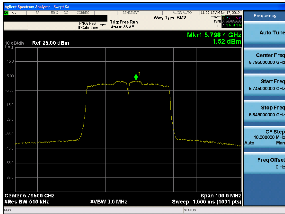
Plot 7-153. Power Spectral Density Plot MIMO/CDD CORE 0 (40MHz BW 802.11n (UNII Band 3) – Ch. 159)
