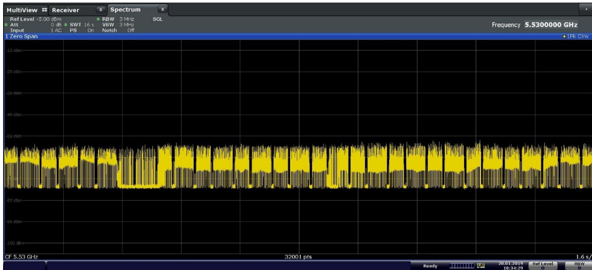
Figure 9-11. 5530MHz - Channel Loading - Mode 2 (80MHz)
