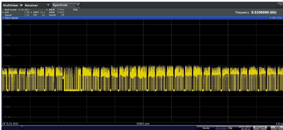
Figure 9-9. 5510MHz - Channel Loading - Mode 2 (40MHz)
