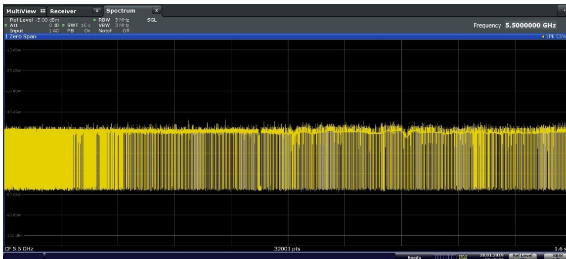
Figure 9-1. 5500MHz - Channel Loading - Mode 1 (20MHz)
