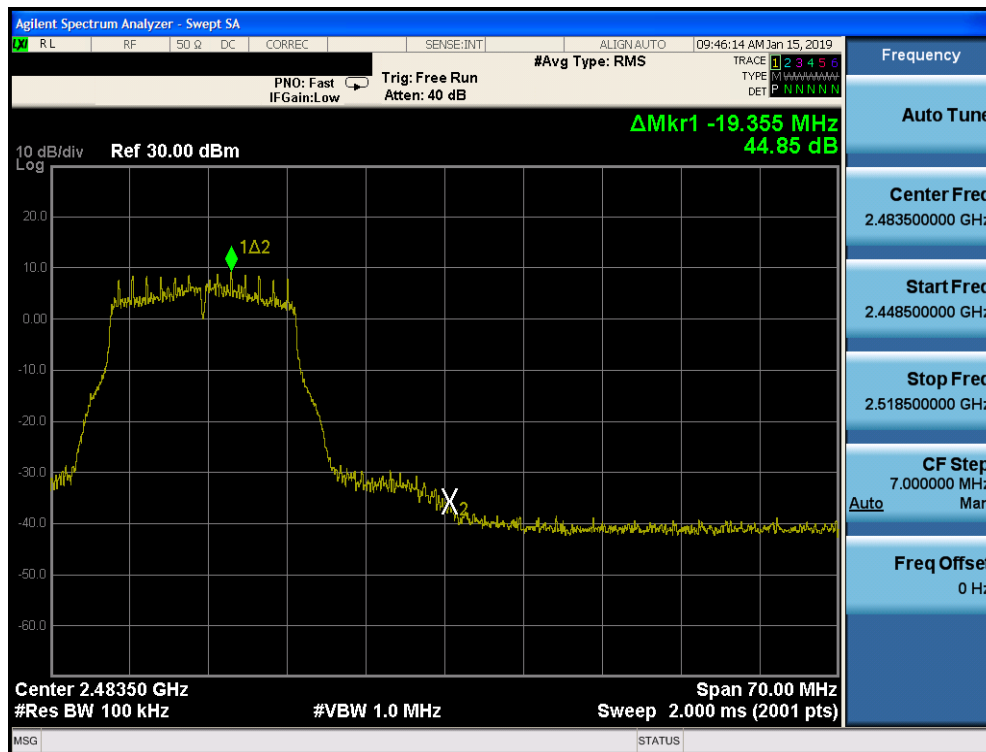
Plot 7-84. Band Edge Plot SISO CORE 0 PRIMARY (802.11g - Ch. 11)
