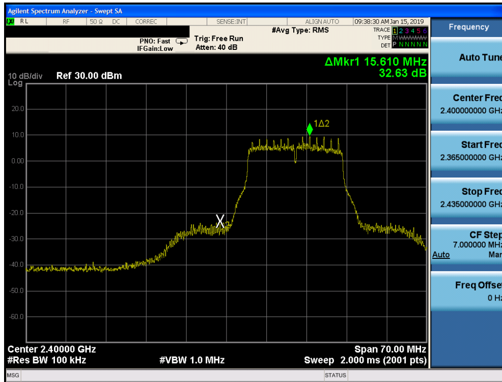
Plot 7-83. Band Edge Plot SISO CORE 0 PRIMARY (802.11g- Ch. 1)
