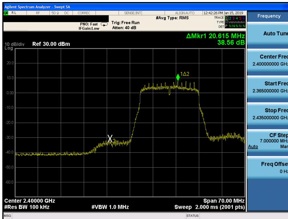
Plot 7-99. Band Edge Plot SISO CORE 0 DIVERSITY (802.11n (2.4GHz) – Ch. 1)
