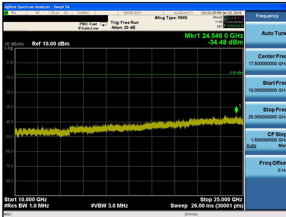
Plot 7-132. Conducted Spurious Plot SISO CORE 1 (802.11b – Ch. 11)
