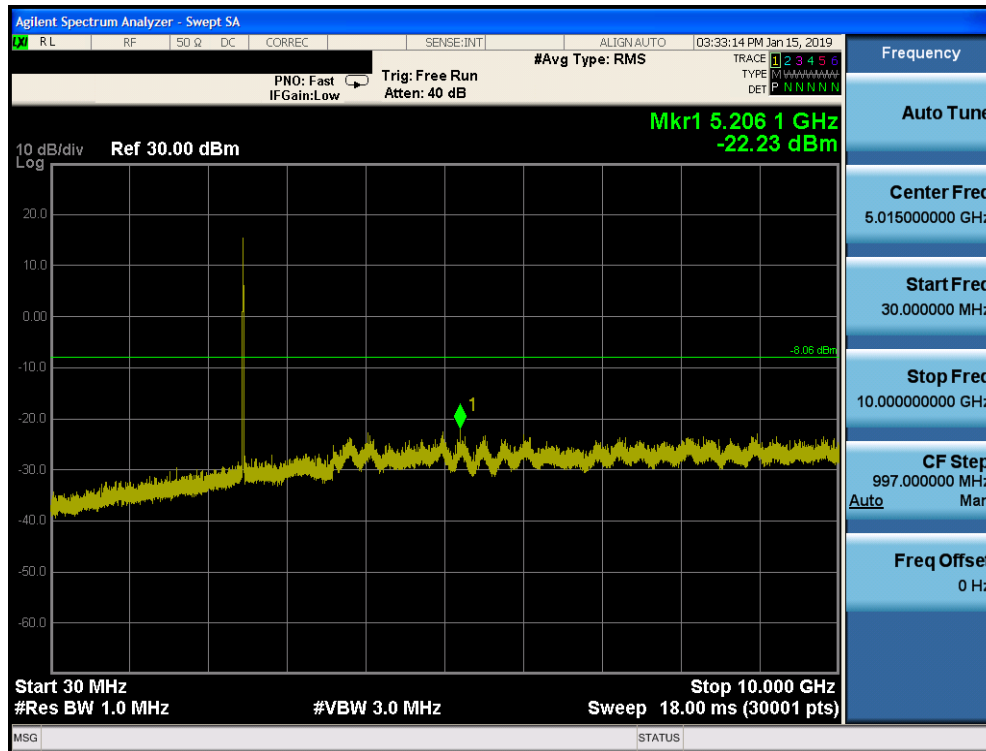
Plot 7-131. Conducted Spurious Plot SISO CORE 1 (802.11b – Ch. 11)
