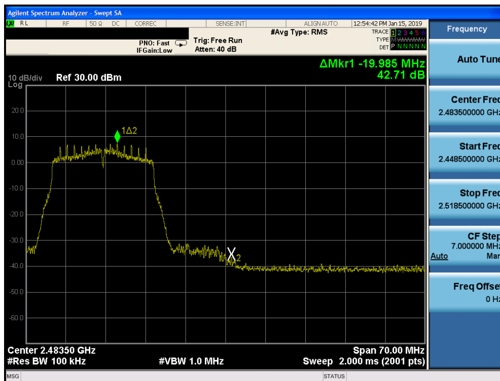
Plot 7-100. Band Edge Plot SISO CORE 0 DIVERSITY (802.11n – Ch. 11)
