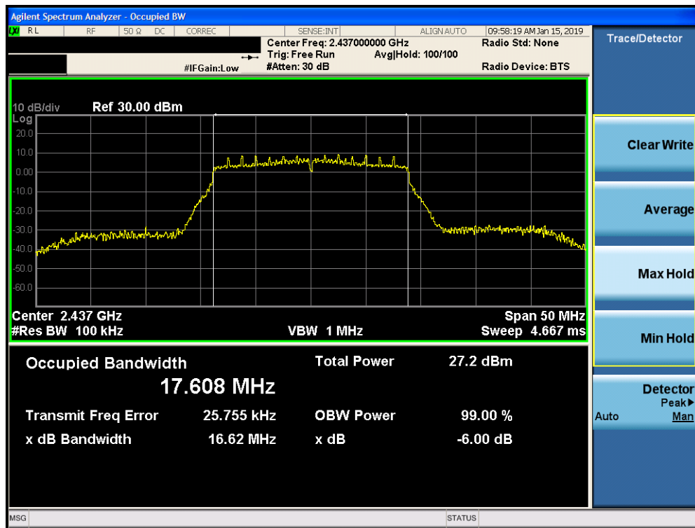
Plot 7-8. 6dB Bandwidth Plot SISO CORE 0 PRIMARY (802.11n (2.4GHz) – Ch. 6)
