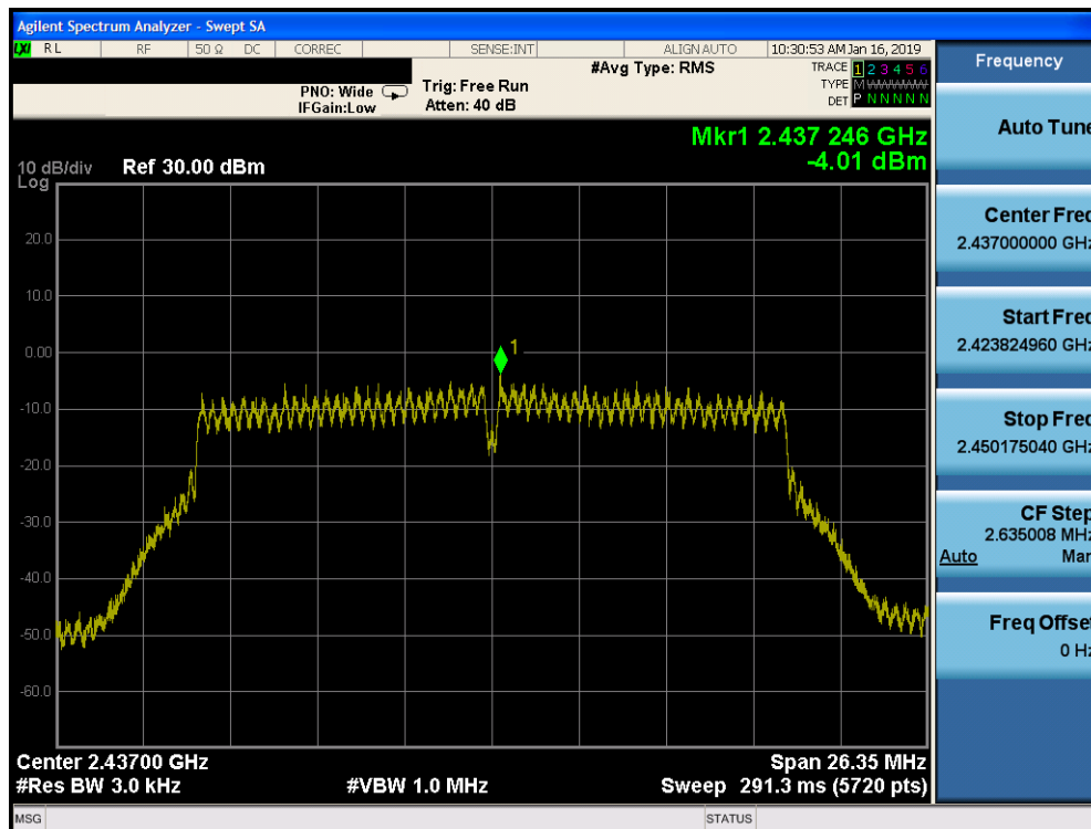
Plot 7-64. Power Spectral Density Plot CDD PRIMARY CORE 1 (802.11n (2.4GHz) – Ch. 6)
