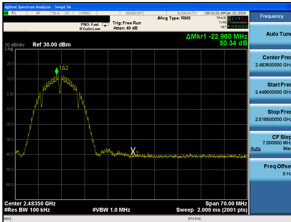
Plot 7-80. Band Edge Plot SISO CORE 0 PRIMARY (802.11b – Ch. 11)
