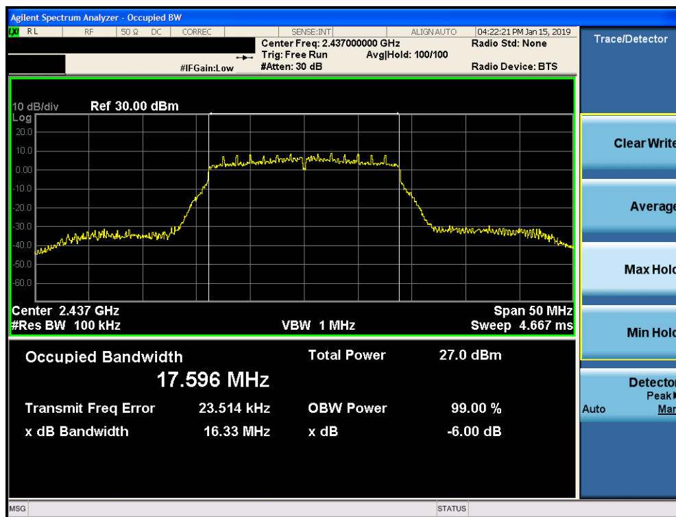
Plot 7-26. 6dB Bandwidth Plot SISO CORE 1 (802.11n) (2.4GHz) – Ch. 6)
