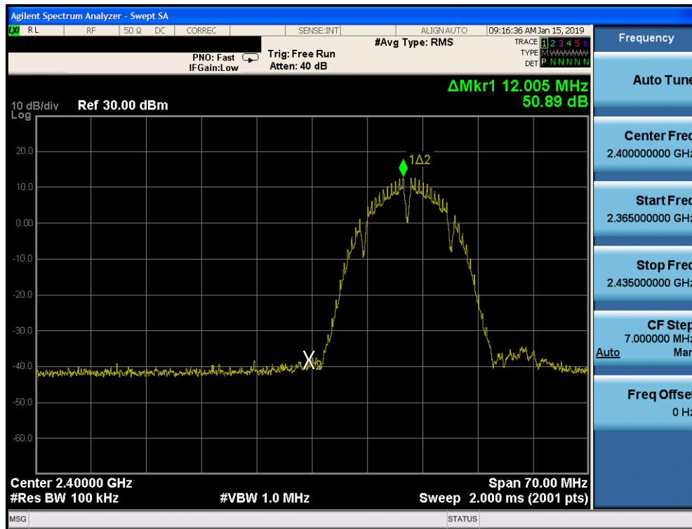
Plot 7-79. Band Edge Plot SISO CORE 0 PRIMARY (802.11b – Ch. 1)
