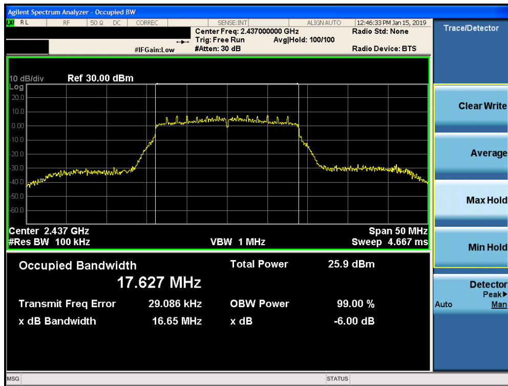
Plot 7-17. 6dB Bandwidth Plot SISO CORE 0 DIVERSITY (802.11n (2.4GHz) – Ch. 6)
