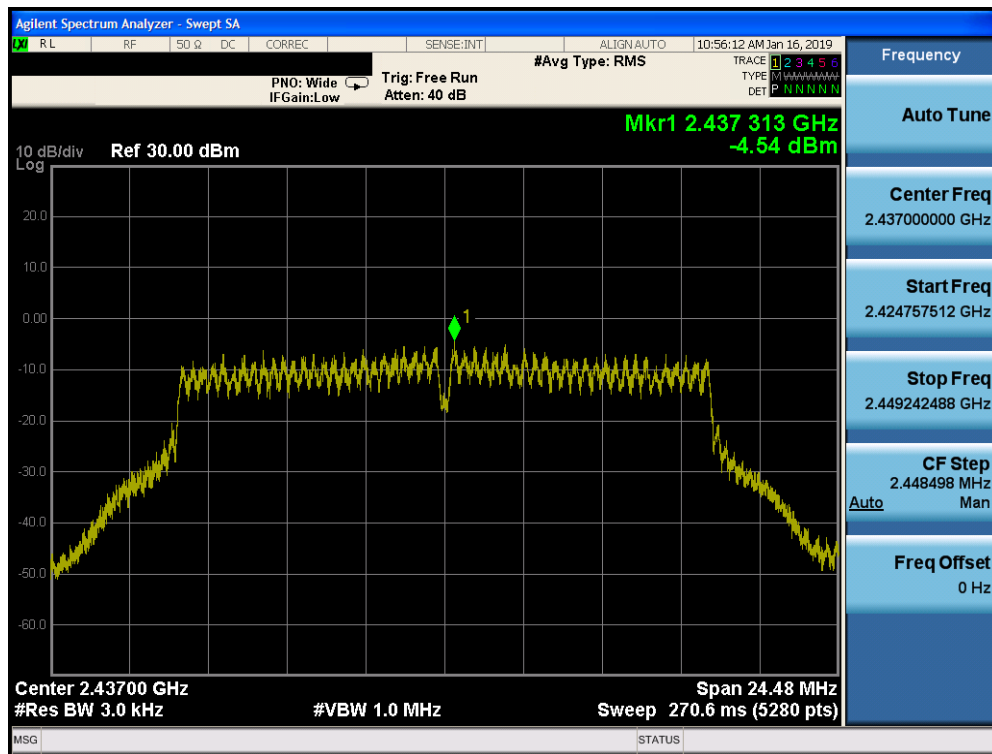
Plot 7-70. Power Spectral Density Plot CDD CORE 1 (802.11g – Ch. 6)
