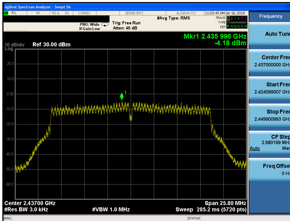
Plot 7-76. Power Spectral Density Plot CDD CORE 1 (802.11n (2.4GHz) – Ch. 6)
