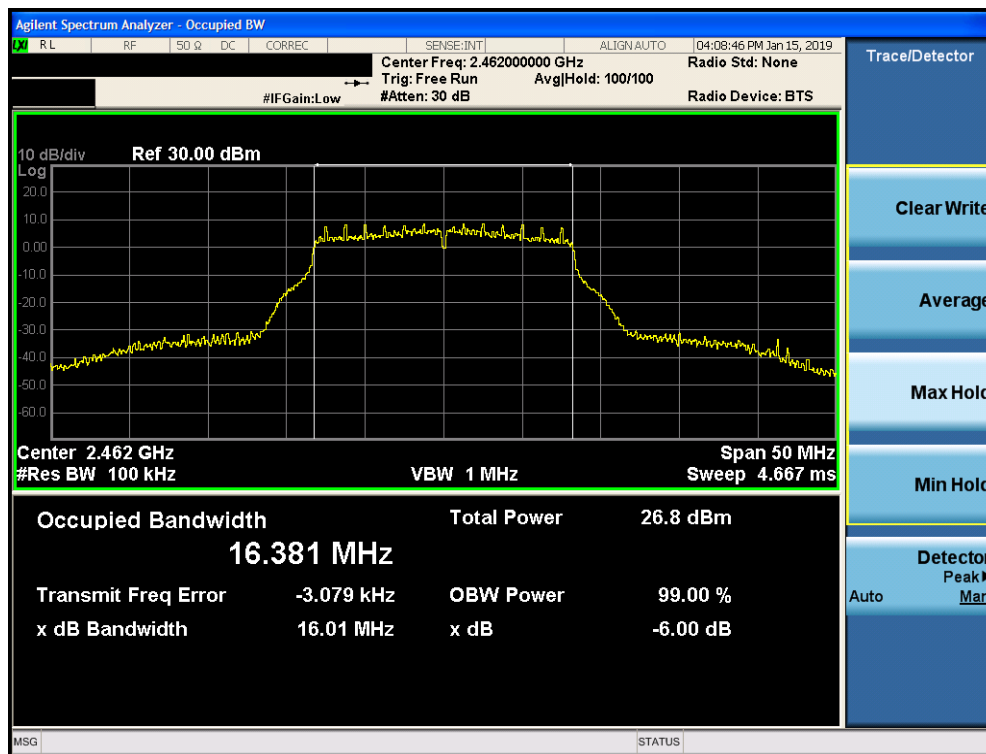
Plot 7-24. 6dB Bandwidth Plot SISO CORE 1 (802.11g – Ch. 11)
