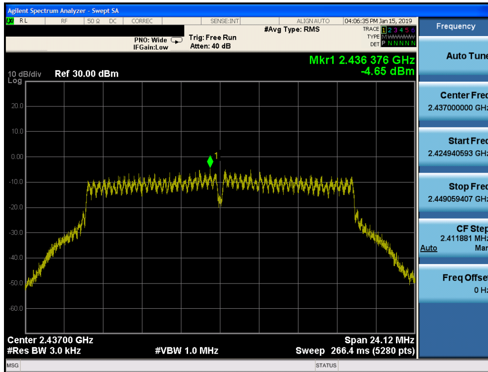
Plot 7-50. Power Spectral Density Plot SISO CORE 1 (802.11g – Ch. 6)
