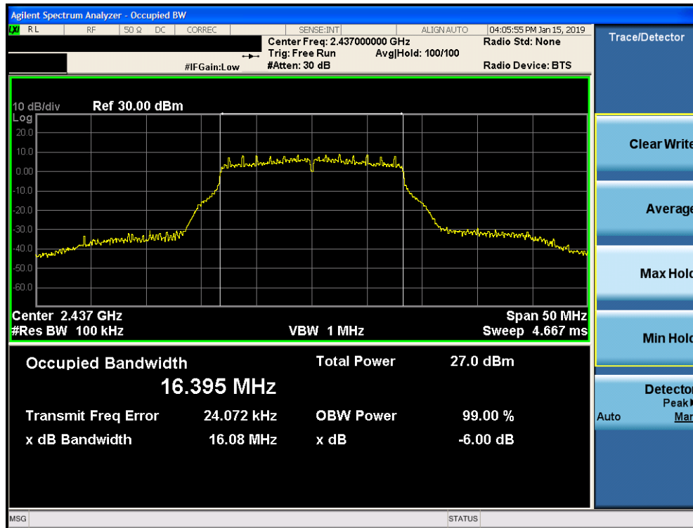
Plot 7-23. 6dB Bandwidth Plot SISO CORE 1 (802.11g – Ch. 6)
