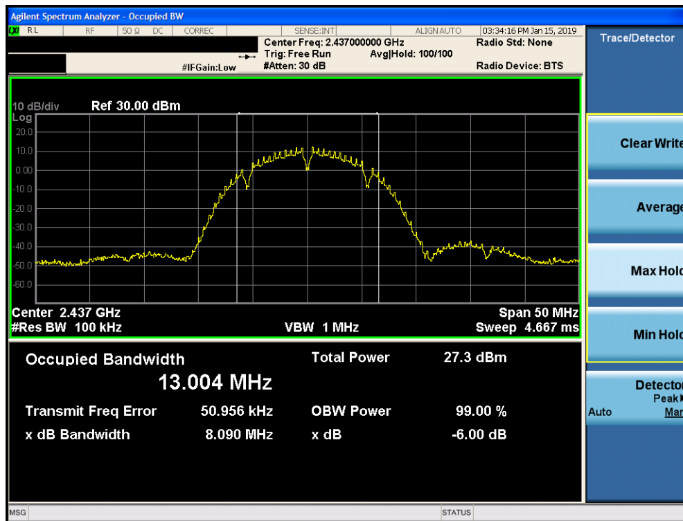
Plot 7-20. 6dB Bandwidth Plot SISO CORE 1 (802.11b – Ch. 6)
