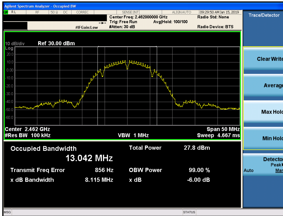
Plot 7-3. 6dB Bandwidth Plot SISO CORE 0 PRIMARY (802.11b – Ch. 11)
