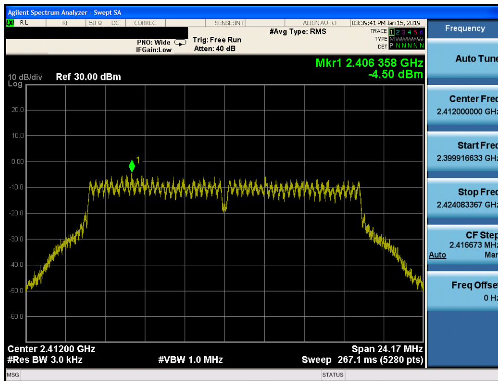
Plot 7-49. Power Spectral Density Plot SISO CORE 1 (802.11g – Ch. 1)
