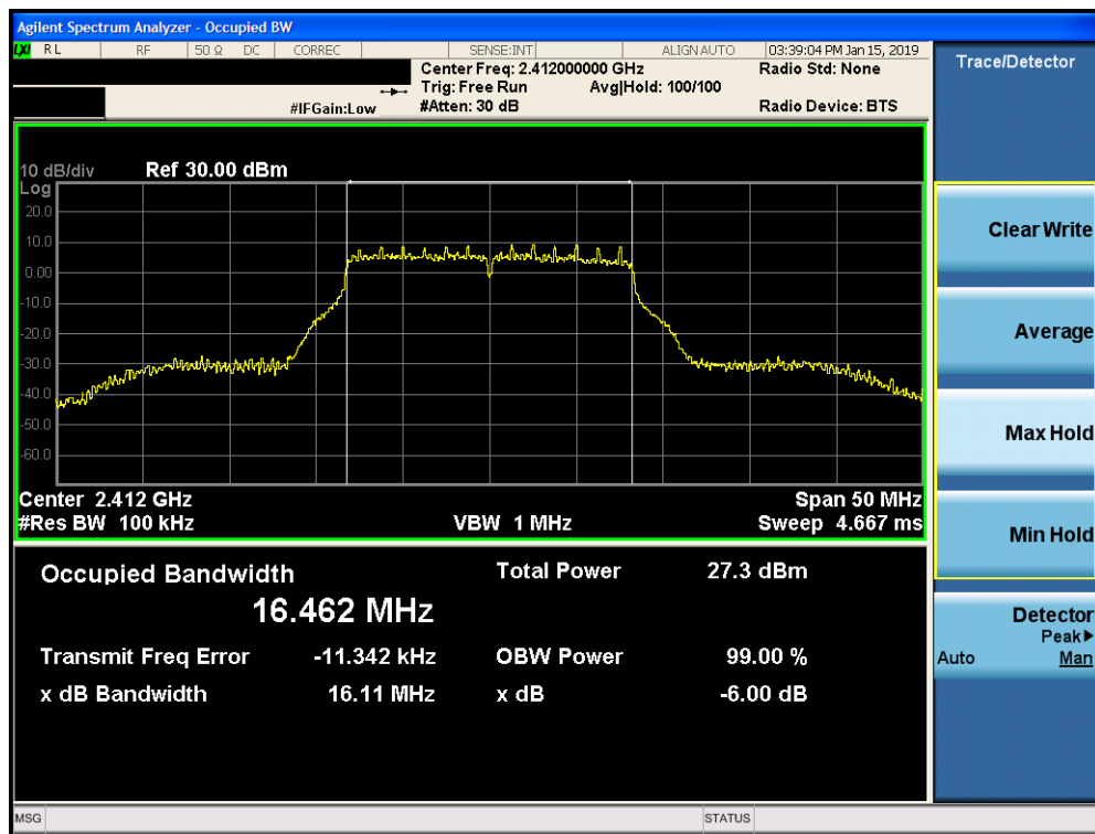
Plot 7-22. 6dB Bandwidth Plot SISO CORE 1 (802.11g – Ch. 1)
