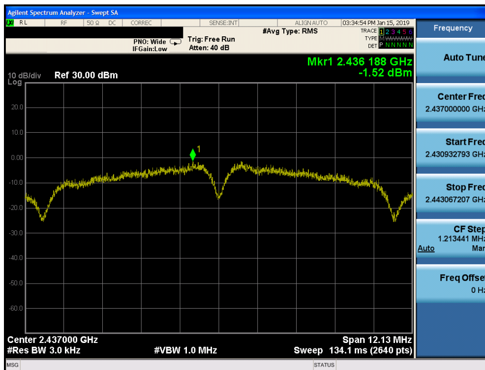
Plot 7-47. Power Spectral Density Plot SISO CORE 1 (802.11b – Ch. 6)
