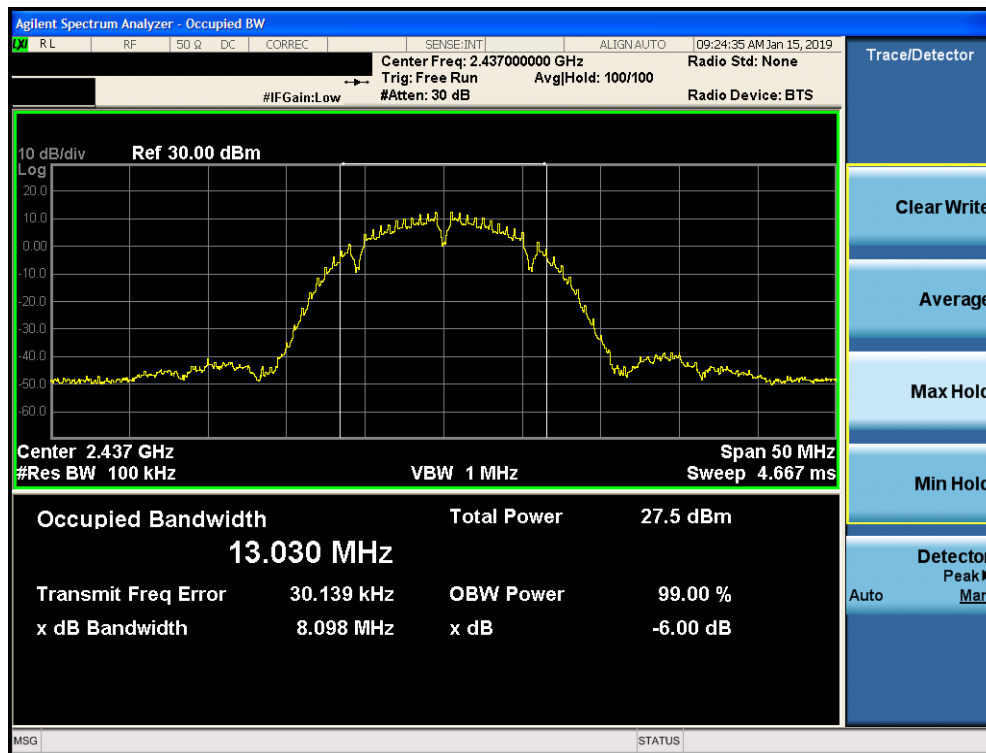
Plot 7-2. 6dB Bandwidth Plot SISO CORE 0 PRIMARY (802.11b – Ch. 6)
