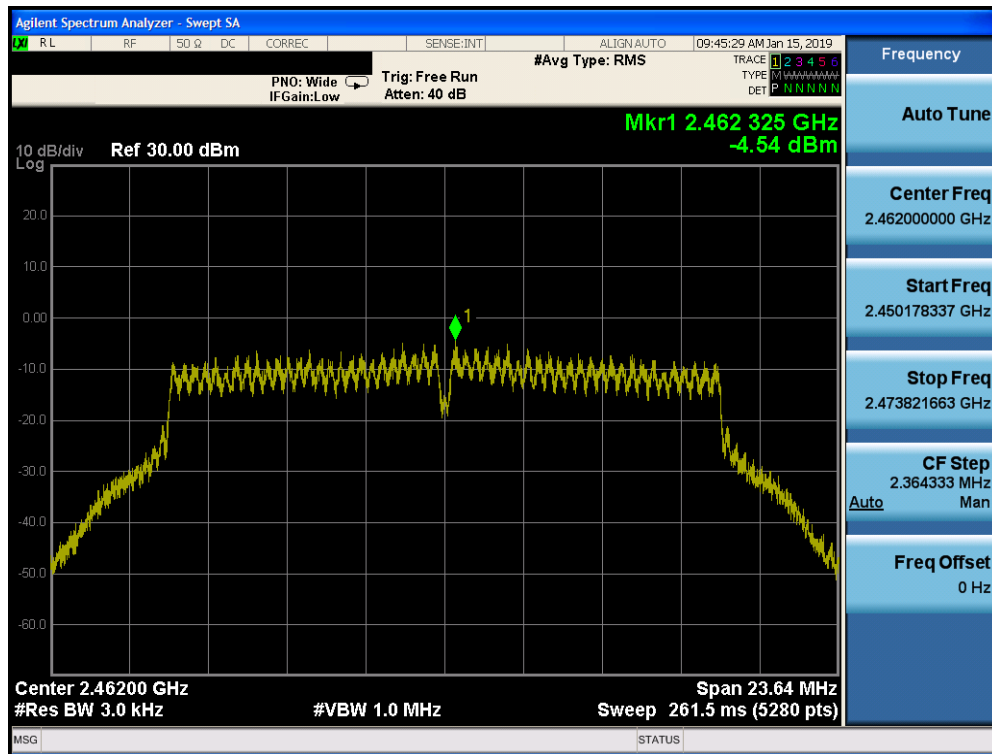
Plot 7-33. Power Spectral Density Plot SISO CORE 0 PRIMARY (802.11g – Ch. 11)
