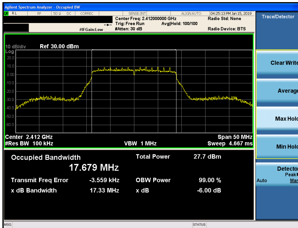
Plot 7-25. 6dB Bandwidth Plot SISO CORE 1 (802.11n) (2.4GHz) – Ch. 1)
