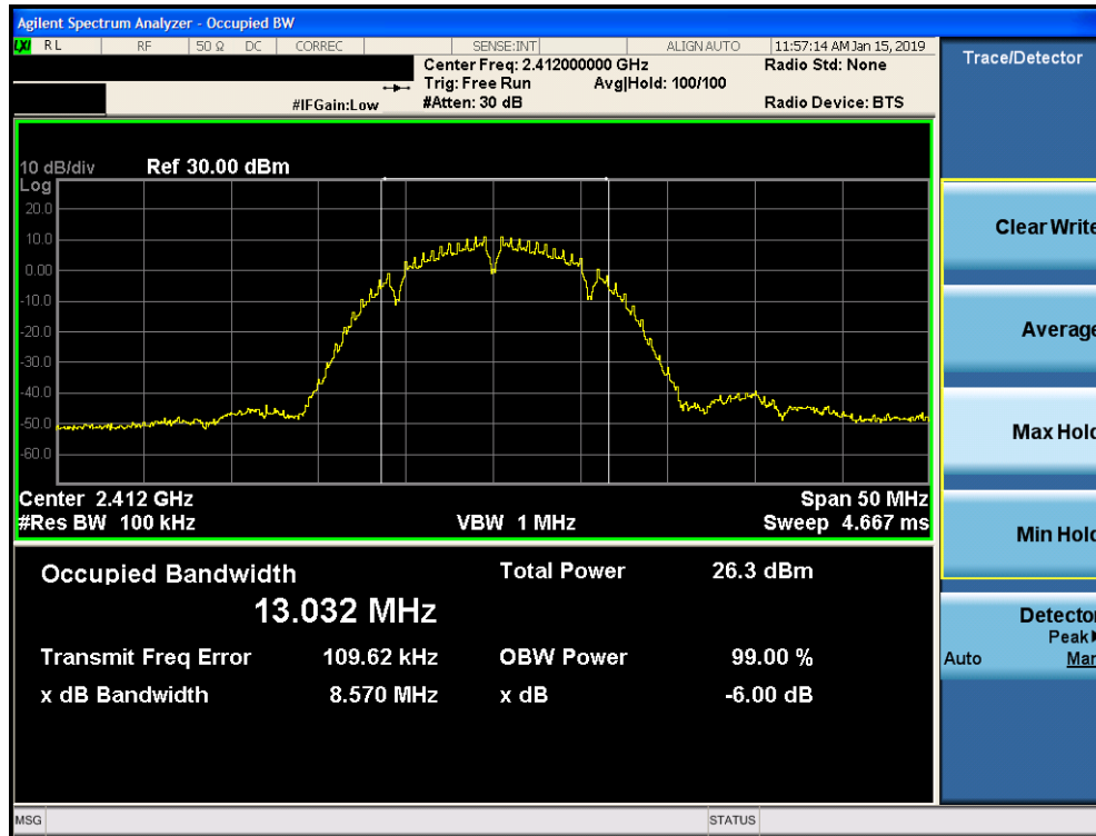
Plot 7-10. 6dB Bandwidth Plot SISO CORE 0 DIVERSITY (802.11b – Ch. 1)
