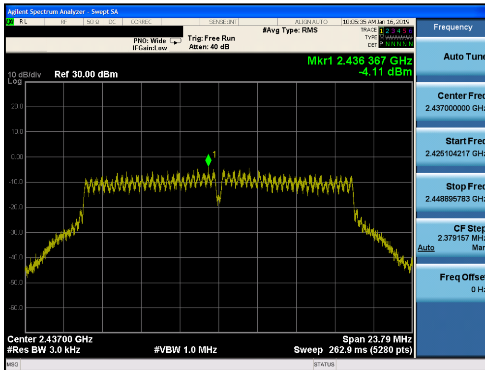
Plot 7-57. Power Spectral Density Plot CDD PRIMARY CORE 0 (802.11g – Ch. 6)
