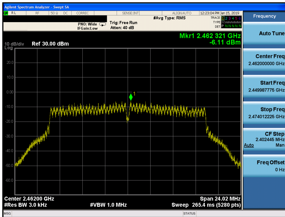
Plot 7-42. Power Spectral Density Plot SISO CORE 0 DIVERSITY (802.11g – Ch. 11)
