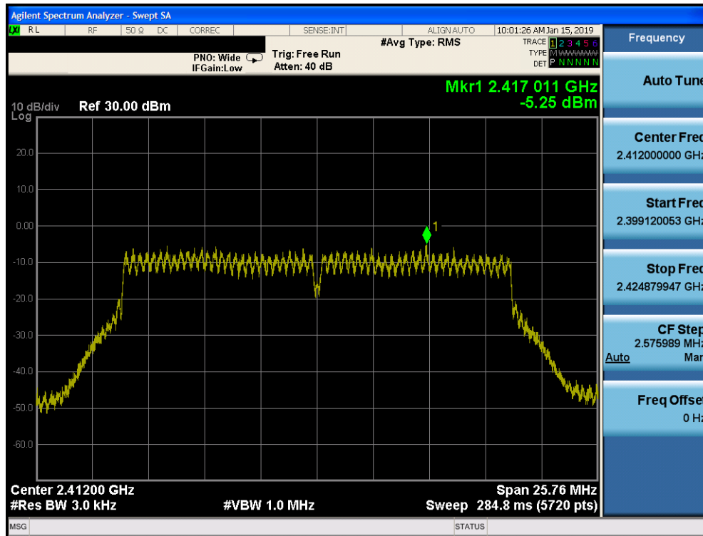
Plot 7-34. Power Spectral Density Plot SISO CORE 0 PRIMARY (802.11n (2.4GHz) – Ch. 1)
