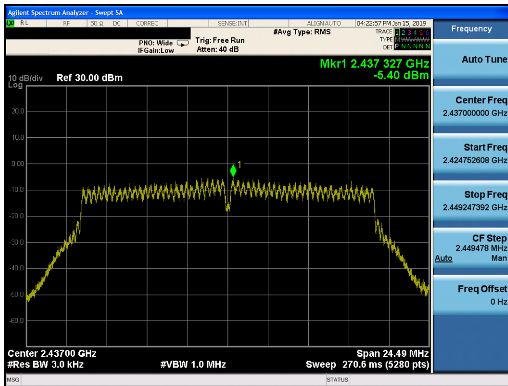
Plot 7-53. Power Spectral Density Plot SISO CORE 1 (802.11n (2.4GHz) – Ch. 6)
