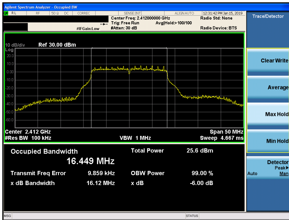
Plot 7-13. 6dB Bandwidth Plot SISO CORE 0 DIVERSITY (802.11g – Ch. 1)
