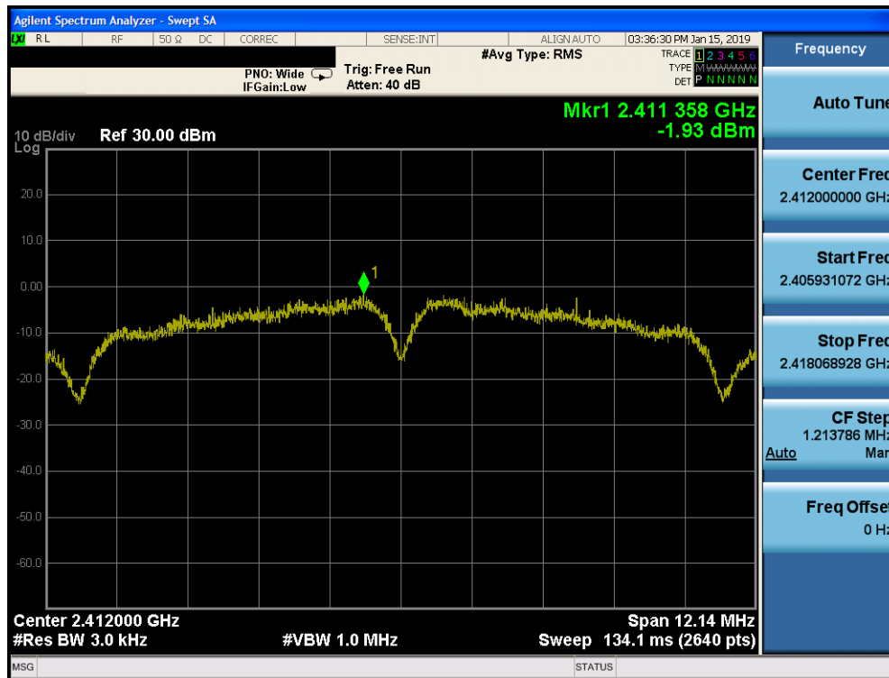
Plot 7-46. Power Spectral Density Plot SISO CORE 1 (802.11b – Ch. 1)
