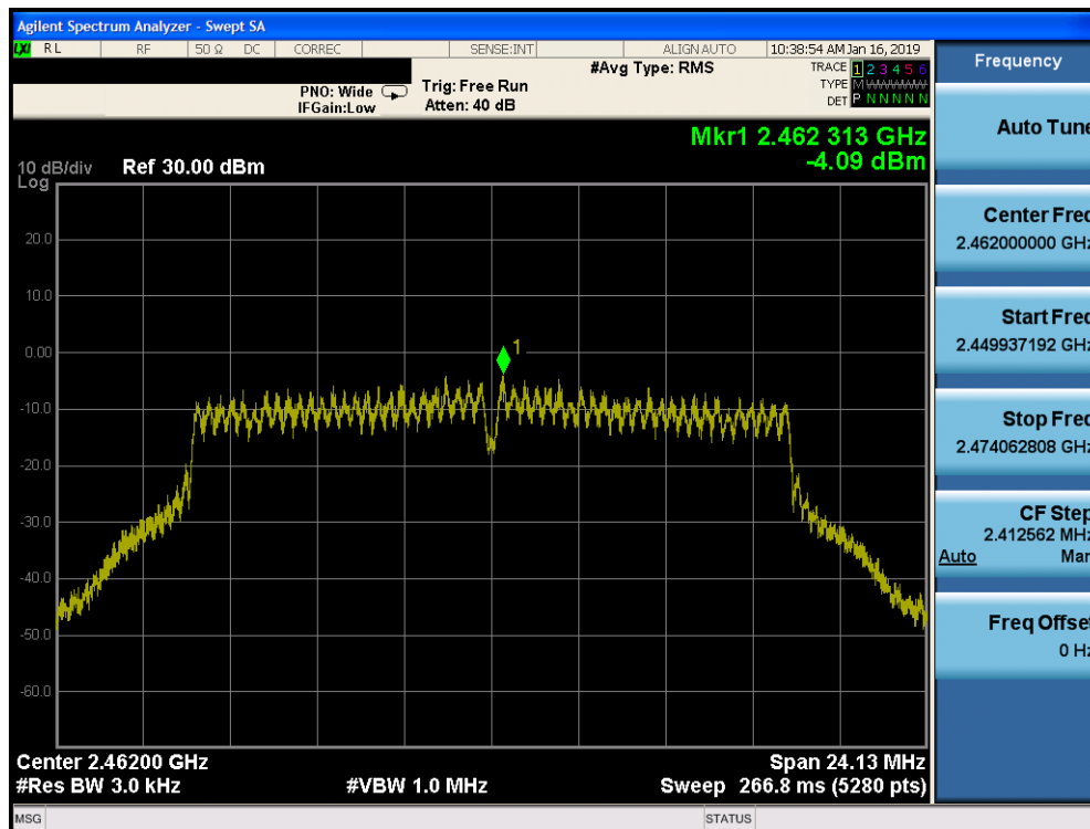
Plot 7-60. Power Spectral Density Plot CDD PRIMARY CORE 1 (802.11g – Ch. 11)
