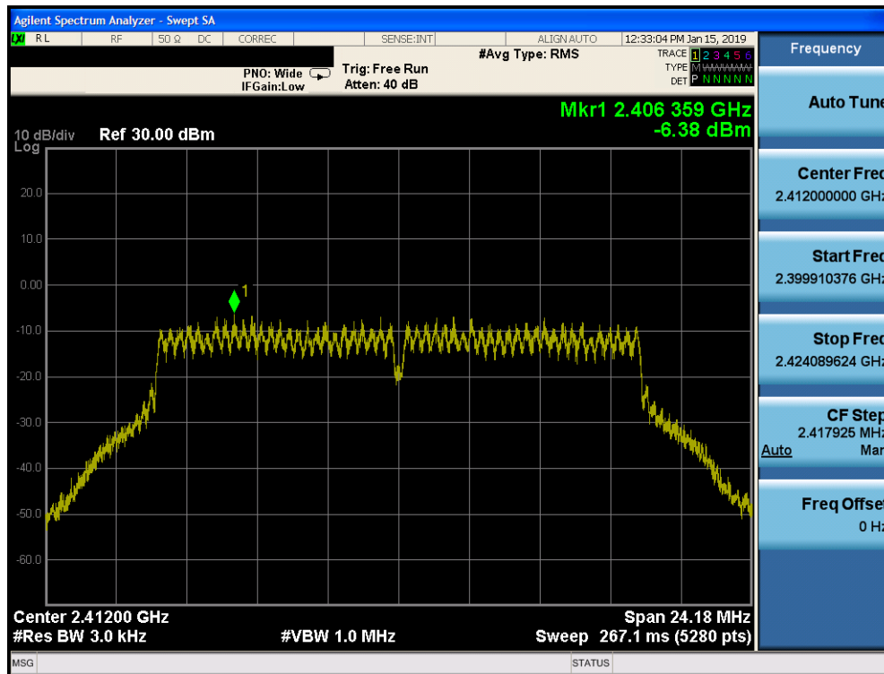
Plot 7-40. Power Spectral Density Plot SISO CORE 0 DIVERSITY (802.11g – Ch. 1)
