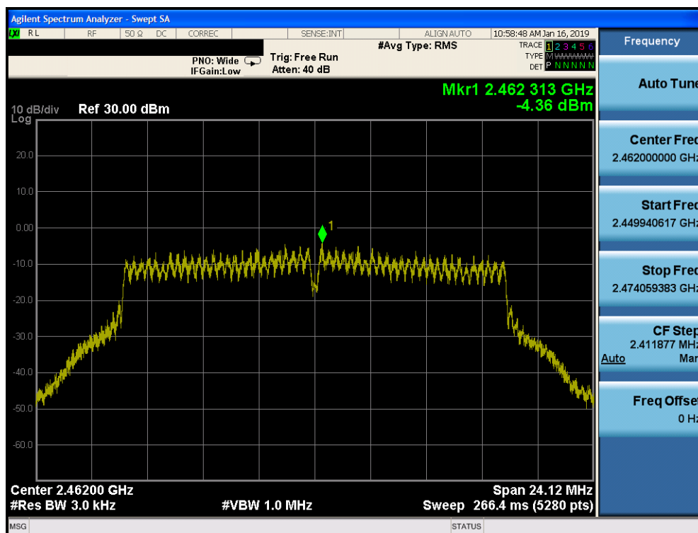
Plot 7-72. Power Spectral Density Plot CDD CORE 1 (802.11g – Ch. 11)
