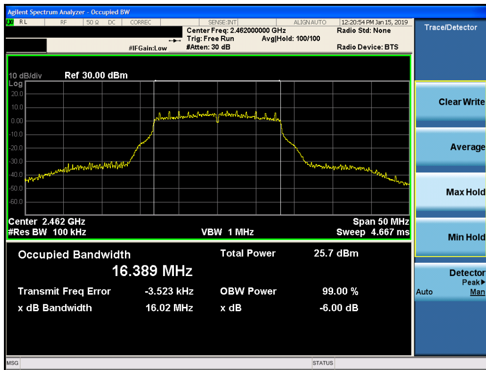
Plot 7-15. 6dB Bandwidth Plot SISO CORE 0 DIVERSITY (802.11g – Ch. 11)
