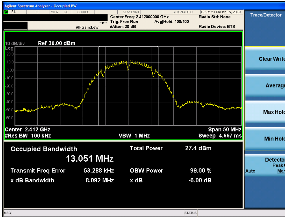
Plot 7-19. 6dB Bandwidth Plot SISO CORE 1 (802.11b – Ch. 1)
