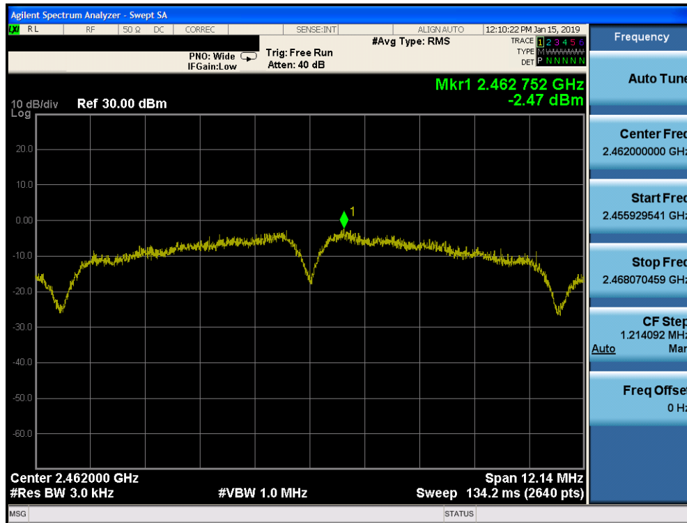
Plot 7-39. Power Spectral Density Plot SISO CORE 0 DIVERSITY (802.11b – Ch. 11)
