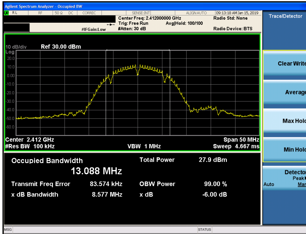
Plot 7-1. 6dB Bandwidth Plot SISO CORE 0 PRIMARY (802.11b – Ch. 1)
