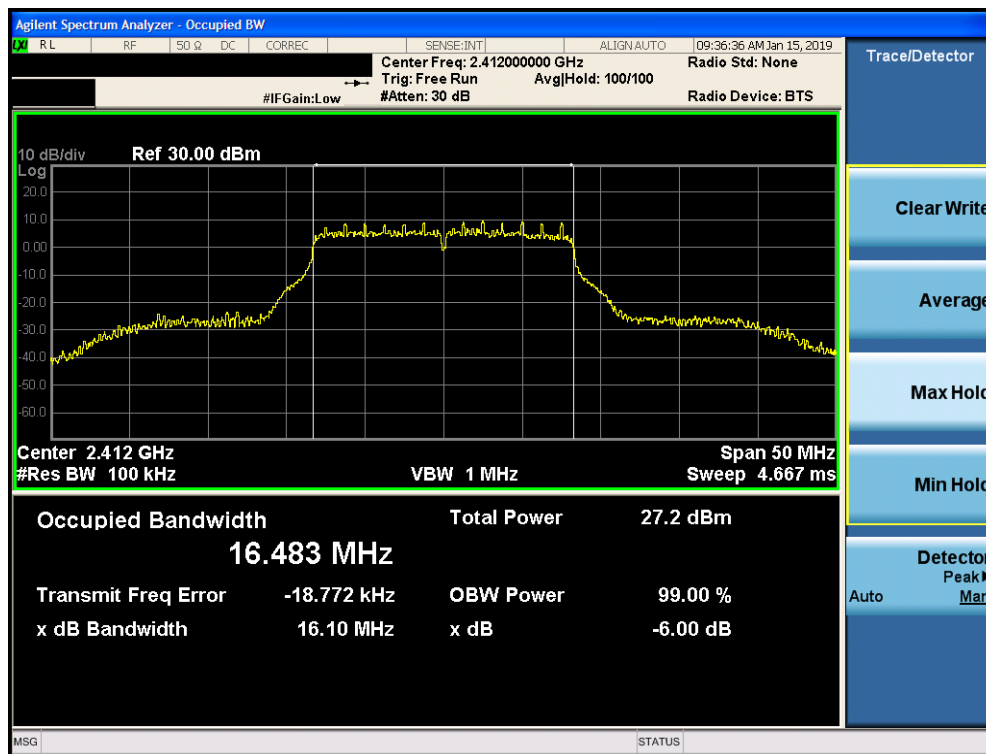
Plot 7-4. 6dB Bandwidth Plot SISO CORE 0 PRIMARY (802.11g – Ch. 1)
