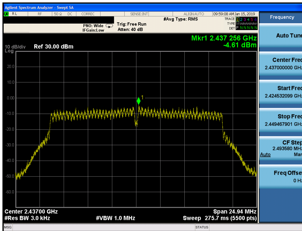
Plot 7-35. Power Spectral Density Plot SISO CORE 0 PRIMARY (802.11n (2.4GHz) – Ch. 6)
