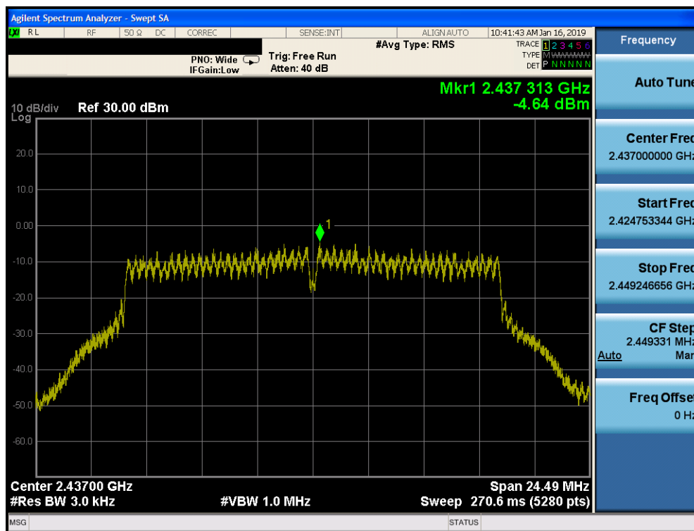
Plot 7-58. Power Spectral Density Plot CDD PRIMARY CORE 1 (802.11g – Ch. 6)
