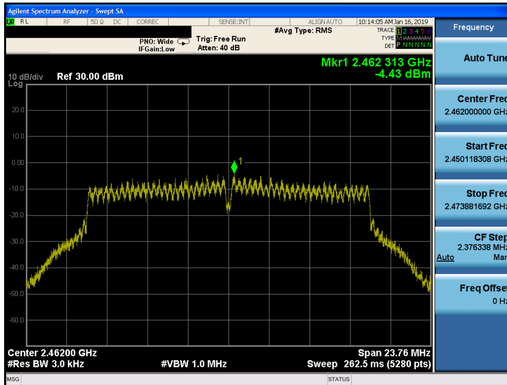
Plot 7-59. Power Spectral Density Plot CDD PRIMARY CORE 0 (802.11g – Ch. 11)
