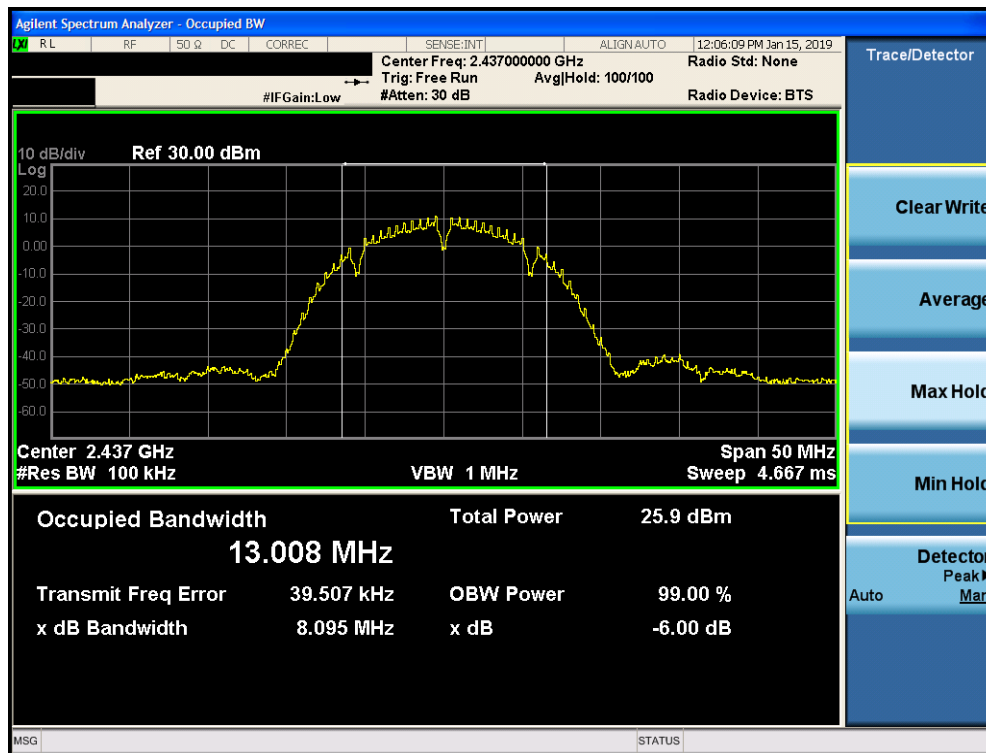
Plot 7-11. 6dB Bandwidth Plot SISO CORE 0 DIVERSITY (802.11b – Ch. 6)
