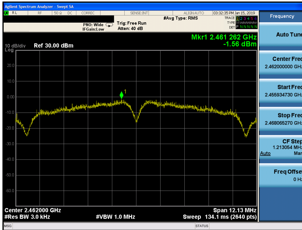
Plot 7-48. Power Spectral Density Plot SISO CORE 1 (802.11b – Ch. 11)
