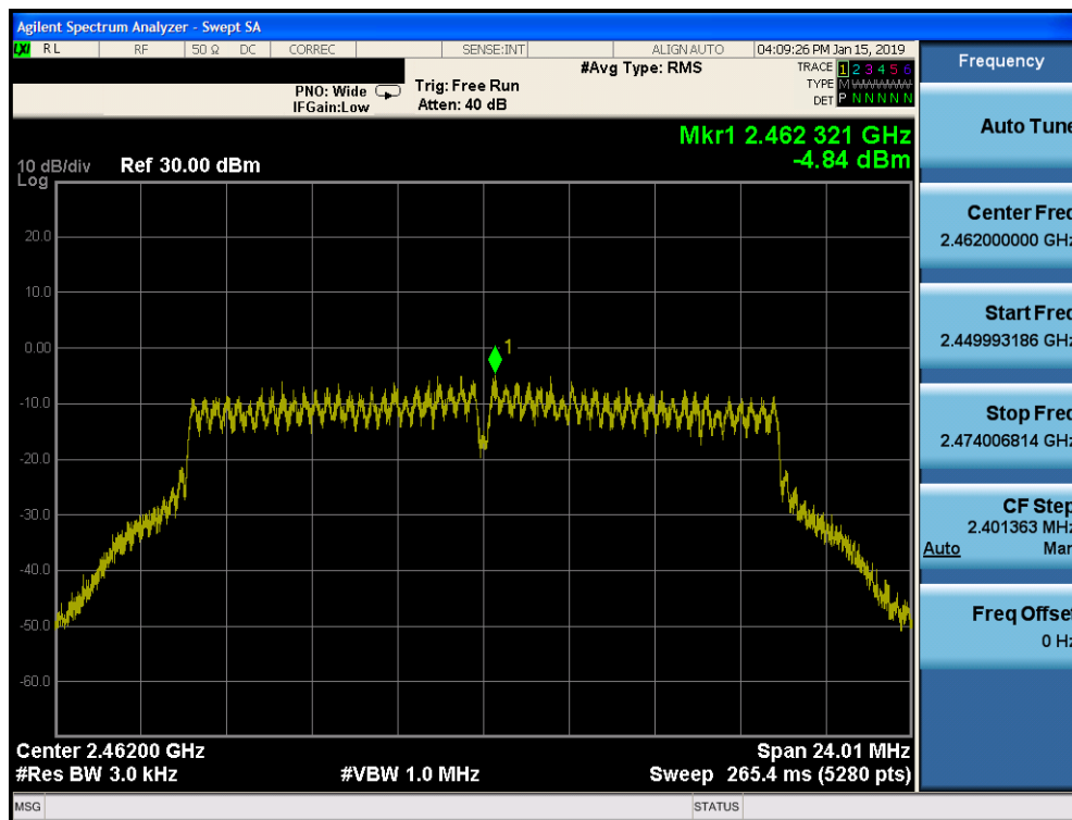
Plot 7-51. Power Spectral Density Plot SISO CORE 1 (802.11g – Ch. 11)
