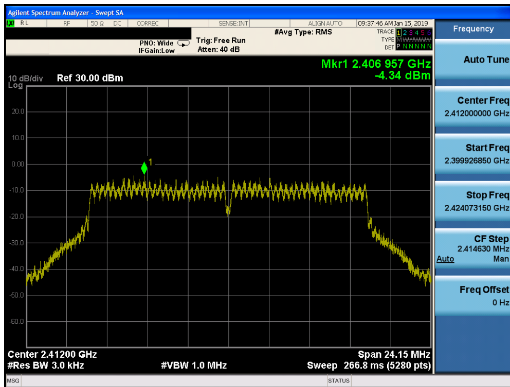
Plot 7-31. Power Spectral Density Plot SISO CORE 0 PRIMARY (802.11g – Ch. 1)
