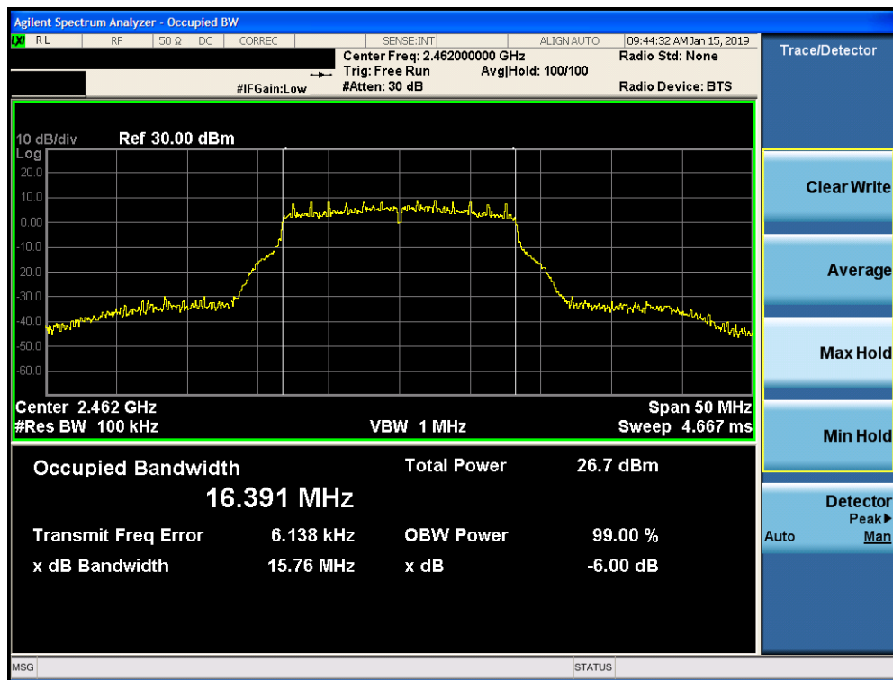
Plot 7-6. 6dB Bandwidth Plot SISO CORE 0 PRIMARY (802.11g – Ch. 11)
