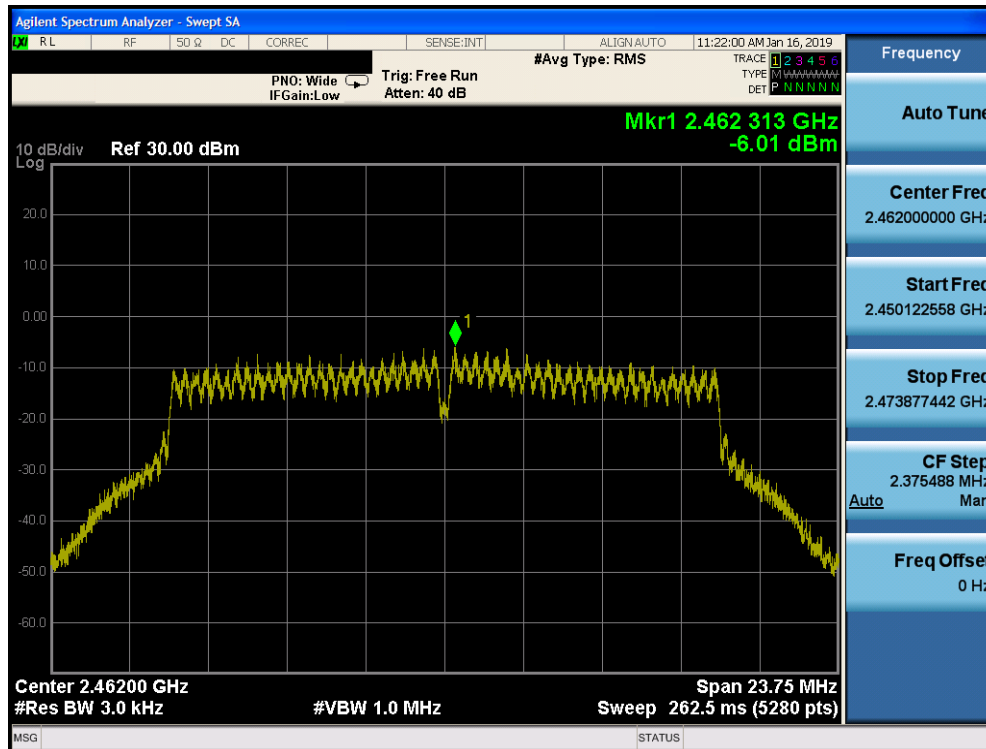
Plot 7-71. Power Spectral Density Plot CDD DIVERSITY CORE 0 (802.11g – Ch. 11)
