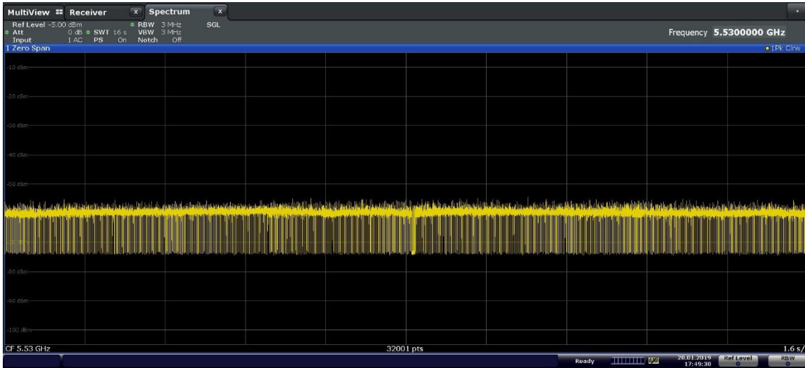
Figure 9-5. 5530MHz - Channel Loading - Mode 1 (80MHz)
