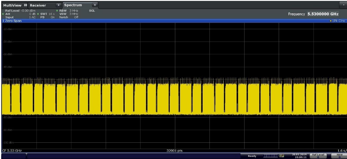
Figure 9-23. 5530MHz - Channel Loading - Mode 4 (80MHz)
