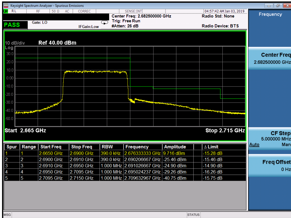
Plot 7-322. Upper ACP Plot (Band 41 - 15.0MHz QPSK - Full RB Configuration)
