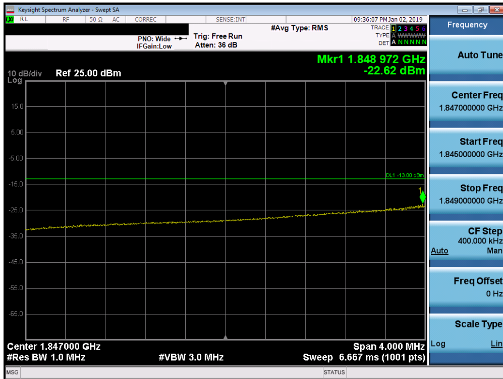
Plot 7-294. Lower Extended Band Edge Plot (Band 25 - 15.0MHz QPSK - Full RB Configuration)
