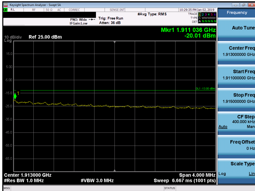
Plot 7-272. Upper Extended Band Edge Plot (Band 2 - 15.0MHz QPSK - Full RB Configuration)
