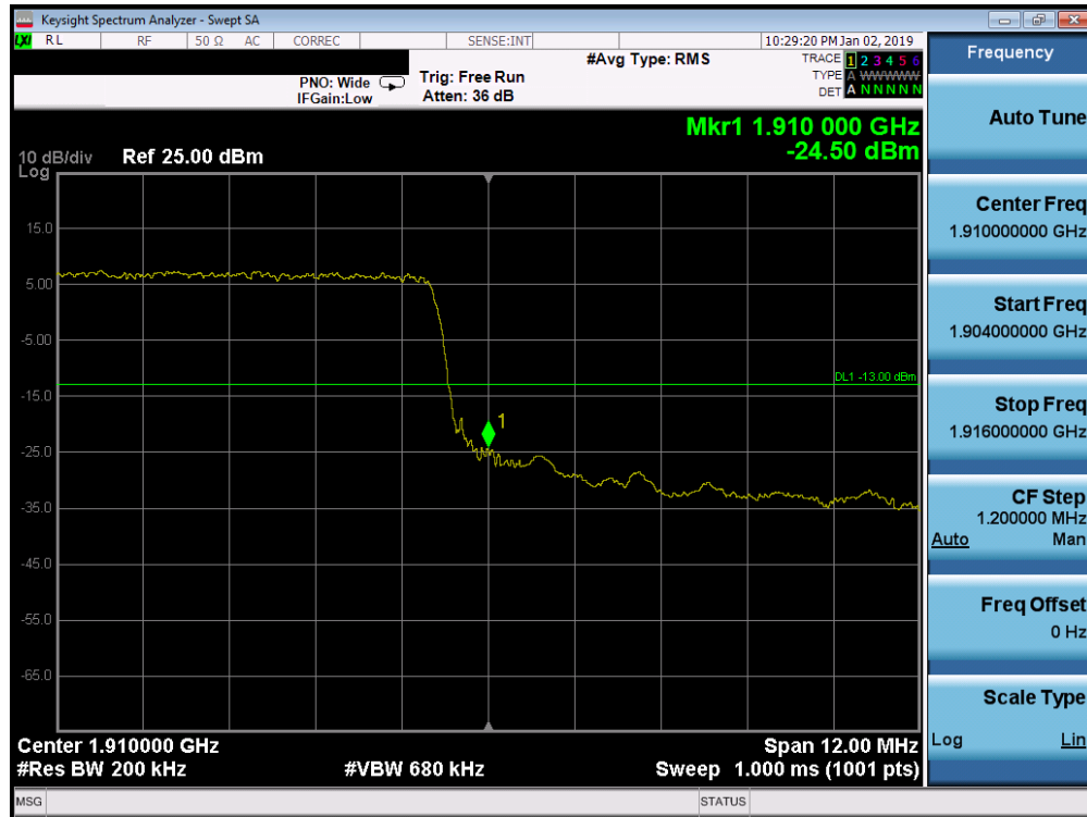
Plot 7-271. Upper Band Edge Plot (Band 2 - 15.0MHz QPSK - Full RB Configuration)
