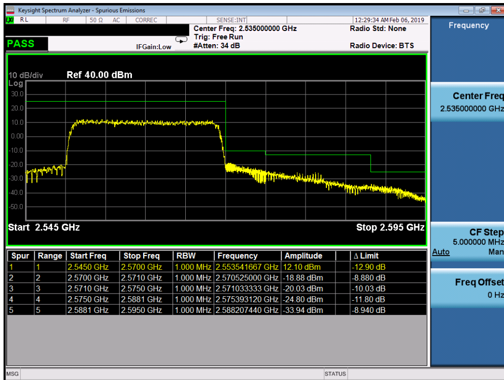
Plot 7-312. Upper ACP Plot (Band 7 - 20.0MHz QPSK - Full RB Configuration)
