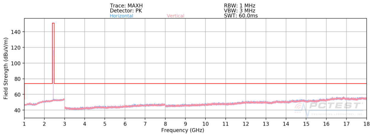
Plot 7-73. Radiated Spurious Plot above 1GHz ANT 1 (BT GFSK ePA – Ch. 39)
