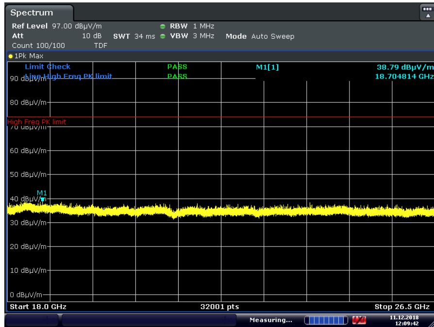
Plot 7-75. Radiated Spurious Plot above 18GHz (GFSK ePA – Ch. 39, Pol. H)
