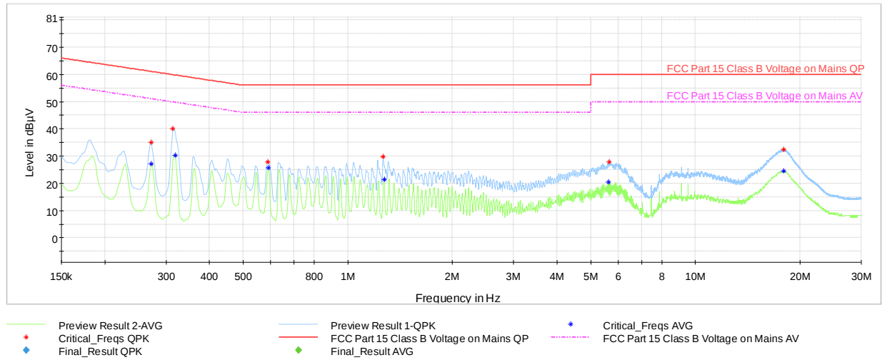
Plot 7-90. AC Line-Conducted Test Plot – GFSK ePA Ch.39 (L1, with Laptop)
