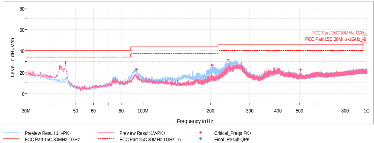
Plot 7-88. Radiated Spurious Plot below 1GHz GFSK ePA – Ch.39, with Laptop
