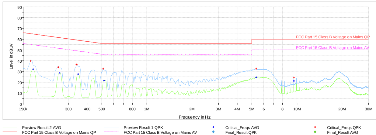
Plot 7-91. AC Line-Conducted Test Plot – GFSK ePA Ch.39 (N, with Laptop)
