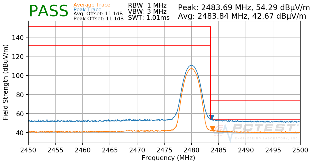
Plot 7-87. Radiated Restricted Upper Band Edge Measurement ANT 1
