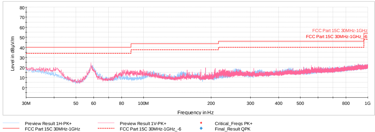
Plot 7-89. Radiated Spurious Plot below 1GHz (2.4GHz – 5GHz), with Laptop
