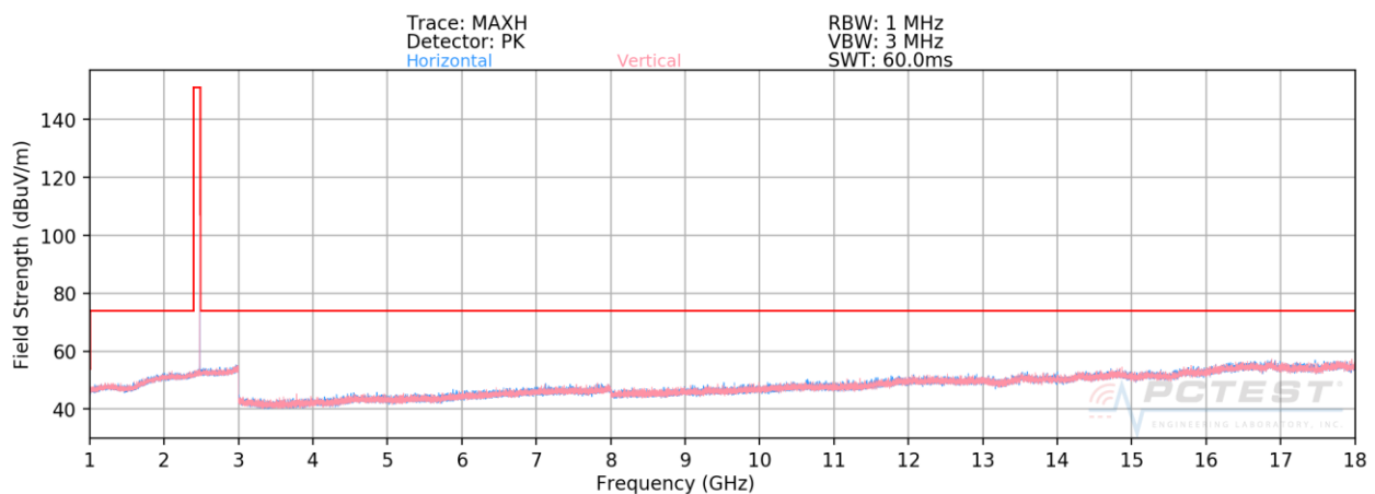
Plot 7-74. Radiated Spurious Plot above 1GHz ANT 1 (BT GFSK ePA – Ch. 78)
