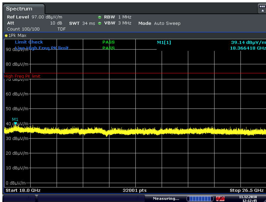
Plot 7-76. Radiated Spurious Plot above 18GHz (GFSK ePA – Ch. 39, Pol. V)
