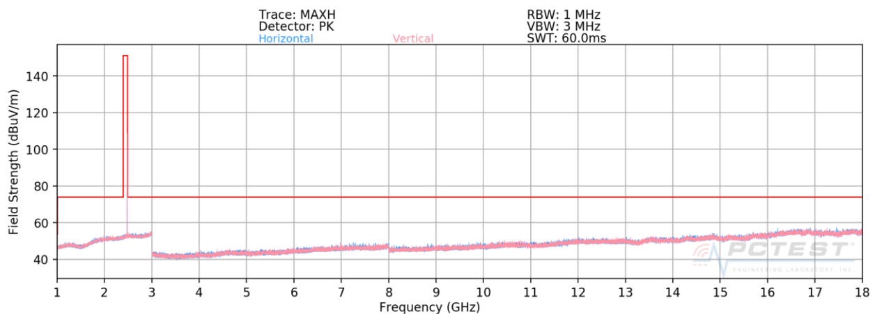
Plot 7-71. Radiated Spurious Plot above 1GHz ANT 0 (BT GFSK ePA – Ch. 78)
