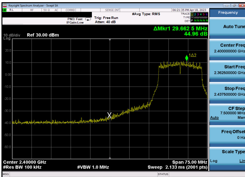
Plot 7-317. Band Edge Plot ANT2 (802.11g- Ch. 4) – 24Mbps
