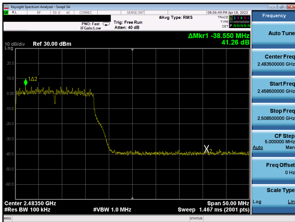
Plot 7-357. Band Edge Plot ANT2 (802.11g – Ch. 12) – 48Mbps
