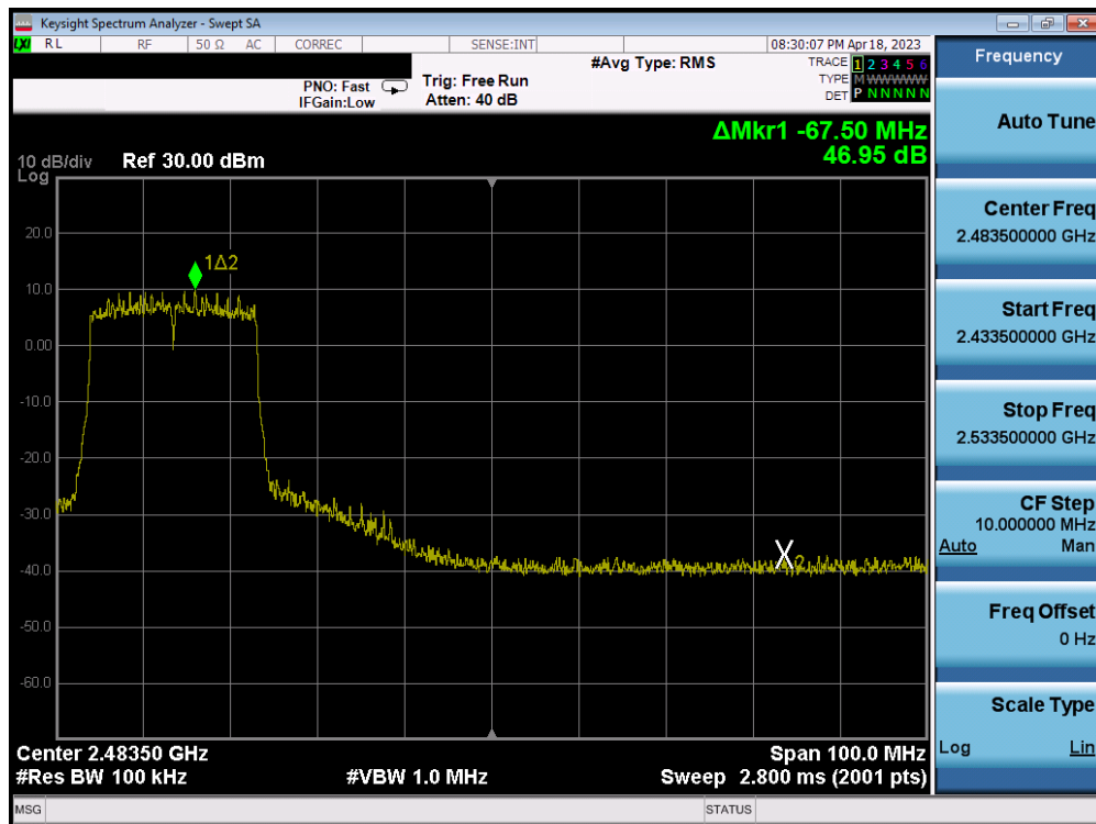
Plot 7-378. Band Edge Plot ANT2 (802.11ax (SU - 2.4GHz) – Ch. 8) – MCS9
