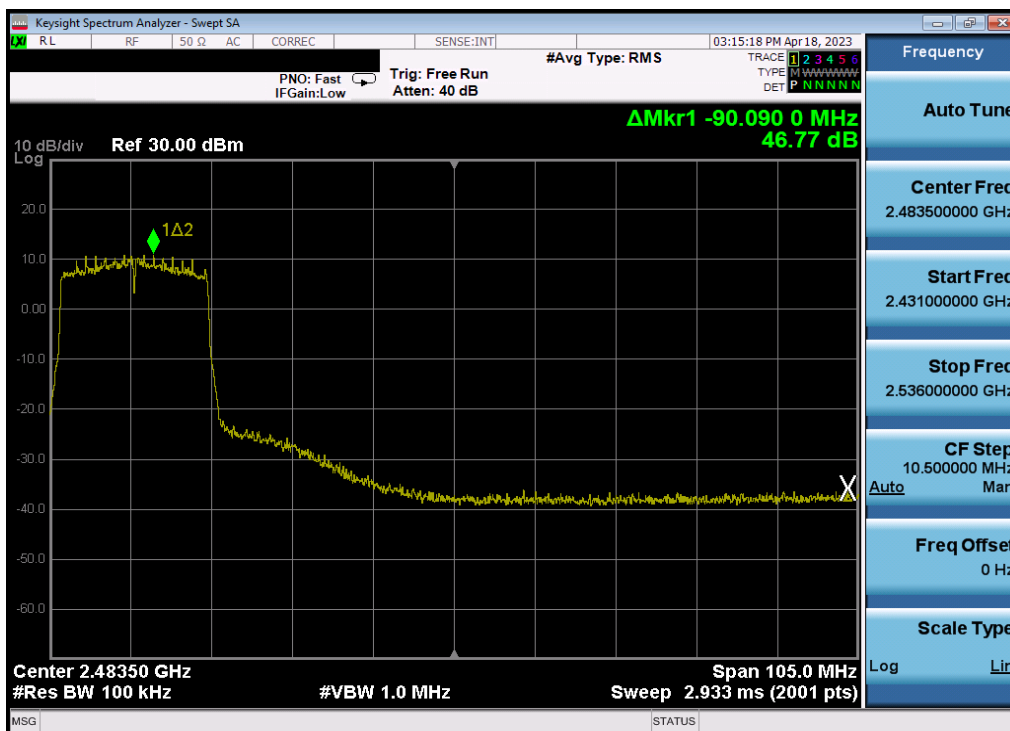
Plot 7-308. Band Edge Plot ANT2 (802.11ax (SU - 2.4GHz) – Ch. 7) – MCS2
