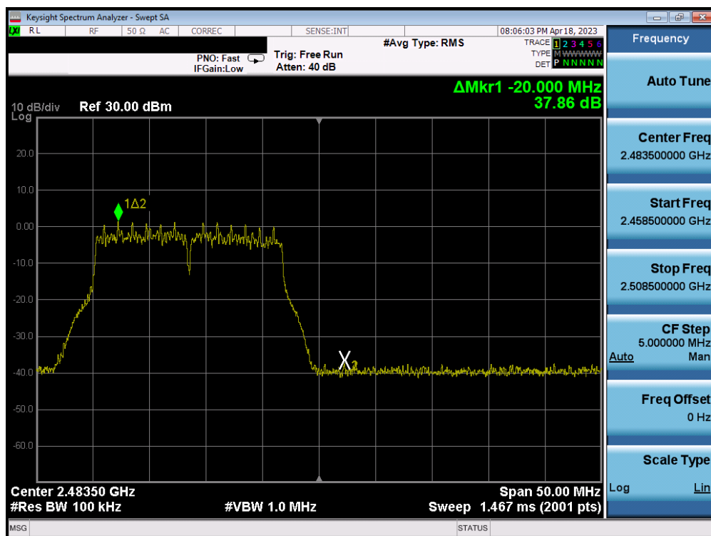
Plot 7-358. Band Edge Plot ANT2 (802.11g – Ch. 13) – 48Mbps
