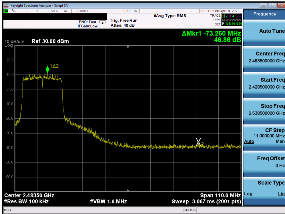
Plot 7-377. Band Edge Plot ANT2 (802.11ax (SU - 2.4GHz) – Ch. 7) – MCS9
