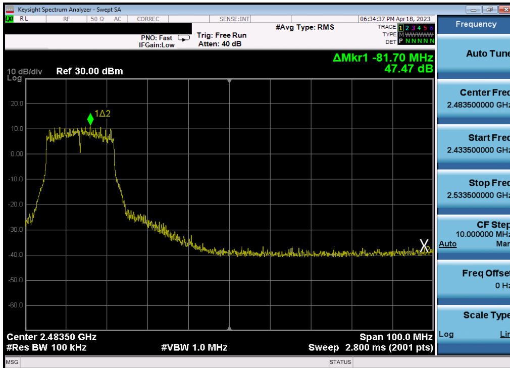
Plot 7-319. Band Edge Plot ANT2 (802.11g – Ch. 8) – 24Mbps
