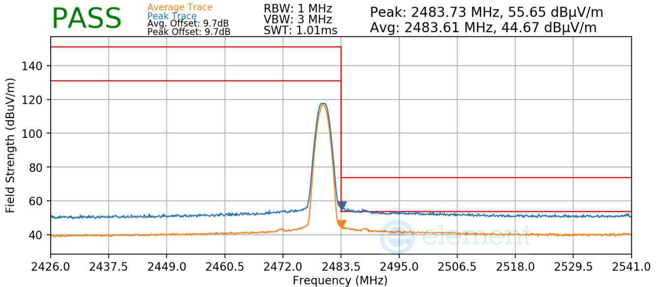
Plot 7-133. Radiated Restricted Upper Band Edge Measurement TxBF (Average & Peak)
