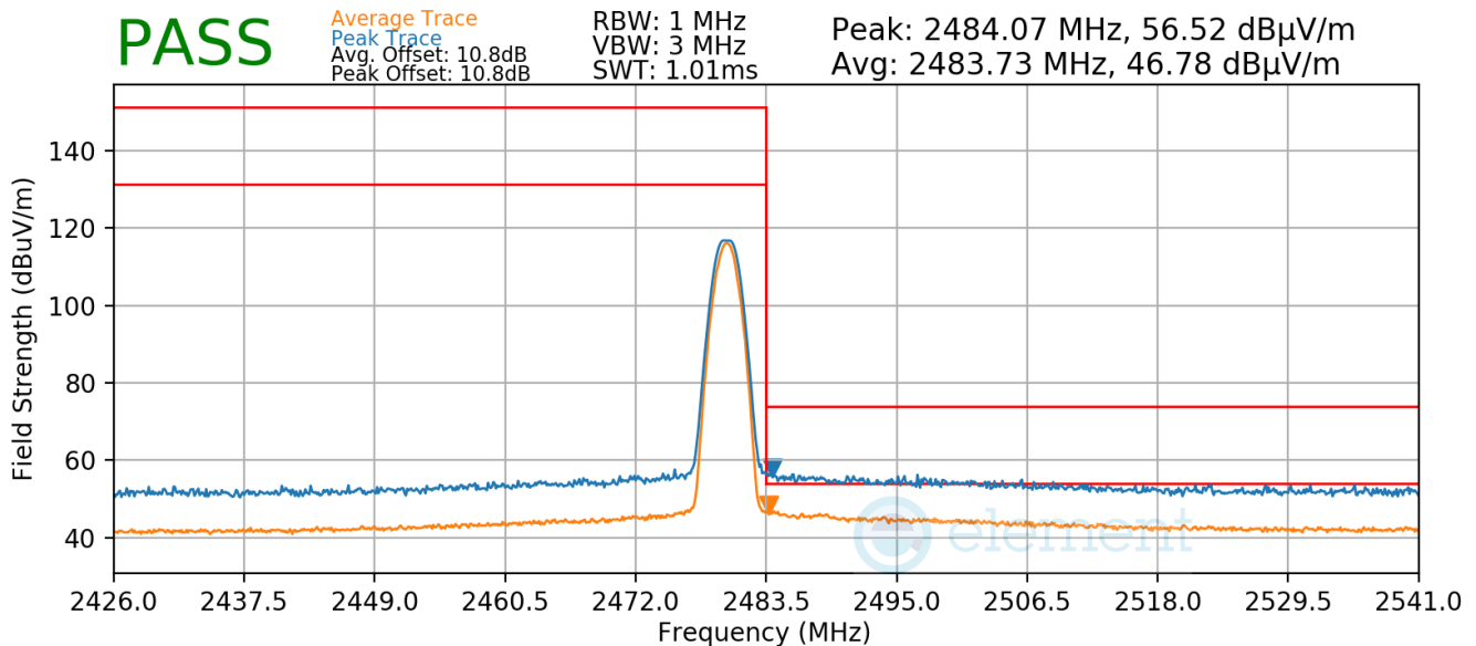
Plot 7-125. Radiated Restricted Upper Band Edge Measurement Ant2 (Average & Peak)
