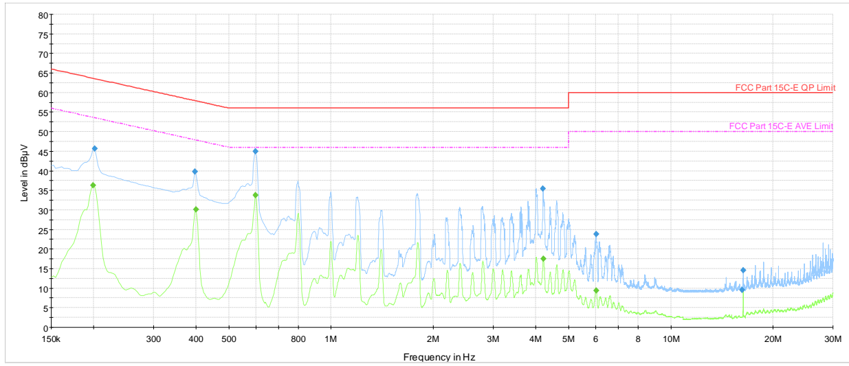
Plot 7-139. AC Line Conducted Plot with Bluetooth LE TxBF (L1, 1Mbps ePA – Ch.0 with AC/DC Adapter)
