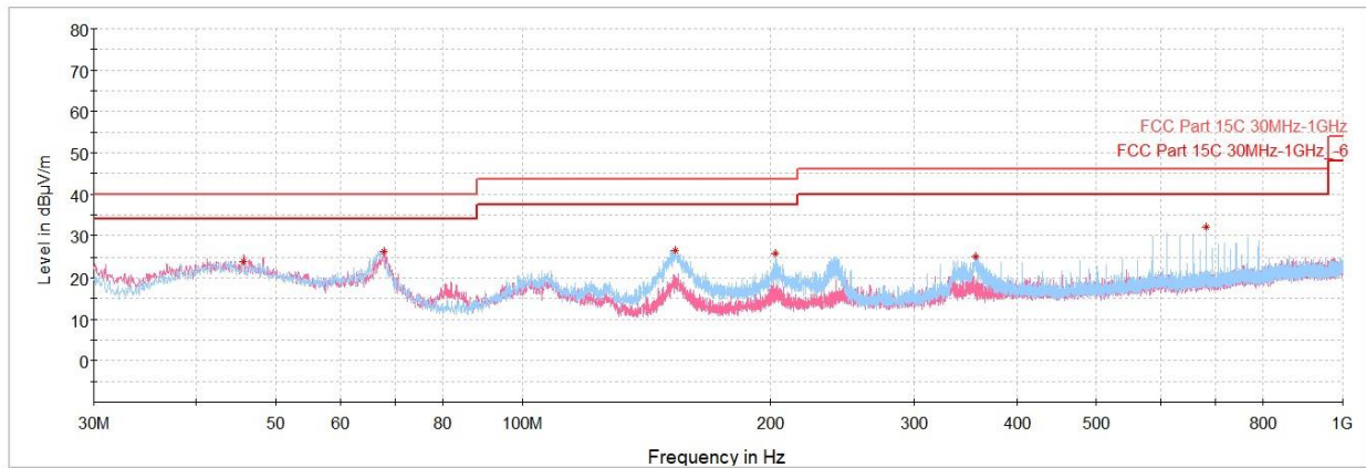
Plot 7-137. Radiated Spurious Emissions Below 1GHz Co-Tx (Pol. H & V with AC/DC Adapter)
