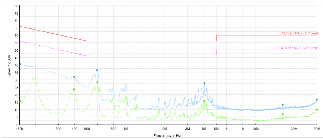
Plot 7-138. AC Line Conducted Plot with Bluetooth LE Tx BF (N, 1Mbps ePA – Ch.0 with AC/DC Adapter)
