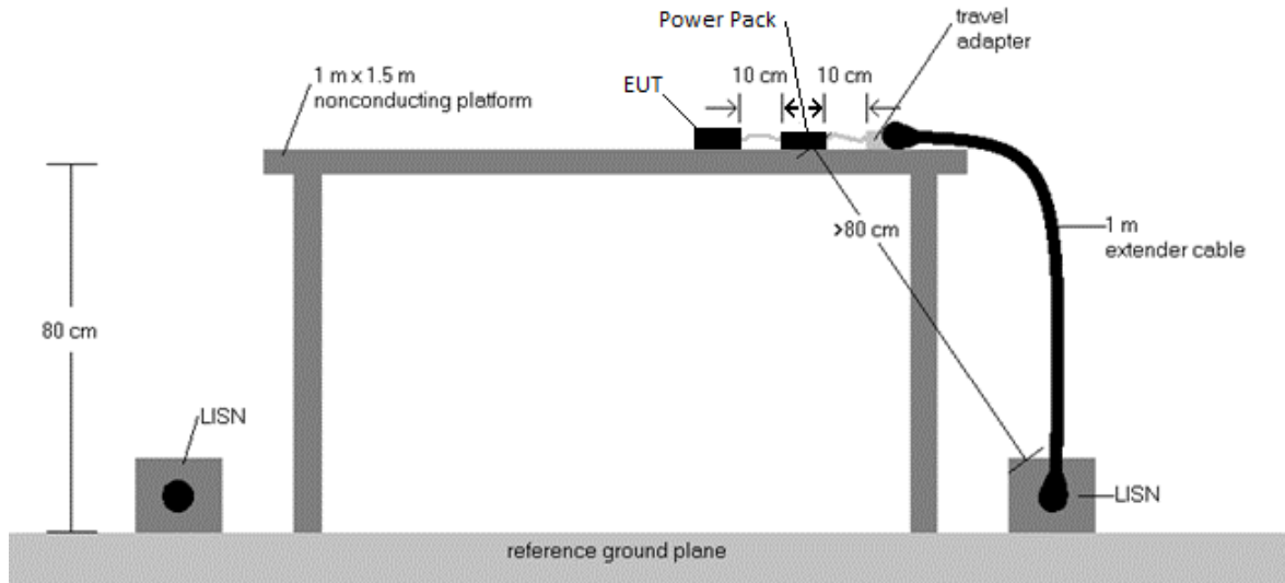
Figure 7-9. Test Instrument & Measurement Setup
