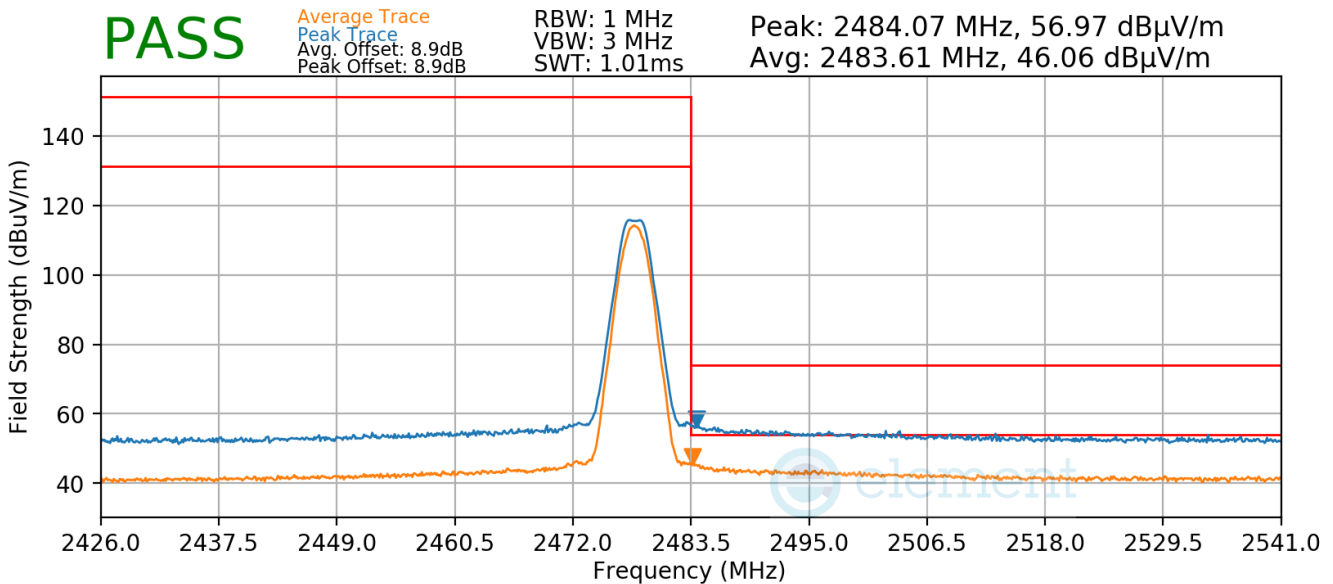
Plot 7-127. Radiated Restricted Upper Band Edge Measurement Ant2 (Average & Peak)
