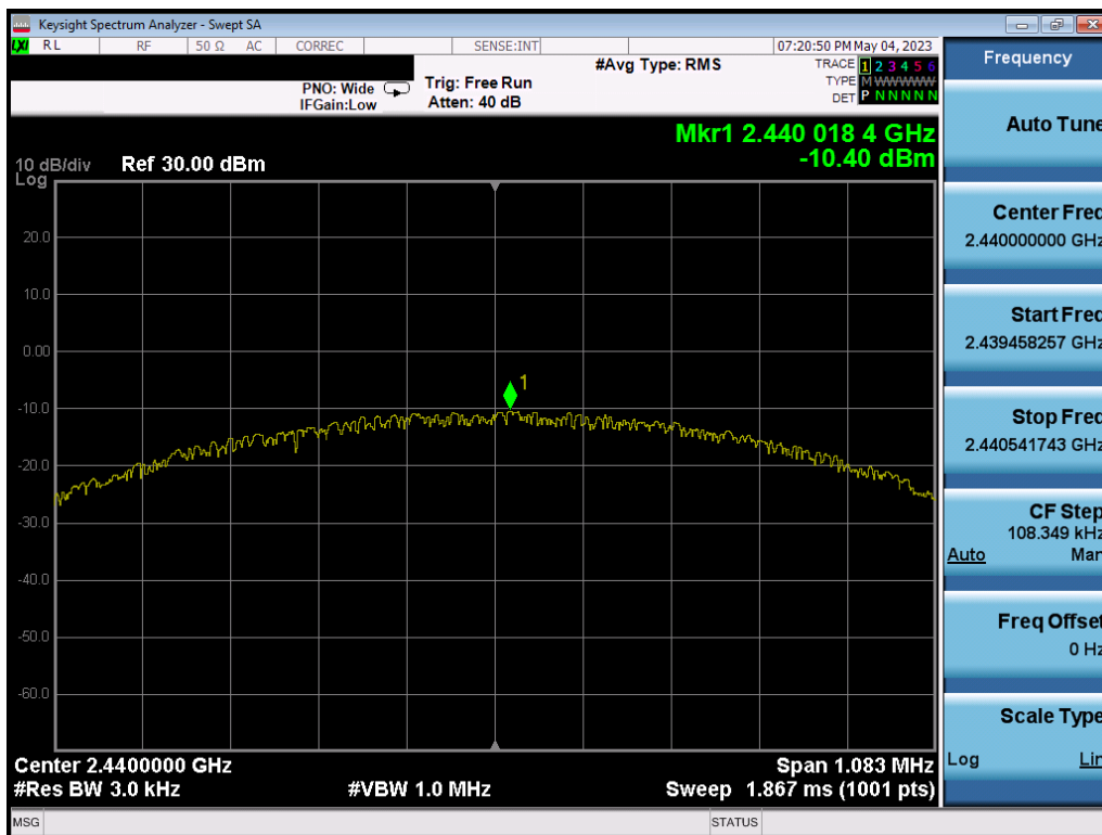
Plot 7-52. Power Spectral Density Plot Ant2 (Bluetooth (LE), 1Mbps, ePA – Ch. 19)
