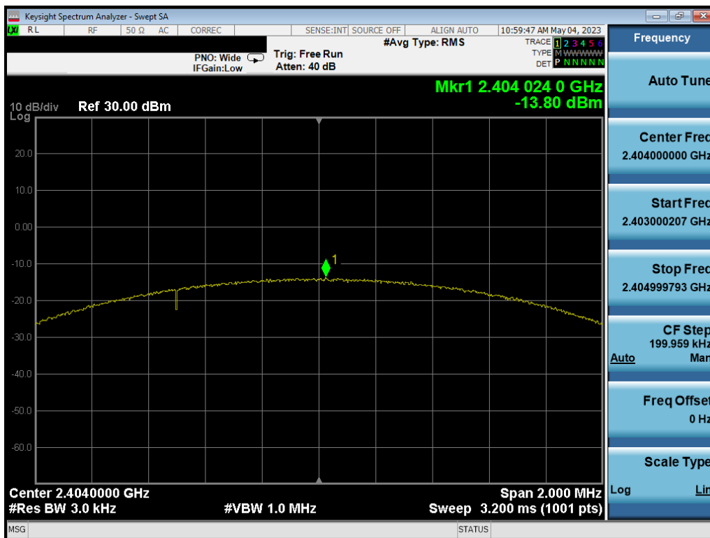
Plot 7-28. Power Spectral Density Plot Ant1 (Bluetooth (LE), 2Mbps, iPA – Ch. 1)
