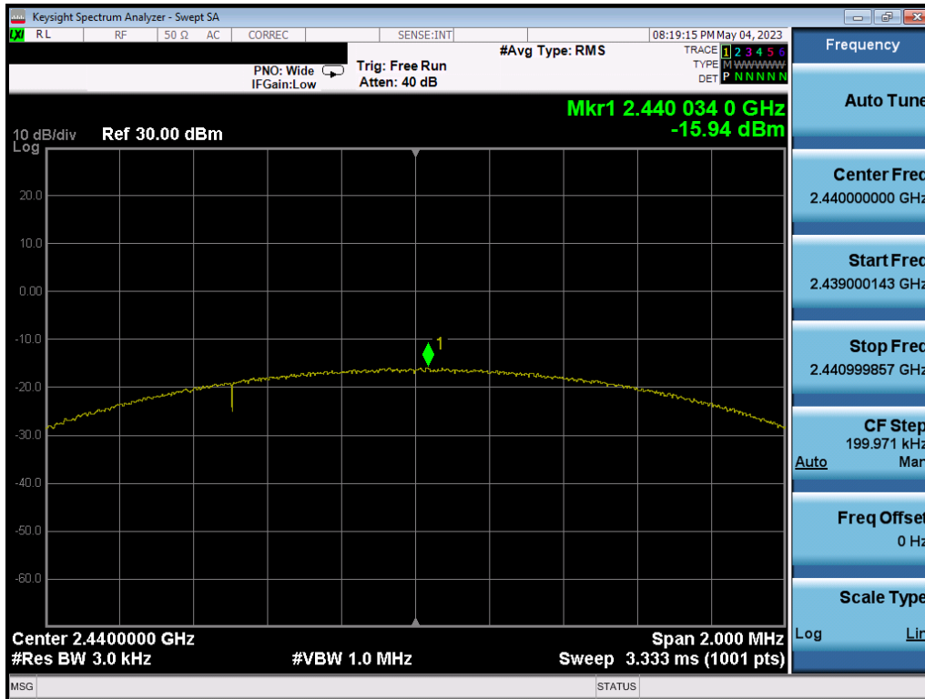
Plot 7-69. Power Spectral Density Plot Ant1 (Bluetooth (LE), 2Mbps, iPA – Ch. 19)
