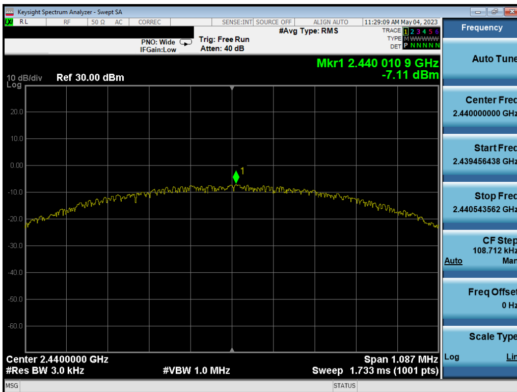
Plot 7-32. Power Spectral Density Plot Ant2 (Bluetooth (LE), 1Mbps, ePA – Ch. 19)
