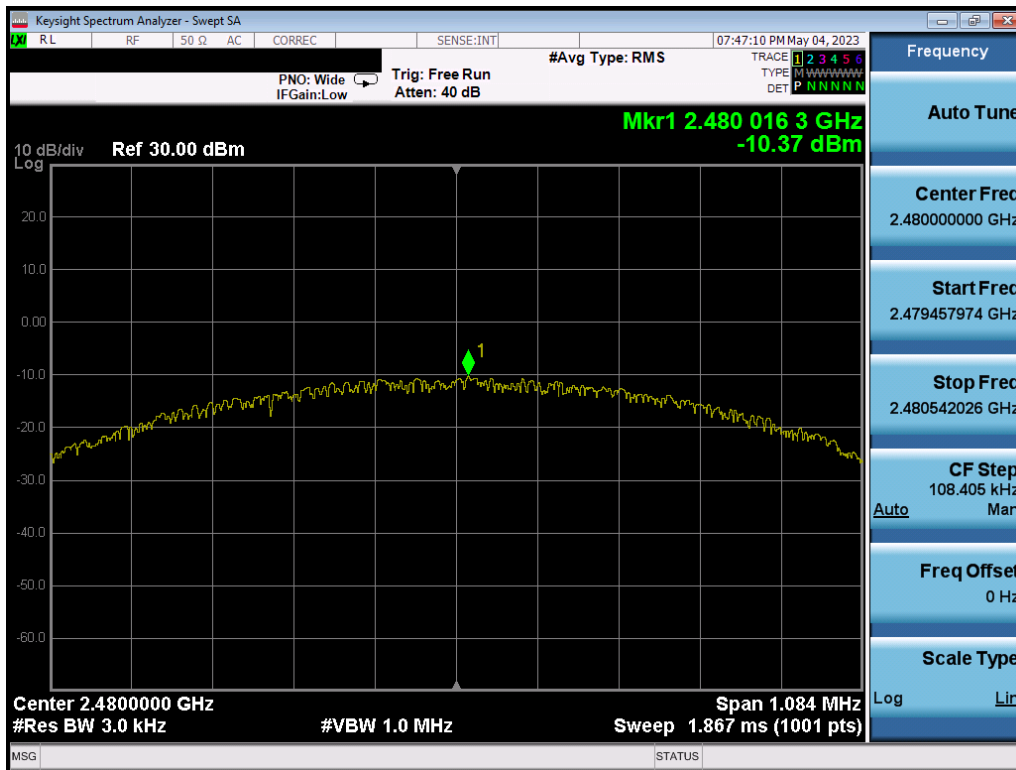
Plot 7-60. Power Spectral Density Plot Ant2 (Bluetooth (LE), 1Mbps, iPA – Ch. 39)
