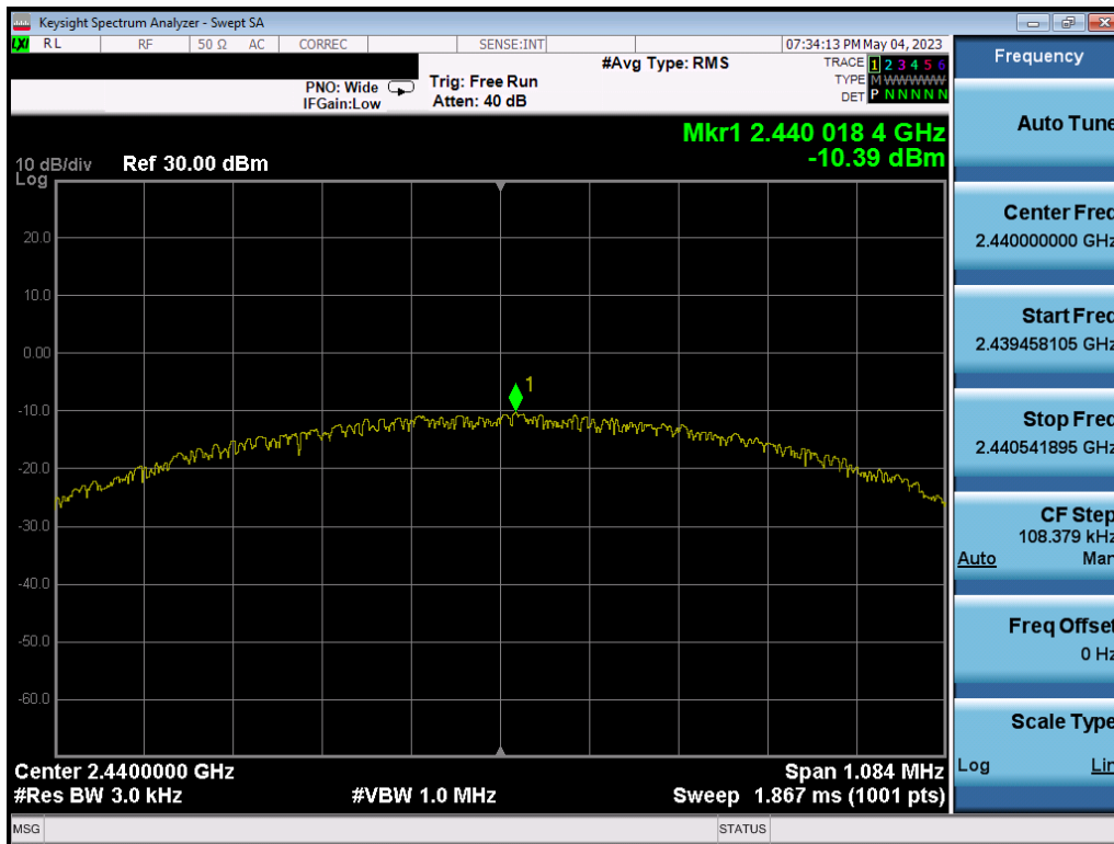
Plot 7-58. Power Spectral Density Plot Ant2 (Bluetooth (LE), 1Mbps, iPA – Ch. 19)
