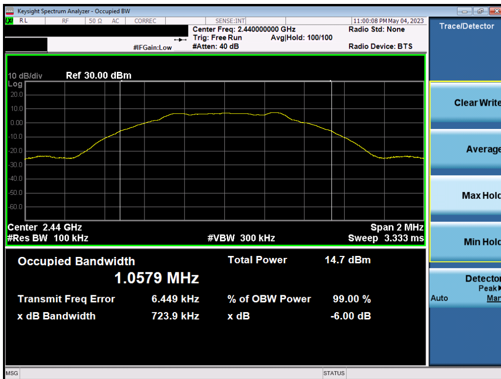
Plot 7-14. 6dB BW & 99% OBW Plot NB UNII_L (Bluetooth (LE), 1Mbps, iPA – Ch. 19)
