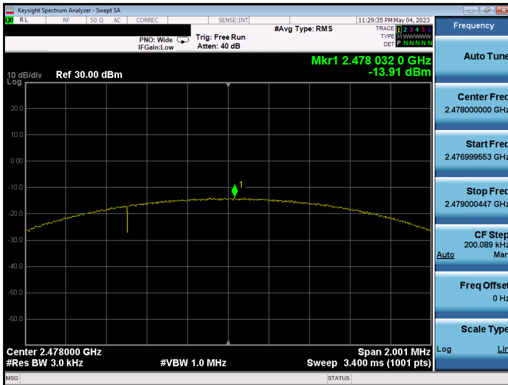
Plot 7-48. Power Spectral Density Plot NB UNII_L (Bluetooth (LE), 2Mbps, iPA – Ch. 38)
