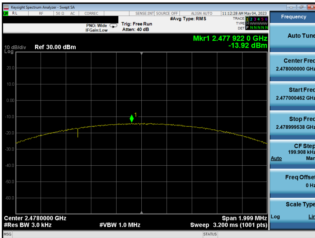
Plot 7-30. Power Spectral Density Plot Ant1 (Bluetooth (LE), 2Mbps, iPA – Ch. 38)
