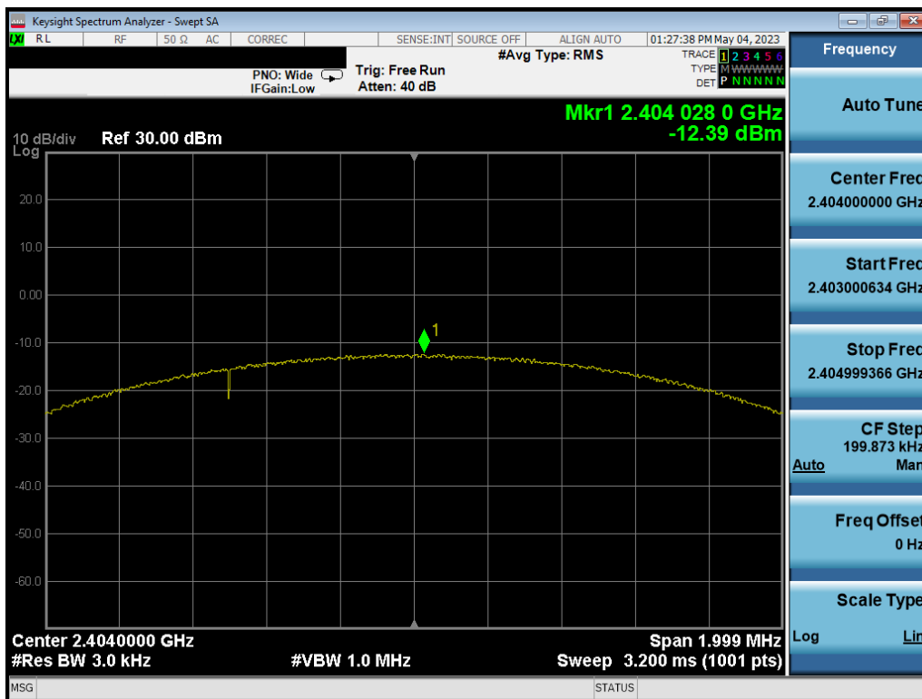
Plot 7-40. Power Spectral Density Plot Ant2 (Bluetooth (LE), 2Mbps, iPA – Ch. 1)
