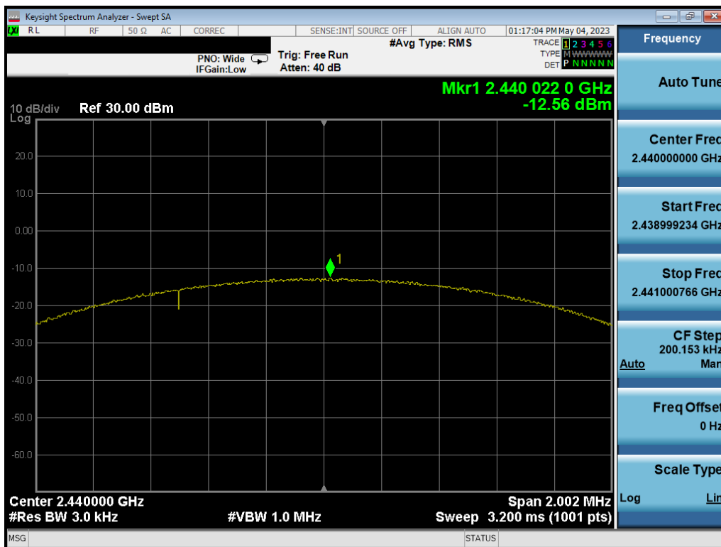
Plot 7-38. Power Spectral Density Plot Ant2 (Bluetooth (LE), 2Mbps, ePA – Ch. 19)
