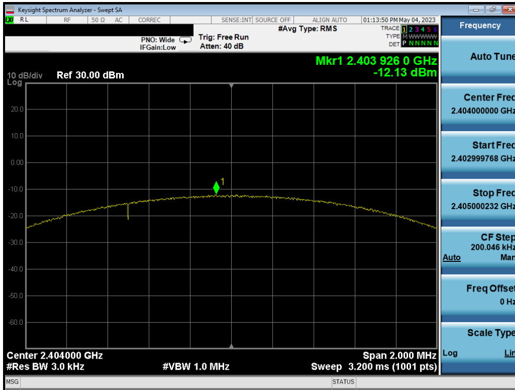
Plot 7-37. Power Spectral Density Plot Ant2 (Bluetooth (LE), 2Mbps, ePA – Ch. 1)
