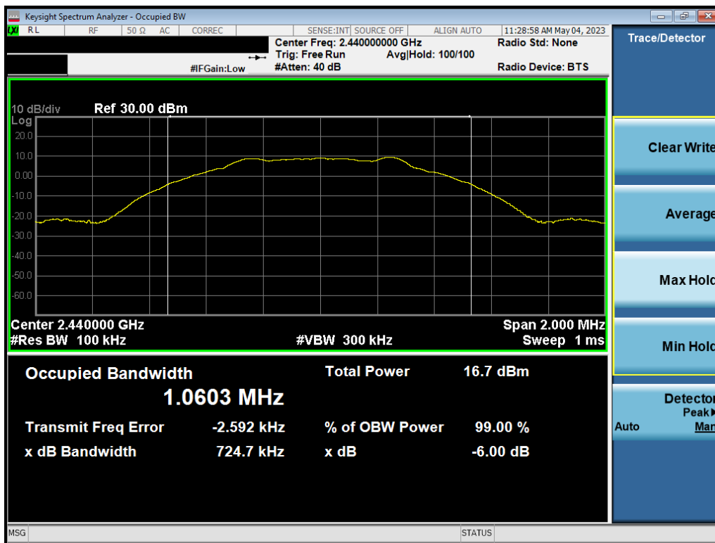
Plot 7-8. 6dB BW & 99% OBW Plot Ant2 (Bluetooth (LE), 1Mbps, ePA – Ch. 19)
