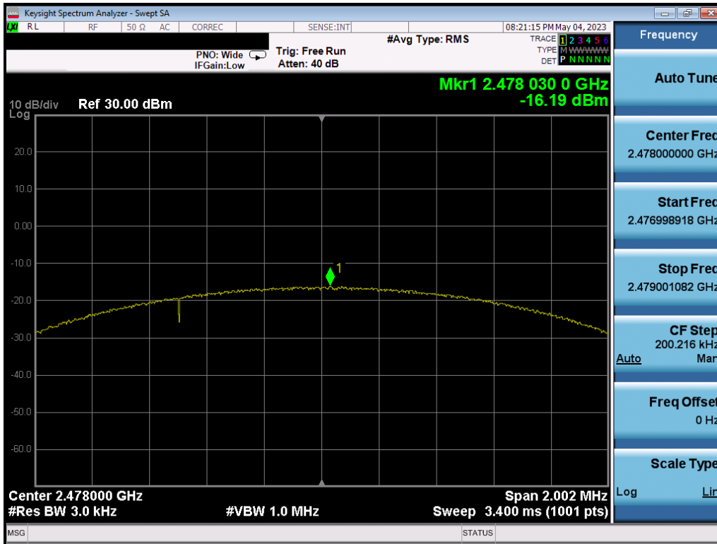
Plot 7-71. Power Spectral Density Plot Ant1 (Bluetooth (LE), 2Mbps, iPA – Ch. 38)
