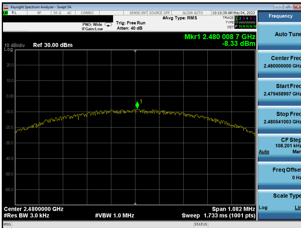
Plot 7-24. Power Spectral Density Plot Ant1 (Bluetooth (LE), 1Mbps, iPA – Ch. 39)
