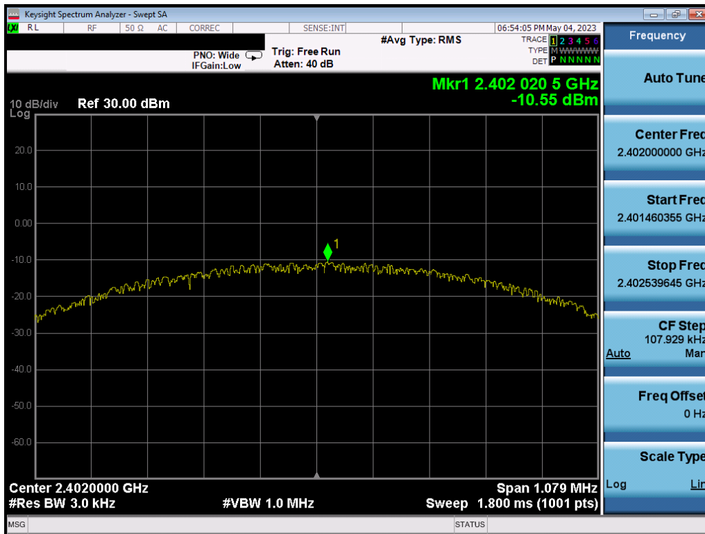
Plot 7-50. Power Spectral Density Plot Ant2 (Bluetooth (LE), 1Mbps, ePA – Ch. 0)
