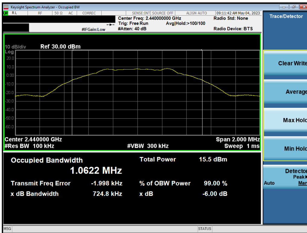
Plot 7-2. 6dB BW & 99% OBW Plot Ant1 (Bluetooth (LE), 1Mbps, ePA – Ch. 19)
