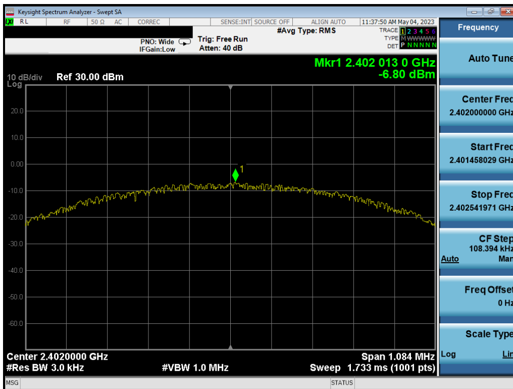
Plot 7-34. Power Spectral Density Plot Ant2 (Bluetooth (LE), 1Mbps, iPA – Ch. 0)
