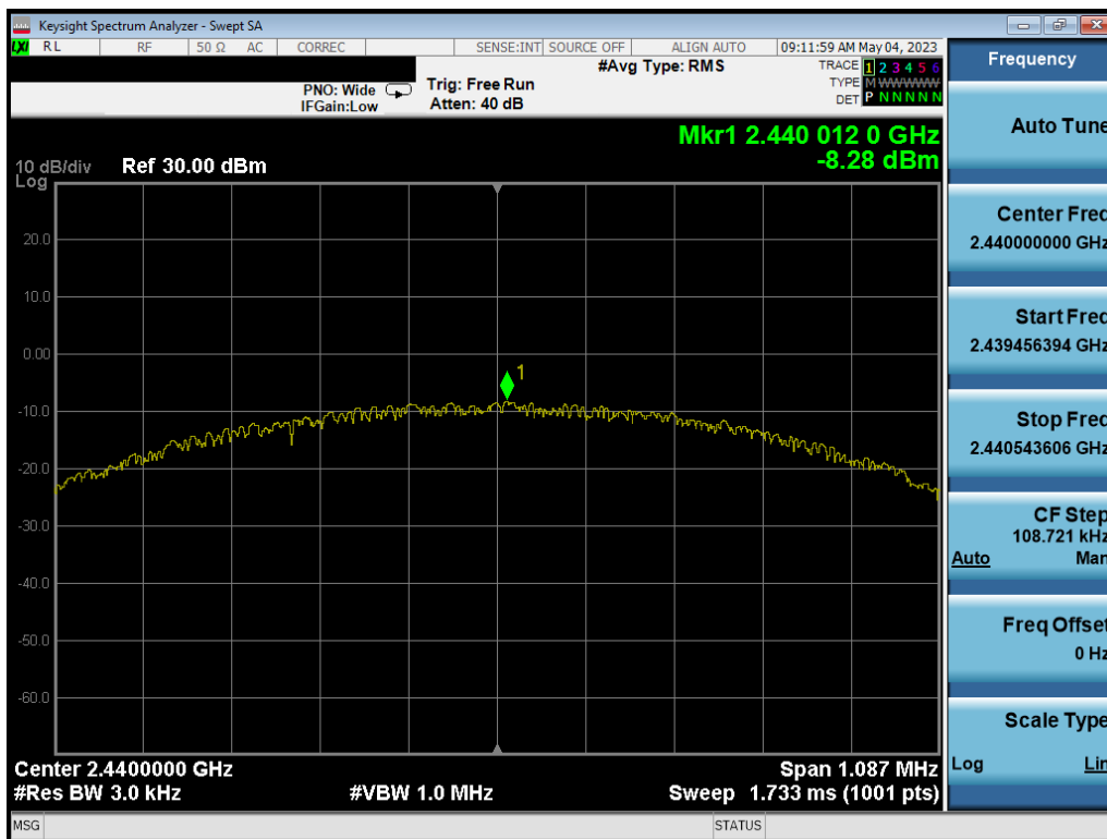
Plot 7-20. Power Spectral Density Plot Ant1 (Bluetooth (LE), 1Mbps, ePA – Ch. 19)
