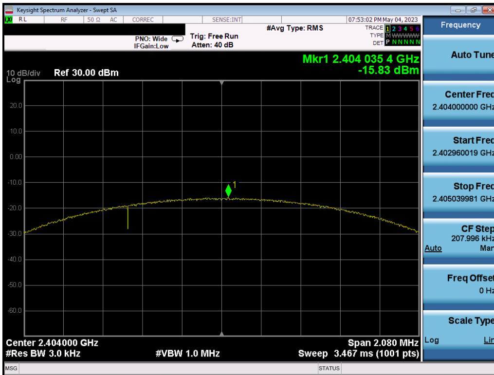
Plot 7-62. Power Spectral Density Plot Ant2 (Bluetooth (LE), 2Mbps, ePA – Ch. 1)
