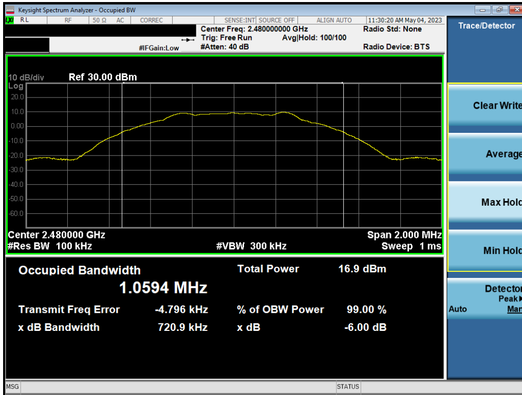
Plot 7-9. 6dB BW & 99% OBW Plot Ant2 (Bluetooth (LE), 1Mbps, ePA – Ch. 39)
