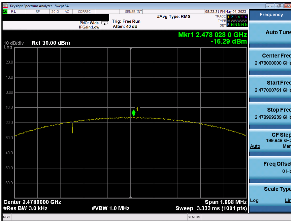
Plot 7-72. Power Spectral Density Plot Ant2 (Bluetooth (LE), 2Mbps, iPA – Ch. 38)
