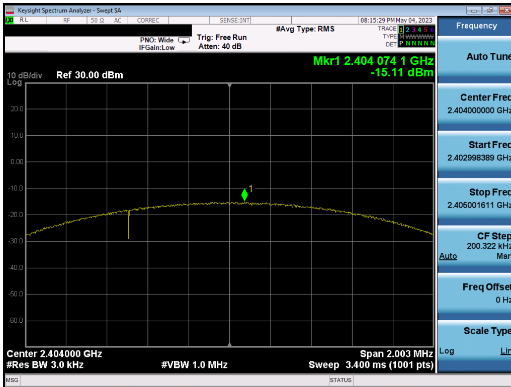
Plot 7-68. Power Spectral Density Plot Ant2 (Bluetooth (LE), 2Mbps, iPA – Ch. 1)
