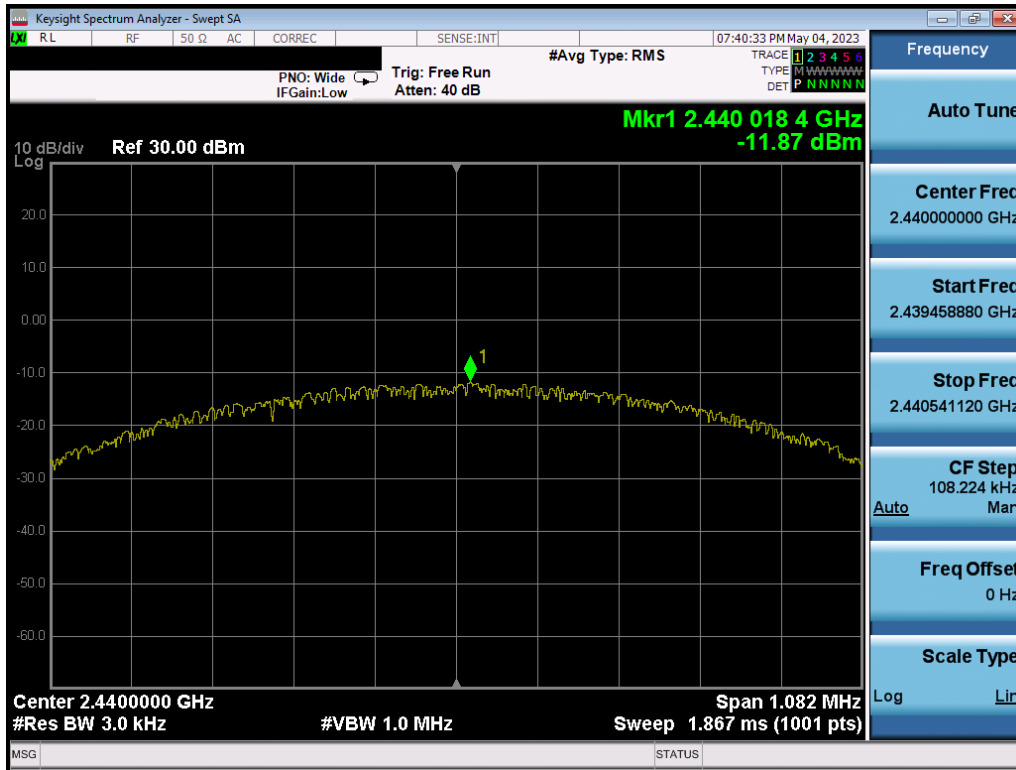
Plot 7-57. Power Spectral Density Plot Ant1 (Bluetooth (LE), 1Mbps, iPA – Ch. 19)
