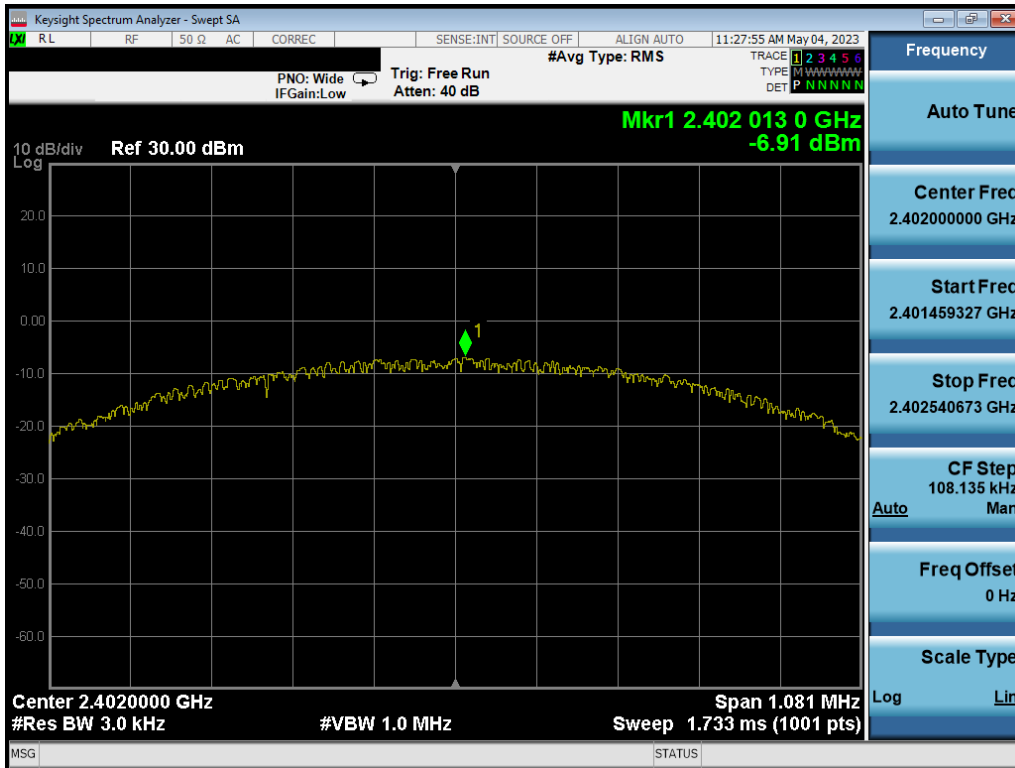
Plot 7-31. Power Spectral Density Plot Ant2 (Bluetooth (LE), 1Mbps, ePA – Ch. 0)
