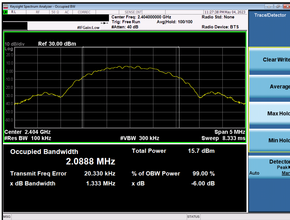
Plot 7-16. 6dB BW & 99% OBW Plot NB UNII_L (Bluetooth (LE), 2Mbps, iPA – Ch. 1)
