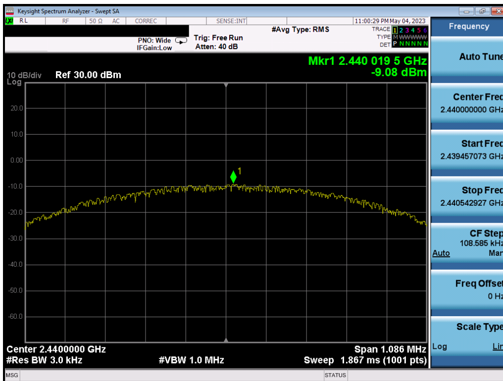
Plot 7-44. Power Spectral Density Plot NB UNII_L (Bluetooth (LE), 1Mbps, iPA – Ch. 19)
