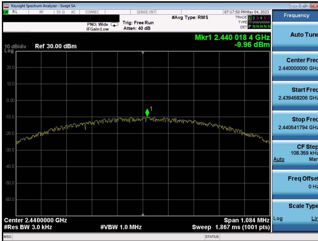
Plot 7-51. Power Spectral Density Plot Ant1 (Bluetooth (LE), 1Mbps, ePA – Ch. 19)
