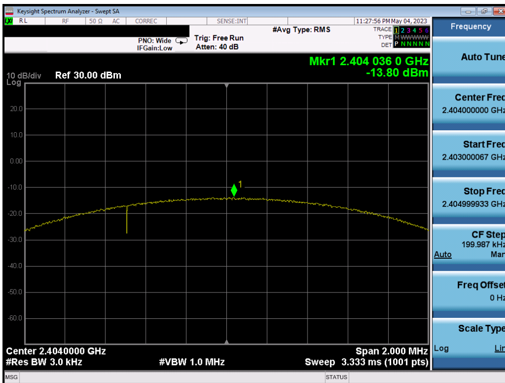
Plot 7-46. Power Spectral Density Plot NB UNII_L (Bluetooth (LE), 2Mbps, iPA – Ch. 1)
