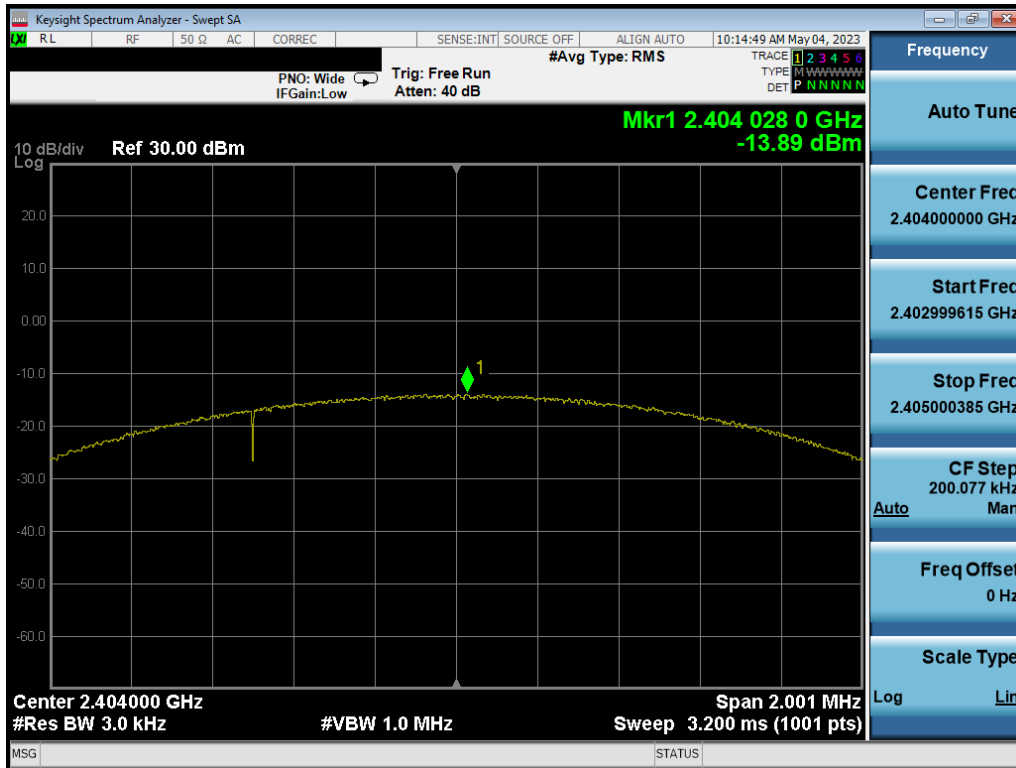
Plot 7-25. Power Spectral Density Plot Ant1 (Bluetooth (LE), 2Mbps, ePA – Ch. 1)
