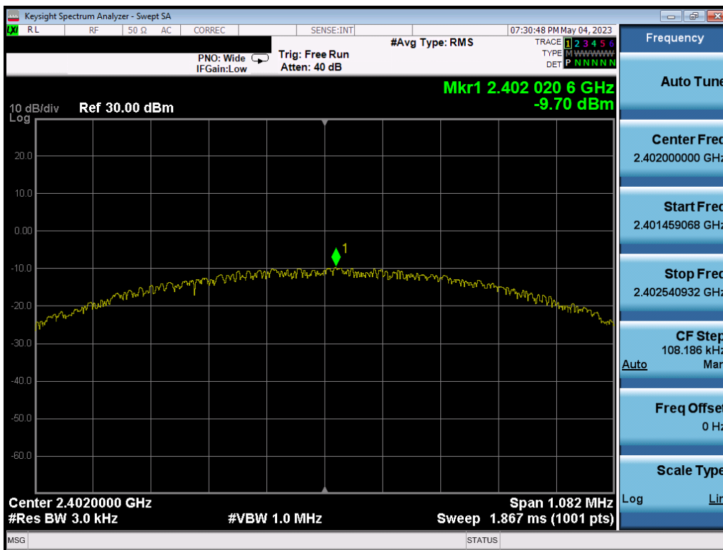
Plot 7-56. Power Spectral Density Plot Ant2 (Bluetooth (LE), 1Mbps, iPA – Ch. 0)
