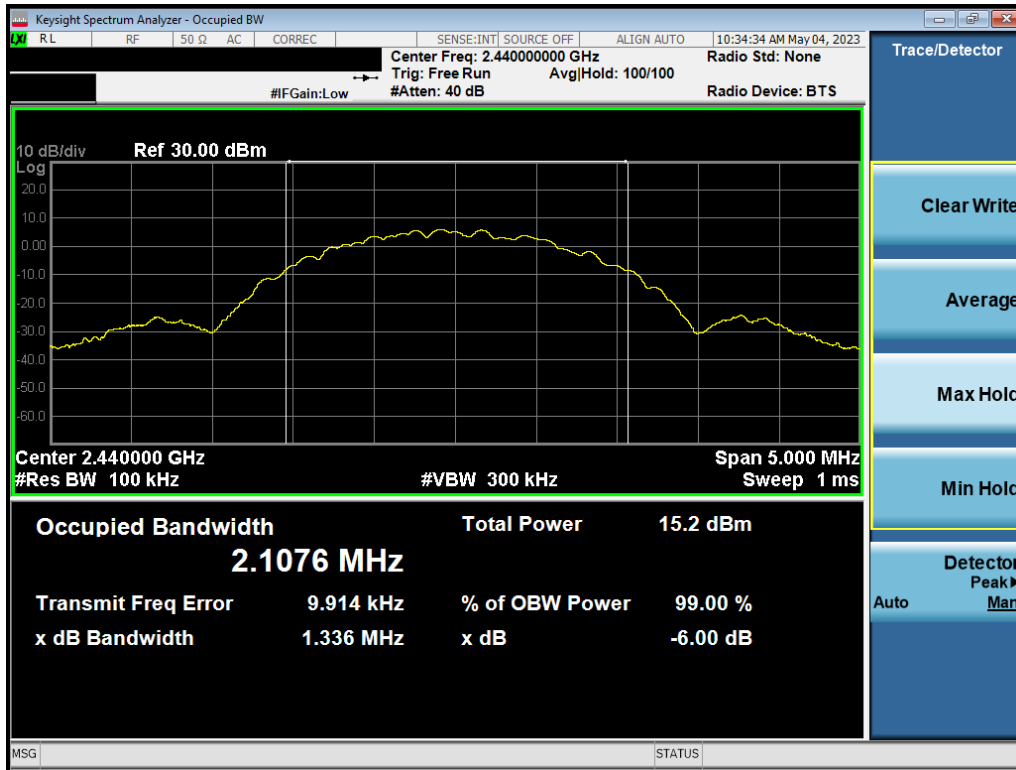
Plot 7-5. 6dB BW & 99% OBW Plot Ant1 (Bluetooth (LE), 2Mbps, ePA – Ch. 19)
