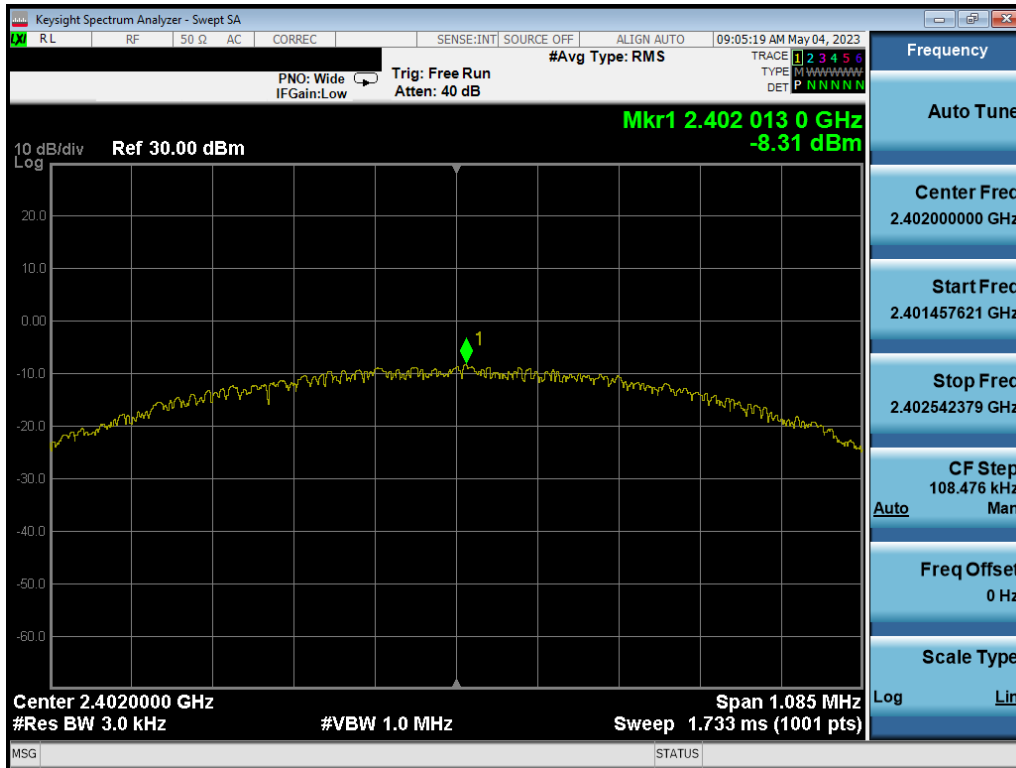
Plot 7-19. Power Spectral Density Plot Ant1 (Bluetooth (LE), 1Mbps, ePA – Ch. 0)
