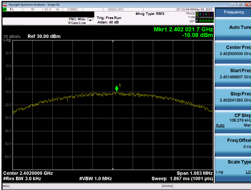
Plot 7-49. Power Spectral Density Plot Ant1 (Bluetooth (LE), 1Mbps, ePA – Ch. 0)
