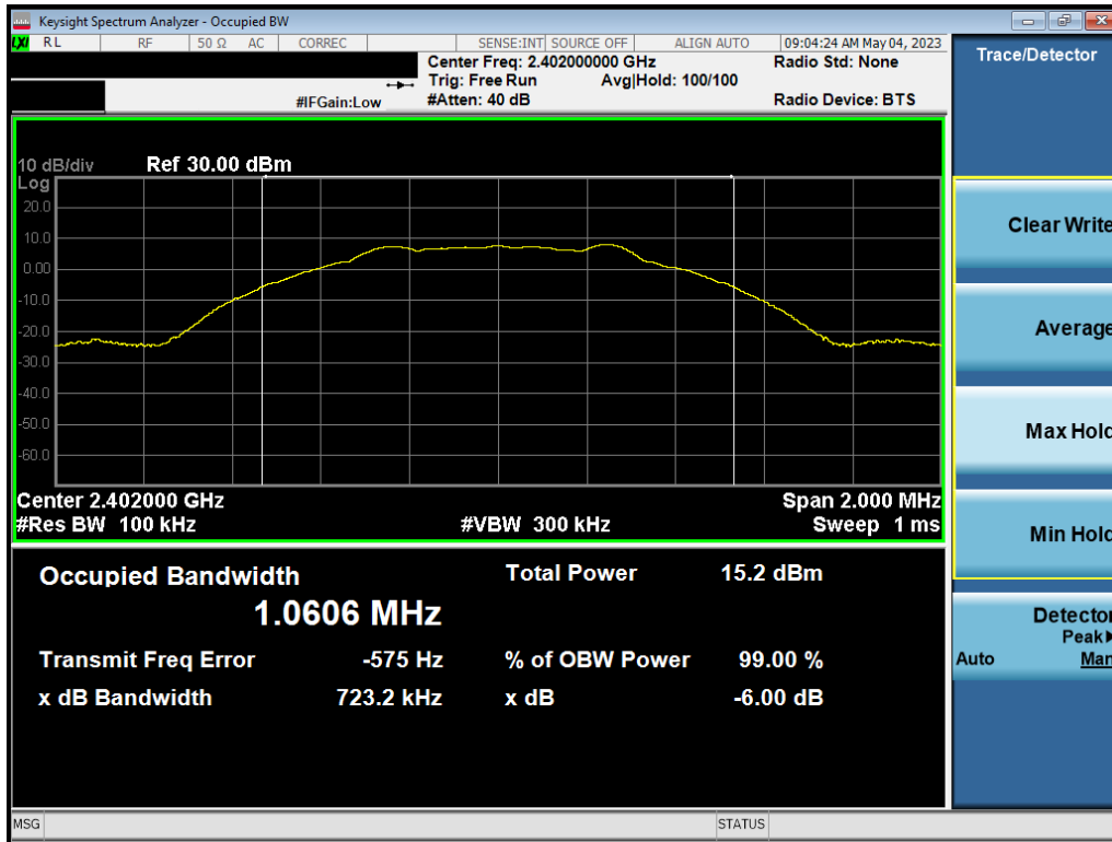
Plot 7-1. 6dB BW & 99% OBW Plot Ant1 (Bluetooth (LE), 1Mbps, ePA – Ch. 0)
