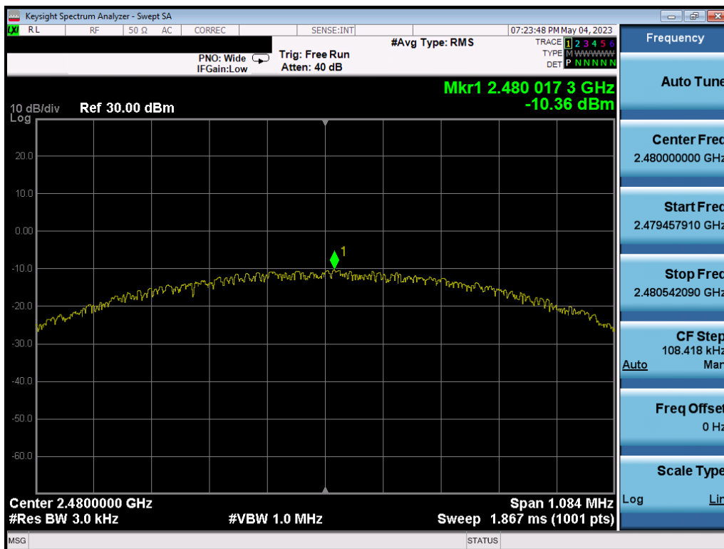
Plot 7-54. Power Spectral Density Plot Ant2 (Bluetooth (LE), 1Mbps, ePA – Ch. 39)
