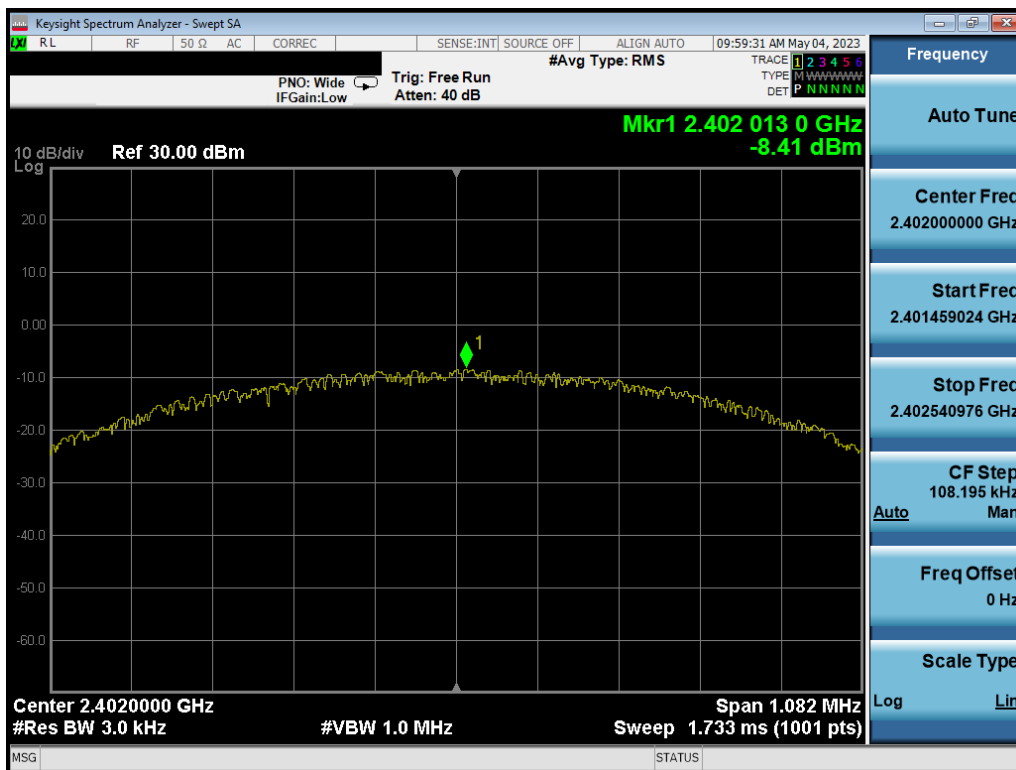
Plot 7-22. Power Spectral Density Plot Ant1 (Bluetooth (LE), 1Mbps, iPA – Ch. 0)
