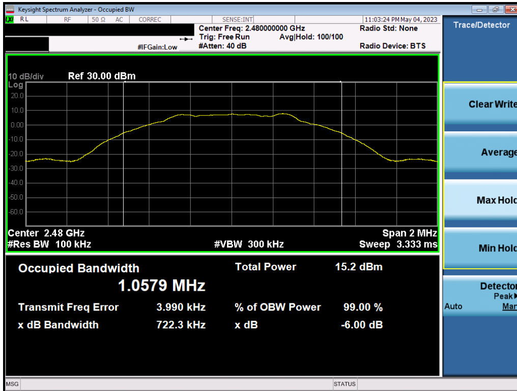
Plot 7-15. 6dB BW & 99% OBW Plot NB UNII_L (Bluetooth (LE), 1Mbps, iPA – Ch. 39)
