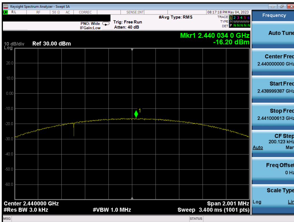
Plot 7-70. Power Spectral Density Plot Ant2 (Bluetooth (LE), 2Mbps, iPA – Ch. 19)
