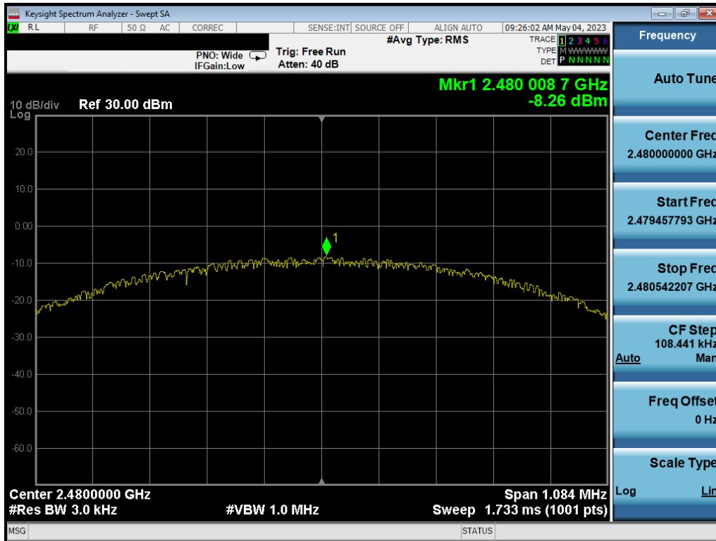
Plot 7-21. Power Spectral Density Plot Ant1 (Bluetooth (LE), 1Mbps, ePA – Ch. 39)
