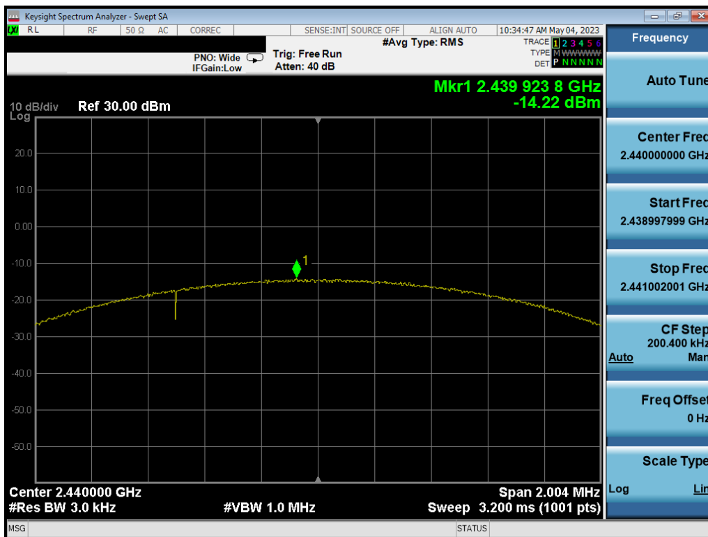
Plot 7-26. Power Spectral Density Plot Ant1 (Bluetooth (LE), 2Mbps, ePA – Ch. 19)
