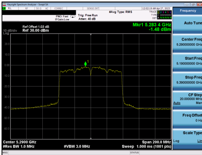
Plot 7-381. PSD CDD Ant1 (80MHz BW 802.11ac – Ch. 58, MCS4)
