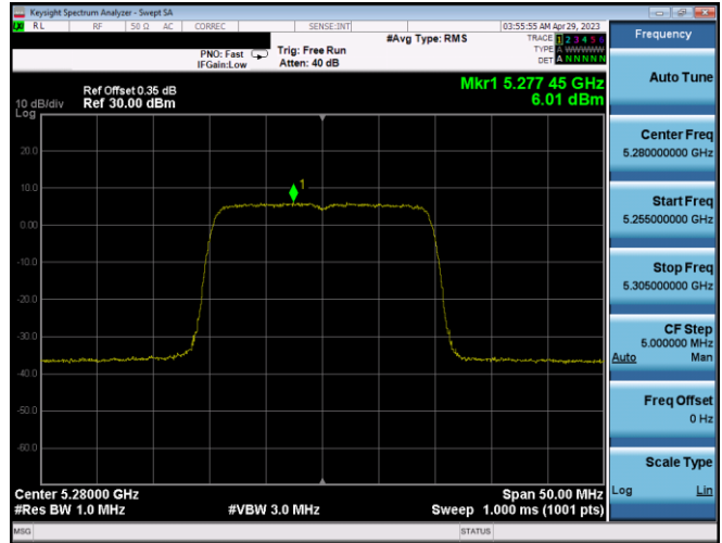
Plot 7-376. PSD CDD Ant2 (20MHz BW 802.11ax(SU) – Ch. 56, MCS4)
