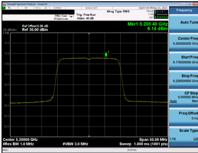
Plot 7-363. PSD CDD Ant1 (20MHz BW 802.11ax(SU) – Ch. 40, MCS4)
