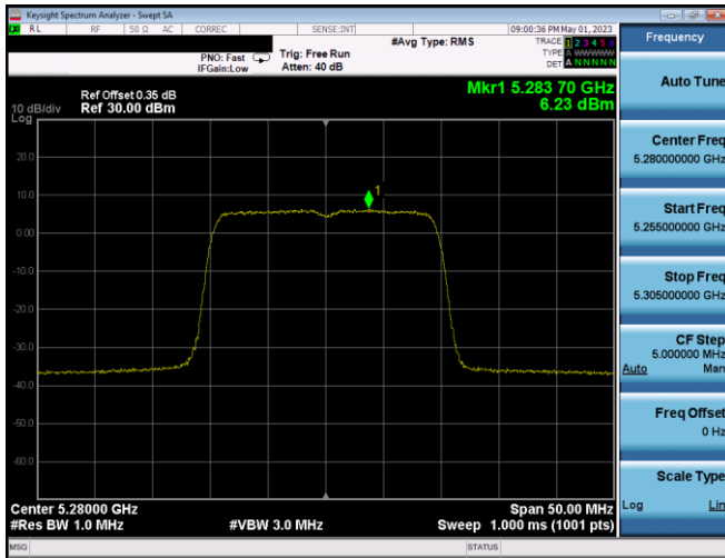
Plot 7-375. PSD CDD Ant1 (20MHz BW 802.11ax(SU) – Ch. 56, MCS4)
