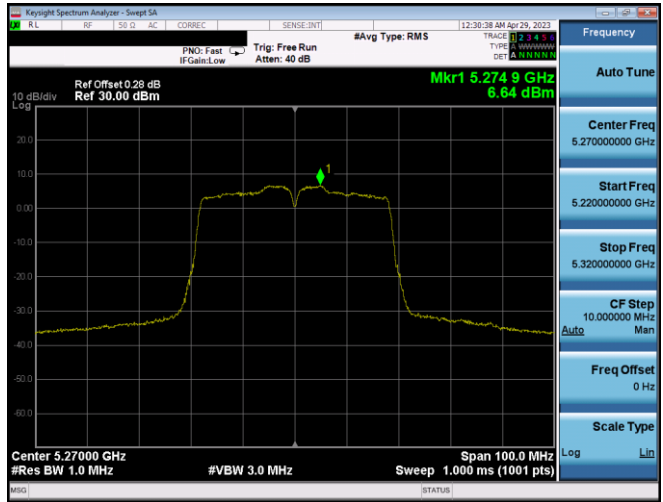
Plot 7-342. PSD CDD Ant2 (40MHz BW 802.11n – Ch. 54, MCS10)
