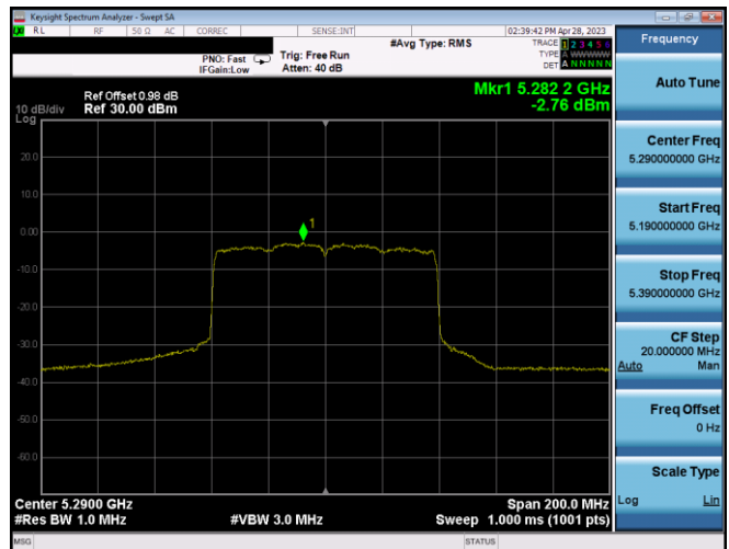
Plot 7-347. PSD CDD Ant1 (80MHz BW 802.11ax(SU) – Ch. 58, MCS2)
