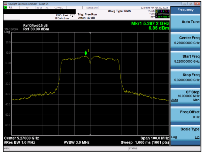
Plot 7-378. PSD CDD Ant2 (40MHz BW 802.11n – Ch. 54, MCS12)
