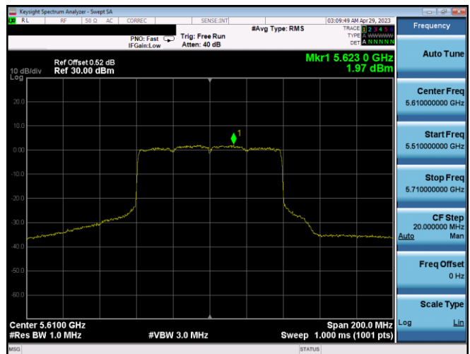
Plot 7-360. PSD CDD Ant2 (80MHz BW 802.11ax(SU) – Ch. 122, MCS2)
