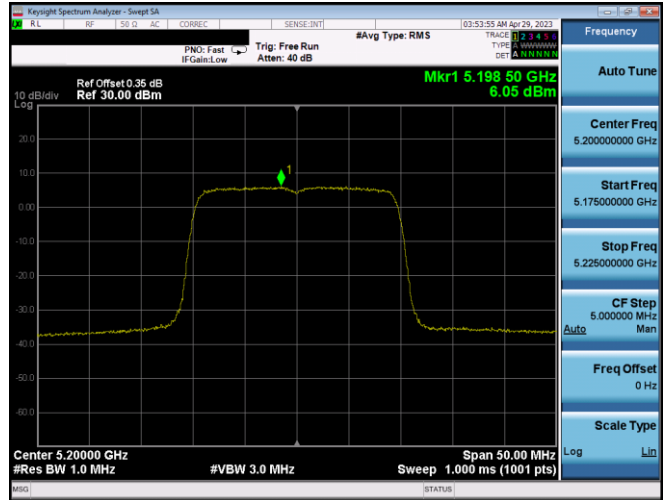
Plot 7-364. PSD CDD Ant2 (20MHz BW 802.11ax(SU) – Ch. 40, MCS4)
