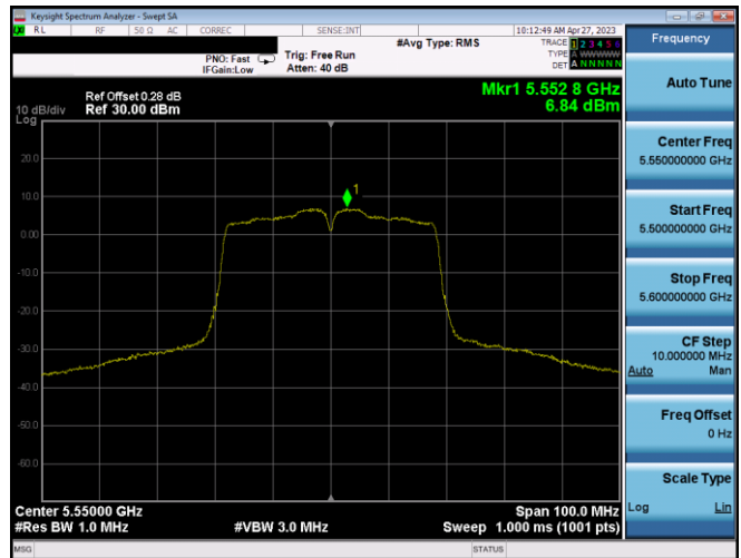
Plot 7-353. PSD CDD Ant1 (40MHz BW 802.11n – Ch. 110, MCS10)
