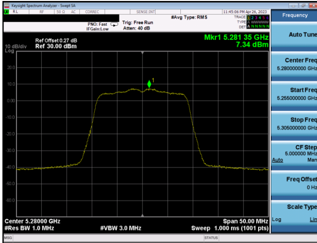
Plot 7-373. PSD CDD Ant1 (20MHz BW 802.11n – Ch. 56, MCS12)
