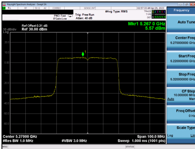
Plot 7-344. PSD CDD Ant2 (40MHz BW 802.11ax(SU) – Ch. 54, MCS2)
