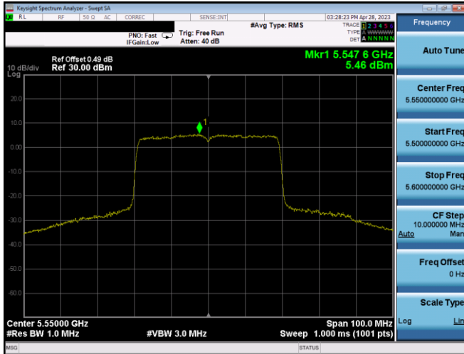
Plot 7-391. PSD CDD Ant1 (40MHz BW 802.11ax(SU) – Ch. 110, MCS4)
