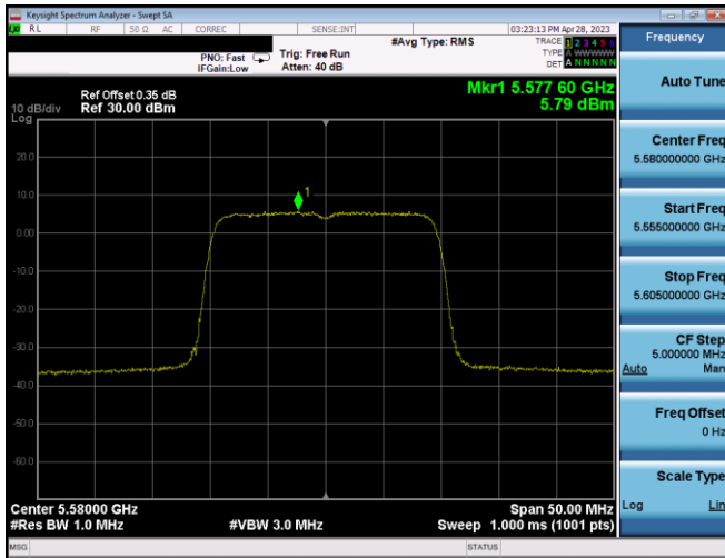
Plot 7-387. PSD CDD Ant1 (20MHz BW 802.11ax(SU) – Ch. 116, MCS4)
