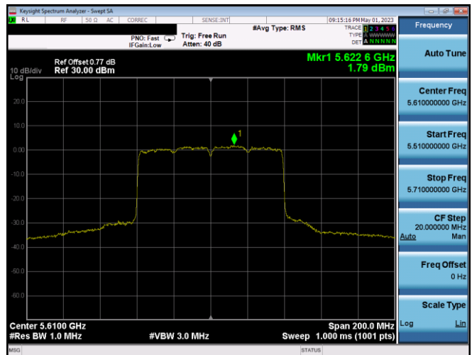
Plot 7-395. PSD CDD Ant1 (80MHz BW 802.11ax(SU) – Ch. 122, MCS4)
