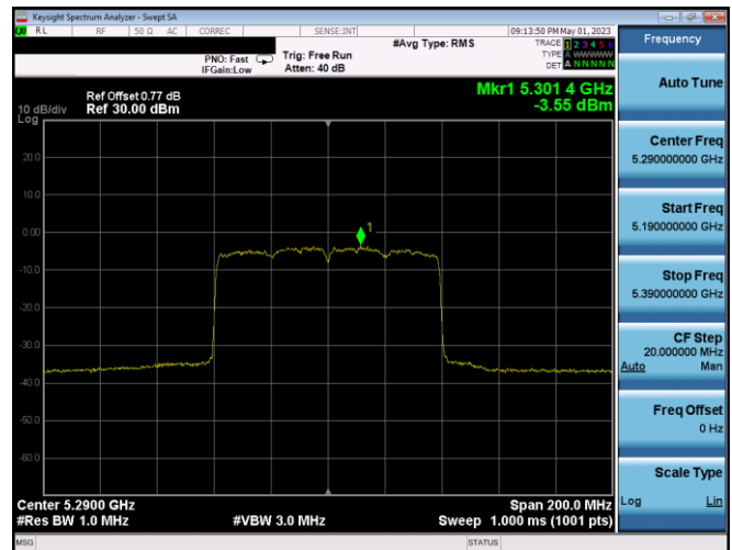
Plot 7-383. PSD CDD Ant1 (80MHz BW 802.11ax(SU) – Ch. 58, MCS4)
