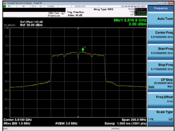
Plot 7-394. PSD CDD Ant2 (80MHz BW 802.11ac – Ch. 122, MCS4)
