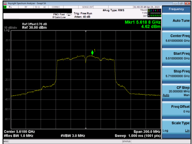
Plot 7-358. PSD CDD Ant2 (80MHz BW 802.11ac – Ch. 122, MCS2)
