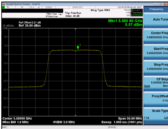
Plot 7-351. PSD CDD Ant1 (20MHz BW 802.11ax(SU) – Ch. 116, MCS2)
