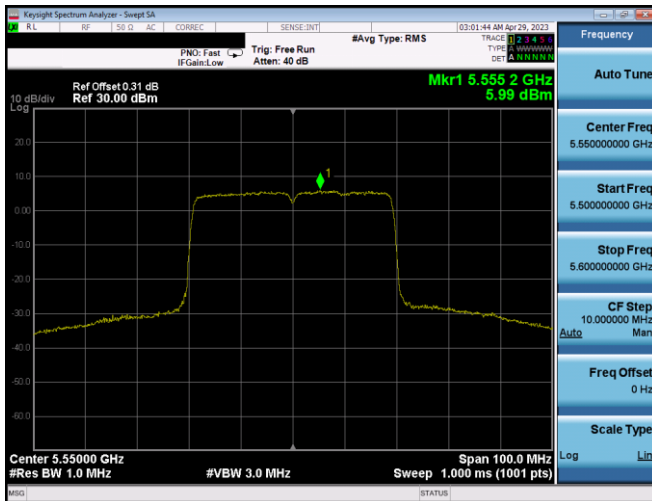
Plot 7-356. PSD CDD Ant2 (40MHz BW 802.11ax(SU) – Ch. 110, MCS2)
