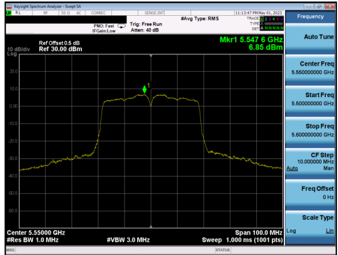
Plot 7-389. PSD CDD Ant1 (40MHz BW 802.11n – Ch. 110, MCS12)
