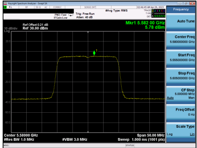
Plot 7-352. PSD CDD Ant2 (20MHz BW 802.11ax(SU) – Ch. 116, MCS2)
