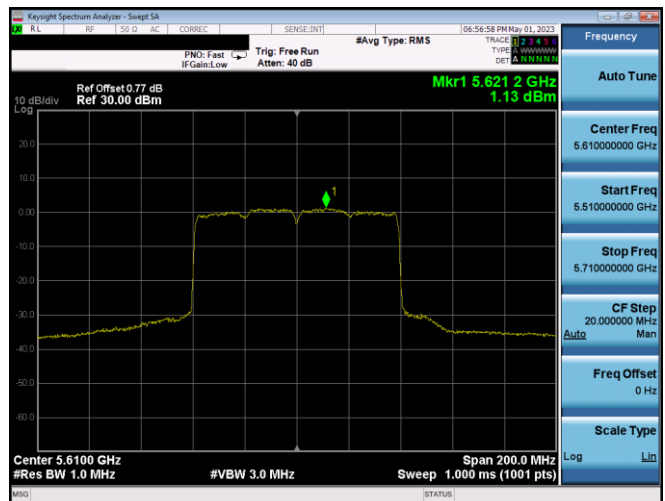
Plot 7-396. PSD CDD Ant2 (80MHz BW 802.11ax(SU) – Ch. 122, MCS4)
