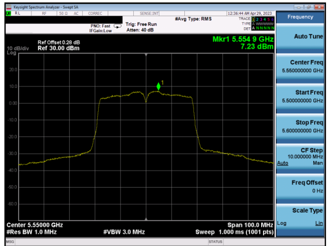
Plot 7-354. PSD CDD Ant2 (40MHz BW 802.11n – Ch. 110, MCS10)
