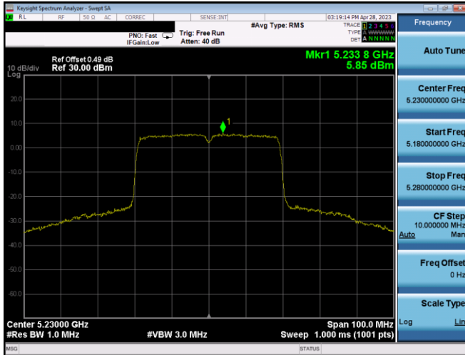
Plot 7-367. PSD CDD Ant1 (40MHz BW 802.11ax(SU) – Ch. 46, MCS4)
