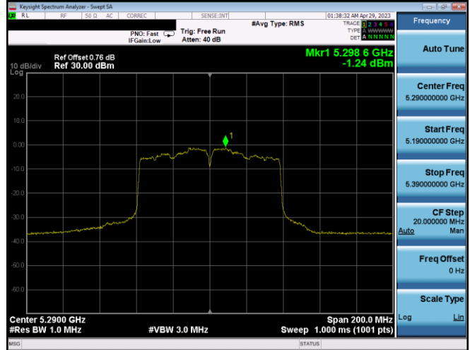
Plot 7-346. PSD CDD Ant2 (80MHz BW 802.11ac – Ch. 58, MCS2)
