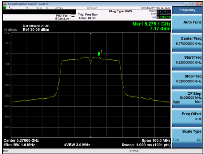
Plot 7-341. PSD CDD Ant1 (40MHz BW 802.11n – Ch. 54, MCS10)
