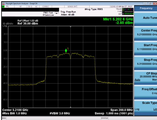
Plot 7-369. PSD CDD Ant1 (80MHz BW 802.11ac – Ch. 42, MCS4)
