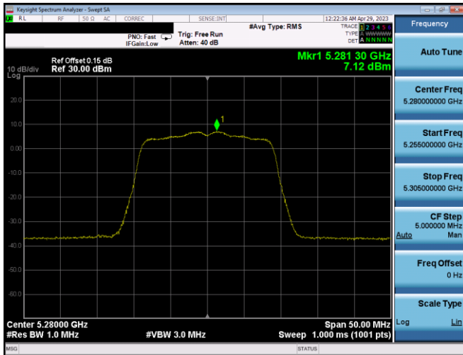
Plot 7-338. PSD CDD Ant2 (20MHz BW 802.11n – Ch. 56, MCS10)
