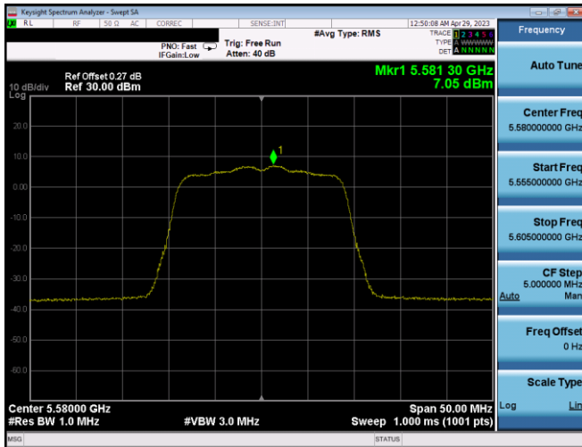
Plot 7-386. PSD CDD Ant2 (20MHz BW 802.11n – Ch. 116, MCS12)
