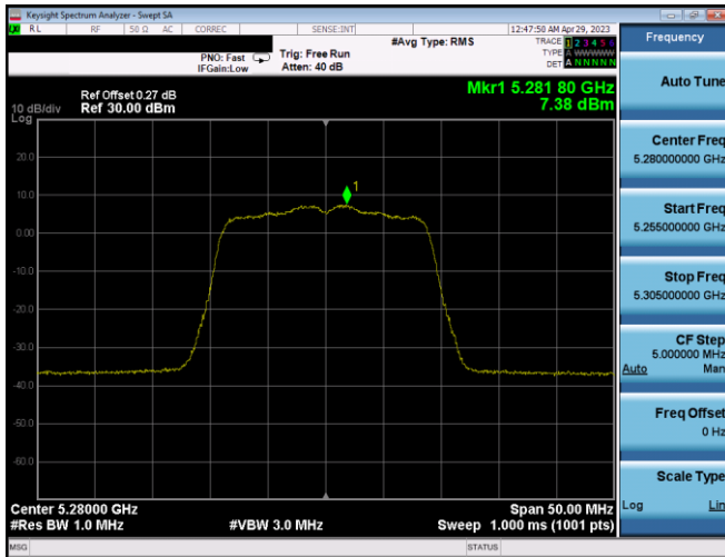
Plot 7-374. PSD CDD Ant2 (20MHz BW 802.11n – Ch. 56, MCS12)
