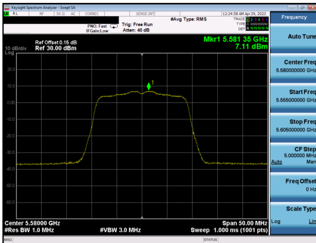
Plot 7-350. PSD CDD Ant2 (20MHz BW 802.11n – Ch. 116, MCS10)
