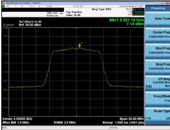
Plot 7-349. PSD CDD Ant1 (20MHz BW 802.11n – Ch. 116, MCS10)
