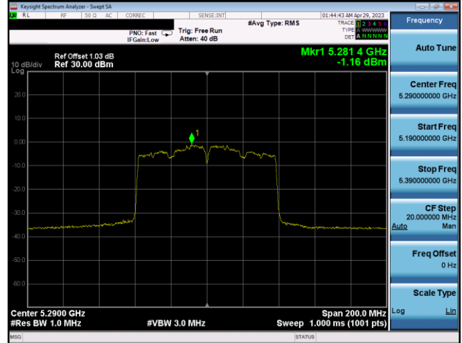
Plot 7-382. PSD CDD Ant2 (80MHz BW 802.11ac – Ch. 58, MCS4)
