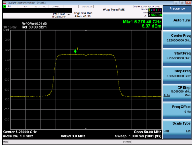
Plot 7-340. PSD CDD Ant2 (20MHz BW 802.11ax(SU) – Ch. 56, MCS2)
