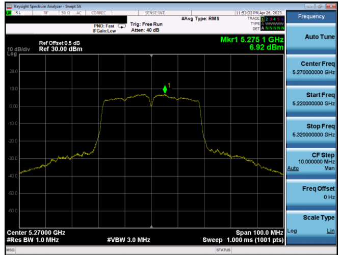
Plot 7-377. PSD CDD Ant1 (40MHz BW 802.11n – Ch. 54, MCS12)
