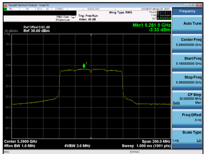
Plot 7-348. PSD CDD Ant2 (80MHz BW 802.11ax(SU) – Ch. 58, MCS2)
