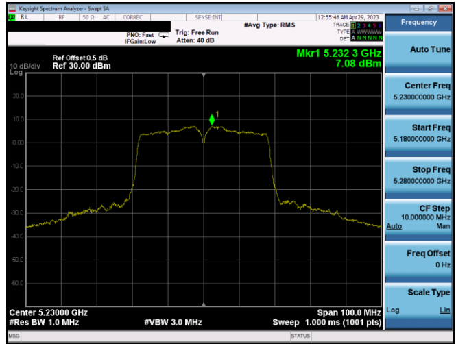
Plot 7-366. PSD CDD Ant2 (40MHz BW 802.11n – Ch. 46, MCS12)
