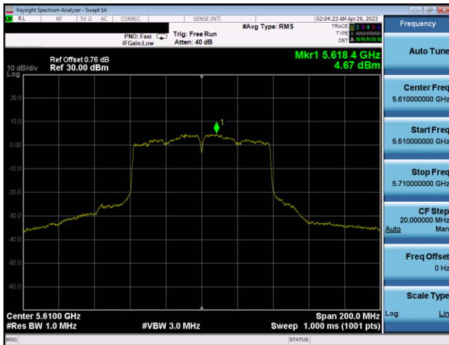
Plot 7-357. PSD CDD Ant1 (80MHz BW 802.11ac – Ch. 122, MCS2)
