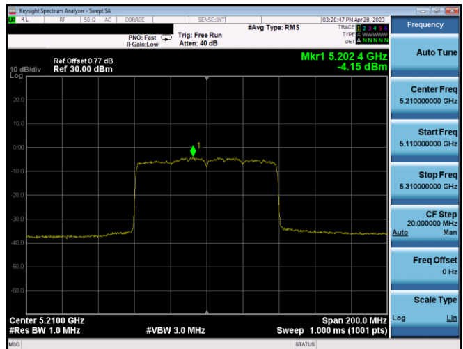
Plot 7-371. PSD CDD Ant1 (80MHz BW 802.11ax(SU) – Ch. 42, MCS4)
