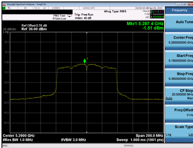
Plot 7-345. PSD CDD Ant1 (80MHz BW 802.11ac – Ch. 58, MCS2)
