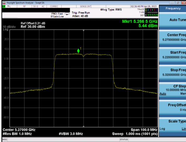
Plot 7-343. PSD CDD Ant1 (40MHz BW 802.11ax(SU) – Ch. 54, MCS2)
