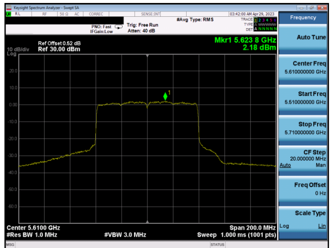
Plot 7-359. PSD CDD Ant1 (80MHz BW 802.11ax(SU) – Ch. 122, MCS2)
