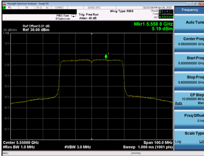
Plot 7-355. PSD CDD Ant1 (40MHz BW 802.11ax(SU) – Ch. 110, MCS2)
