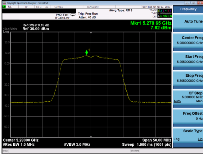
Plot 7-337. PSD CDD Ant1 (20MHz BW 802.11n – Ch. 56, MCS10)
