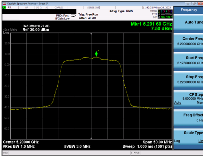
Plot 7-361. PSD CDD Ant1 (20MHz BW 802.11n – Ch. 40, MCS12)
