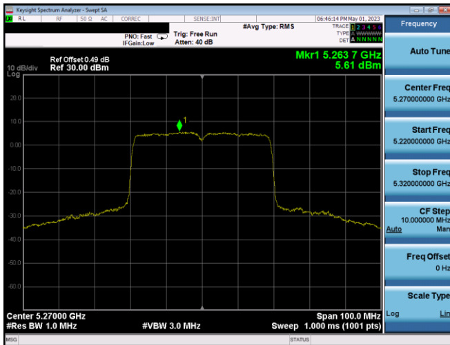
Plot 7-380. PSD CDD Ant2 (40MHz BW 802.11ax(SU) – Ch. 54, MCS4)
