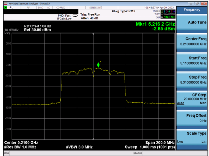
Plot 7-370. PSD CDD Ant2 (80MHz BW 802.11ac – Ch. 42, MCS4)
