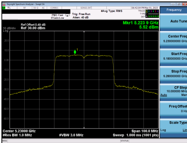
Plot 7-368. PSD CDD Ant2 (40MHz BW 802.11ax(SU) – Ch. 46, MCS4)
