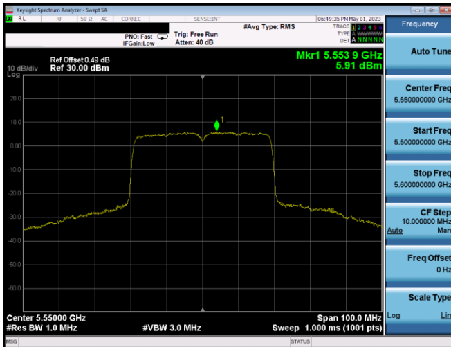
Plot 7-392. PSD CDD Ant2 (40MHz BW 802.11ax(SU) – Ch. 110, MCS4)
