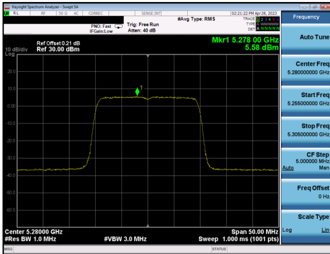
Plot 7-339. PSD CDD Ant1 (20MHz BW 802.11ax(SU) – Ch. 56, MCS2)
