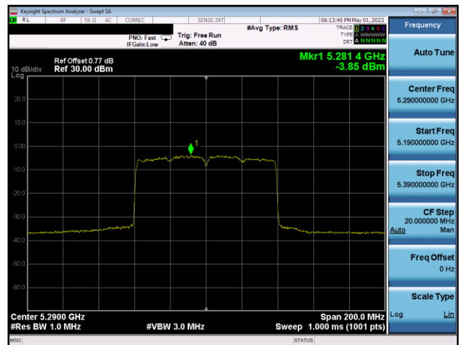
Plot 7-384. PSD CDD Ant2 (80MHz BW 802.11ax(SU) – Ch. 58, MCS4)
