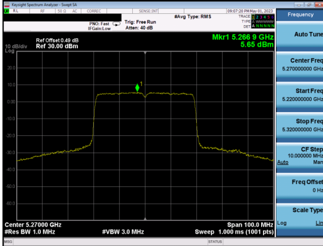
Plot 7-379. PSD CDD Ant1 (40MHz BW 802.11ax(SU) – Ch. 54, MCS4)
