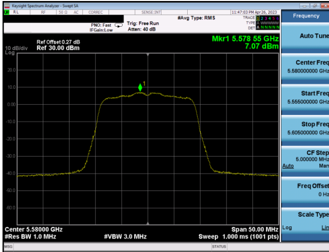
Plot 7-385. PSD CDD Ant1 (20MHz BW 802.11n – Ch. 116, MCS12)
