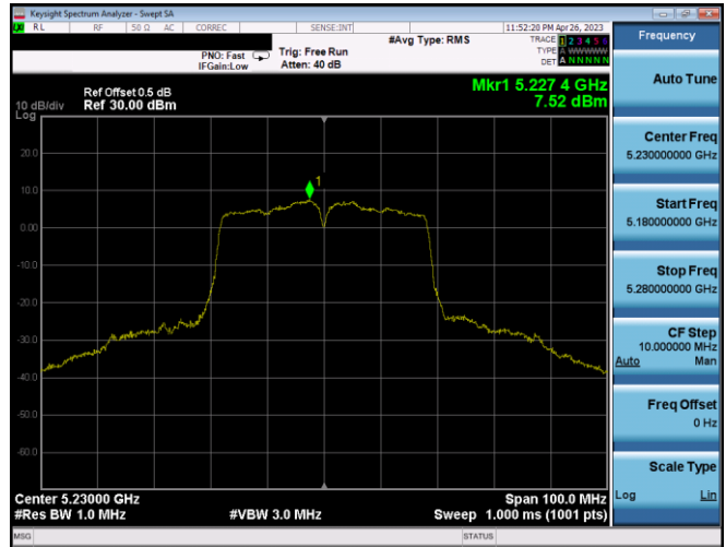
Plot 7-365. PSD CDD Ant1 (40MHz BW 802.11n – Ch. 46, MCS12)
