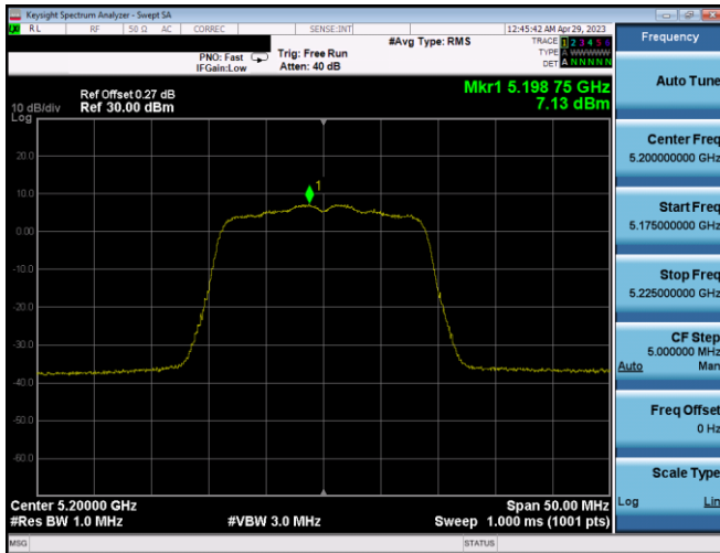
Plot 7-362. PSD CDD Ant2 (20MHz BW 802.11n – Ch. 40, MCS12)
