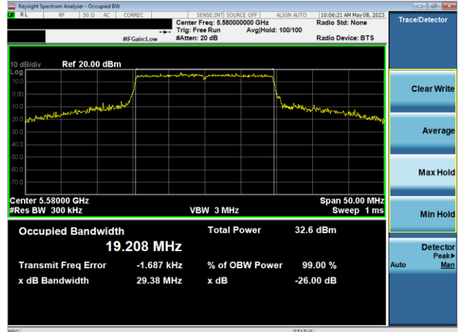
Plot 7-28. 26dB BW & 99% OBW Ant 1 (20MHz BW 11ax – RU242 – Ch.116)
