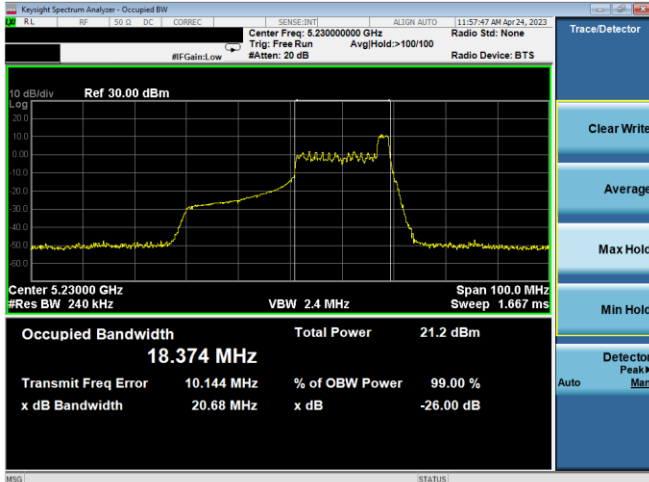
Plot 7-7. 26dB BW & 99% OBW Ant 1 (40MHz BW 11ax Index 17 – RU26 – Ch.46)
