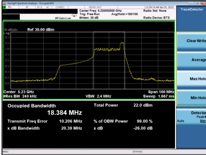
Plot 7-43. 26dB BW & 99% OBW Ant 2 (40MHz BW 11ax Index 17 – RU26 – Ch.46)
