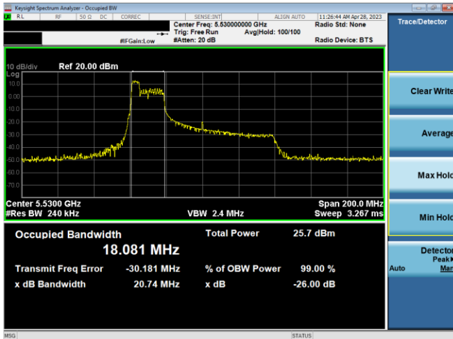
Plot 7-33. 26dB BW & 99% OBW Ant 1 (80MHz BW 11ax Index 37 – RU52 – Ch.106)
