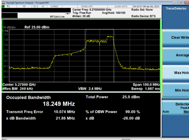
Plot 7-19. 26dB BW & 99% OBW Ant 1 (40MHz BW 11ax Index 44 – RU52 – Ch.54)
