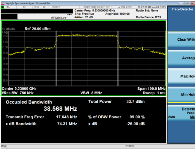
Plot 7-8. 26dB BW & 99% OBW Ant 1 (40MHz BW 11ax – RU484 – Ch.46)
