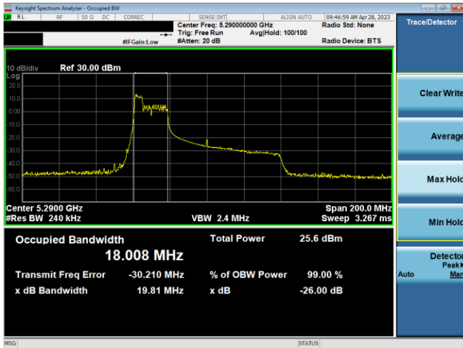
Plot 7-21. 26dB BW & 99% OBW Ant 1 (80MHz BW 11ax Index 37 – RU52 – Ch.58)
