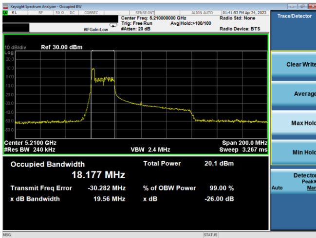
Plot 7-9. 26dB BW & 99% OBW Ant 1 (80MHz BW 11ax Index 0 – RU26 – Ch.42)
