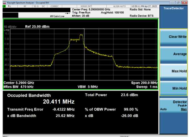
Plot 7-58. 26dB BW & 99% OBW Ant 2 (80MHz BW 11ax Index 44 – RU52 – Ch.58)
