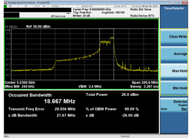
Plot 7-35. 26dB BW & 99% OBW Ant 1 (80MHz BW 11ax Index 52 – RU52 – Ch.106)
