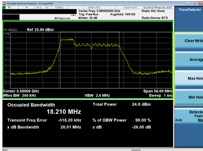
Plot 7-25. 26dB BW & 99% OBW Ant 1 (20MHz BW 11ax Index 37 – RU52 – Ch.116)
