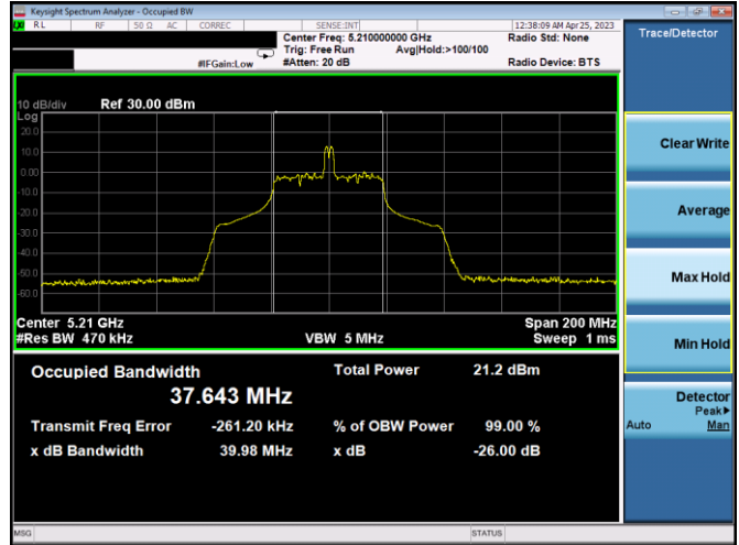
Plot 7-46. 26dB BW & 99% OBW Ant 2 (80MHz BW 11ax Index 18 – RU26 – Ch.42)
