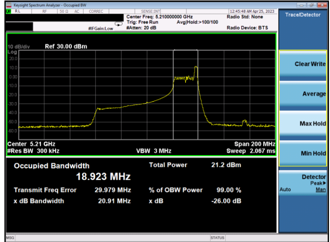
Plot 7-47. 26dB BW & 99% OBW Ant 2 (80MHz BW 11ax Index 36 – RU26 – Ch.42)
