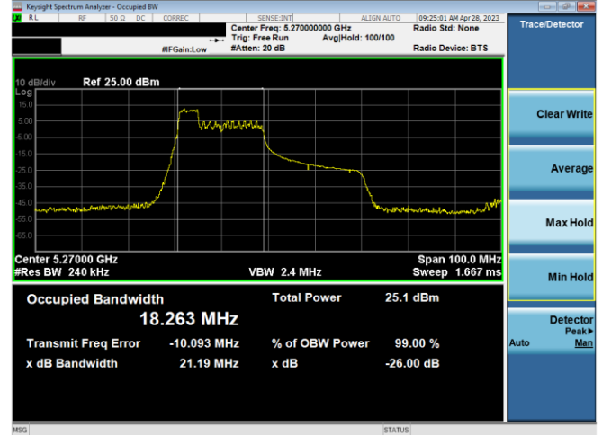
Plot 7-17. 26dB BW & 99% OBW Ant 1 (40MHz BW 11ax Index 37 – RU52 – Ch.54)
