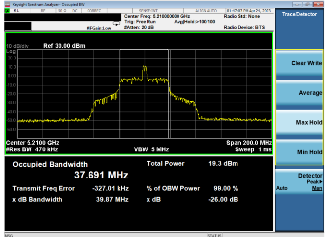
Plot 7-10. 26dB BW & 99% OBW Ant 1 (80MHz BW 11ax Index 18 – RU26 – Ch.42)
