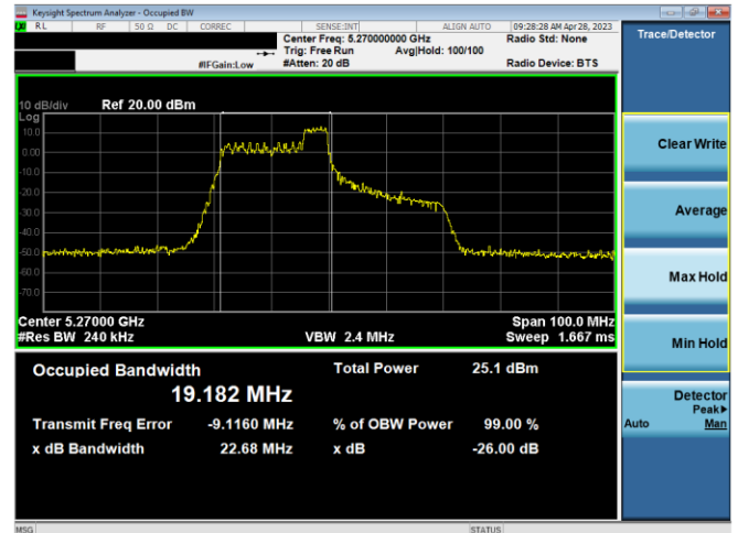
Plot 7-18. 26dB BW & 99% OBW Ant 1 (40MHz BW 11ax Index 40 – RU52 – Ch.54)
