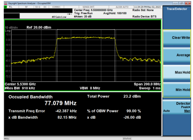
Plot 7-36. 26dB BW & 99% OBW Ant 1 (80MHz BW 11ax – RU996 – Ch.106)
