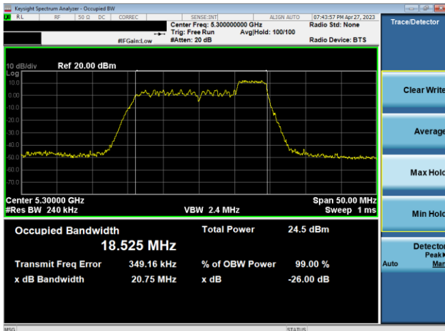
Plot 7-51. 26dB BW & 99% OBW Ant 2 (20MHz BW 11ax Index 40– RU52 – Ch.60)
