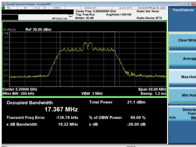
Plot 7-38. 26dB BW & 99% OBW Ant 2 (20MHz BW 11ax Index 4 – RU26 – Ch.40)
