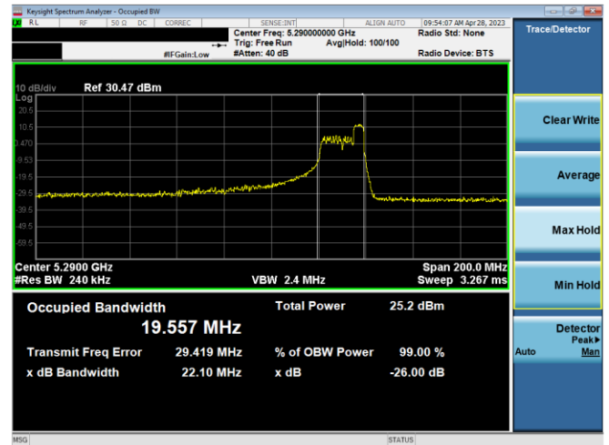
Plot 7-23. 26dB BW & 99% OBW Ant 1 (80MHz BW 11ax Index 52 – RU52 – Ch.58)
