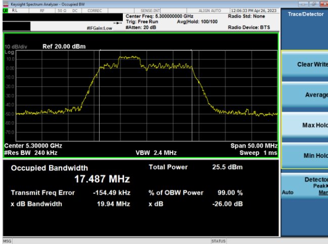
Plot 7-14. 26dB BW & 99% OBW Ant 1 (20MHz BW 11ax Index 38 – RU52 – Ch.60)
