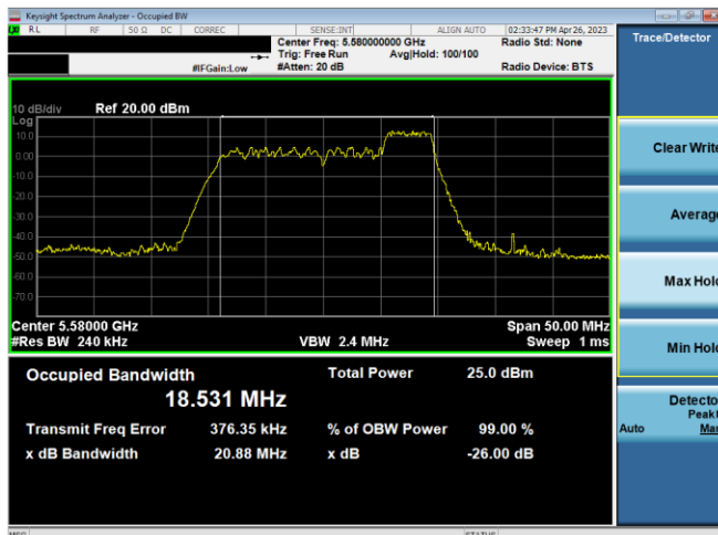
Plot 7-27. 26dB BW & 99% OBW Ant 1 (20MHz BW 11ax Index 40 – RU52 – Ch.116)
