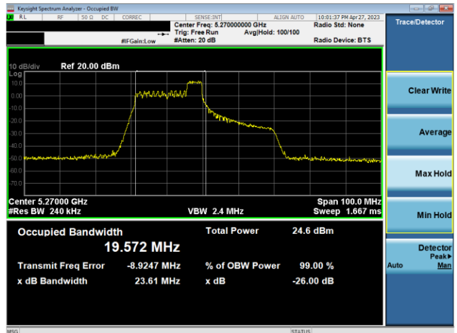
Plot 7-54. 26dB BW & 99% OBW Ant 2 (40MHz BW 11ax Index 44 – RU52 – Ch.54)
