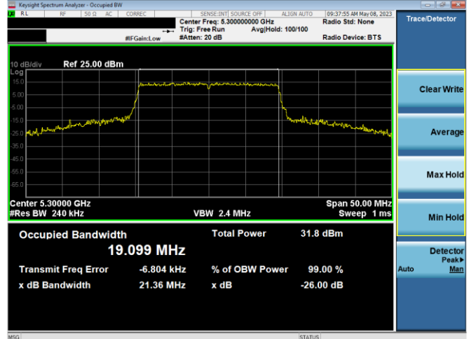
Plot 7-16. 26dB BW & 99% OBW Ant 1 (20MHz BW 11ax– RU242 – Ch.60)
