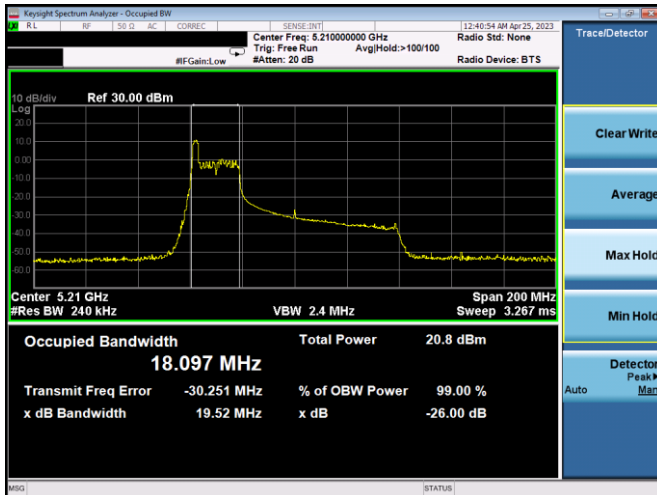
Plot 7-45. 26dB BW & 99% OBW Ant 2 (80MHz BW 11ax Index 0 – RU26 – Ch.42)
