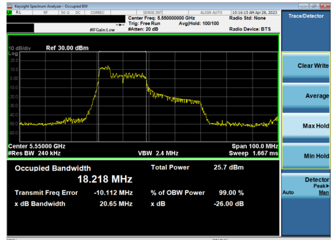
Plot 7-29. 26dB BW & 99% OBW Ant 1 (40MHz BW 11ax Index 37 – RU52 – Ch.110)
