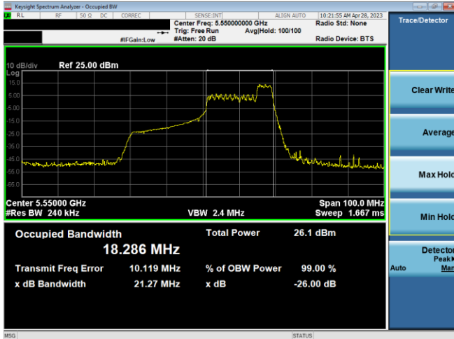
Plot 7-31. 26dB BW & 99% OBW Ant 1 (40MHz BW 11ax Index 44 – RU52 – Ch.110)
