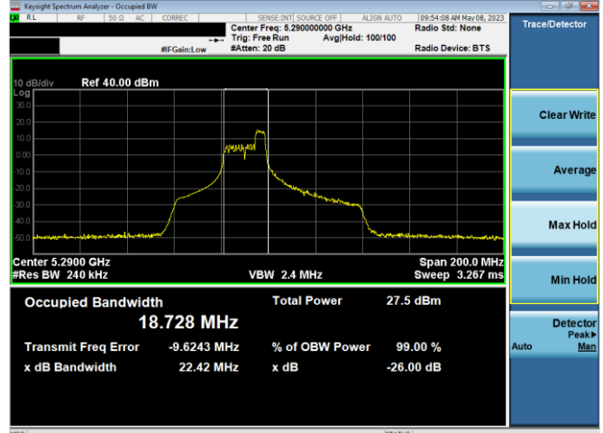
Plot 7-22. 26dB BW & 99% OBW Ant 1 (80MHz BW 11ax Index 44 – RU52 – Ch.58)
