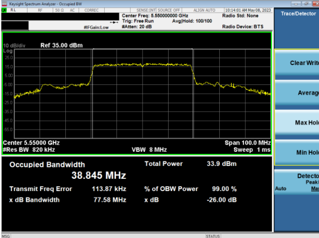
Plot 7-32. 26dB BW & 99% OBW Ant 1 (40MHz BW 11ax – RU484 – Ch.110)
