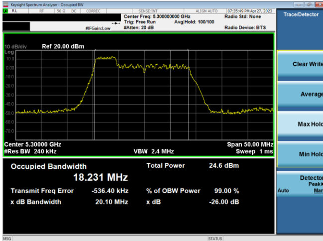
Plot 7-49. 26dB BW & 99% OBW Ant 2 (20MHz BW 11ax Index 37 – RU52 – Ch.60)
