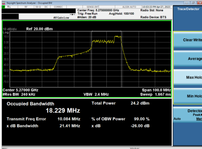
Plot 7-55. 26dB BW & 99% OBW Ant 2 (40MHz BW 11ax Index 44 – RU52 – Ch.54)
