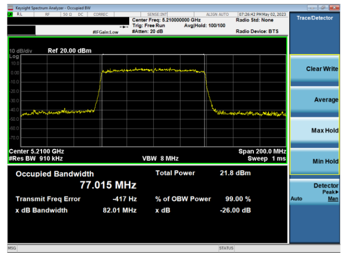
Plot 7-48. 26dB BW & 99% OBW Ant 2 (80MHz BW 11ax – RU996 – Ch.42)
