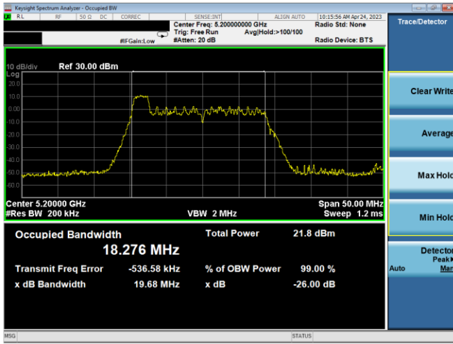
Plot 7-1. 26dB BW & 99% OBW Ant 1 (20MHz BW 11ax Index 0 – RU26 – Ch.40)
