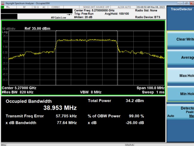
Plot 7-20. 26dB BW & 99% OBW Ant 1 (40MHz BW 11ax – RU484 – Ch.54)
