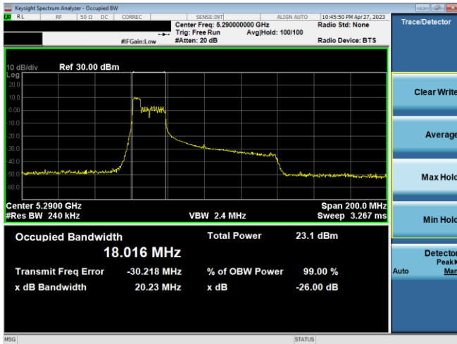
Plot 7-57. 26dB BW & 99% OBW Ant 2 (80MHz BW 11ax Index 37 – RU52 – Ch.58)
