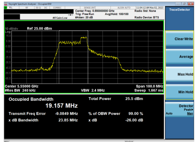
Plot 7-30. 26dB BW & 99% OBW Ant 1 (40MHz BW 11ax Index 40 – RU52 – Ch.110)
