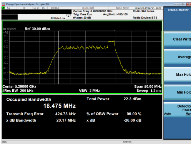
Plot 7-3. 26dB BW & 99% OBW Ant 1 (20MHz BW 11ax Index 8 – RU26 – Ch.40)
