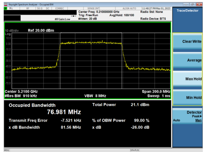
Plot 7-12. 26dB BW & 99% OBW Ant 1 (80MHz BW 11ax – RU996 – Ch.42)
