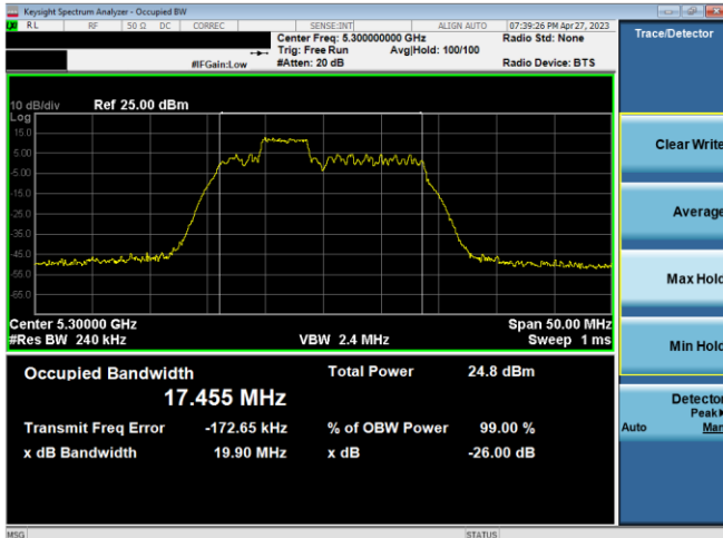
Plot 7-50. 26dB BW & 99% OBW Ant 2 (20MHz BW 11ax Index 38 – RU52 – Ch.60)
