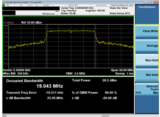
Plot 7-40. 26dB BW & 99% OBW Ant 2 (20MHz BW 11ax– RU242 – Ch.40)
