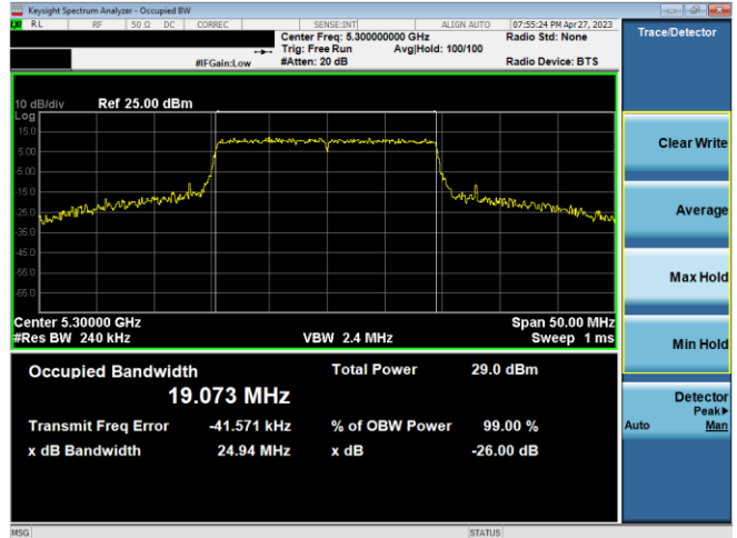
Plot 7-52. 26dB BW & 99% OBW Ant 2 (20MHz BW 11ax– RU242 – Ch.60)
