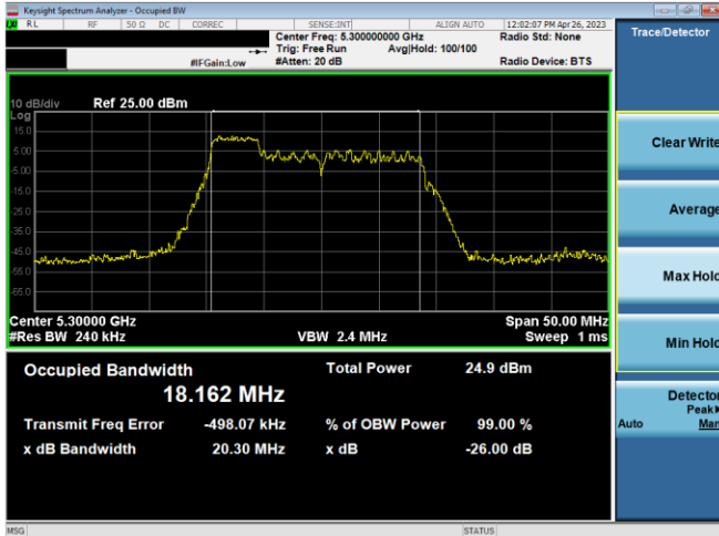
Plot 7-13. 26dB BW & 99% OBW Ant 1 (20MHz BW 11ax Index 37 – RU52 – Ch.60)
