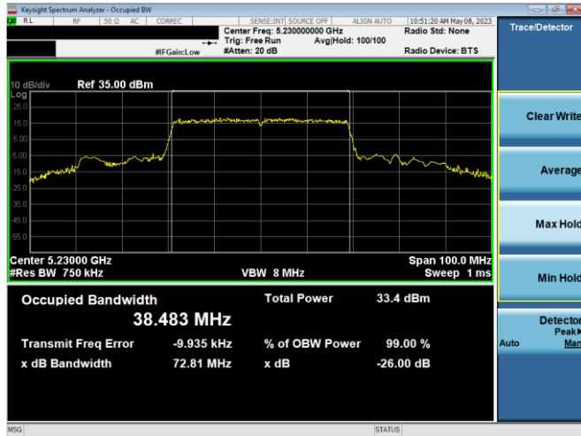
Plot 7-44. 26dB BW & 99% OBW Ant 2 (40MHz BW 11ax – RU484 – Ch.46)
