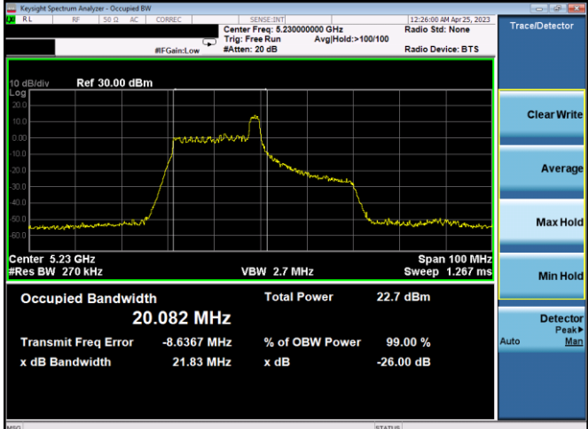
Plot 7-42. 26dB BW & 99% OBW Ant 2 (40MHz BW 11ax Index 8 – RU26 – Ch.46)
