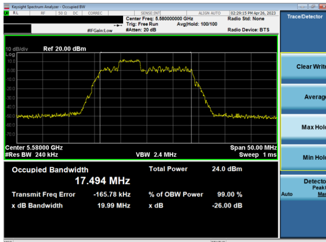
Plot 7-26. 26dB BW & 99% OBW Ant 1 (20MHz BW 11ax Index 38 – RU52 – Ch.116)
