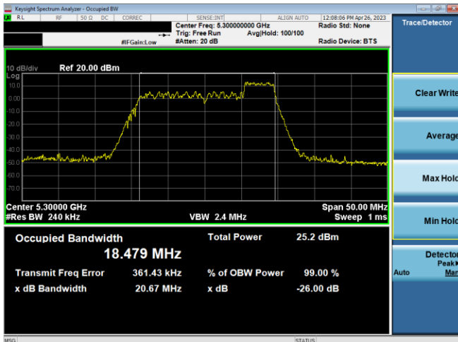
Plot 7-15. 26dB BW & 99% OBW Ant 1 (20MHz BW 11ax Index 40– RU52 – Ch.60)
