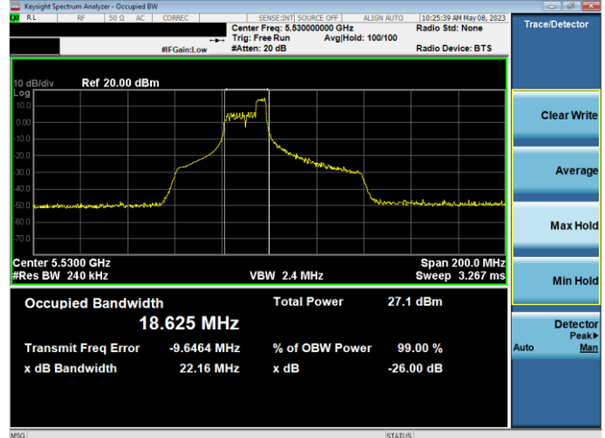
Plot 7-34. 26dB BW & 99% OBW Ant 1 (80MHz BW 11ax Index 44 – RU52 – Ch.106)
