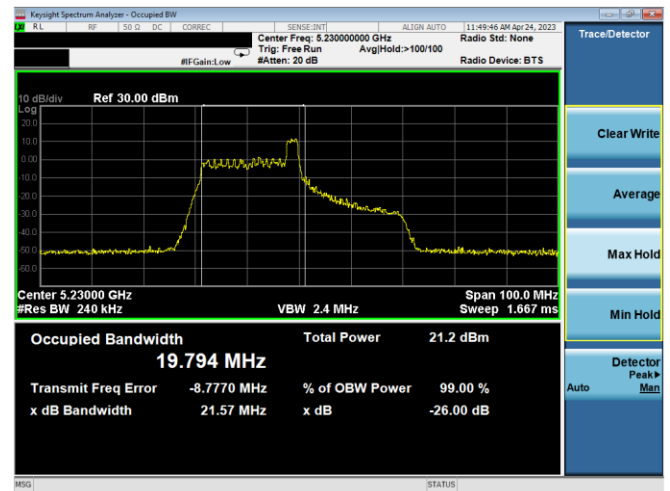
Plot 7-6. 26dB BW & 99% OBW Ant 1 (40MHz BW 11ax Index 8 – RU26 – Ch.46)
