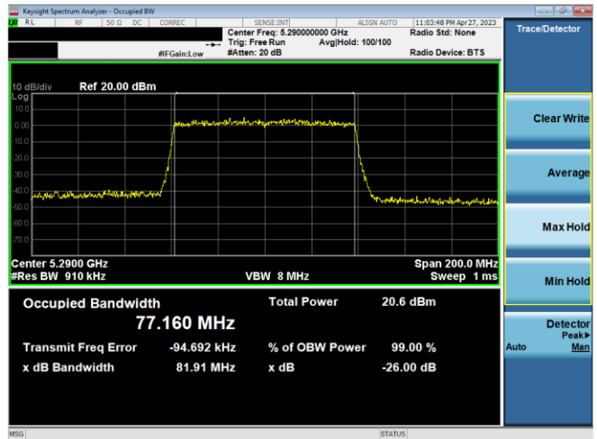
Plot 7-60. 26dB BW & 99% OBW Ant 2 (80MHz BW 11ax – RU996 – Ch.58)
