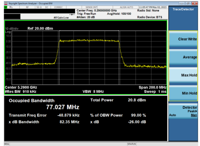
Plot 7-24. 26dB BW & 99% OBW Ant 1 (80MHz BW 11ax – RU996 – Ch.58)
