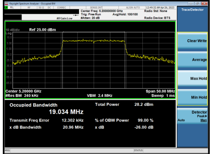
Plot 7-4. 26dB BW & 99% OBW Ant 1 (20MHz BW 11ax– RU242 – Ch.40)
