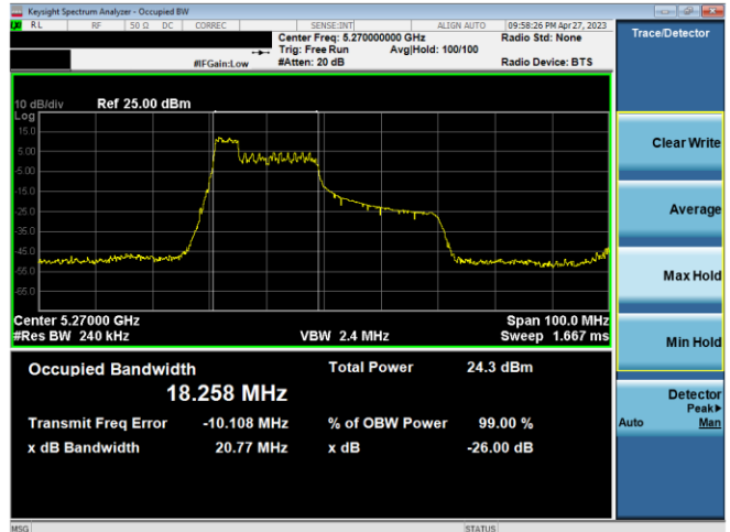
Plot 7-53. 26dB BW & 99% OBW Ant 2 (40MHz BW 11ax Index 37 – RU52 – Ch.54)
