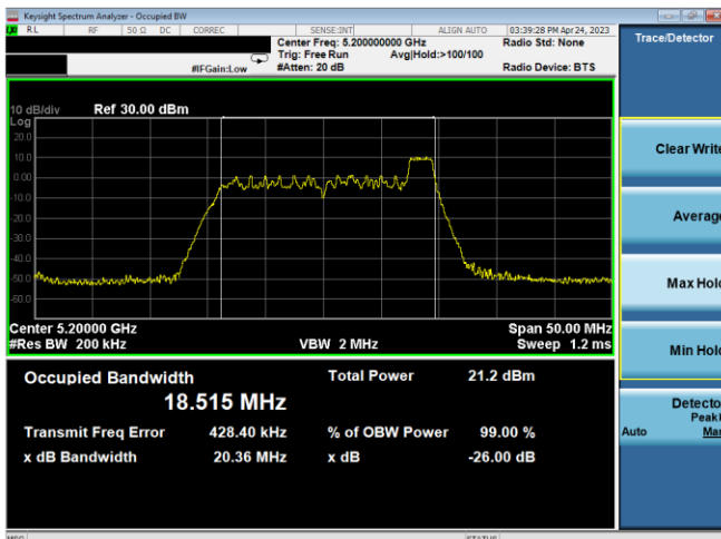
Plot 7-39. 26dB BW & 99% OBW Ant 2 (20MHz BW 11ax Index 8– RU26 – Ch.40)
