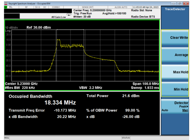
Plot 7-5. 26dB BW & 99% OBW Ant 1 (40MHz BW 11ax Index 0 – RU26 – Ch.46)
