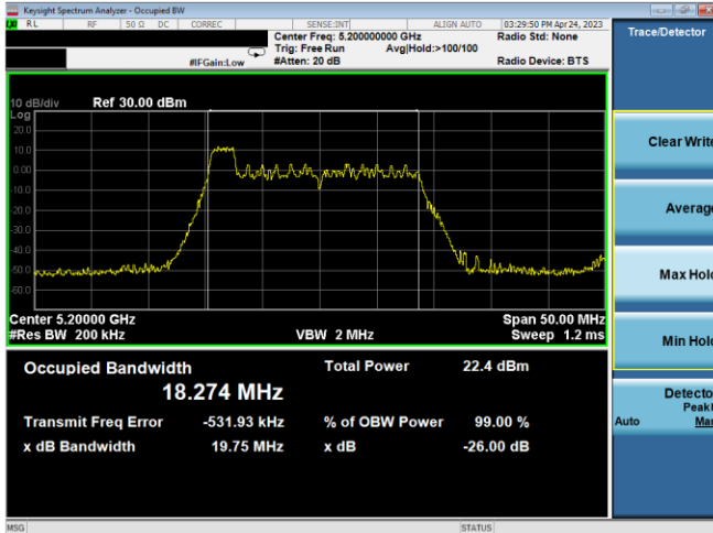
Plot 7-37. 26dB BW & 99% OBW Ant 2 (20MHz BW 11ax Index 0 – RU26 – Ch.40)
