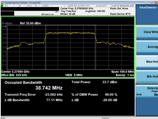
Plot 7-56. 26dB BW & 99% OBW Ant 2 (40MHz BW 11ax – RU484 – Ch.54)
