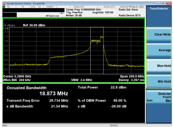
Plot 7-59. 26dB BW & 99% OBW Ant 2 (80MHz BW 11ax Index 52 – RU52 – Ch.58)
