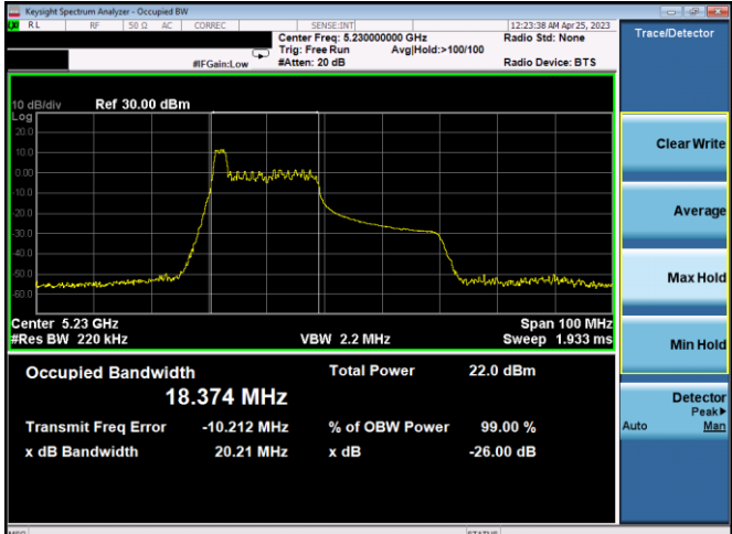
Plot 7-41. 26dB BW & 99% OBW Ant 2 (40MHz BW 11ax Index 0 – RU26 – Ch.46)
