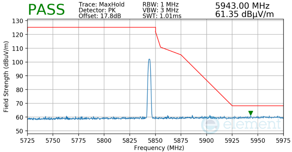
Plot 7-25. Radiated Upper Band Edge Measurement
