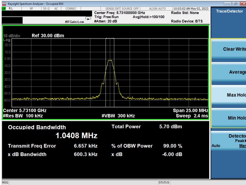
Plot 7-4. 6dB BW & 99% OBW (BDR, 5731MHz)
