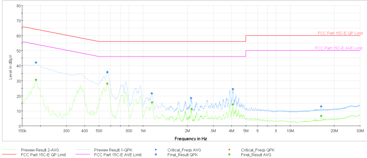
Plot 7-28. AC Line Conducted Plot (BDR – 5201MHz) (N) with AC/DC Adapter
