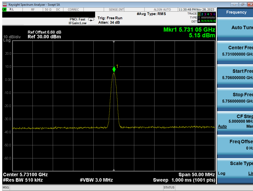
Plot 7-10. PSD (BDR, 5731MHz)
