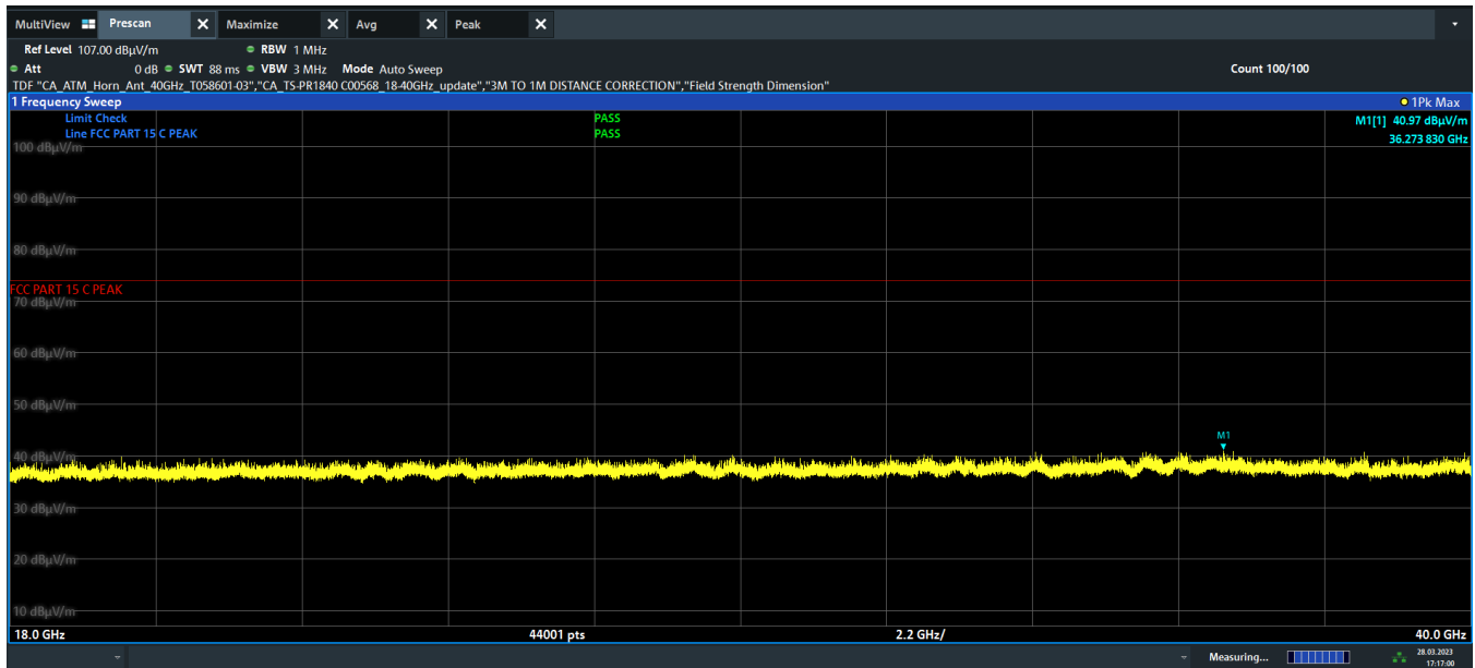
Plot 7-21. Radiated Spurious Emissions Above 18GHz (BDR – 5788MHz Pol. H)
