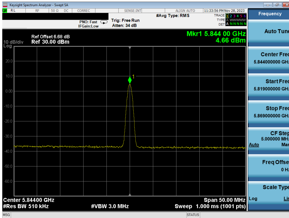
Plot 7-12. PSD (BDR, 5844MHz)
