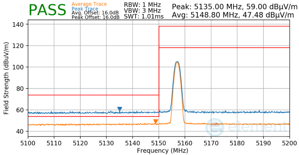
Plot 7-23. Radiated Lower Band Edge Measurement
