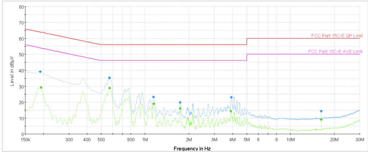
Plot 7-27. AC Line Conducted Plot (BDR – 5201MHz) (L1) with AC/DC Adapter
