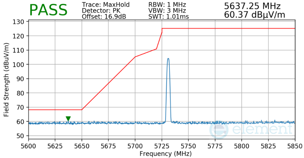
Plot 7-24. Radiated Lower Band Edge Measurement
