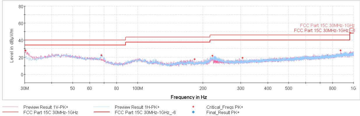
Plot 7-26. RSE 30MHz - 1GHz (BDR - 5201MHz), with AC/DC Adapter
