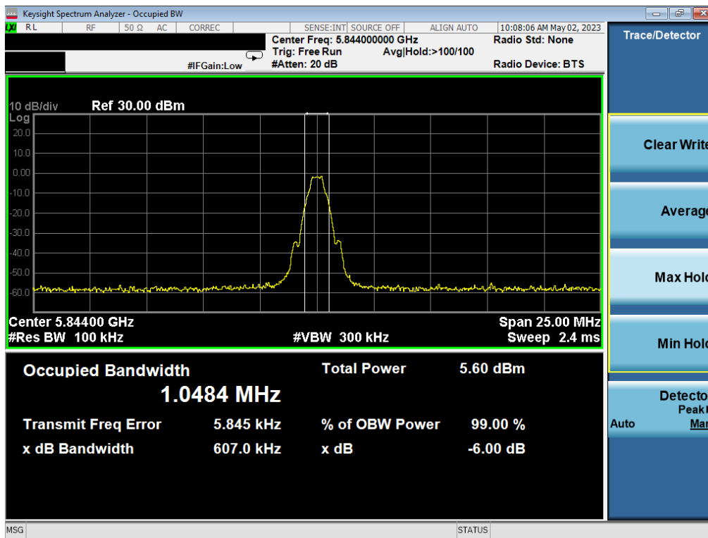
Plot 7-6. 6dB BW & 99% OBW (BDR, 5844MHz)
