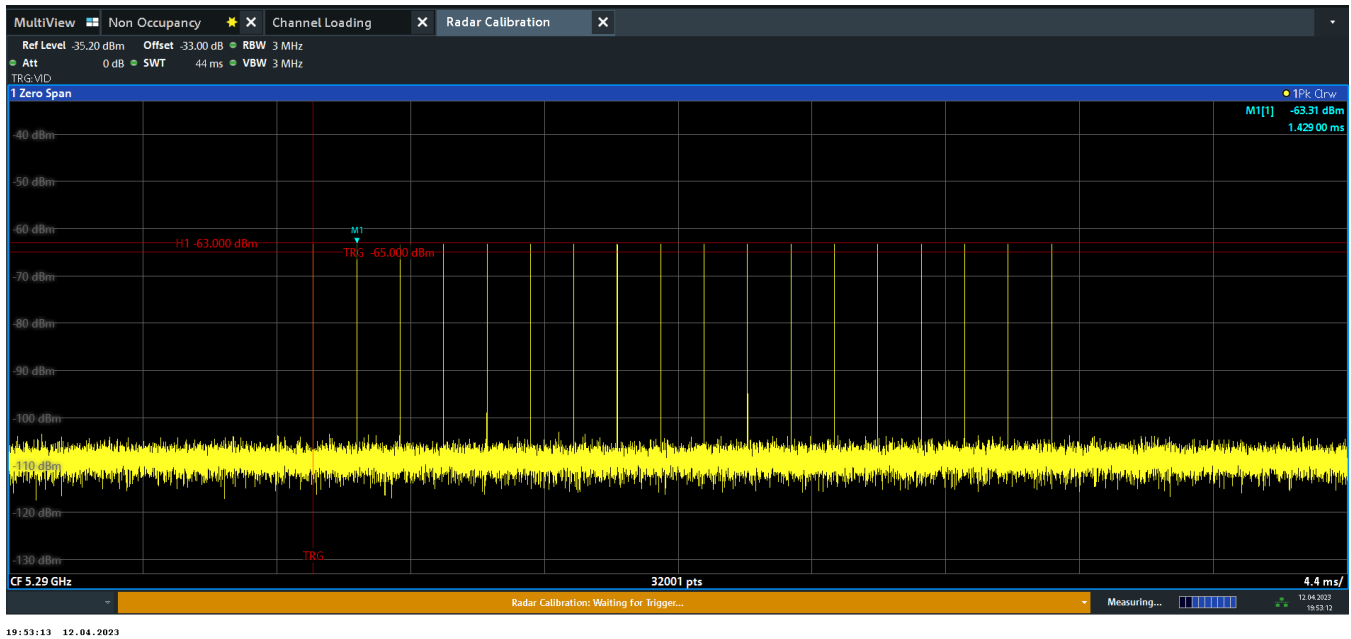
Figure 7-3. 5290MHz – Radar Pulse Type 0 (80MHz)
