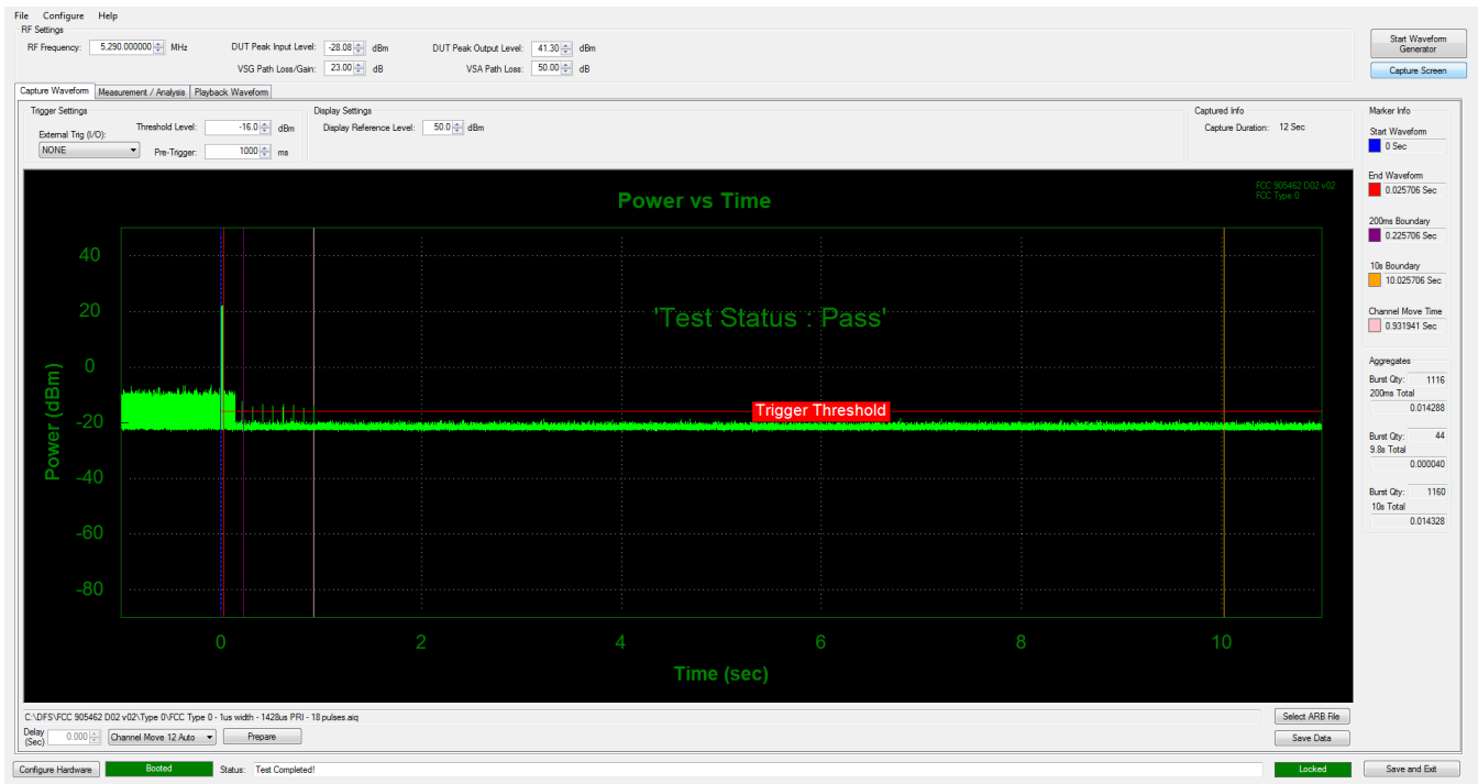
Figure 9-9. 5290MHz - Channel Move/ Closing Transmission Time - Mode 1 (80 MHz)
