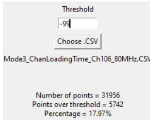
Figure 9-6. 5530MHz - Channel Loading Calculation - Mode 3 (80MHz)
