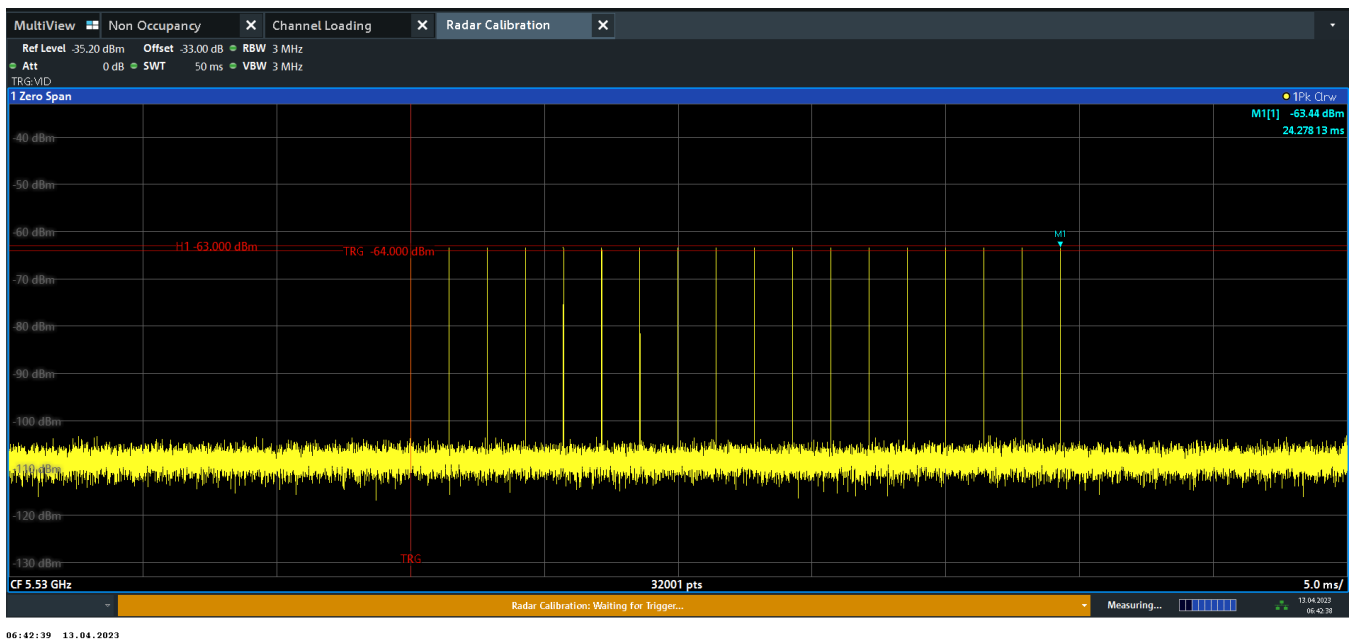
Figure 7-4. 5530MHz – Radar Pulse Type 0 (80MHz)
