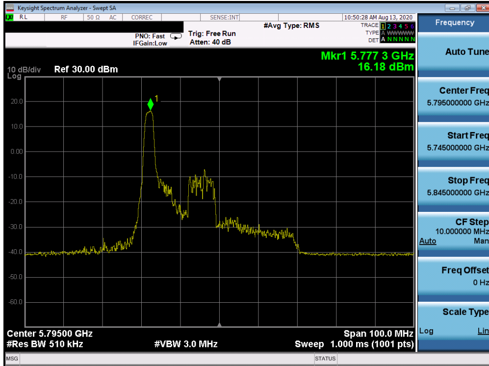
Plot 7-1157. Power Spectral Density Plot CDD Diversity Antenna 2b (40MHz BW 802.11ax Index 0 – RU26 (UNII Band 3) – Ch. 159)
