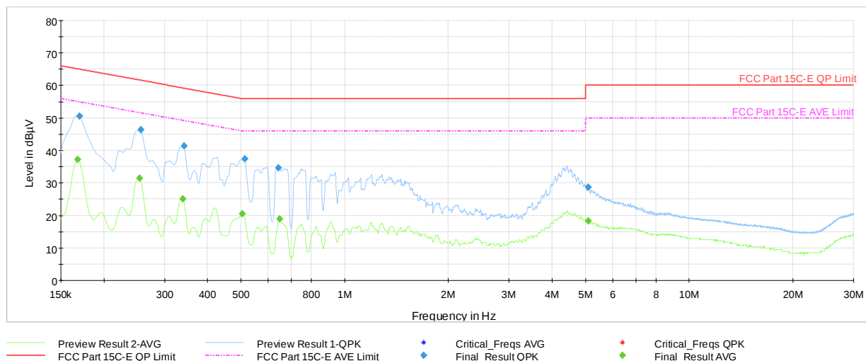
Plot 6-6. AC Line Conducted Plot (N, Charging Rate 10C, with AC/DC Adapter)
