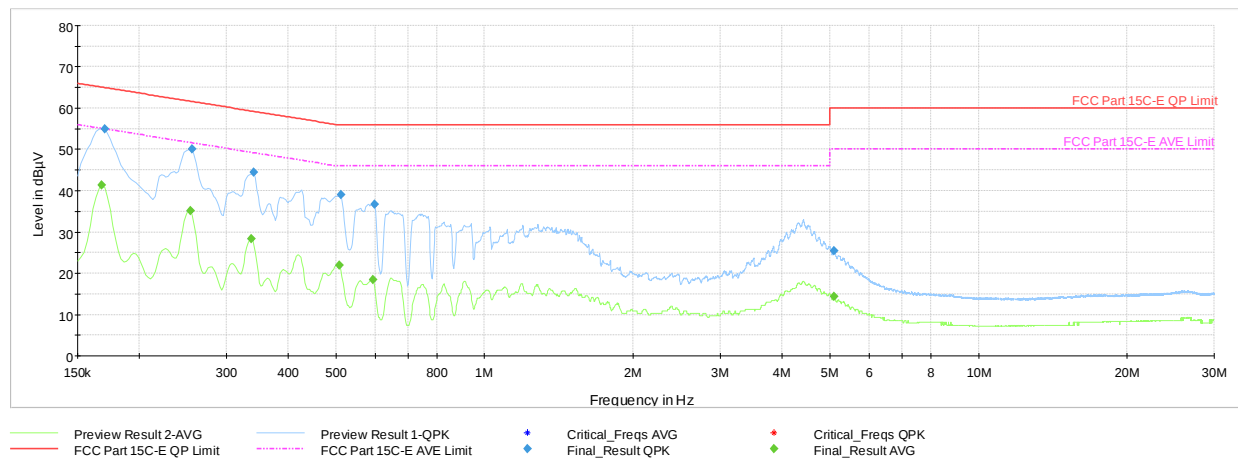
Plot 6-5. AC Line Conducted Plot (L1, Charging Rate 10C, with AC/DC Adapter)
