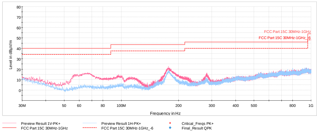
Plot 6-4. Radiated Spurious Emissions 30MHz-1000MHz (Charging Rate 10C, with AC/DC Adapter)
