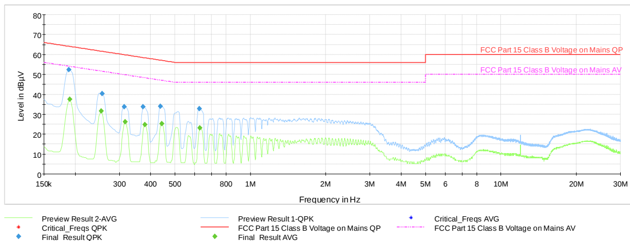
Plot 7-229. AC Line Conducted Emissions with 802.11ax (RU26) Ch.6 (L1, with Laptop)
