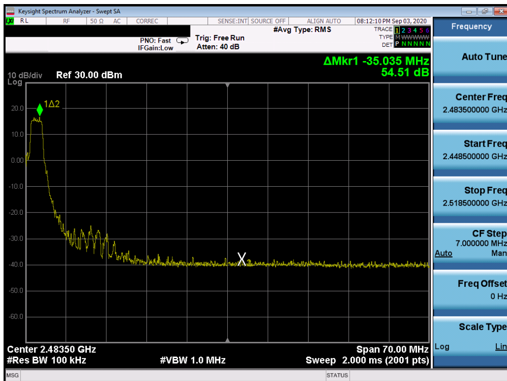
Plot 7-78. Band Edge Antenna 3a (802.11ax OFDMA – RU26 Index 8 – Ch. 7)
