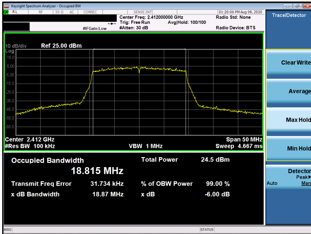
Plot 7-22. 6dB Bandwidth Plot Antenna 1a (802.11ax OFDMA – RU242 – Ch. 1)
