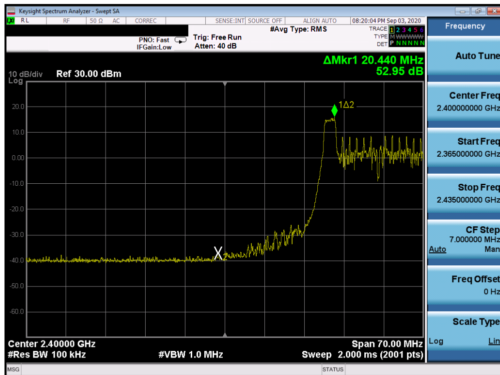
Plot 7-76. Band Edge Antenna 3a (802.11ax OFDMA – RU26 Index 0 – Ch. 4)
