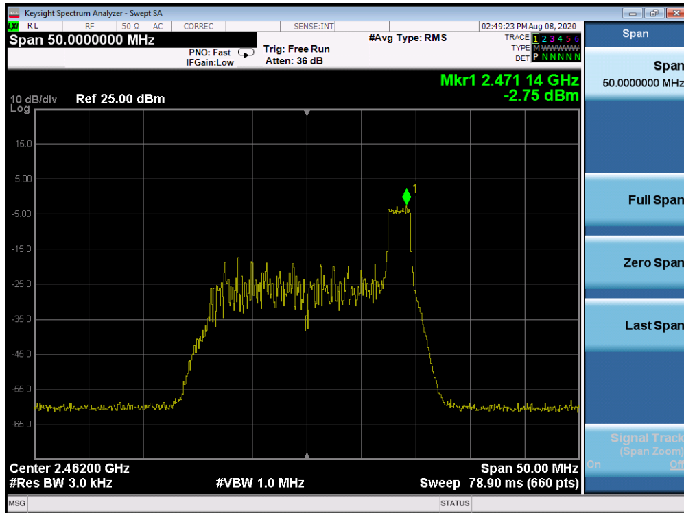
Plot 7-45. Power Spectral Density Plot Antenna 1a (802.11ax OFDMA – RU26 Index 8 – Ch. 11)
