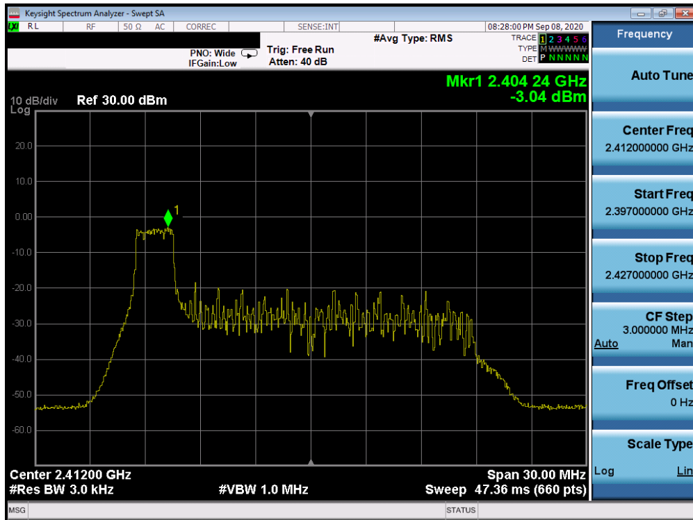
Plot 7-37. Power Spectral Density Plot Antenna 1a (802.11ax OFDMA – RU26 Index 0 – Ch. 1)
