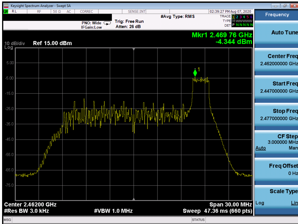
Plot 7-65. Power Spectral Density Plot CDD Antenna 3a (802.11ax OFDMA – RU26 Index 8 – Ch. 11)
