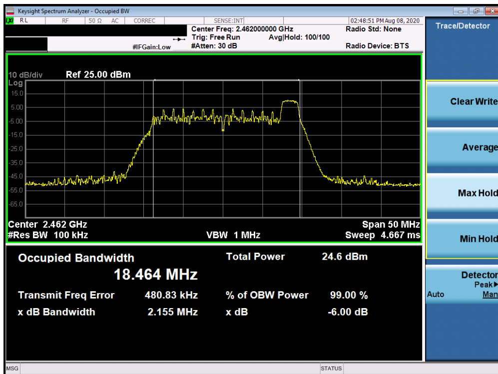
Plot 7-21. 6dB Bandwidth Plot Antenna 1a (802.11ax OFDMA – RU26 Index 8 – Ch. 11)
