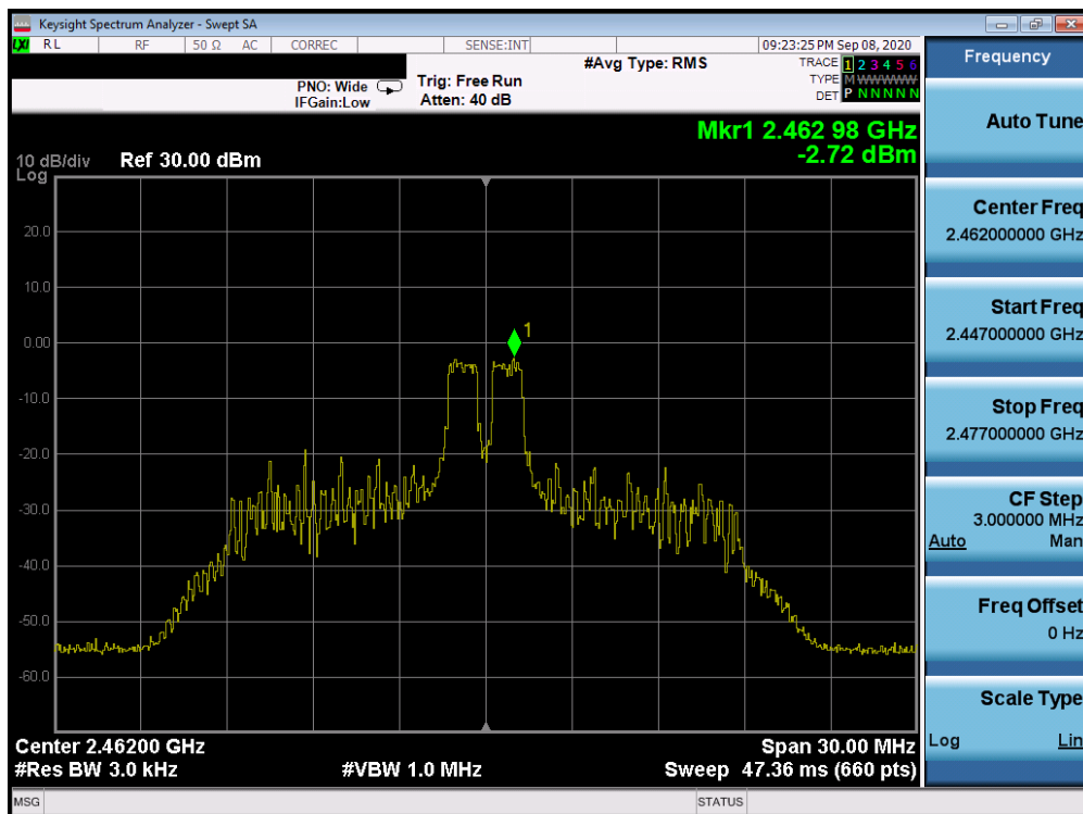
Plot 7-44. Power Spectral Density Plot Antenna 1a (802.11ax OFDMA – RU26 Index 4 – Ch. 11)
