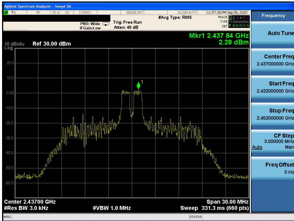
Plot 7-57. Power Spectral Density Plot CDD Antenna 3a (802.11ax OFDMA – RU26 Index 4 – Ch. 6)
