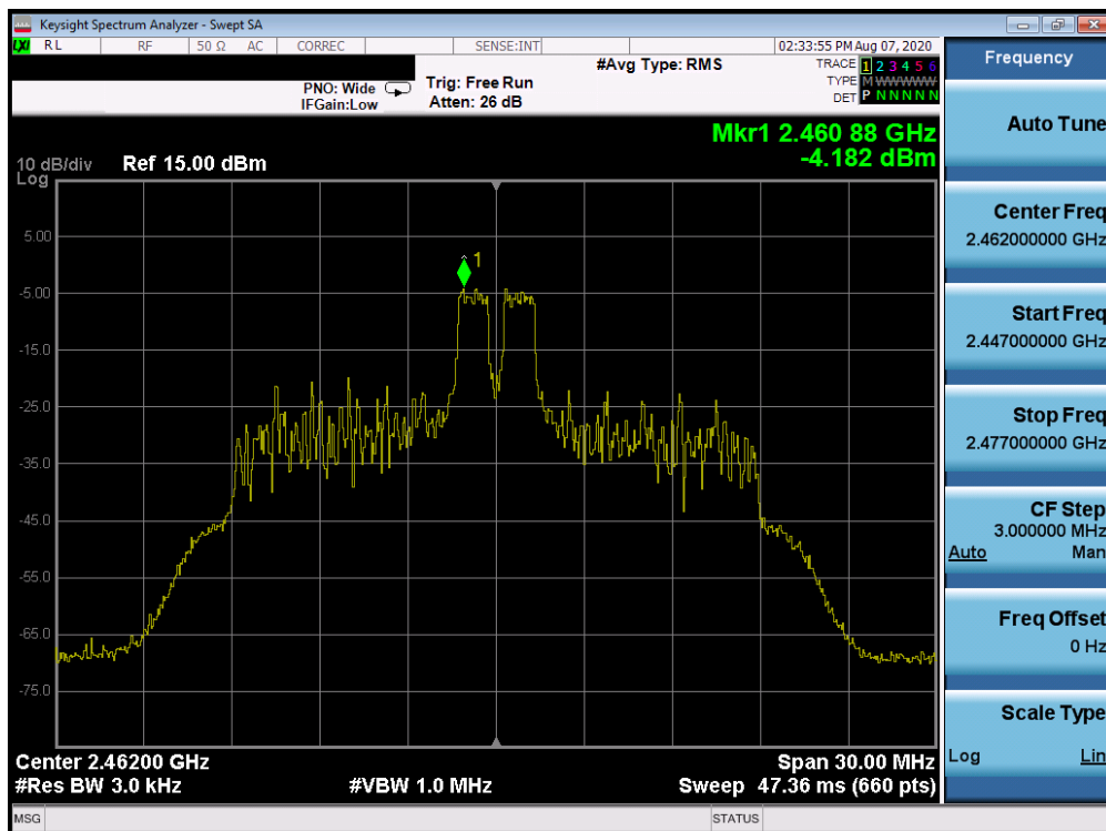
Plot 7-64. Power Spectral Density Plot CDD Antenna 1a (802.11ax OFDMA – RU26 Index 4 – Ch. 11)
