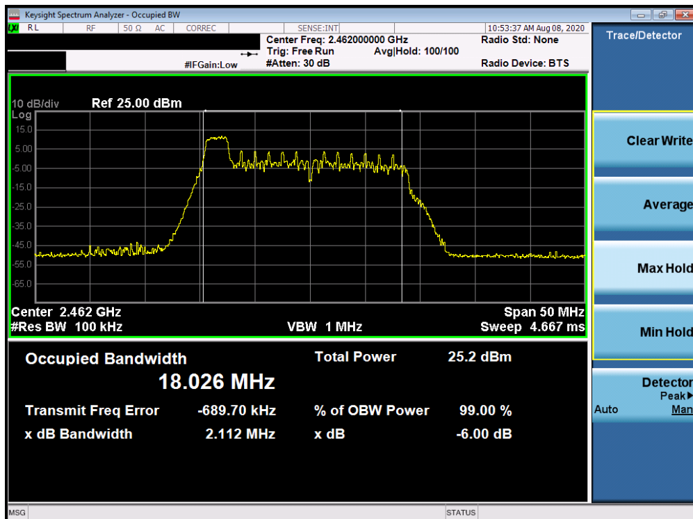
Plot 7-7. 6dB Bandwidth Plot Antenna 3a (802.11ax OFDMA – RU26 Index 0 – Ch. 11)
