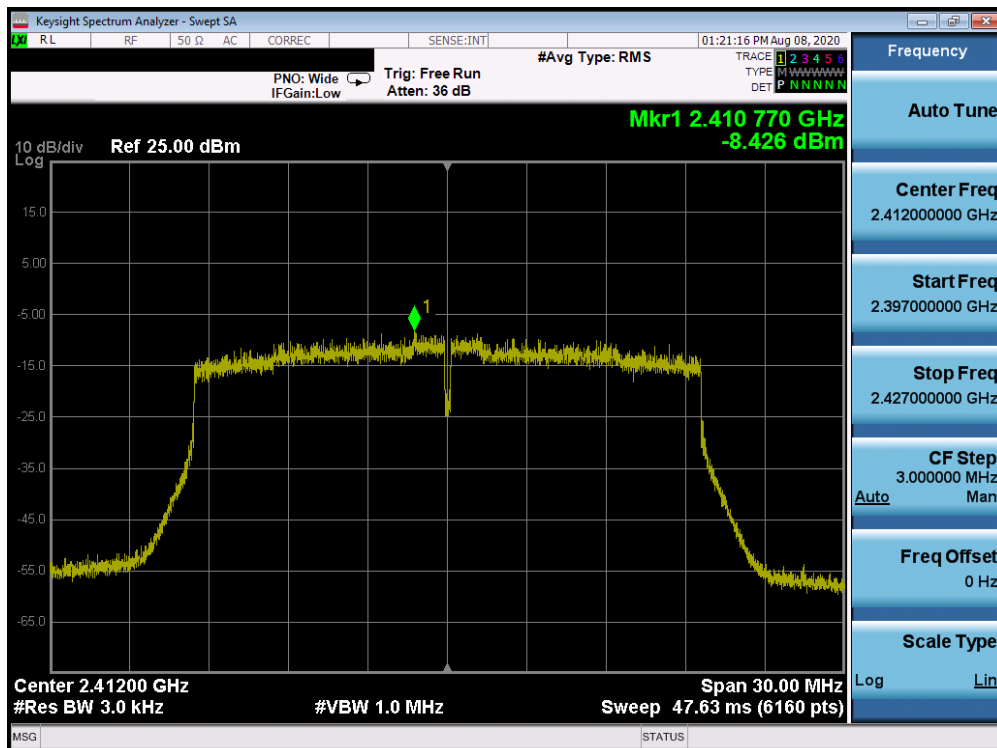
Plot 7-46. Power Spectral Density Plot Antenna 1a (802.11ax OFDMA – RU242 – Ch. 1)
