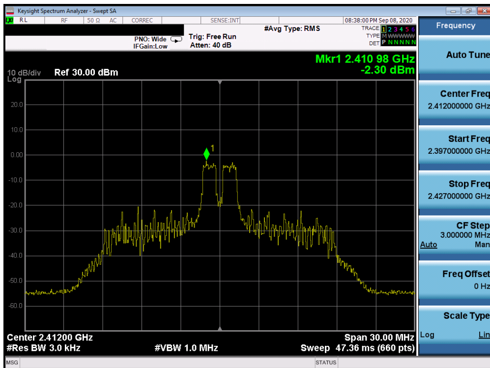
Plot 7-38. Power Spectral Density Plot Antenna 1a (802.11ax OFDMA – RU26 Index 4 – Ch. 1)
