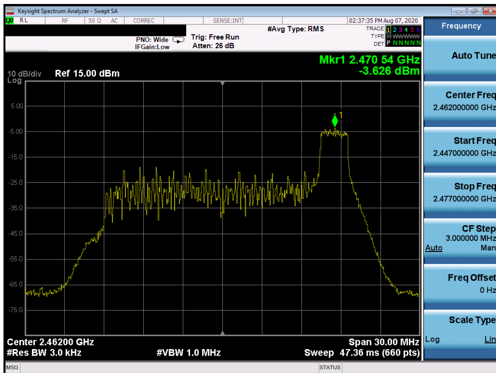
Plot 7-66. Power Spectral Density Plot CDD Antenna 1a (802.11ax OFDMA – RU26 Index 8 – Ch. 11)
