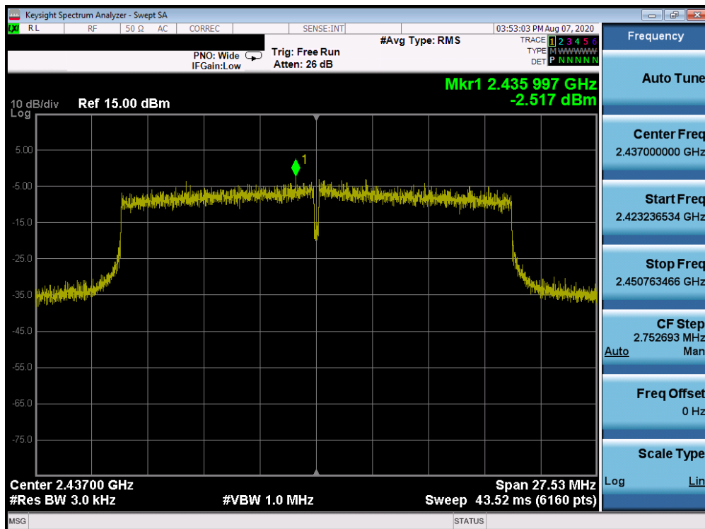
Plot 7-70. Power Spectral Density Plot CDD Antenna 1a (802.11ax OFDMA – RU242 – Ch. 6)
