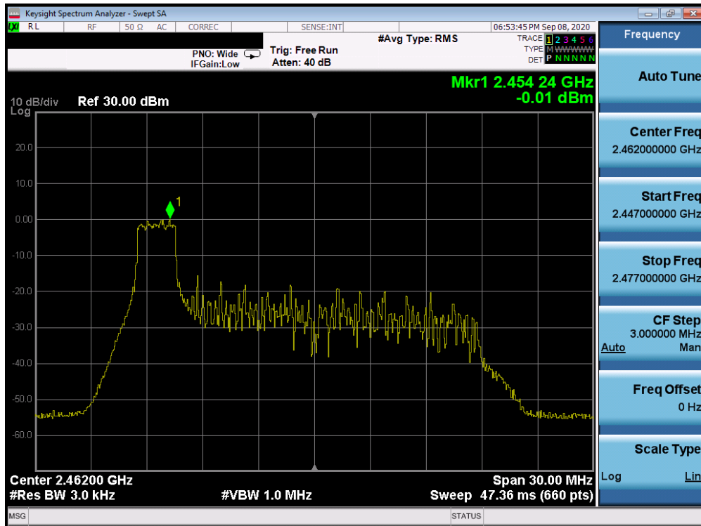
Plot 7-31. Power Spectral Density Plot Antenna 3a (802.11ax OFDMA – RU26 Index 0 – Ch. 11)
