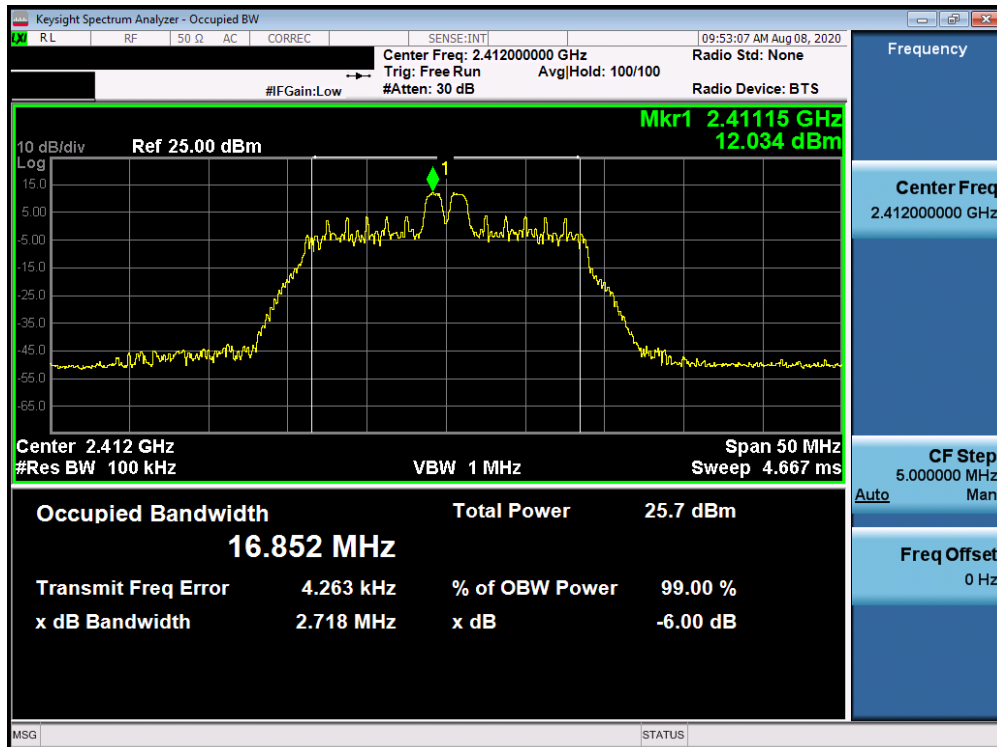
Plot 7-2. 6dB Bandwidth Plot Antenna 3a (802.11ax OFDMA – RU26 Index 4 – Ch. 1)
