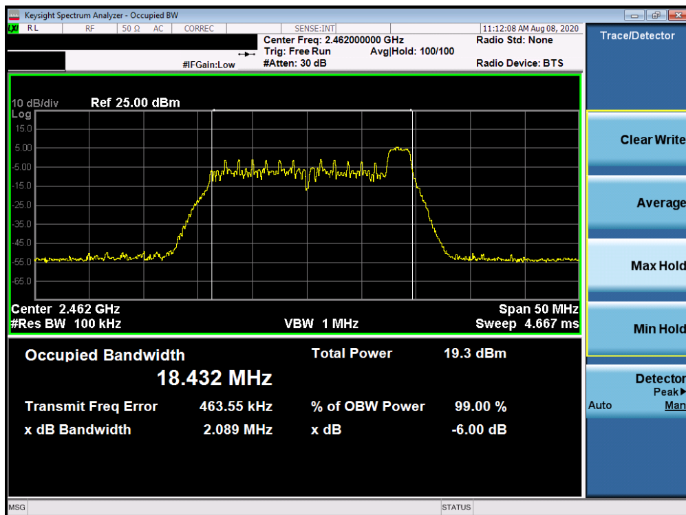
Plot 7-9. 6dB Bandwidth Plot Antenna 3a (802.11ax OFDMA – RU26 Index 8 – Ch. 11)
