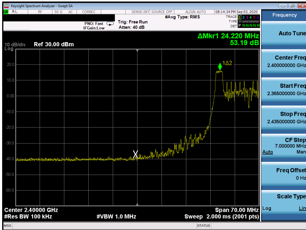
Plot 7-77. Band Edge Antenna 3a (802.11ax OFDMA – RU26 Index 0 – Ch. 5)
