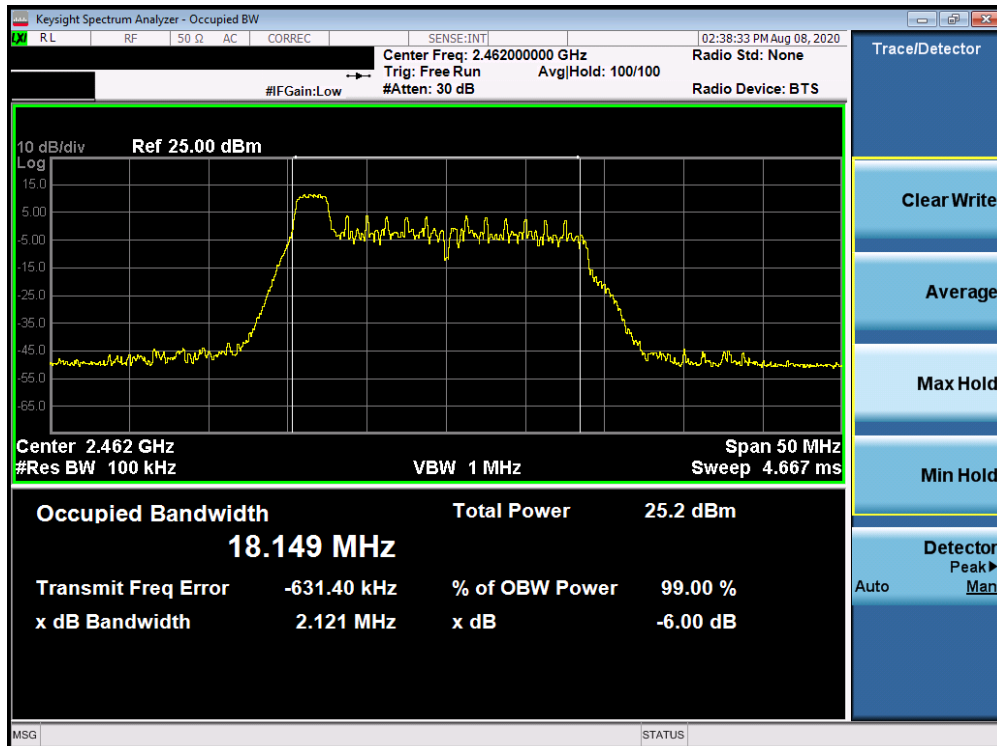
Plot 7-19. 6dB Bandwidth Plot Antenna 1a (802.11ax OFDMA – RU26 Index 0 – Ch. 11)
