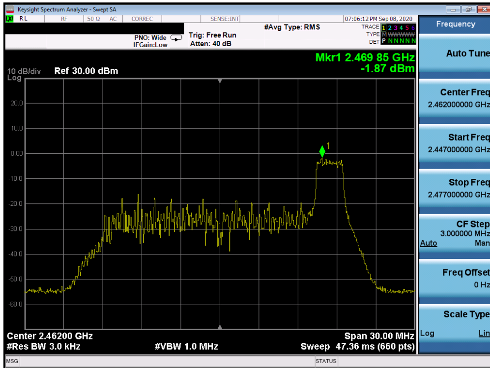
Plot 7-33. Power Spectral Density Plot Antenna 3a (802.11ax OFDMA – RU26 Index 8 – Ch. 11)
