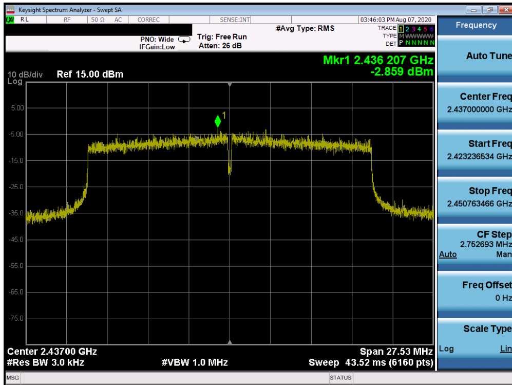
Plot 7-69. Power Spectral Density Plot CDD Antenna 3a (802.11ax OFDMA – RU242 – Ch. 6)
