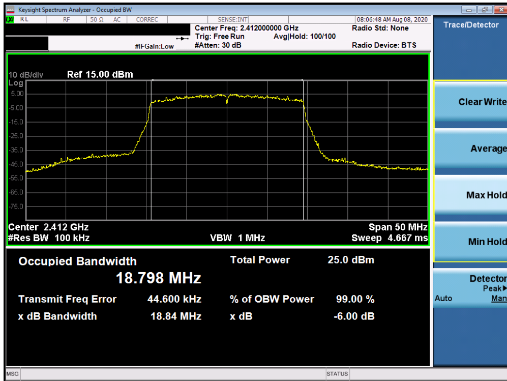
Plot 7-10. 6dB Bandwidth Plot Antenna 3a (802.11ax OFDMA – RU242 – Ch. 1)
