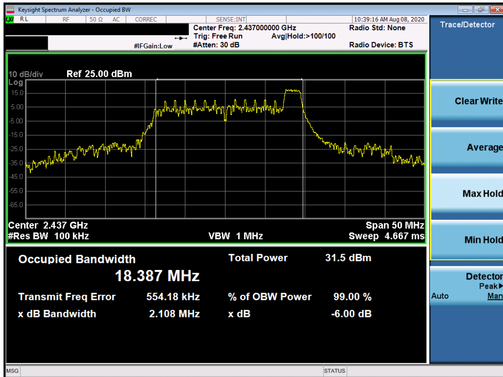
Plot 7-6. 6dB Bandwidth Plot Antenna 3a (802.11ax OFDMA – RU26 Index 8 – Ch. 6)
