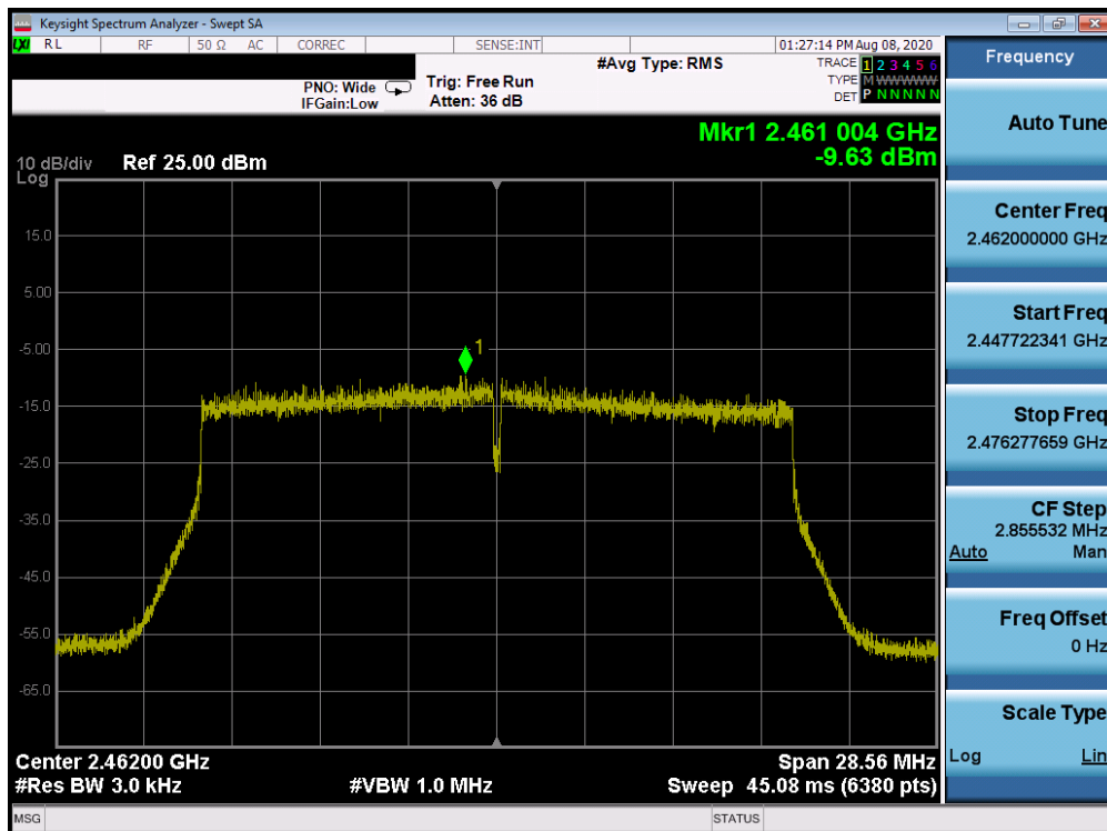
Plot 7-48. Power Spectral Density Plot Antenna 1a (802.11ax OFDMA – RU242 – Ch. 11)
