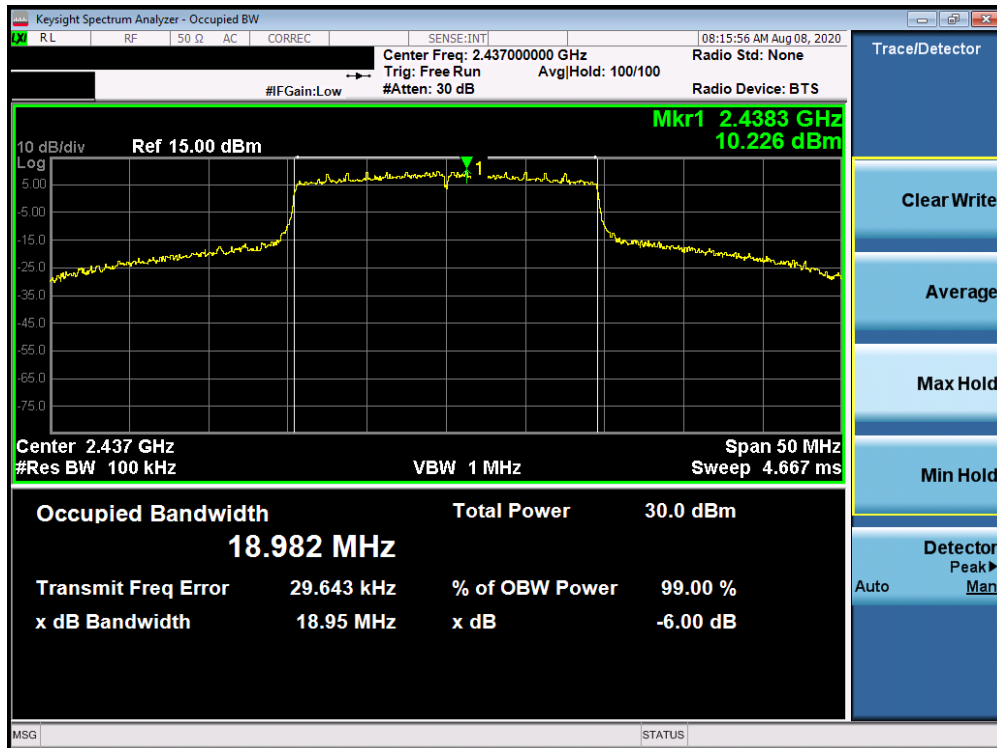
Plot 7-11. 6dB Bandwidth Plot Antenna 3a (802.11ax OFDMA – RU242 – Ch. 6)
