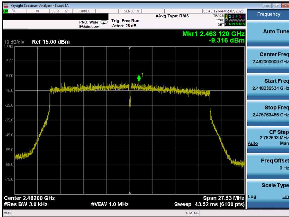
Plot 7-71. Power Spectral Density Plot CDD Antenna 3a (802.11ax OFDMA – RU242 – Ch. 11)
