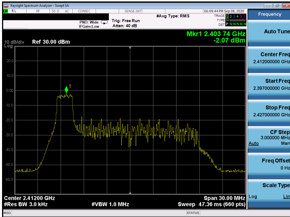
Plot 7-25. Power Spectral Density Plot Antenna 3a (802.11ax OFDMA – RU26 Index 0 – Ch. 1)
