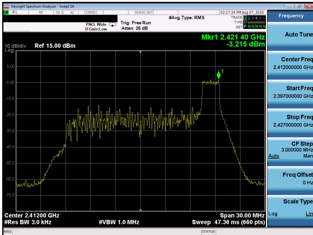
Plot 7-54. Power Spectral Density Plot CDD Antenna 1a (802.11ax OFDMA – RU26 Index 8 – Ch. 1)
