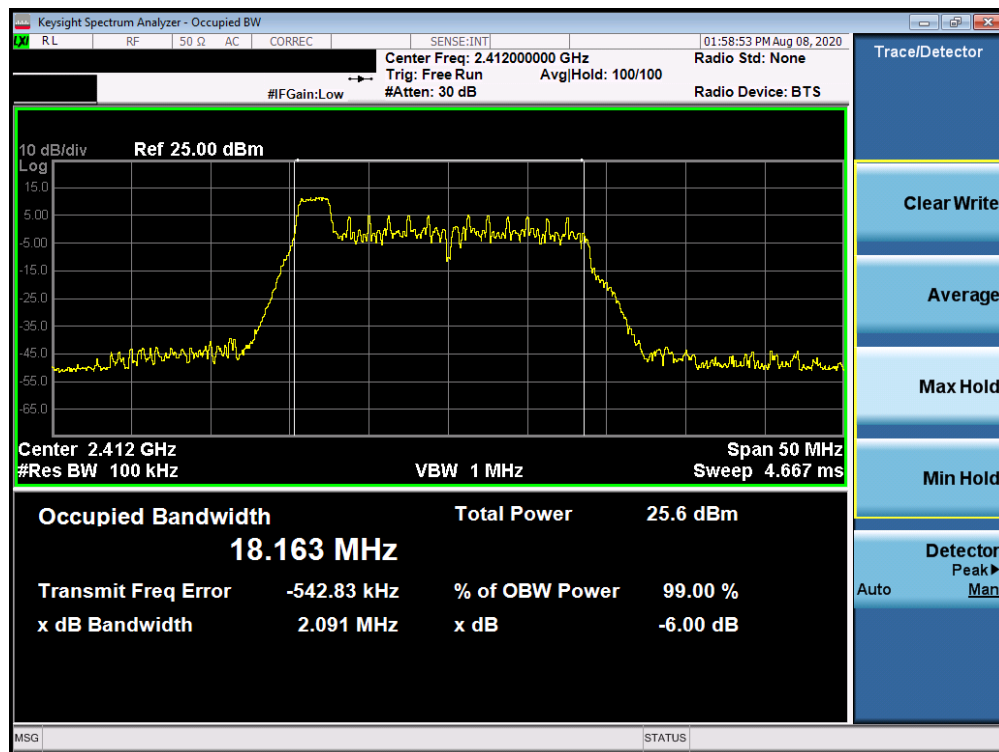
Plot 7-13. 6dB Bandwidth Plot Antenna 1a (802.11ax OFDMA – RU26 Index 0 – Ch. 1)
