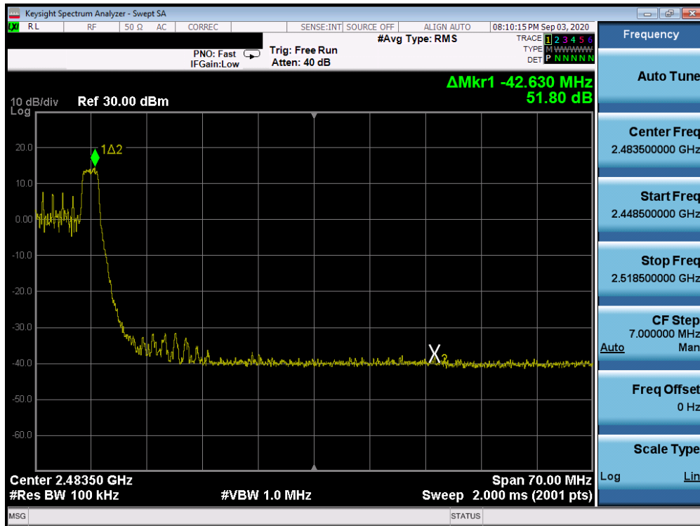
Plot 7-79. Band Edge Antenna 3a (802.11ax OFDMA – RU26 Index 8 – Ch. 8)
