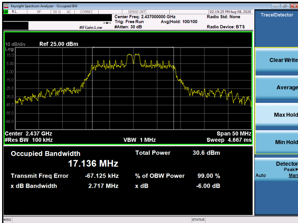
Plot 7-17. 6dB Bandwidth Plot Antenna 1a (802.11ax OFDMA – RU26 Index 4 – Ch. 6)
