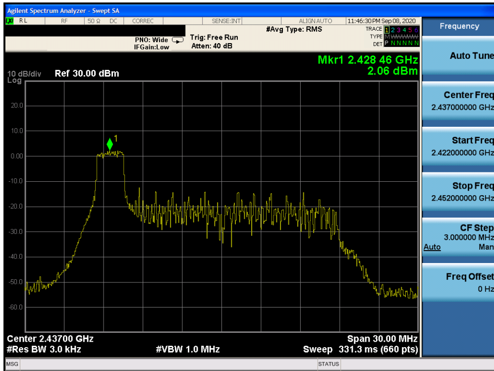
Plot 7-55. Power Spectral Density Plot CDD Antenna 3a (802.11ax OFDMA – RU26 Index 0 – Ch. 6)
