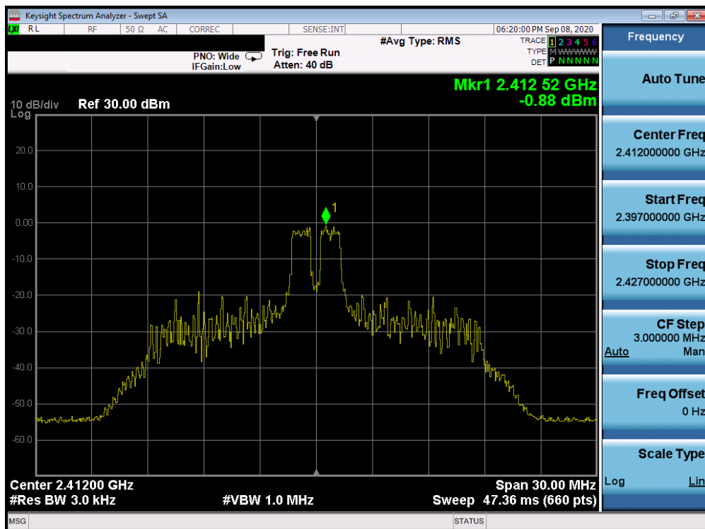
Plot 7-26. Power Spectral Density Plot Antenna 3a (802.11ax OFDMA – RU26 Index 4 – Ch. 1)
