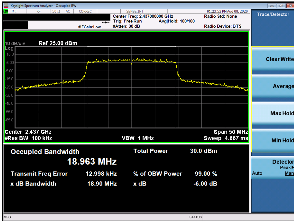
Plot 7-23. 6dB Bandwidth Plot Antenna 1a (802.11ax OFDMA – RU242 – Ch. 6)
