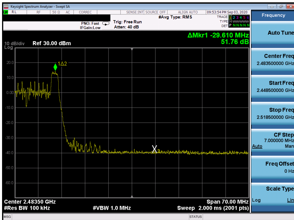
Plot 7-80. Band Edge Antenna 3a (802.11ax OFDMA – RU26 Index 8 – Ch. 9)
