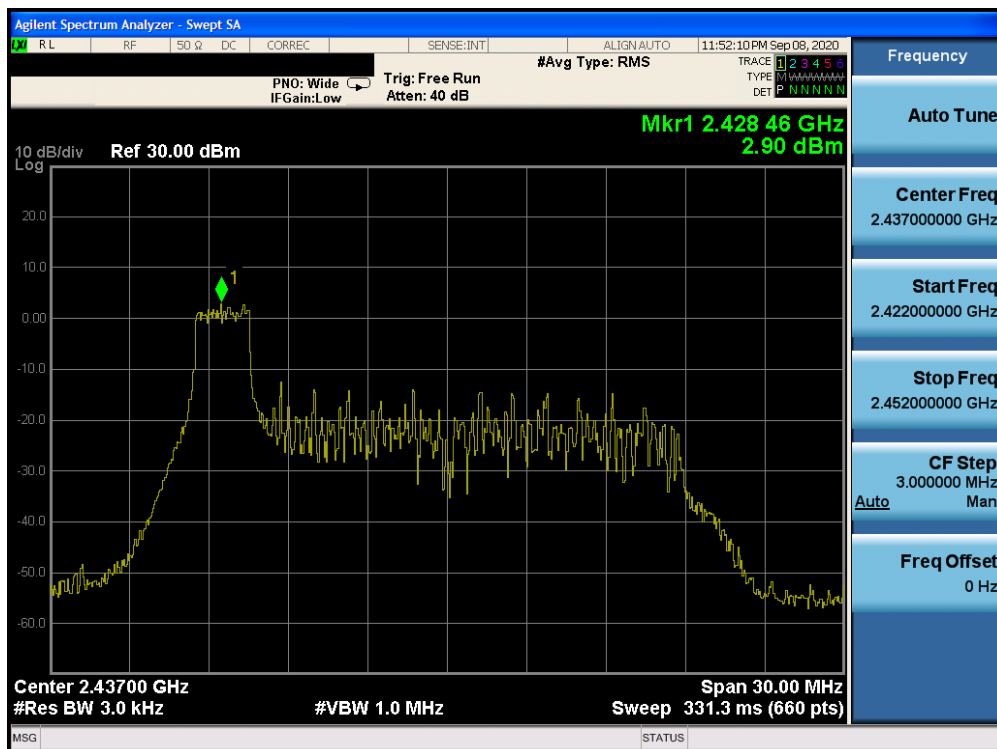
Plot 7-56. Power Spectral Density Plot CDD Antenna 1a (802.11ax OFDMA – RU26 Index 0 – Ch. 6)
