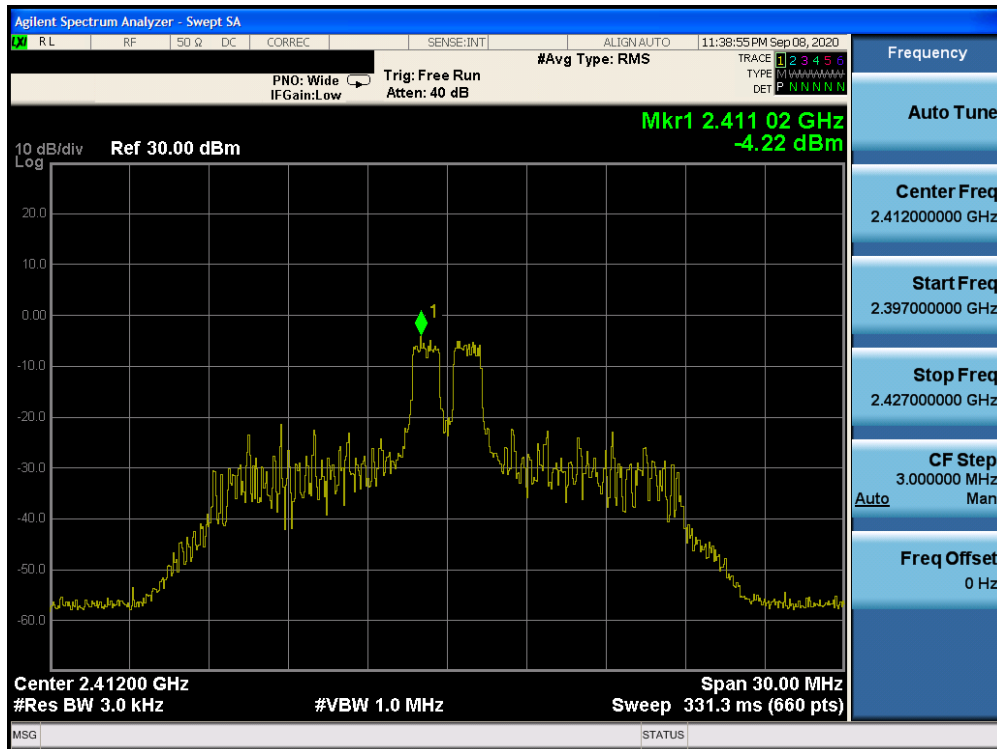
Plot 7-51. Power Spectral Density Plot CDD Antenna 3a (802.11ax OFDMA – RU26 Index 4 – Ch. 1)
