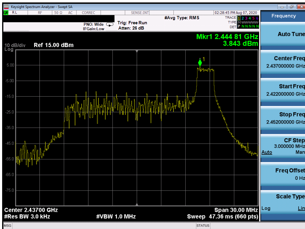
Plot 7-60. Power Spectral Density Plot CDD Antenna 1a (802.11ax OFDMA – RU26 Index 8 – Ch. 6)
