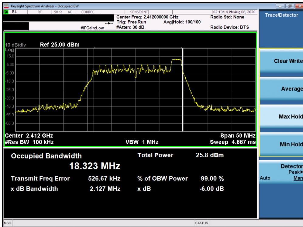
Plot 7-15. 6dB Bandwidth Plot Antenna 1a (802.11ax OFDMA – RU26 Index 8 – Ch. 1)
