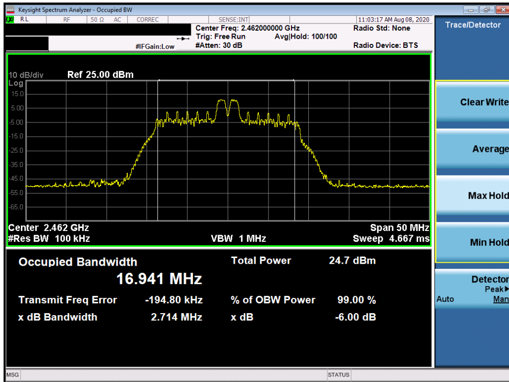
Plot 7-8. 6dB Bandwidth Plot Antenna 3a (802.11ax OFDMA – RU26 Index 4 – Ch. 11)
