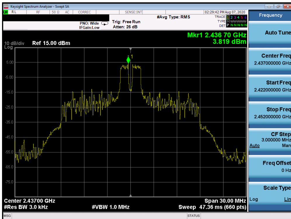
Plot 7-58. Power Spectral Density Plot CDD Antenna 1a (802.11ax OFDMA – RU26 Index 4 – Ch. 6)
