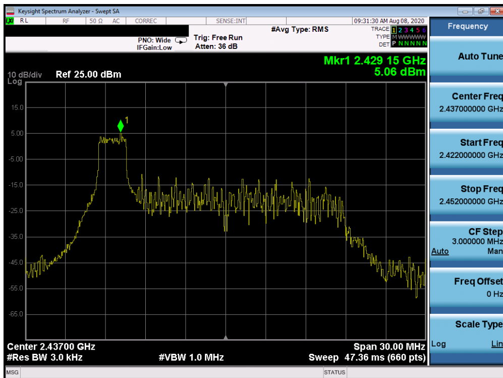
Plot 7-28. Power Spectral Density Plot Antenna 3a (802.11ax OFDMA – RU26 Index 0 – Ch. 6)
