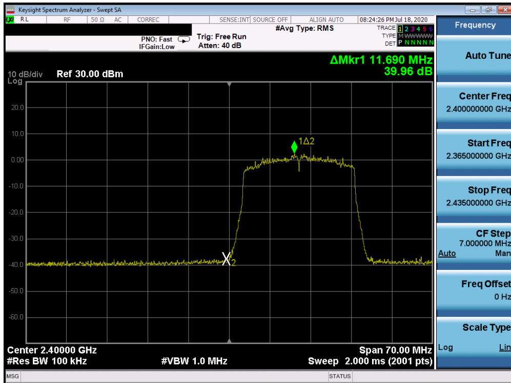
Plot 7-84. Band Edge Antenna 3a (802.11ax OFDMA – RU242 – Ch. 1)
