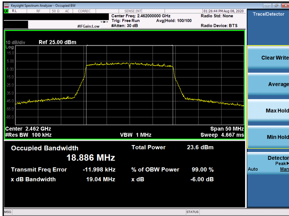
Plot 7-24. 6dB Bandwidth Plot Antenna 1a (802.11ax OFDMA – RU242 – Ch. 11)
