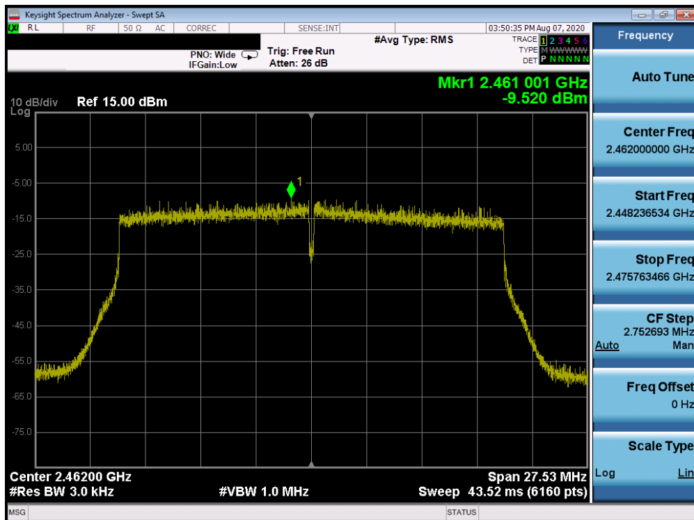
Plot 7-72. Power Spectral Density Plot CDD Antenna 1a (802.11ax OFDMA – RU242 – Ch. 11)
