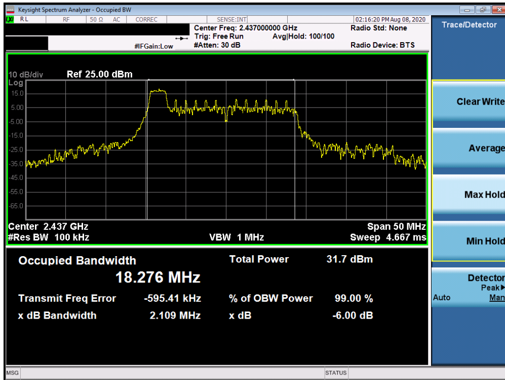
Plot 7-16. 6dB Bandwidth Plot Antenna 1a (802.11ax OFDMA – RU26 Index 0 – Ch. 6)
