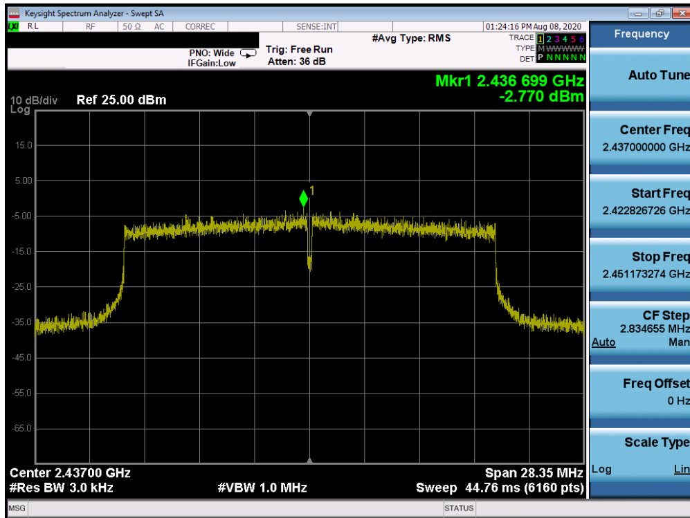
Plot 7-47. Power Spectral Density Plot Antenna 1a (802.11ax OFDMA – RU242 – Ch. 6)
