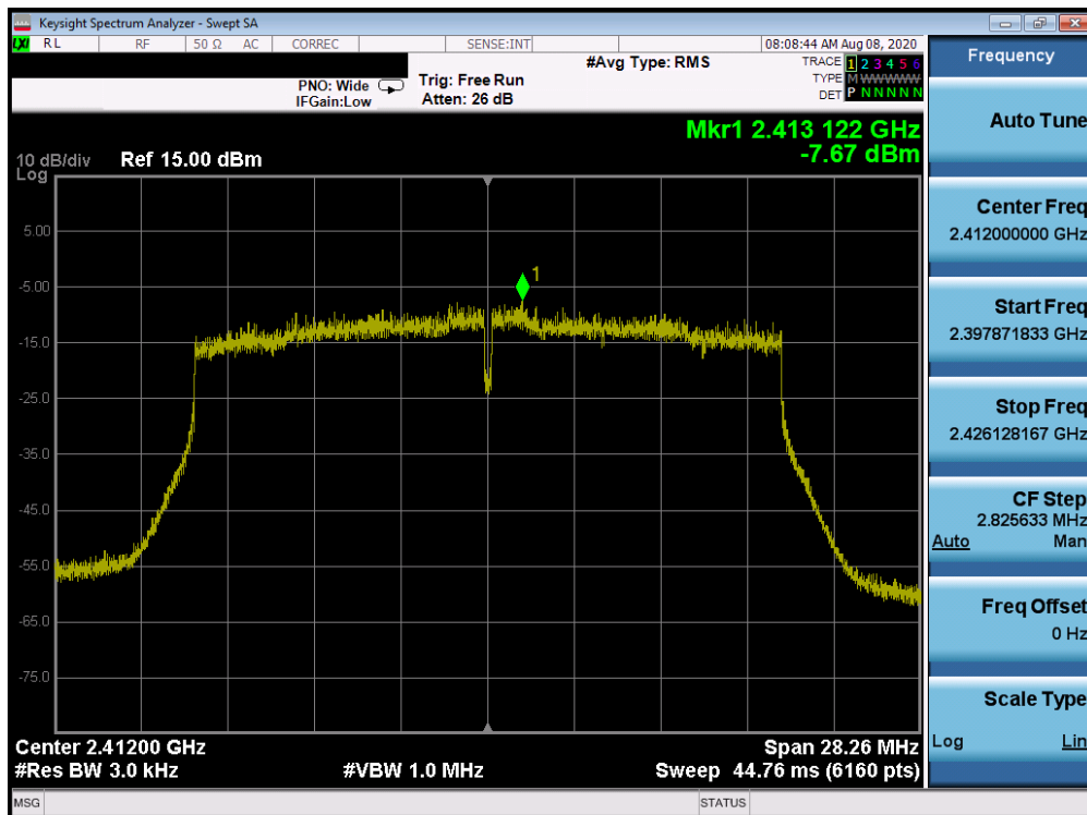
Plot 7-34. Power Spectral Density Plot Antenna 3a (802.11ax OFDMA – RU242 – Ch. 1)
