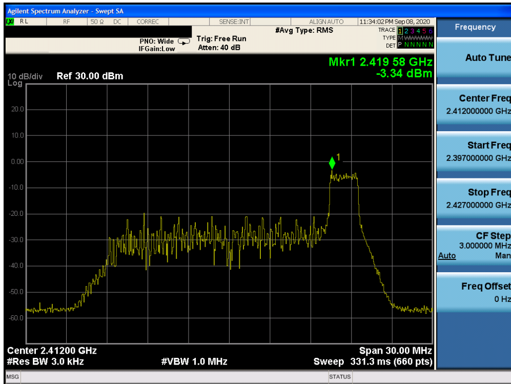
Plot 7-53. Power Spectral Density Plot CDD Antenna 3a (802.11ax OFDMA – RU26 Index 8 – Ch. 1)
