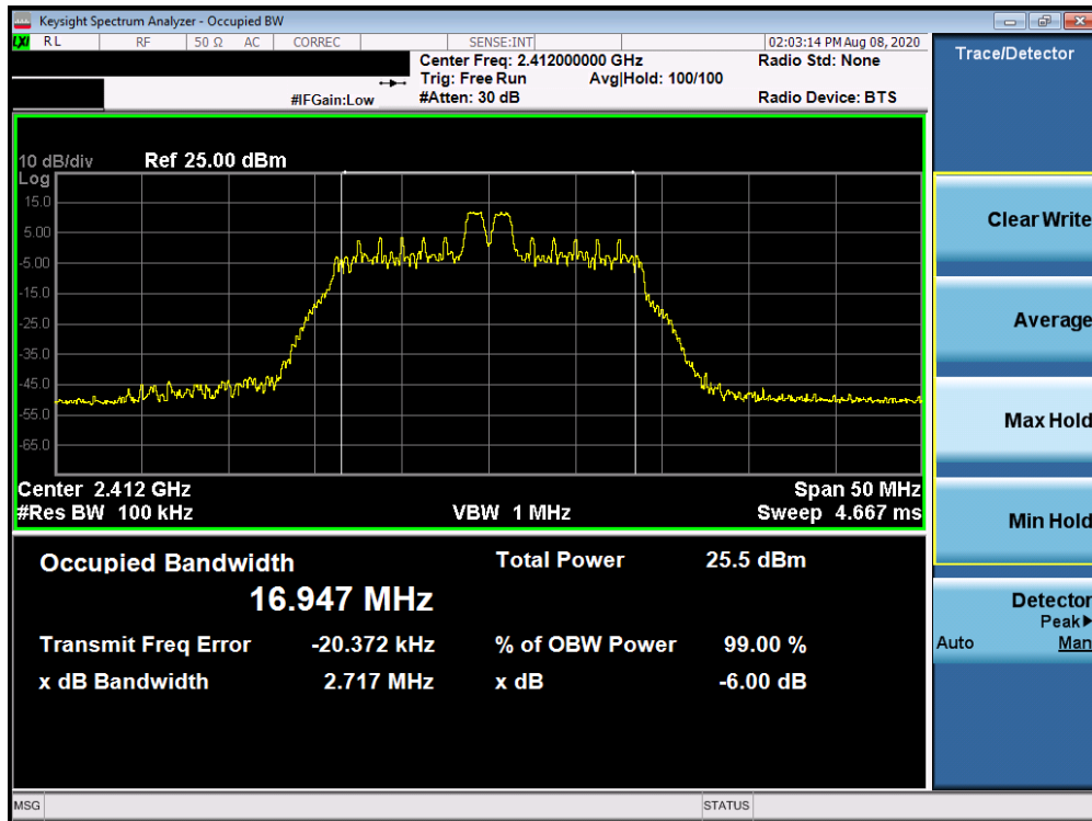
Plot 7-14. 6dB Bandwidth Plot Antenna 1a (802.11ax OFDMA – RU26 Index 4 – Ch. 1)
