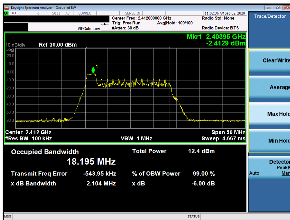
Plot 7-1. 6dB Bandwidth Plot Antenna 3a (802.11ax OFDMA – RU26 Index 0 – Ch. 1)
