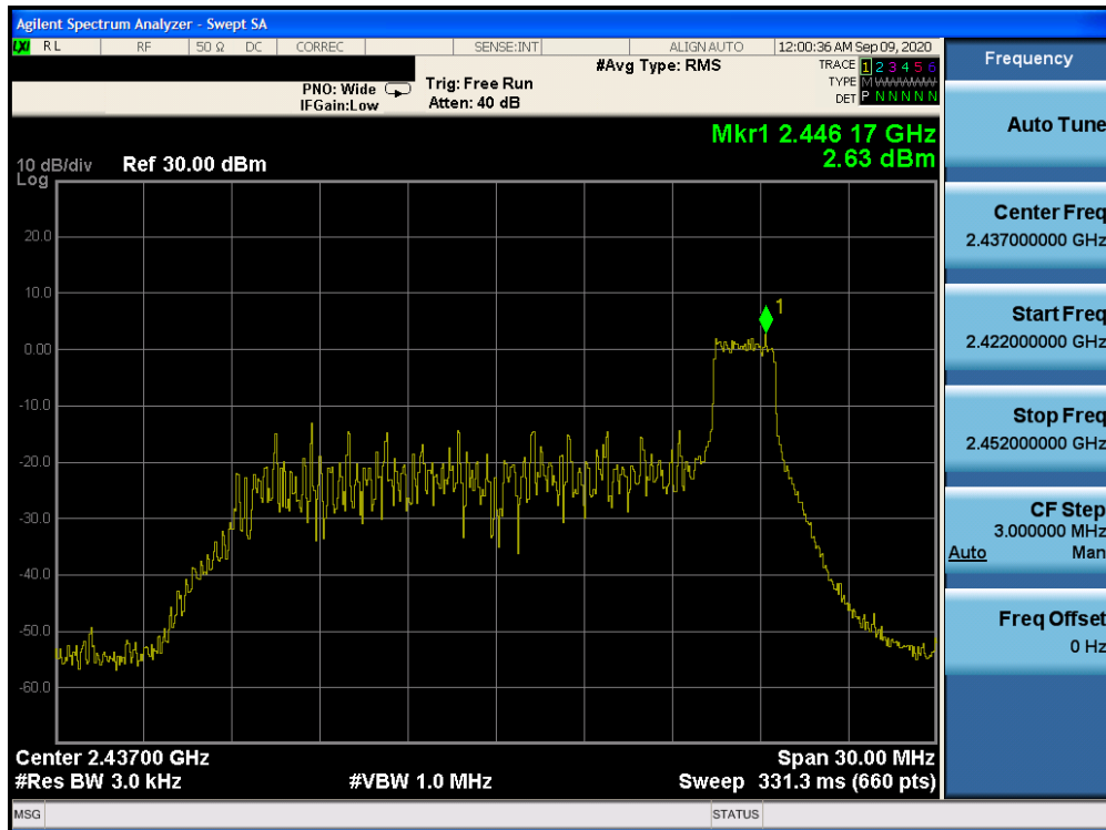
Plot 7-59. Power Spectral Density Plot CDD Antenna 3a (802.11ax OFDMA – RU26 Index 8 – Ch. 6)
