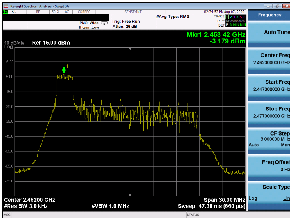
Plot 7-62. Power Spectral Density Plot CDD Antenna 1a (802.11ax OFDMA – RU26 Index 0 – Ch. 11)
