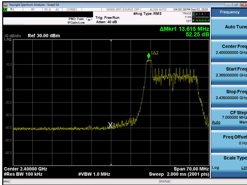
Plot 7-75. Band Edge Antenna 3a (802.11ax OFDMA – RU26 Index 0 – Ch. 3)
