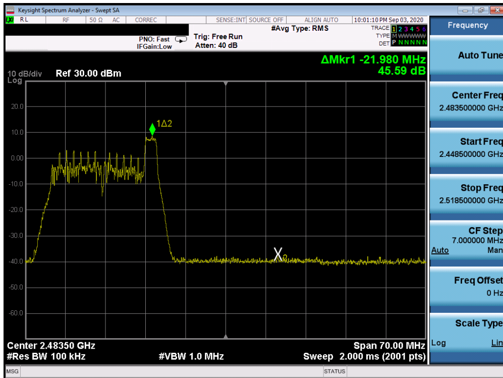
Plot 7-82. Band Edge Antenna 3a (802.11ax OFDMA – RU26 Index 8 – Ch. 11)
