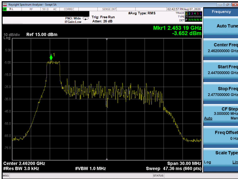
Plot 7-61. Power Spectral Density Plot CDD Antenna 3a (802.11ax OFDMA – RU26 Index 0 – Ch. 11)
