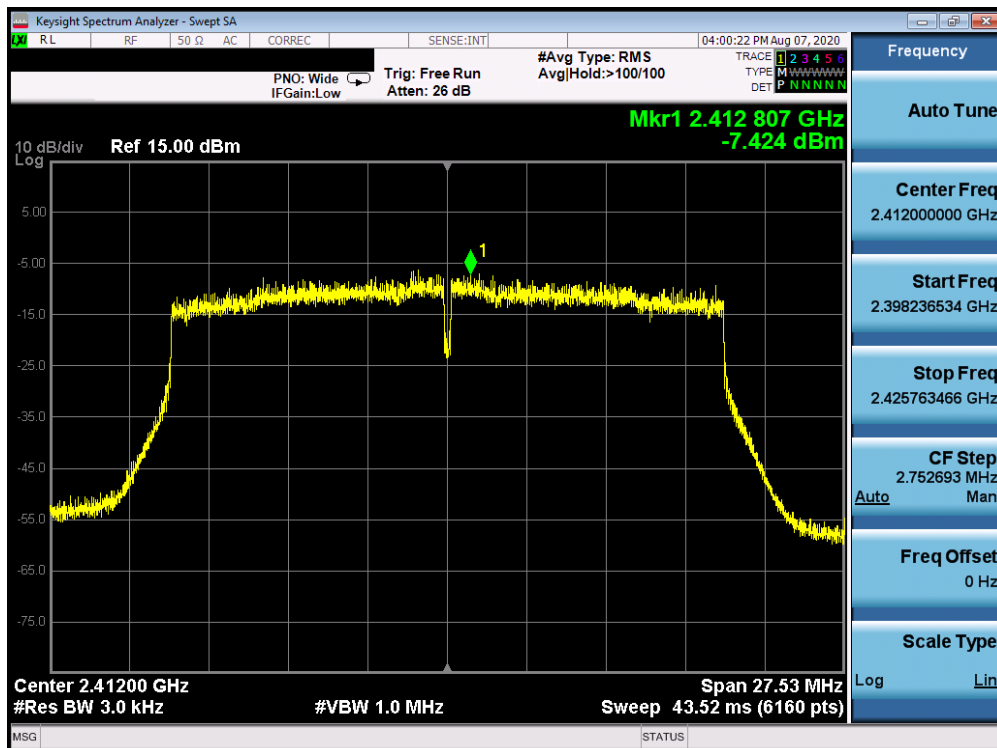
Plot 7-68. Power Spectral Density Plot CDD Antenna 1a (802.11ax OFDMA – RU242 – Ch. 1)
