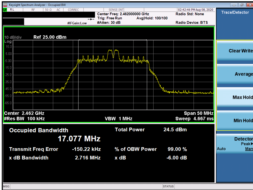
Plot 7-20. 6dB Bandwidth Plot Antenna 1a (802.11ax OFDMA – RU26 Index 4 – Ch. 11)
