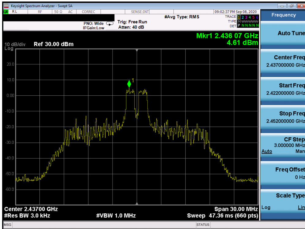
Plot 7-41. Power Spectral Density Plot Antenna 1a (802.11ax OFDMA – RU26 Index 4 – Ch. 6)
