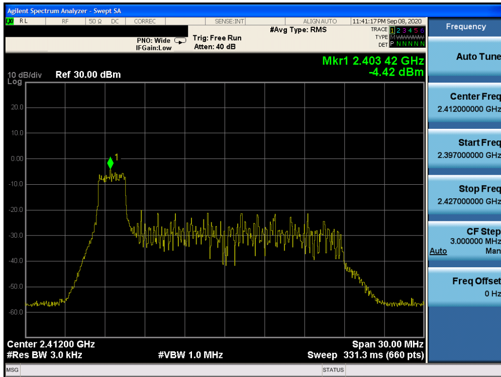
Plot 7-49. Power Spectral Density Plot CDD Antenna 3a (802.11ax OFDMA – RU26 Index 0 – Ch. 1)
