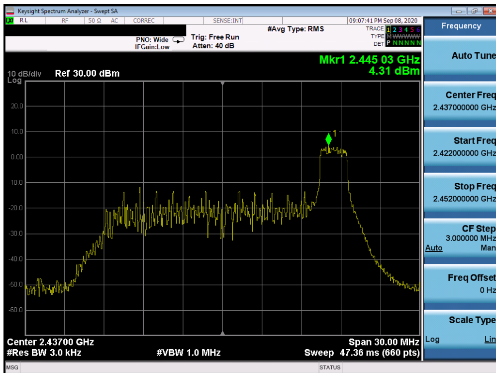
Plot 7-42. Power Spectral Density Plot Antenna 1a (802.11ax OFDMA – RU26 Index 8 – Ch. 6)
