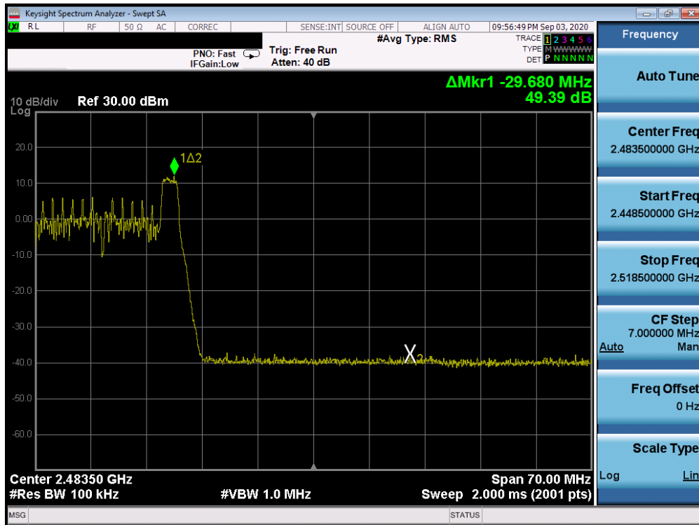
Plot 7-81. Band Edge Antenna 3a (802.11ax OFDMA – RU26 Index 8 – Ch. 10)
