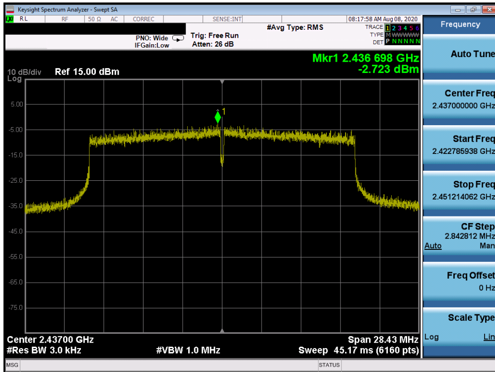
Plot 7-35. Power Spectral Density Plot Antenna 3a (802.11ax OFDMA – RU242 – Ch. 6)
