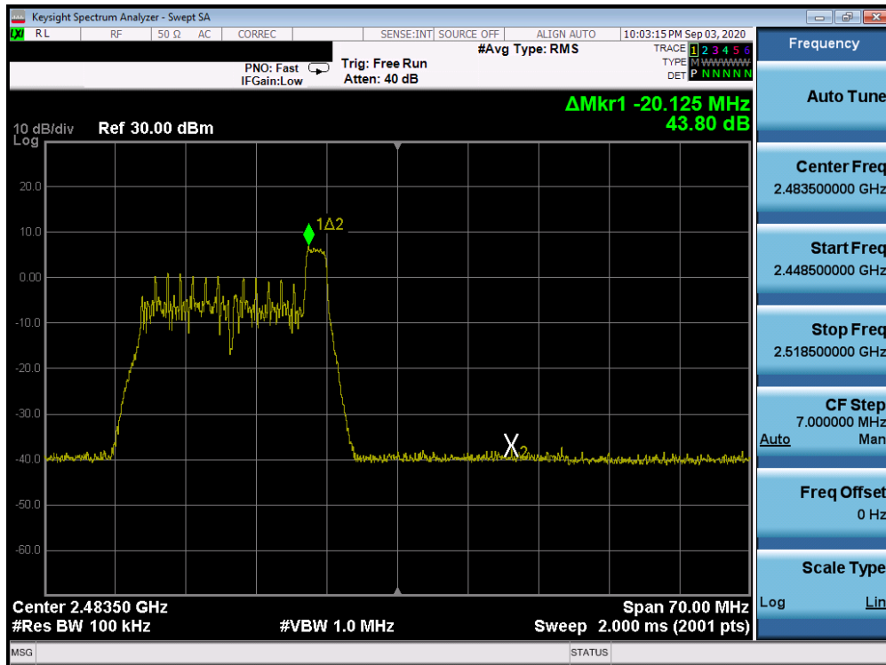
Plot 7-83. Band Edge Antenna 3a (802.11ax OFDMA – RU26 Index 8 – Ch. 12)
