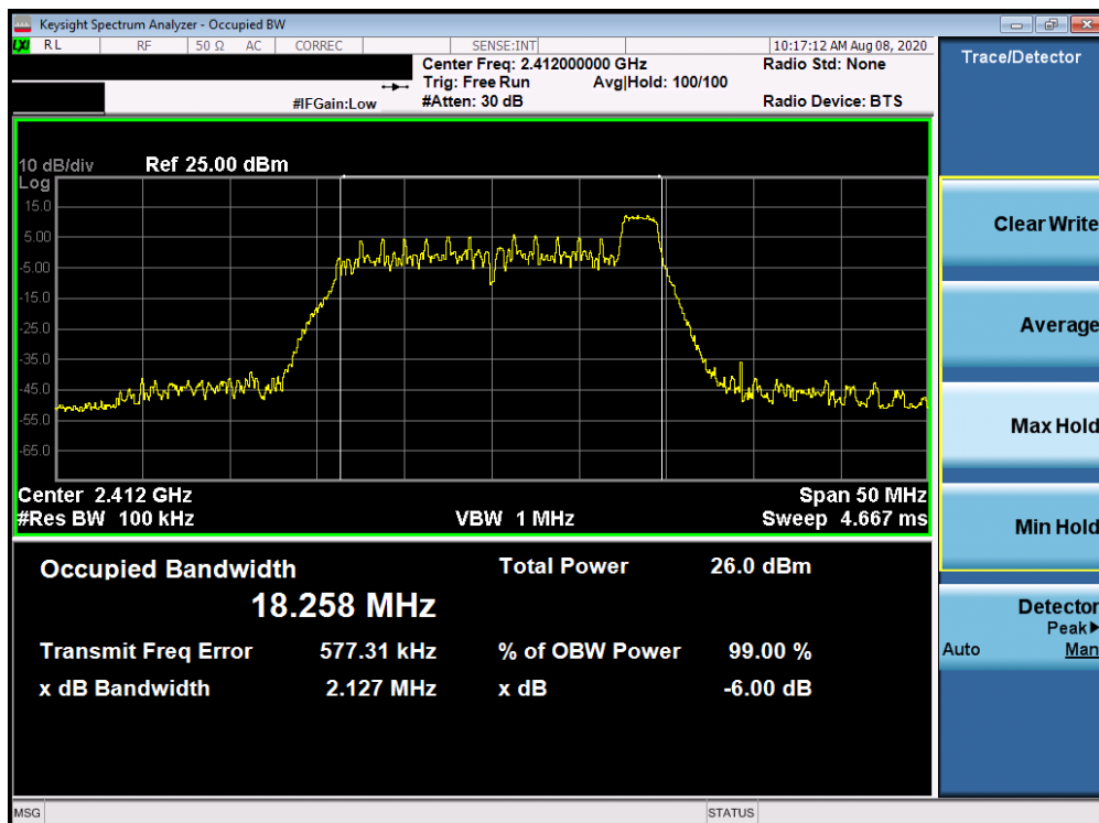
Plot 7-3. 6dB Bandwidth Plot Antenna 3a (802.11ax OFDMA – RU26 Index 8 – Ch. 1)
