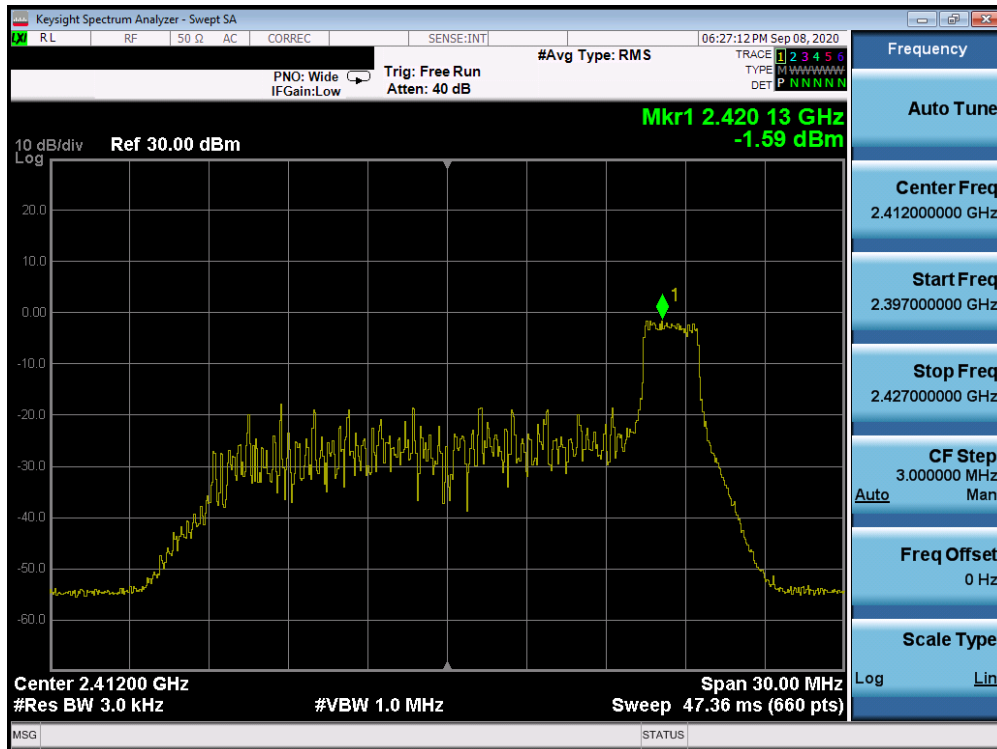
Plot 7-27. Power Spectral Density Plot Antenna 3a (802.11ax OFDMA – RU26 Index 8 – Ch. 1)
