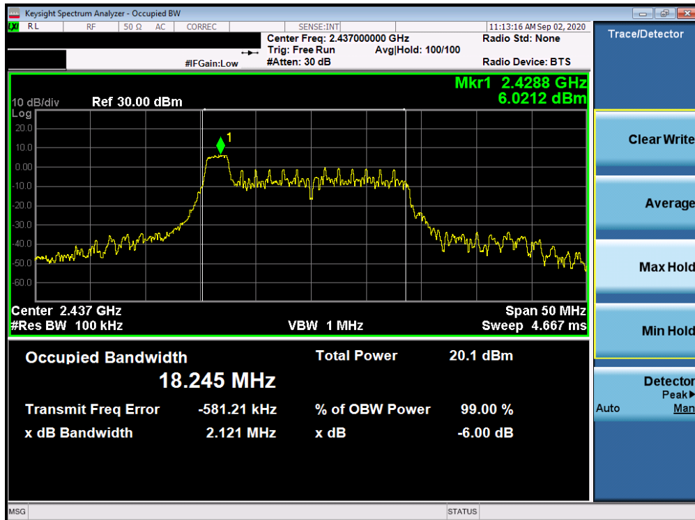
Plot 7-4. 6dB Bandwidth Plot Antenna 3a (802.11ax OFDMA – RU26 Index 0 – Ch. 6)
