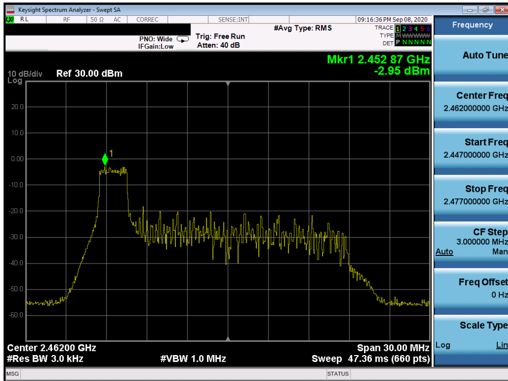
Plot 7-43. Power Spectral Density Plot Antenna 1a (802.11ax OFDMA – RU26 Index 0 – Ch. 11)
