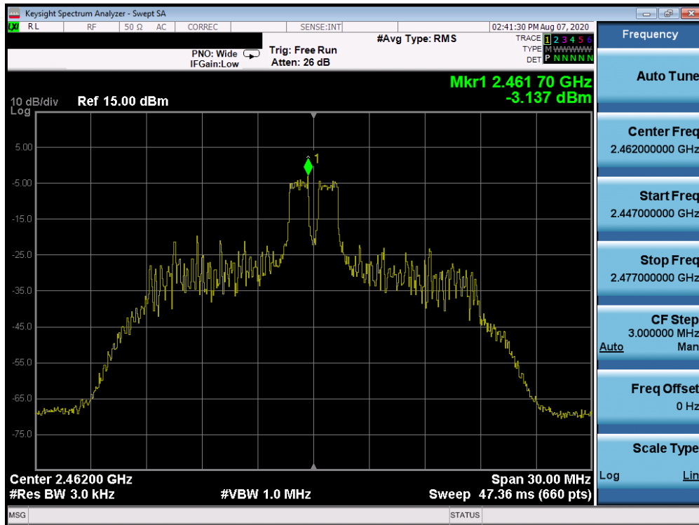
Plot 7-63. Power Spectral Density Plot CDD Antenna 3a (802.11ax OFDMA – RU26 Index 4 – Ch. 11)
