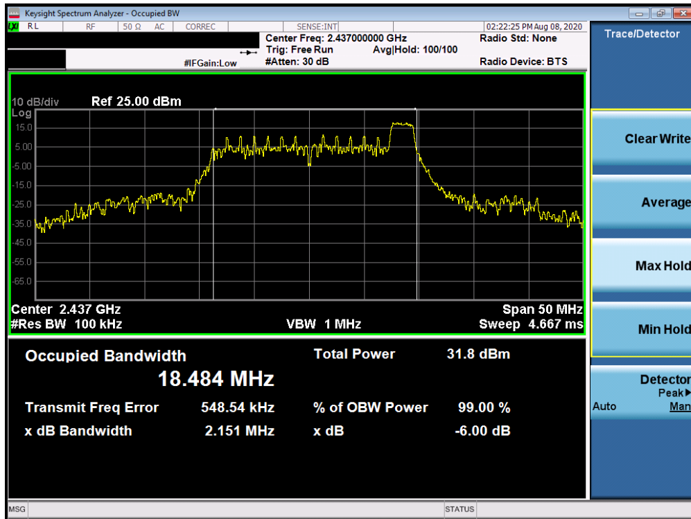
Plot 7-18. 6dB Bandwidth Plot Antenna 1a (802.11ax OFDMA – RU26 Index 8 – Ch. 6)
