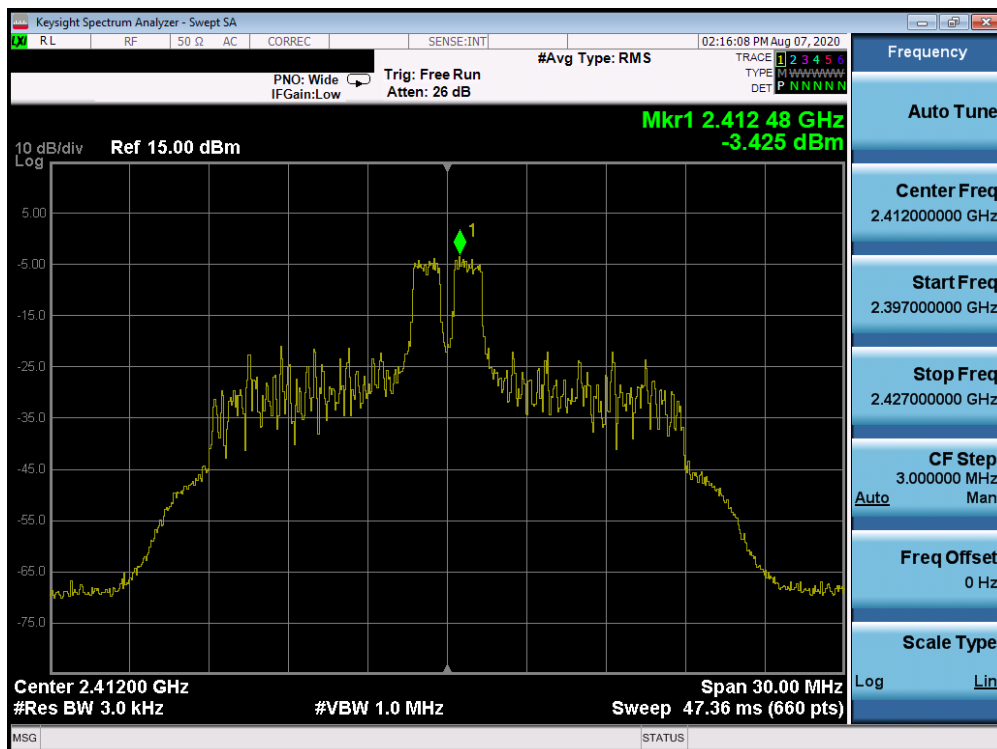
Plot 7-52. Power Spectral Density Plot CDD Antenna 1a (802.11ax OFDMA – RU26 Index 4 – Ch. 1)
