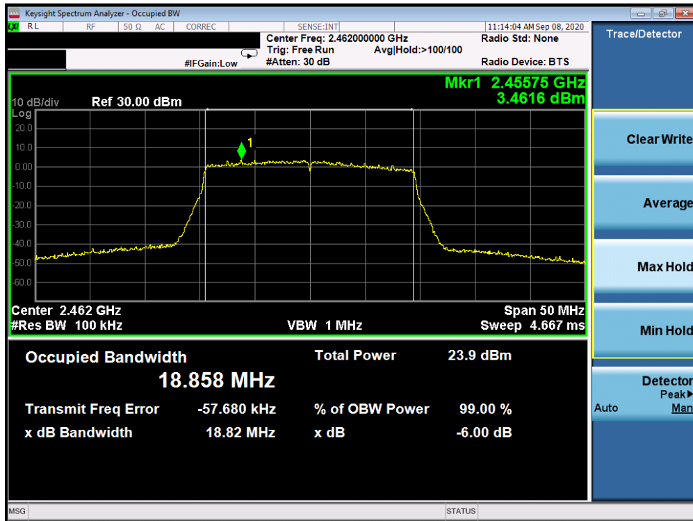
Plot 7-12. 6dB Bandwidth Plot Antenna 3a (802.11ax OFDMA – RU242 – Ch. 11)
