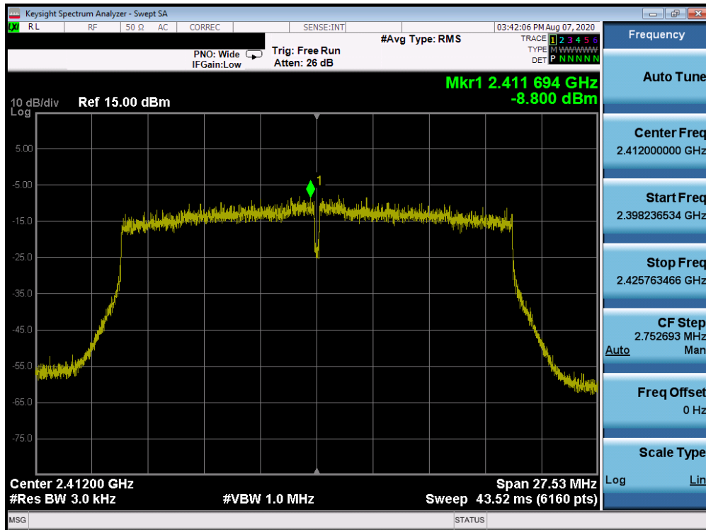
Plot 7-67. Power Spectral Density Plot CDD Antenna 3a (802.11ax OFDMA – RU242 – Ch. 1)
