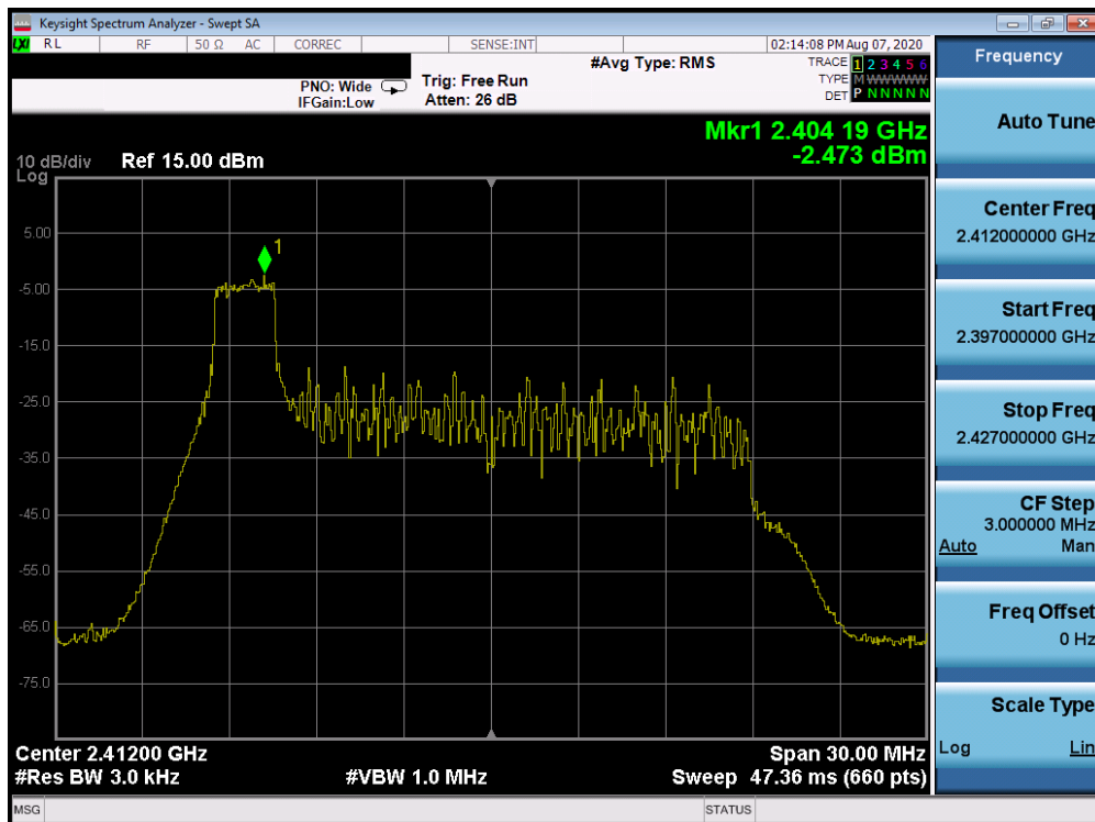
Plot 7-50. Power Spectral Density Plot CDD Antenna 1a (802.11ax OFDMA – RU26 Index 0 – Ch. 1)
