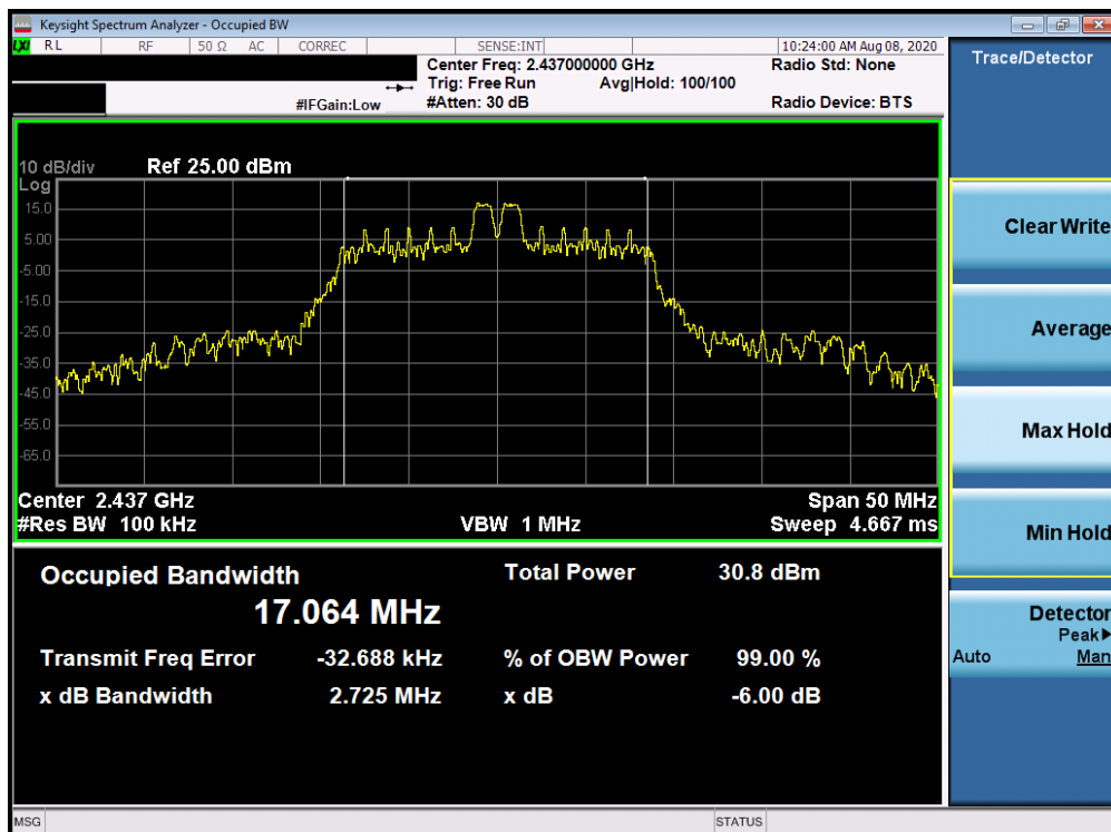
Plot 7-5. 6dB Bandwidth Plot Antenna 3a (802.11ax OFDMA – RU26 Index 4 – Ch. 6)
