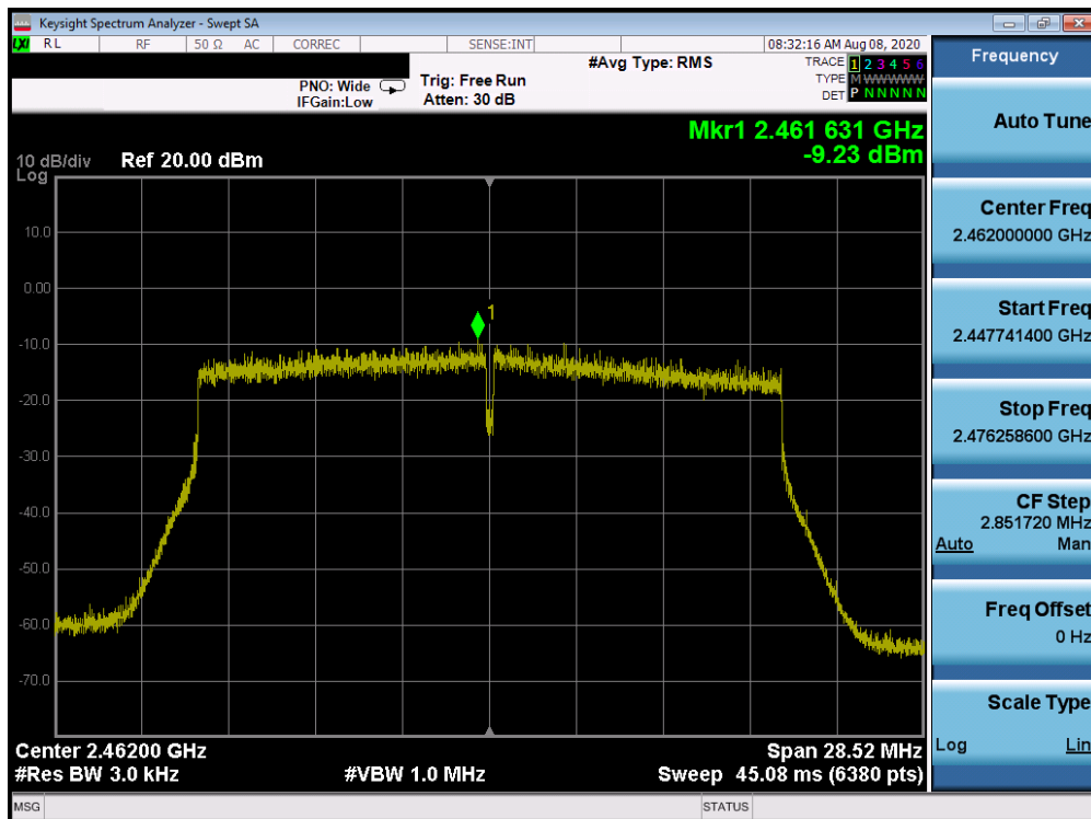
Plot 7-36. Power Spectral Density Plot Antenna 3a (802.11ax OFDMA – RU242 – Ch. 11)
