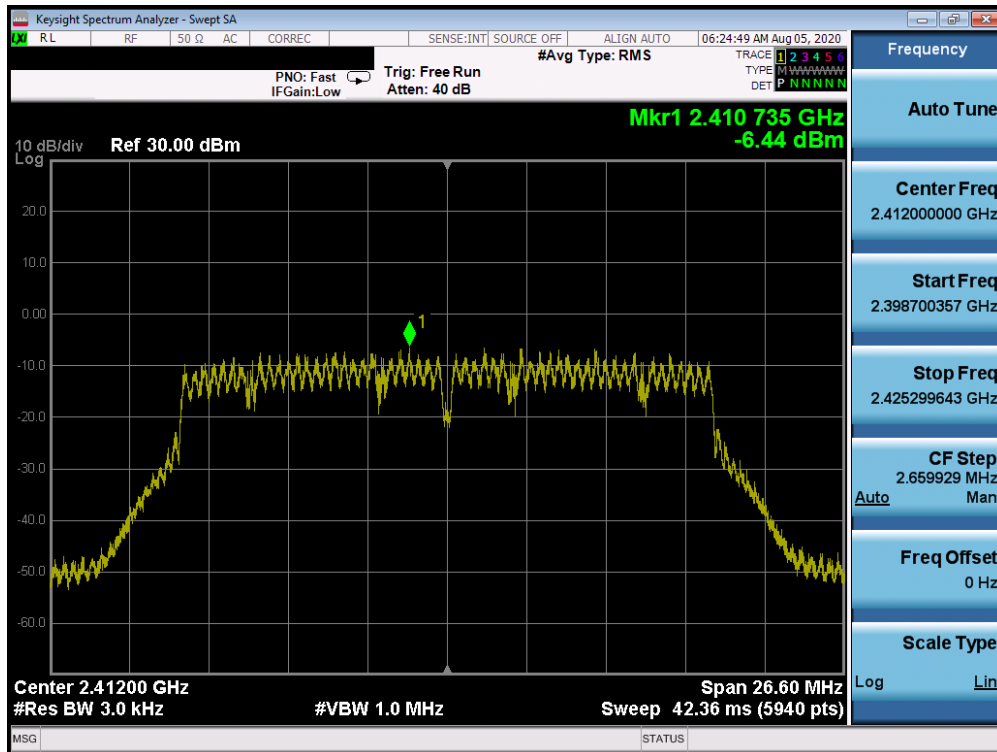
Plot 7-34. Power Spectral Density Plot ANT 1a (802.11n (2.4GHz) – Ch. 1)
