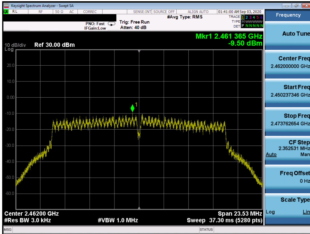
Plot 7-33. Power Spectral Density Plot ANT 1a (802.11g – Ch. 11)
