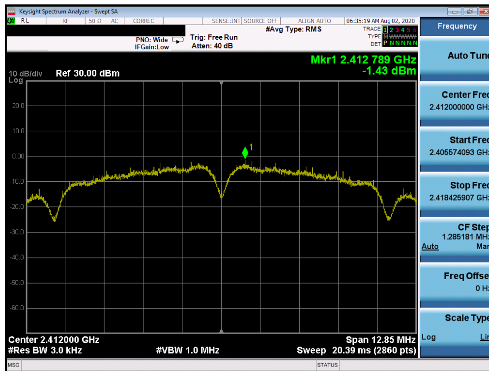
Plot 7-19. Power Spectral Density Plot ANT 3a (802.11b - Ch. 1)
