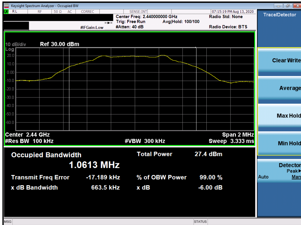
Plot 7-2. 6dB Bandwidth Plot Antenna 3a (Bluetooth (LE), 1Mbps, ePA – Ch. 19)
