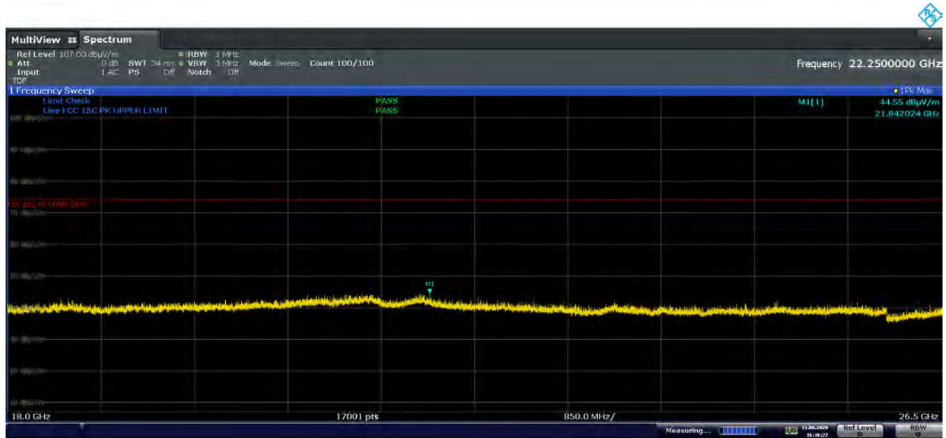
Plot 7-91. Radiated Spurious Emissions Above 18GHz TxBF (1Mbps, ePA – Ch.19, Pol. V)
