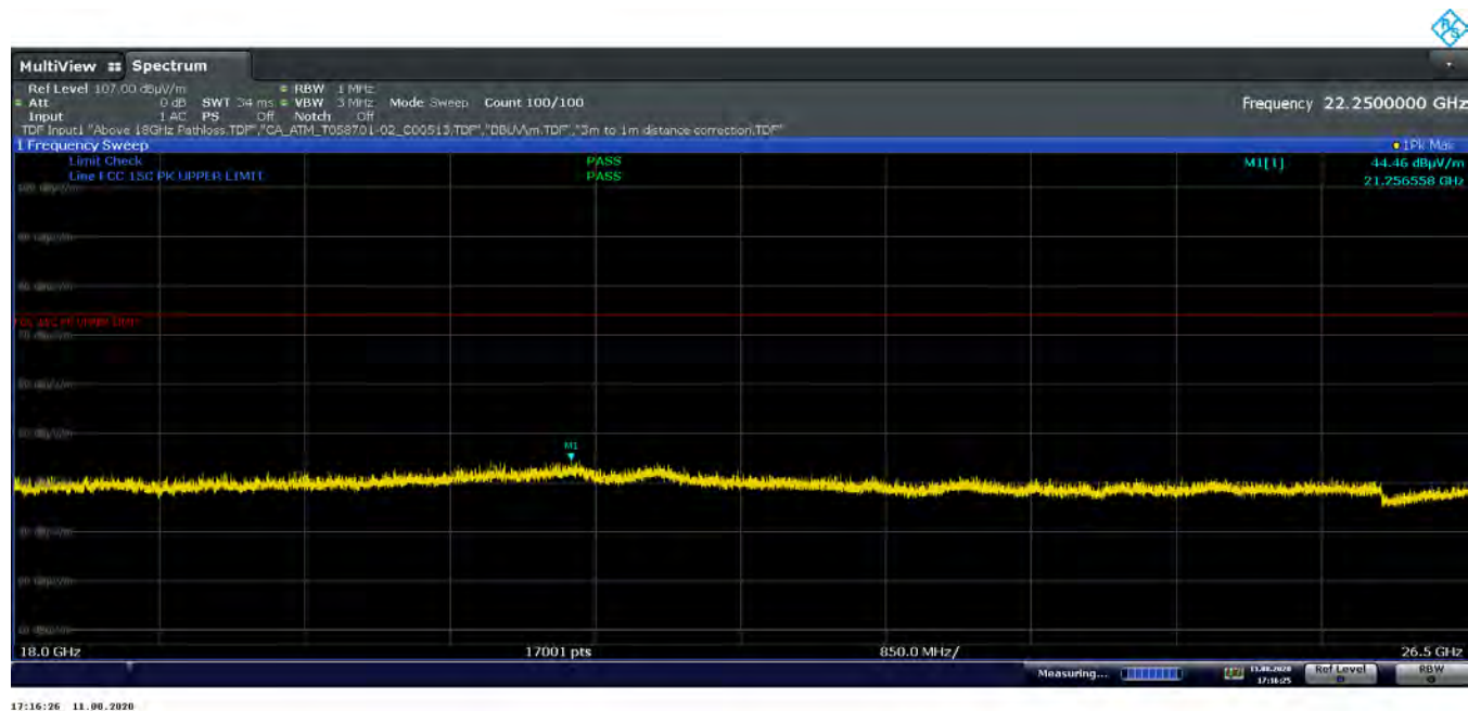
Plot 7-90. Radiated Spurious Emissions Above 18GHz TxBF (4Mbps – Ch.38, ePA, Ant. Pol. H)
