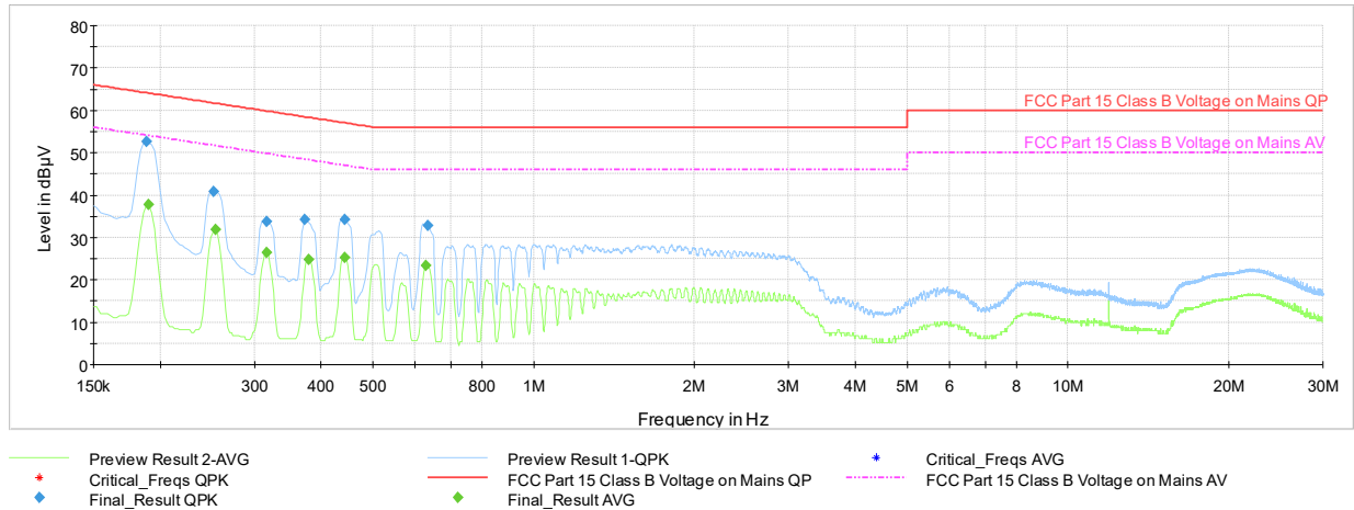
Plot 7-105. AC Line Conducted Plot with Bluetooth HDR (L1, 4Mbps ePA - Ch.1 with Laptop)
