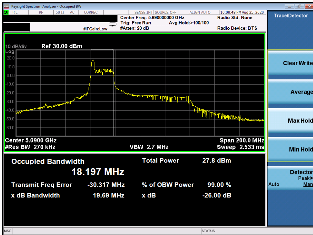
Plot 7-156. 26dB Bandwidth Plot Antenna 2a (80MHz BW 802.11ax Index 0 – RU26 (UNII Band 2C) – Ch. 138)
