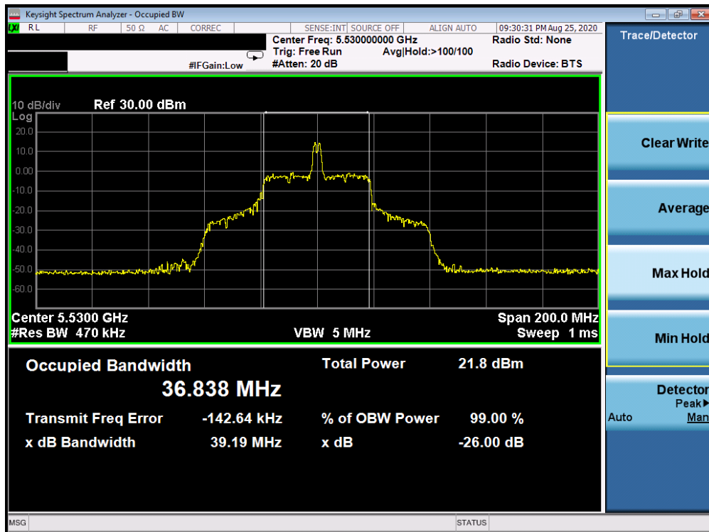
Plot 7-154. 26dB Bandwidth Plot Antenna 2a (80MHz BW 802.11ax Index 18 – RU26 (UNII Band 2C) – Ch. 106)
