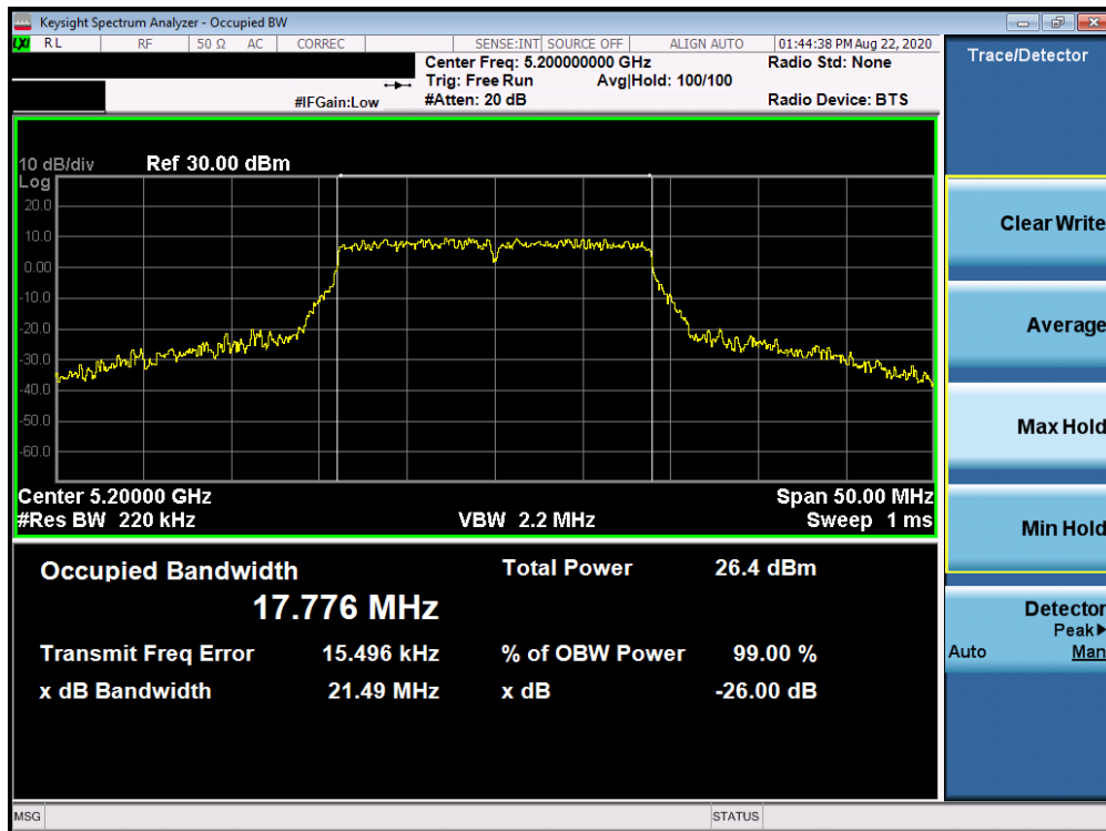
Plot 7-2. 26dB Bandwidth Plot Antenna 2b (20MHz BW 802.11n (UNII Band 1) – Ch. 40)
