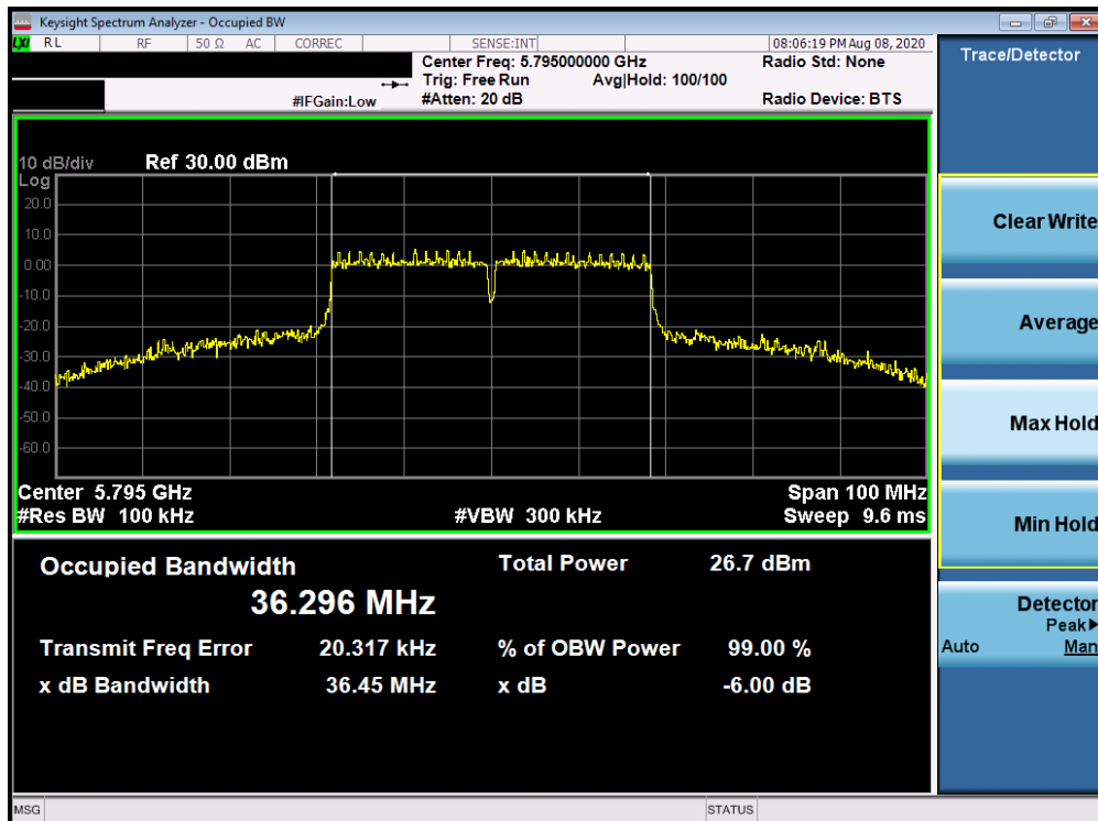
Plot 7-71. 6dB Bandwidth Plot Antenna 2a (40MHz BW 802.11n (UNII Band 3) – Ch. 159)
