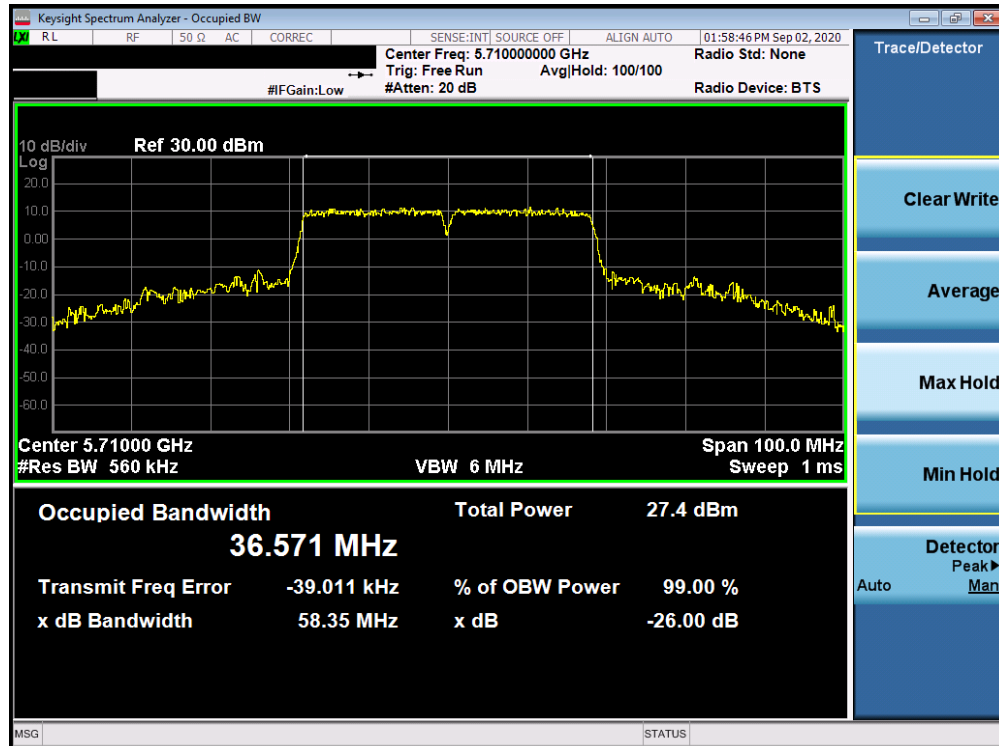
Plot 7-58. 26dB Bandwidth Plot Antenna 1b (40MHz BW 802.11n (UNII Band 2C) – Ch. 142)
