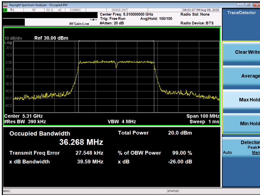
Plot 7-31. 26dB Bandwidth Plot Antenna 2a (40MHz BW 802.11n (UNII Band 2A) – Ch. 62)
