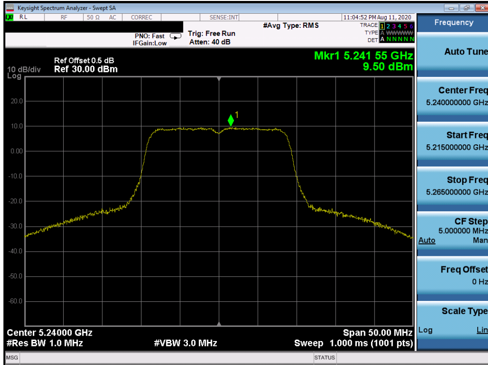
Plot 7-83. Power Spectral Density Plot Antenna 2b (20MHz BW 802.11n (UNII Band 1) – Ch. 48)
