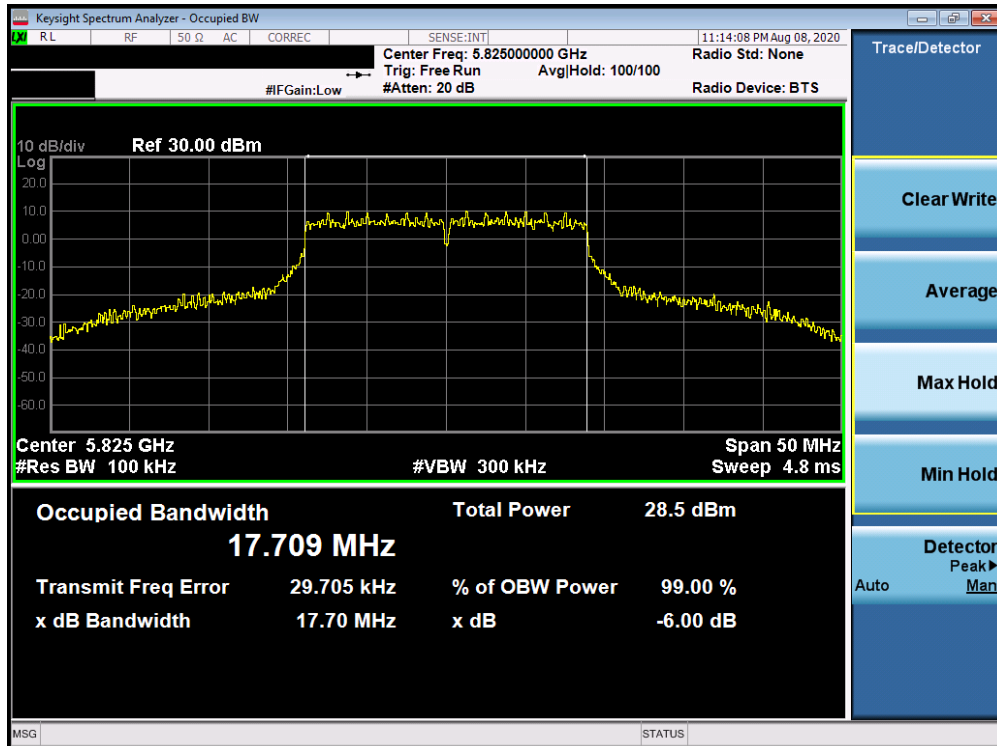
Plot 7-75. 6dB Bandwidth Plot Antenna 1b (20MHz BW 802.11n (UNII Band 3) – Ch. 165)
