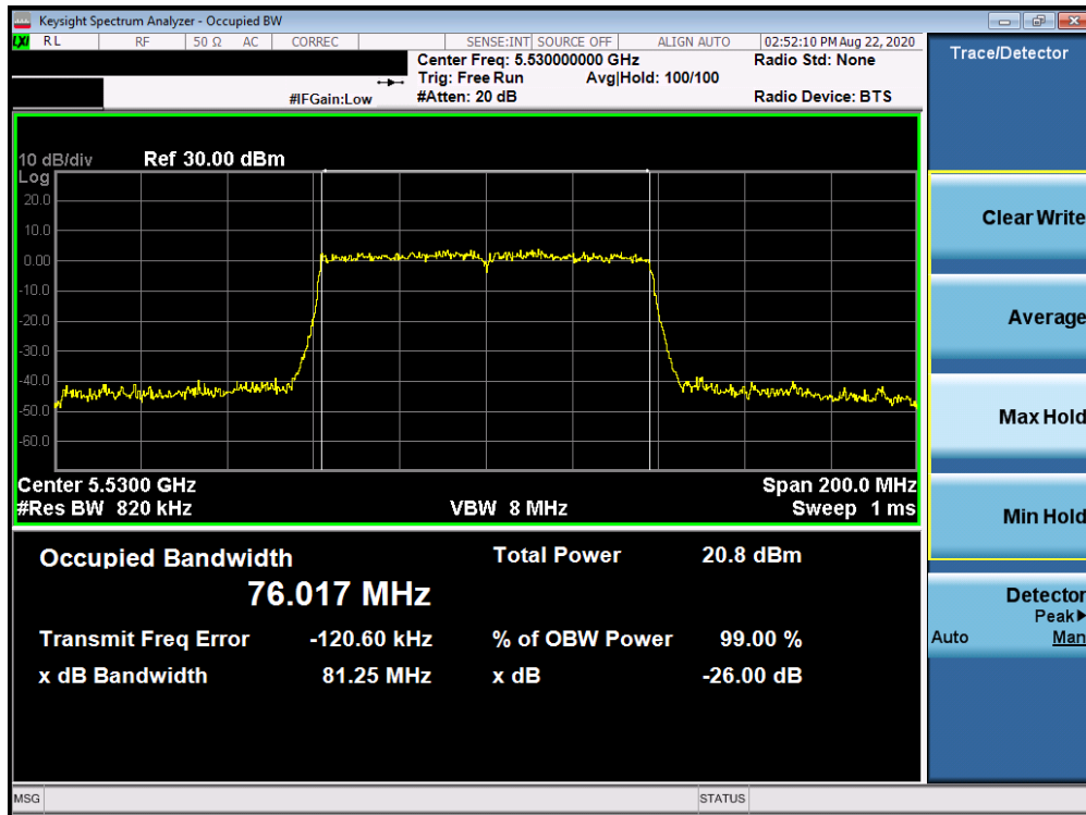
Plot 7-19. 26dB Bandwidth Plot Antenna 2b (80MHz BW 802.11ac (UNII Band 2C) – Ch. 106)
