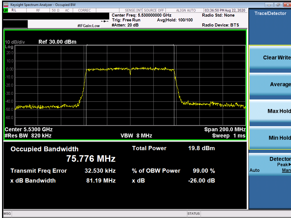
Plot 7-39. 26dB Bandwidth Plot Antenna 2a (80MHz BW 802.11ac (UNII Band 2C) – Ch. 106)
