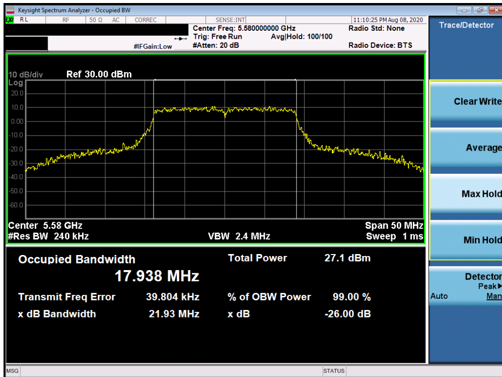
Plot 7-54. 26dB Bandwidth Plot Antenna 1b (20MHz BW 802.11n (UNII Band 2C) – Ch. 116)
