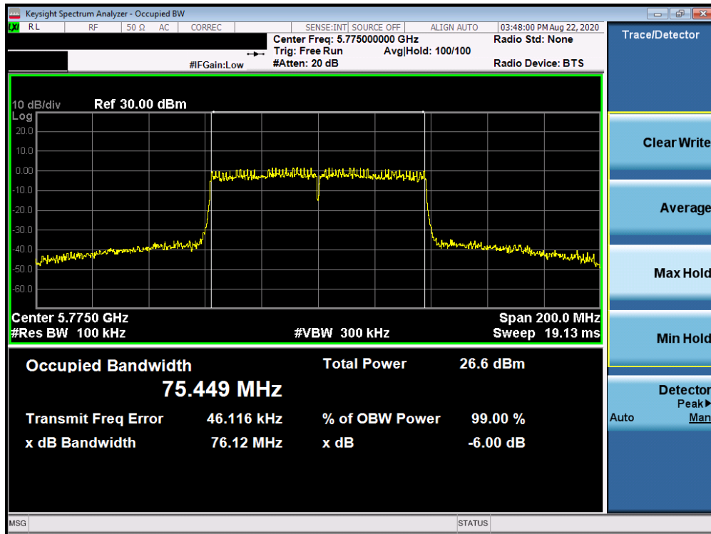
Plot 7-78. 6dB Bandwidth Plot Antenna 1b (80MHz BW 802.11ac (UNII Band 3) – Ch. 155)
