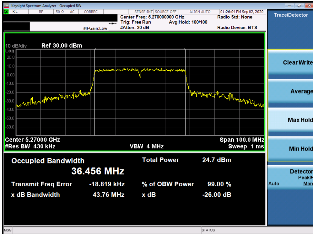
Plot 7-30. 26dB Bandwidth Plot Antenna 2a (40MHz BW 802.11n (UNII Band 2A) – Ch. 54)
