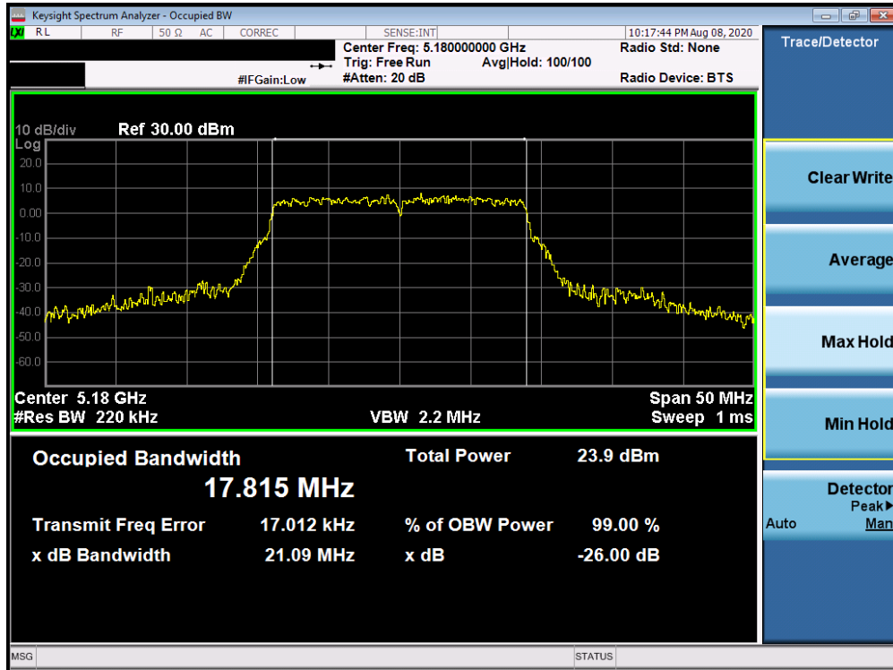
Plot 7-1. 26dB Bandwidth Plot Antenna 2b (20MHz BW 802.11n (UNII Band 1) – Ch. 36)
