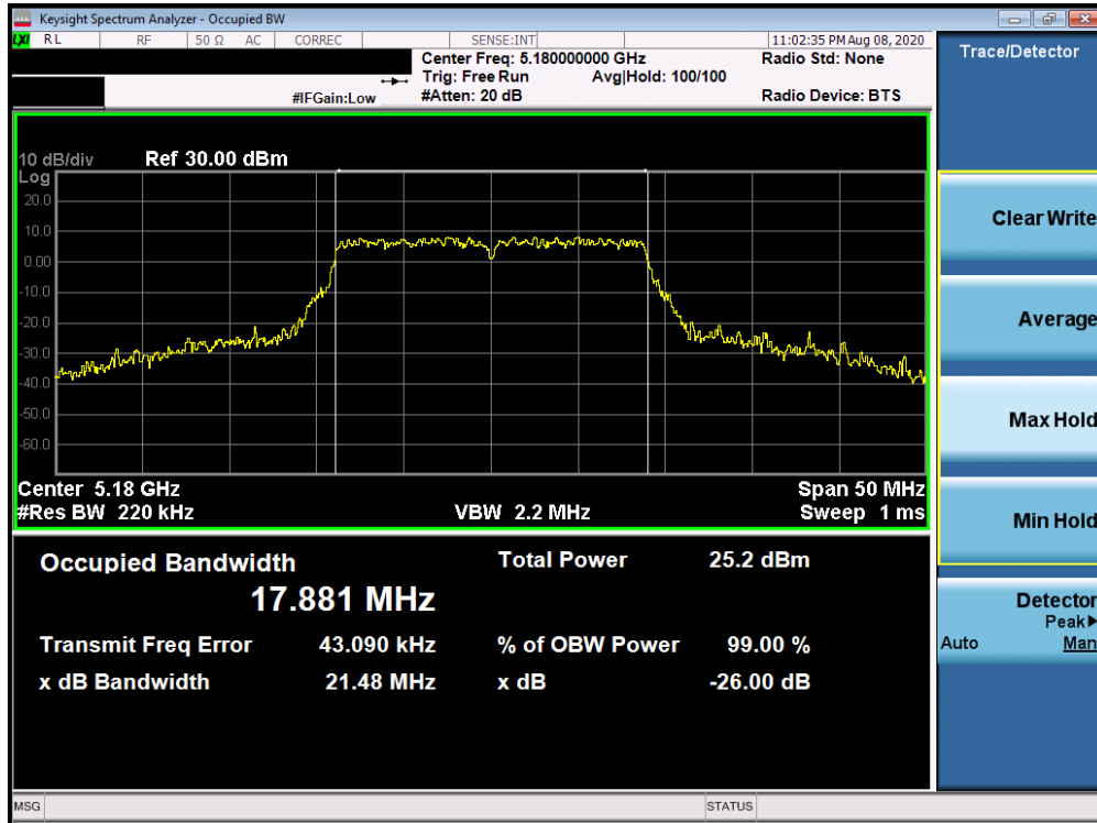
Plot 7-41. 26dB Bandwidth Plot Antenna 1b (20MHz BW 802.11n (UNII Band 1) – Ch. 36)
