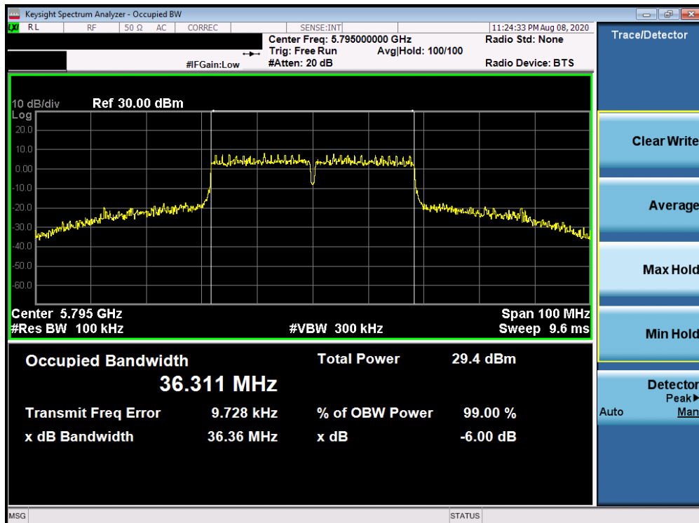
Plot 7-77. 6dB Bandwidth Plot Antenna 1b (40MHz BW 802.11n (UNII Band 3) – Ch. 159)
