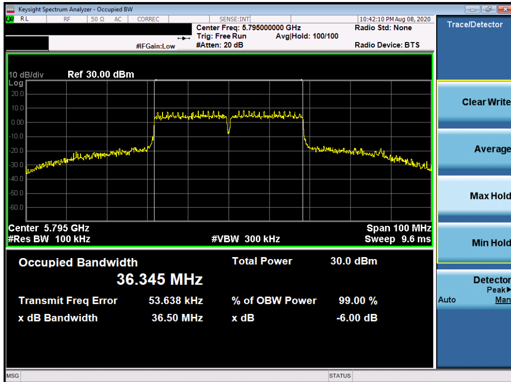
Plot 7-65. 6dB Bandwidth Plot Antenna 2b (40MHz BW 802.11n (UNII Band 3) – Ch. 159)
