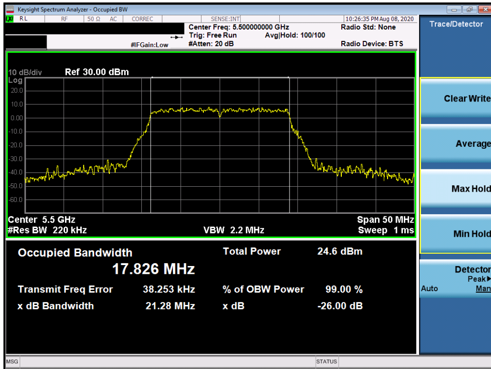
Plot 7-13. 26dB Bandwidth Plot Antenna 2b (20MHz BW 802.11n (UNII Band 2C) – Ch. 100)
