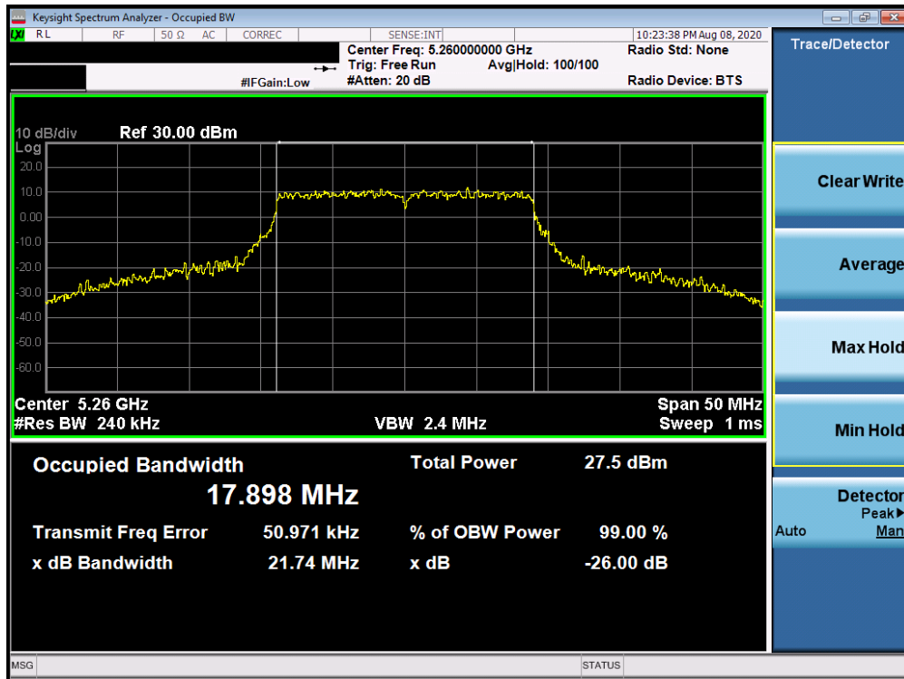
Plot 7-7. 26dB Bandwidth Plot Antenna 2b (20MHz BW 802.11n (UNII Band 2A) – Ch. 52)
