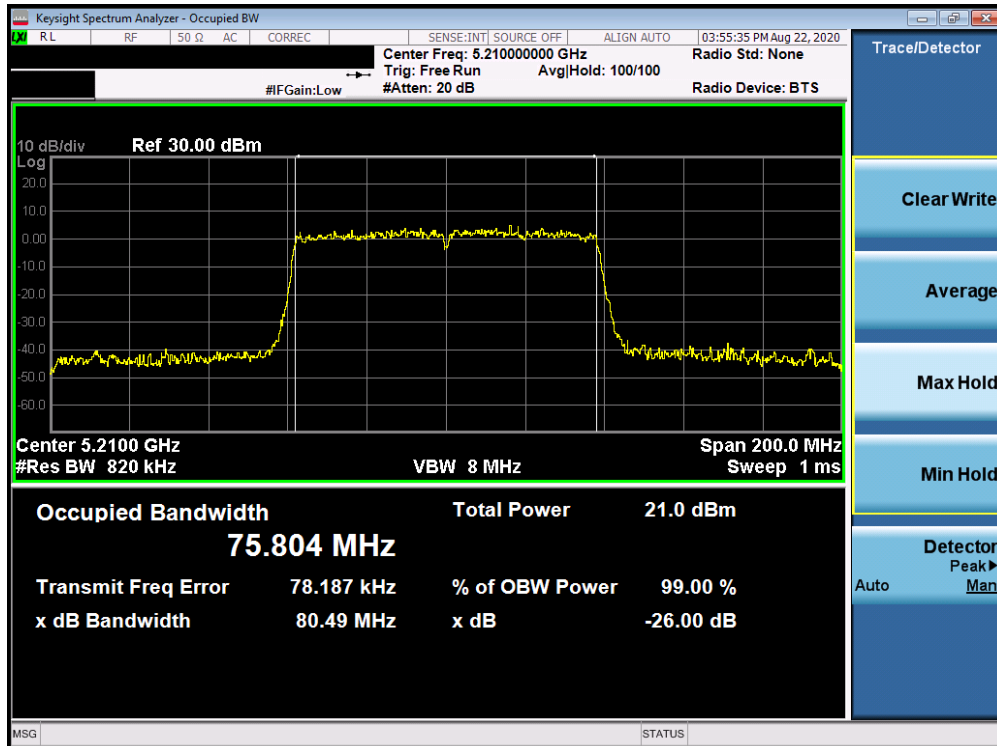
Plot 7-46. 26dB Bandwidth Plot Antenna 1b (80MHz BW 802.11ac (UNII Band 1) – Ch. 42)
