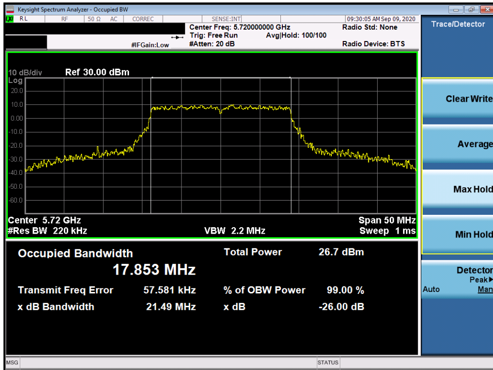
Plot 7-15. 26dB Bandwidth Plot Antenna 2b (20MHz BW 802.11n (UNII Band 2C) – Ch. 144)
