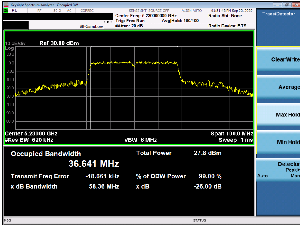
Plot 7-45. 26dB Bandwidth Plot Antenna 1b (40MHz BW 802.11n (UNII Band 1) – Ch. 46)
