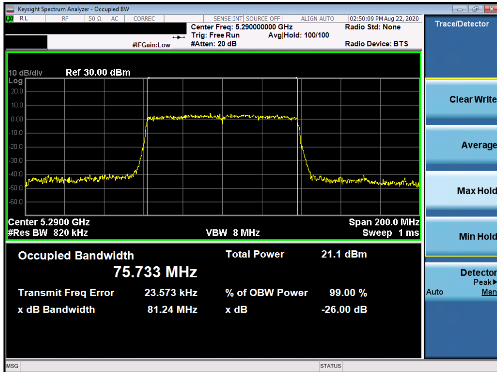
Plot 7-12. 26dB Bandwidth Plot Antenna 2b (80MHz BW 802.11ac (UNII Band 2A) – Ch. 58)
