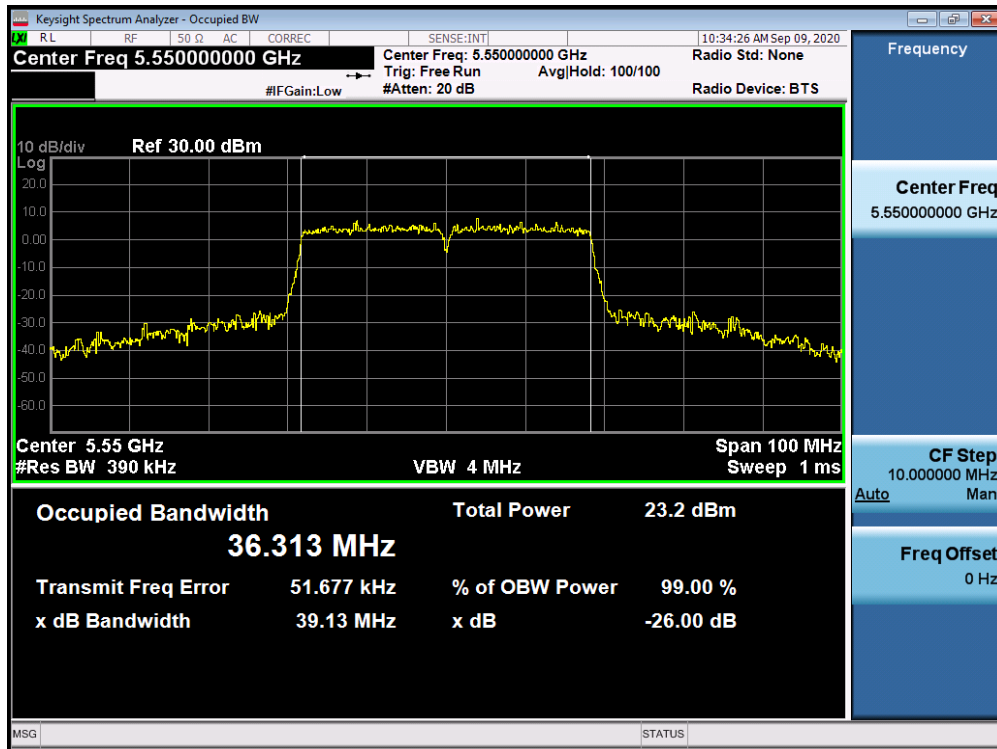
Plot 7-37. 26dB Bandwidth Plot Antenna 2a (40MHz BW 802.11n (UNII Band 2C) – Ch. 110)
