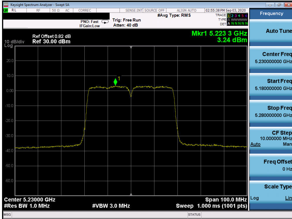
Plot 7-87. ISED Power Spectral Density Plot Antenna 2b (40MHz BW 802.11n (UNII Band 1) – Ch. 46)
