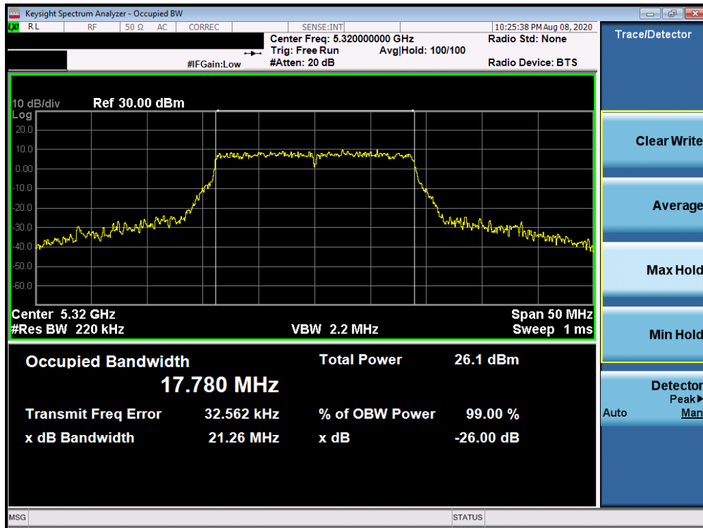
Plot 7-9. 26dB Bandwidth Plot Antenna 2b (20MHz BW 802.11n (UNII Band 2A) – Ch. 64)
