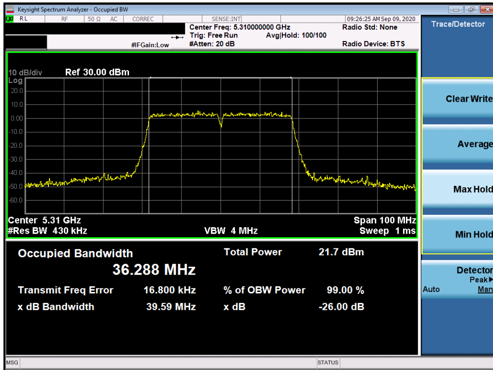
Plot 7-11. 26dB Bandwidth Plot Antenna 2b (40MHz BW 802.11n (UNII Band 2A) – Ch. 62)
