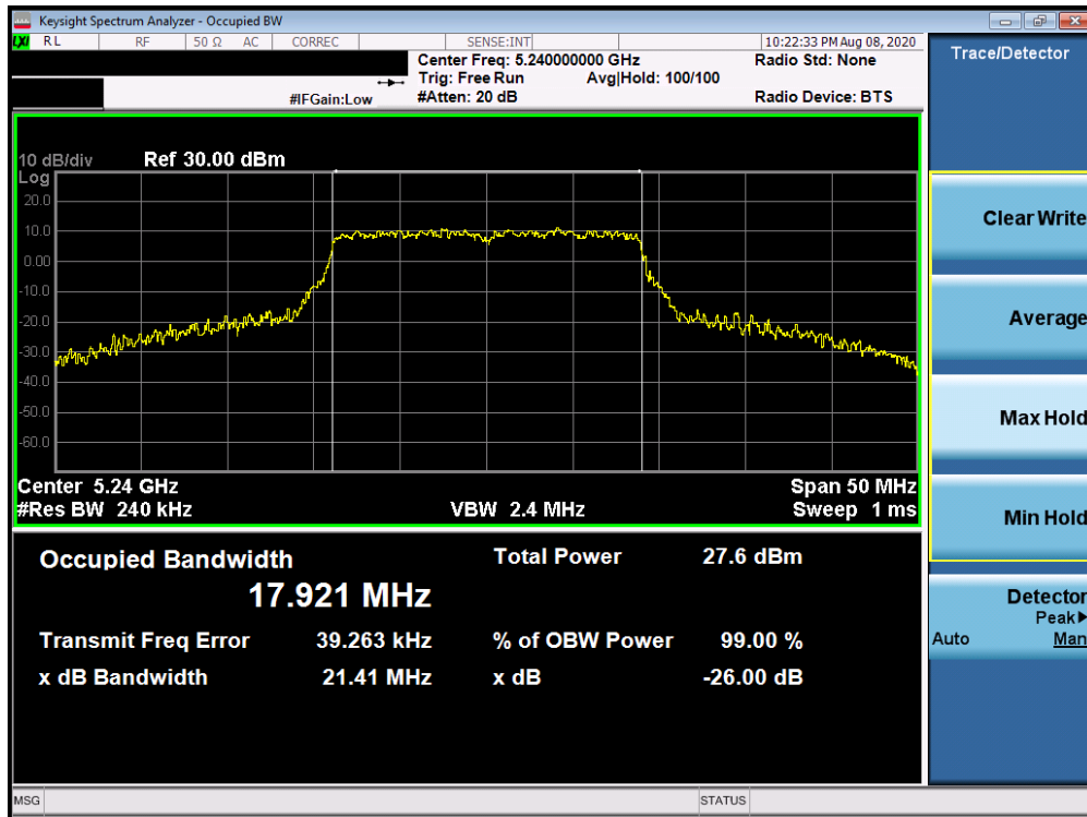
Plot 7-3. 26dB Bandwidth Plot Antenna 2b (20MHz BW 802.11n (UNII Band 1) – Ch. 48)
