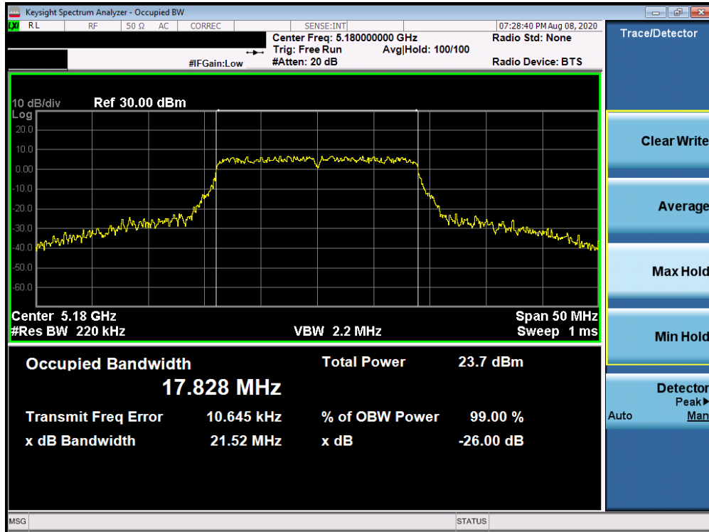
Plot 7-21. 26dB Bandwidth Plot Antenna 2a (20MHz BW 802.11n (UNII Band 1) – Ch. 36)
