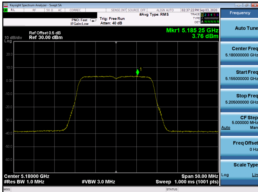
Plot 7-80. ISED Power Spectral Density Plot Antenna 2b (20MHz BW 802.11n (UNII Band 1) – Ch. 36)
