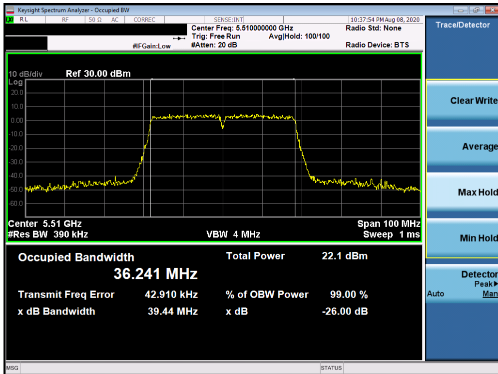
Plot 7-16. 26dB Bandwidth Plot Antenna 2b (40MHz BW 802.11n (UNII Band 2C) – Ch. 102)
