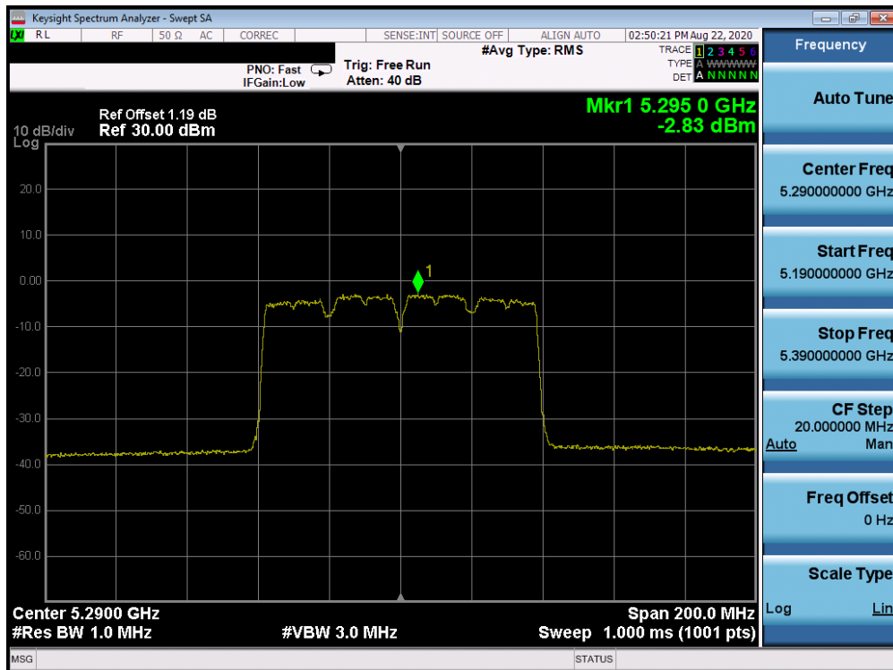
Plot 7-94. Power Spectral Density Plot Antenna 2b (80MHz BW 802.11ac (UNII Band 2A) – Ch. 58)
