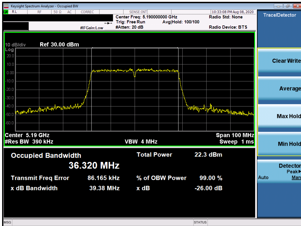
Plot 7-4. 26dB Bandwidth Plot Antenna 2b (40MHz BW 802.11n (UNII Band 1) – Ch. 38)
