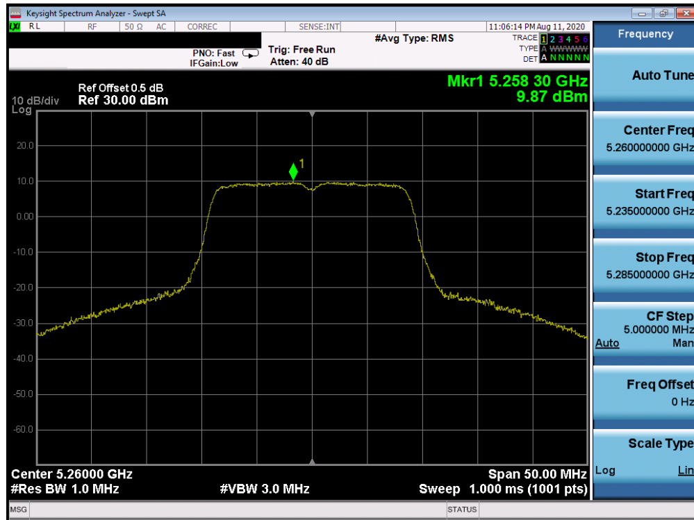
Plot 7-89. Power Spectral Density Plot Antenna 2b (20MHz BW 802.11n (UNII Band 2A) – Ch. 52)
