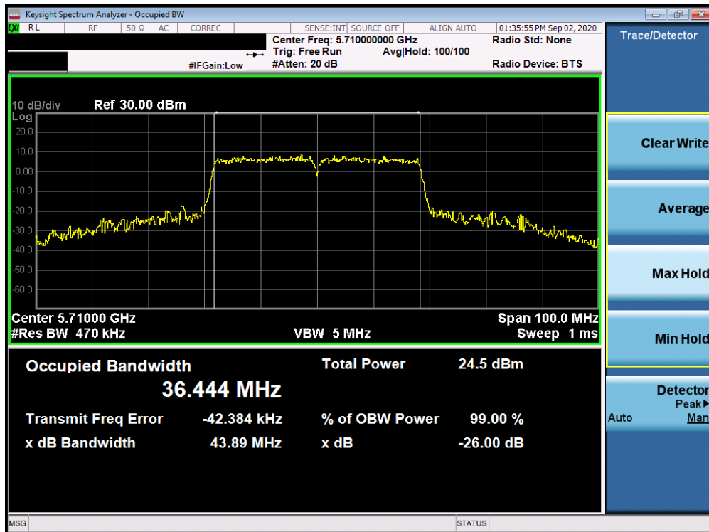
Plot 7-38. 26dB Bandwidth Plot Antenna 2a (40MHz BW 802.11n (UNII Band 2C) – Ch. 142)
