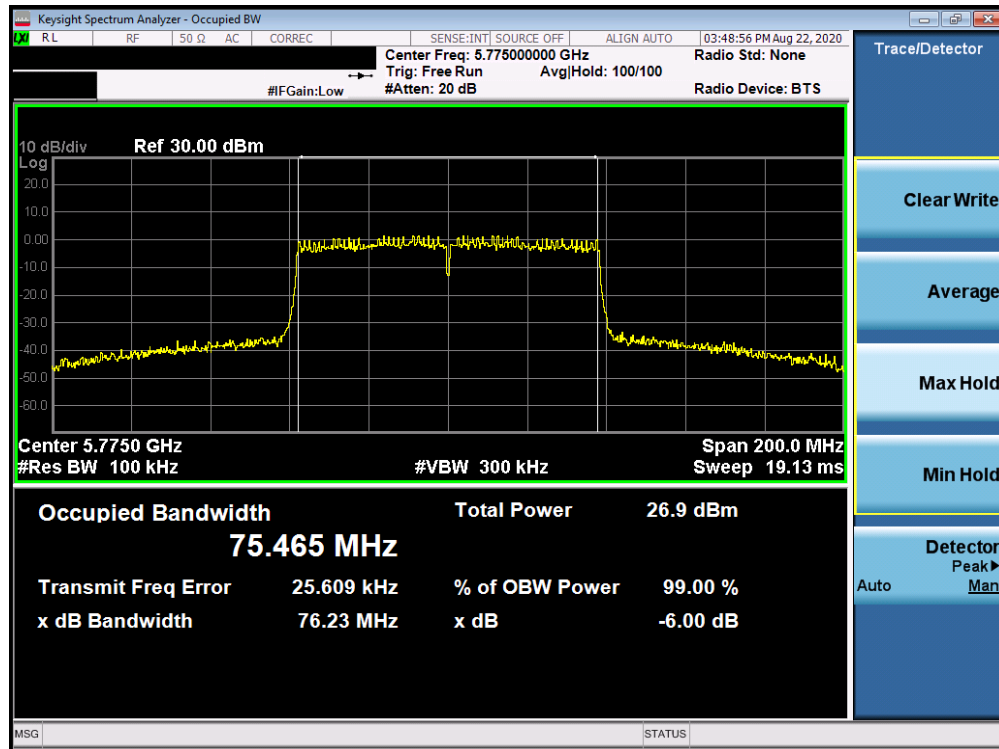
Plot 7-72. 6dB Bandwidth Plot Antenna 2a (80MHz BW 802.11ac (UNII Band 3) – Ch. 155)
