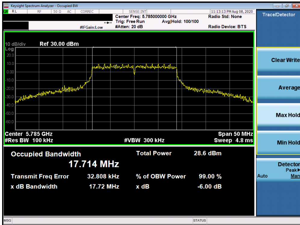
Plot 7-74. 6dB Bandwidth Plot Antenna 1b (20MHz BW 802.11n (UNII Band 3) – Ch. 157)
