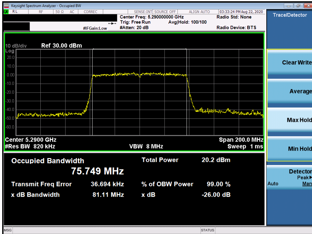
Plot 7-32. 26dB Bandwidth Plot Antenna 2a (80MHz BW 802.11ac (UNII Band 2A) – Ch. 58)
