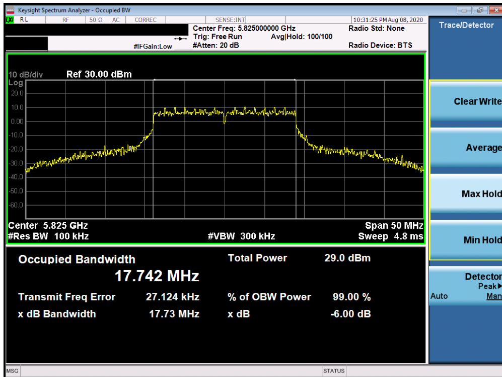
Plot 7-63. 6dB Bandwidth Plot Antenna 2b (20MHz BW 802.11n (UNII Band 3) – Ch. 165)
