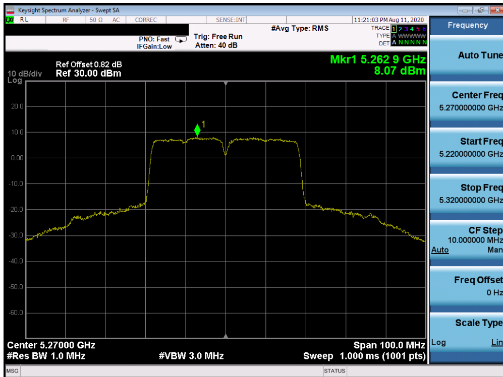
Plot 7-92. Power Spectral Density Plot Antenna 2b (40MHz BW 802.11n (UNII Band 2A) – Ch. 54)
