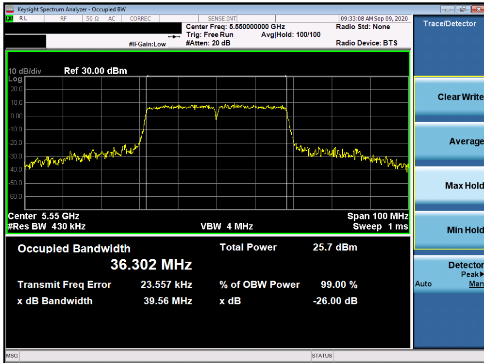
Plot 7-17. 26dB Bandwidth Plot Antenna 2b (40MHz BW 802.11n (UNII Band 2C) – Ch. 110)
