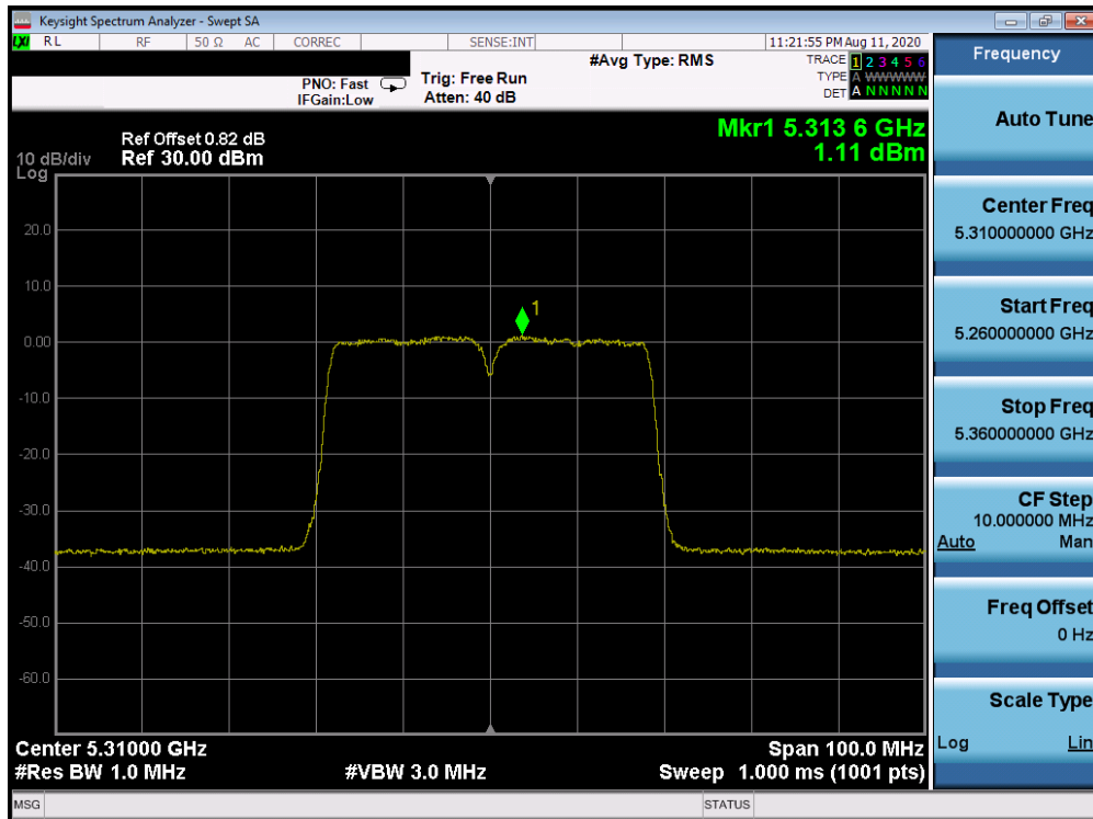
Plot 7-93. Power Spectral Density Plot Antenna 2b (40MHz BW 802.11n (UNII Band 2A) – Ch. 62)
