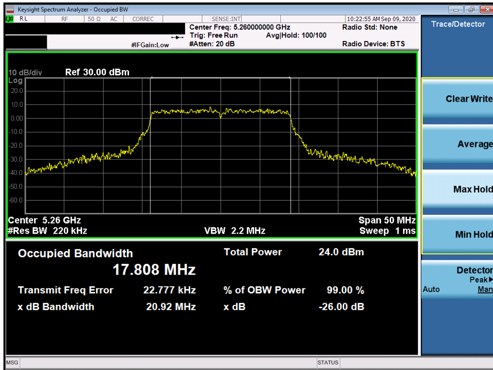
Plot 7-27. 26dB Bandwidth Plot Antenna 2a (20MHz BW 802.11n (UNII Band 2A) – Ch. 52)
