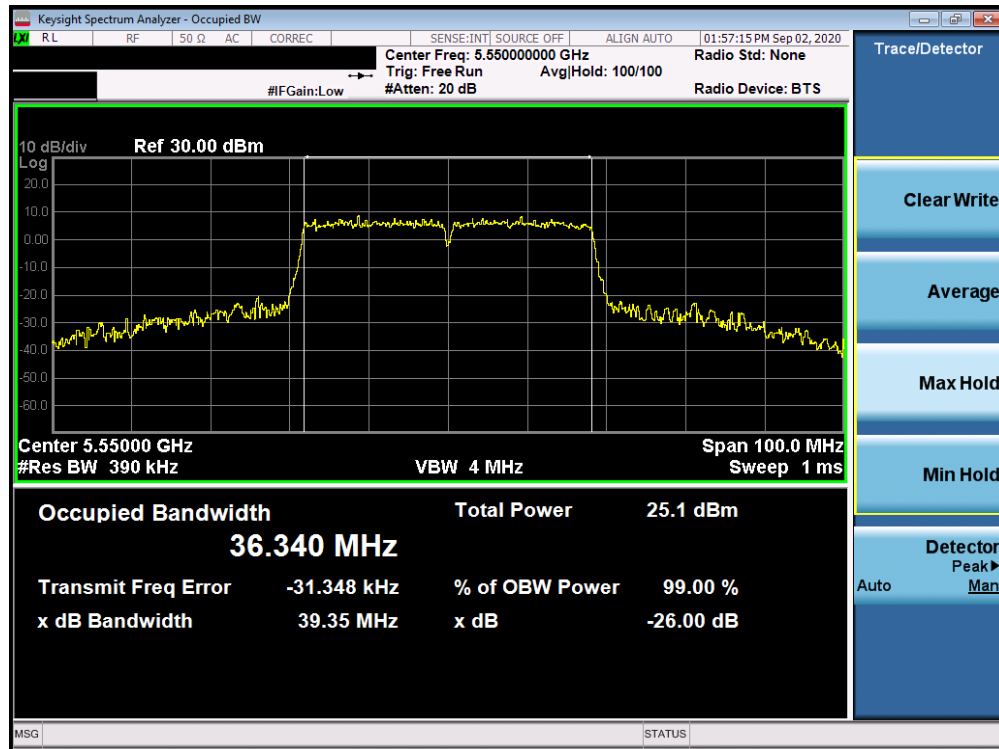
Plot 7-57. 26dB Bandwidth Plot Antenna 1b (40MHz BW 802.11n (UNII Band 2C) – Ch. 110)
