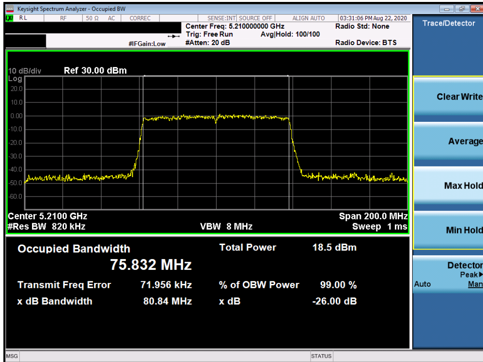
Plot 7-26. 26dB Bandwidth Plot Antenna 2a (80MHz BW 802.11ac (UNII Band 1) – Ch. 42)
