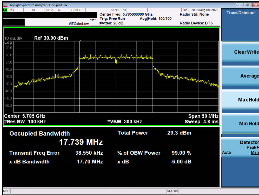
Plot 7-62. 6dB Bandwidth Plot Antenna 2b (20MHz BW 802.11n (UNII Band 3) – Ch. 157)
