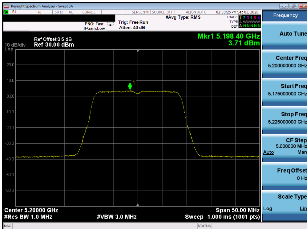
Plot 7-82. ISED Power Spectral Density Plot Antenna 2b (20MHz BW 802.11n (UNII Band 1) – Ch. 40)
