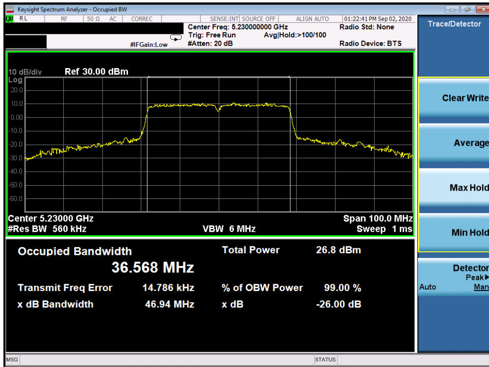
Plot 7-25. 26dB Bandwidth Plot Antenna 2a (40MHz BW 802.11n (UNII Band 1) – Ch. 46)
