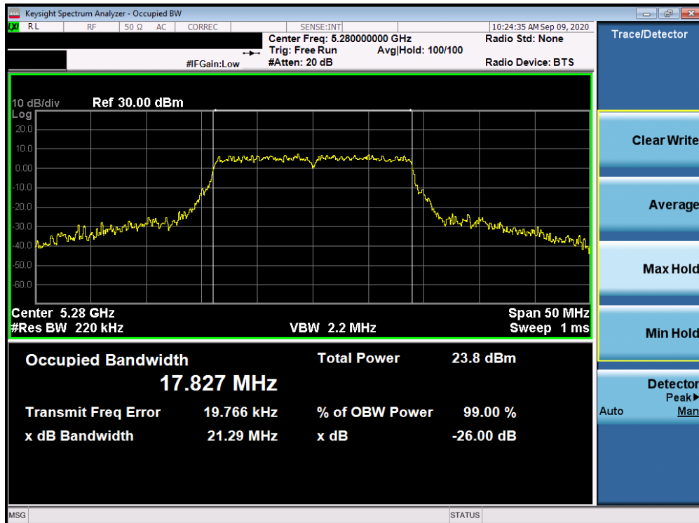
Plot 7-28. 26dB Bandwidth Plot Antenna 2a (20MHz BW 802.11n (UNII Band 2A) – Ch. 56)
