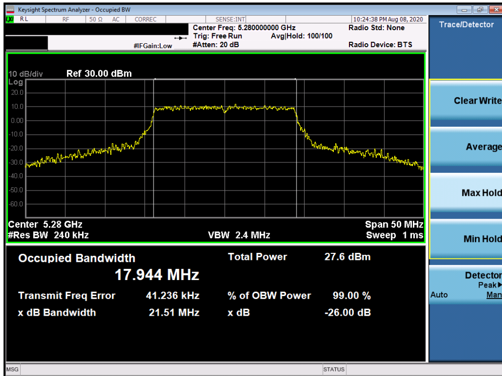
Plot 7-8. 26dB Bandwidth Plot Antenna 2b (20MHz BW 802.11n (UNII Band 2A) – Ch. 56)
