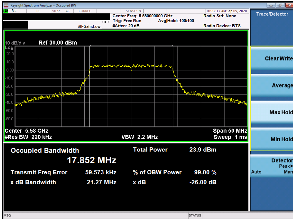
Plot 7-34. 26dB Bandwidth Plot Antenna 2a (20MHz BW 802.11n (UNII Band 2C) – Ch. 116)
