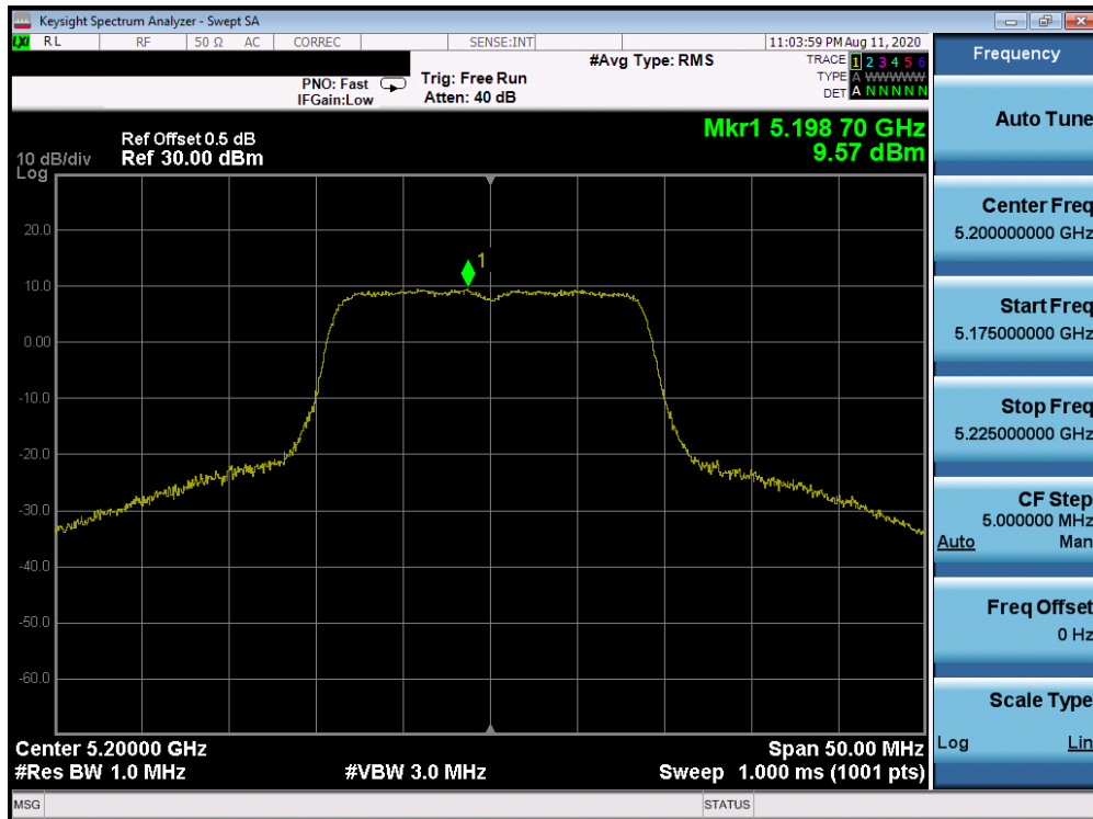
Plot 7-81. Power Spectral Density Plot Antenna 2b (20MHz BW 802.11n (UNII Band 1) – Ch. 40)
