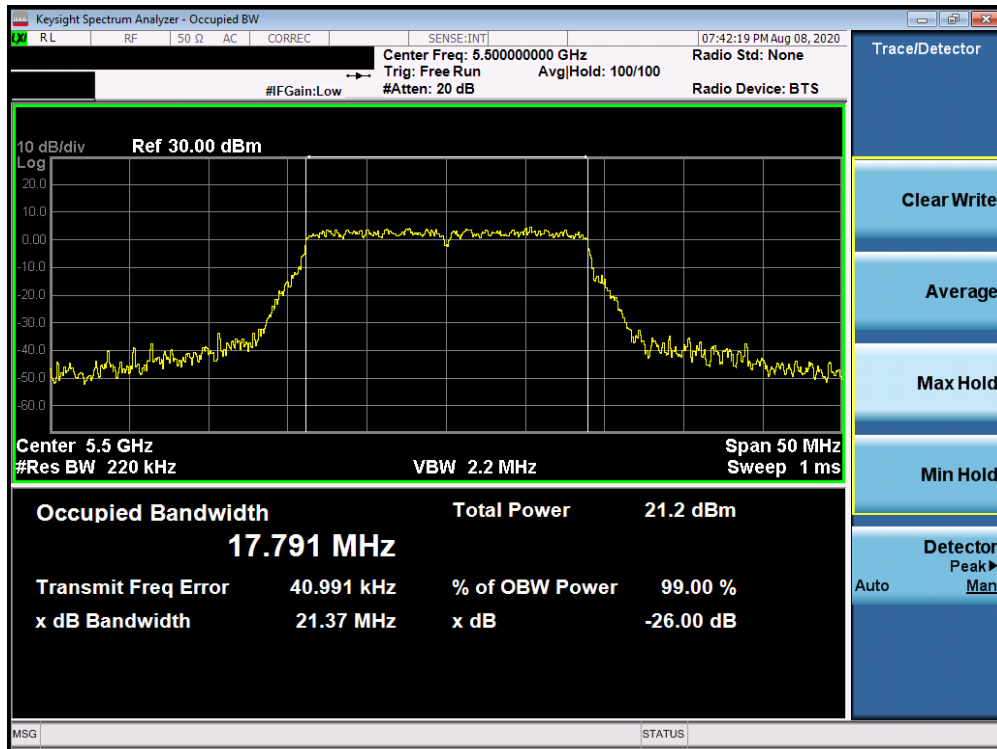
Plot 7-33. 26dB Bandwidth Plot Antenna 2a (20MHz BW 802.11n (UNII Band 2C) – Ch. 100)
