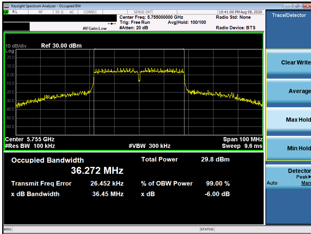
Plot 7-64. 6dB Bandwidth Plot Antenna 2b (40MHz BW 802.11n (UNII Band 3) – Ch. 151)
