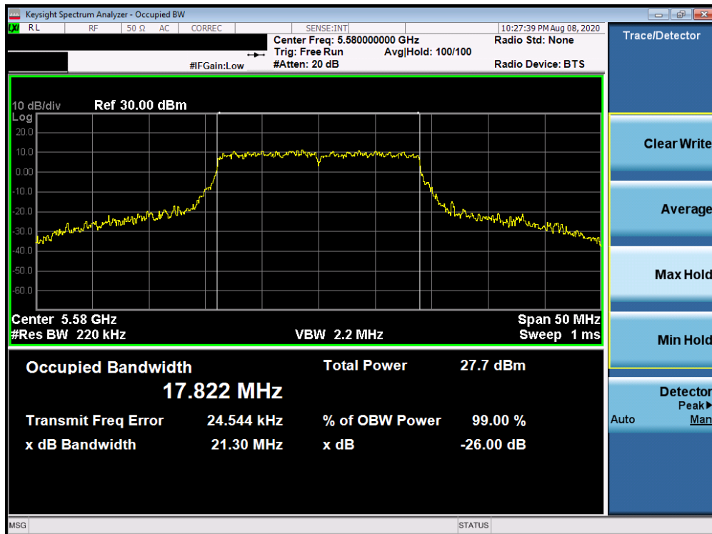
Plot 7-14. 26dB Bandwidth Plot Antenna 2b (20MHz BW 802.11n (UNII Band 2C) – Ch. 116)
