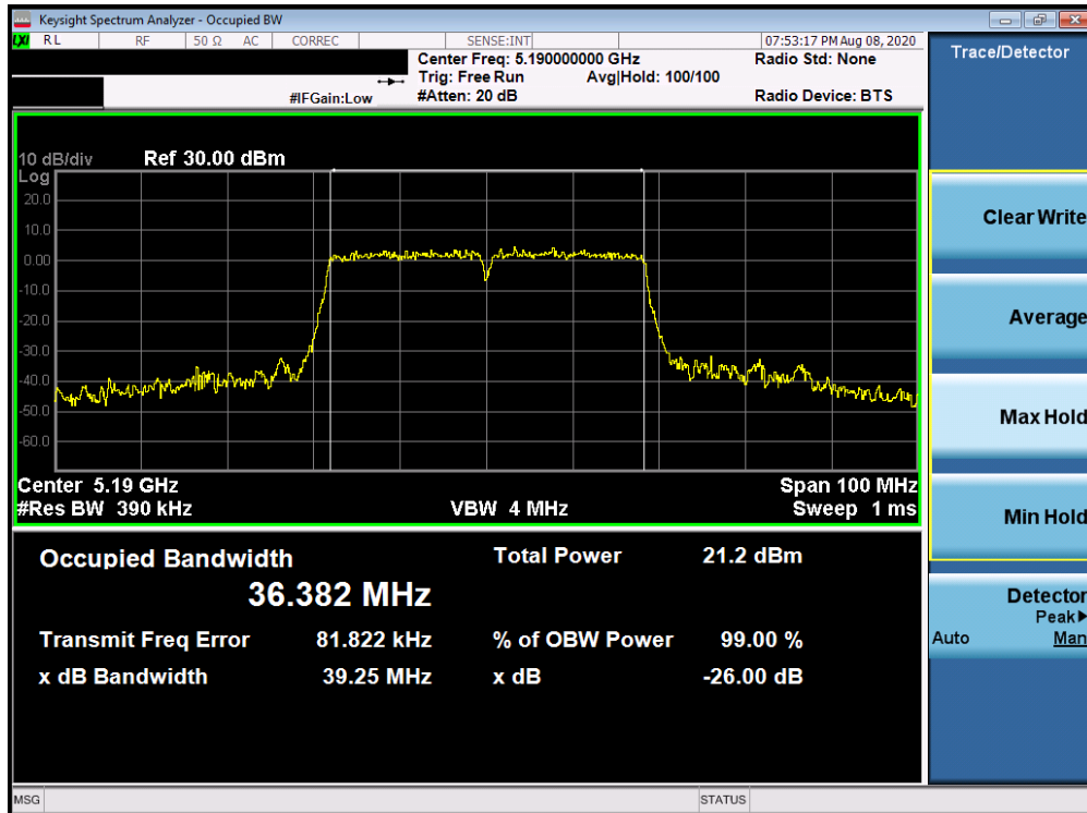
Plot 7-24. 26dB Bandwidth Plot Antenna 2a (40MHz BW 802.11n (UNII Band 1) – Ch. 38)
