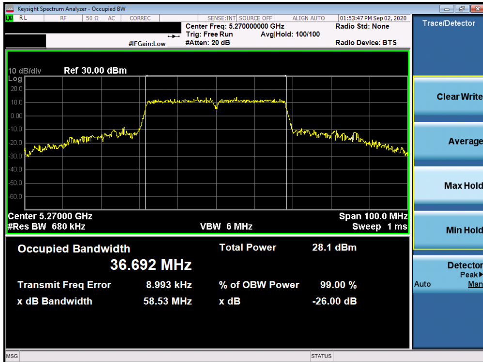
Plot 7-50. 26dB Bandwidth Plot Antenna 1b (40MHz BW 802.11n (UNII Band 2A) – Ch. 54)
