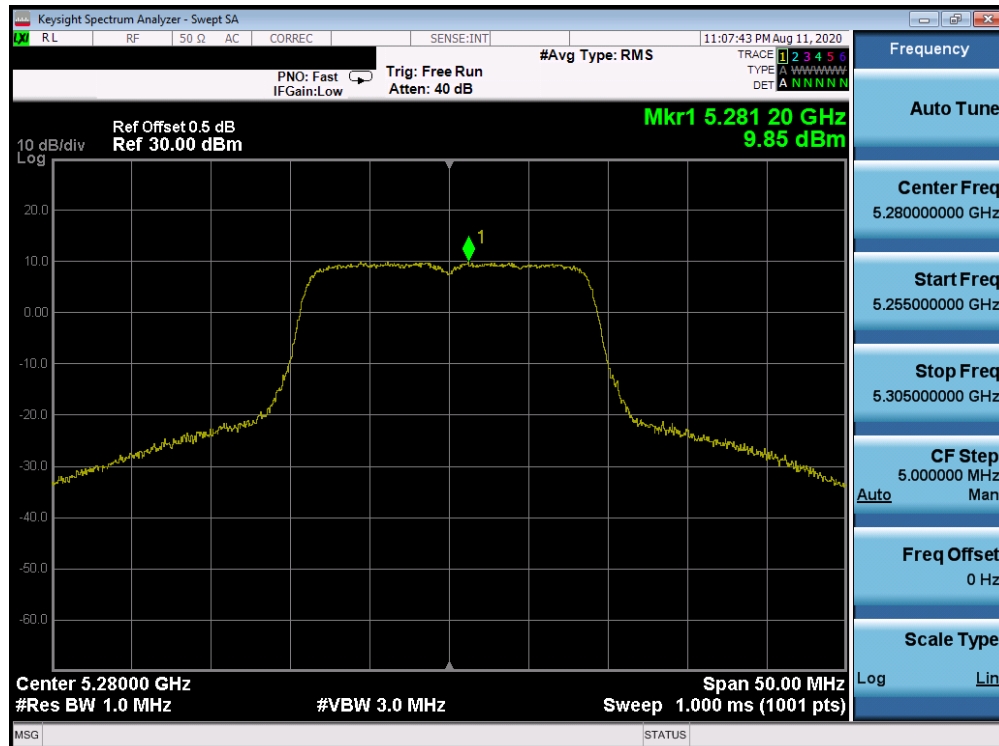
Plot 7-90. Power Spectral Density Plot Antenna 2b (20MHz BW 802.11n (UNII Band 2A) – Ch. 56)
