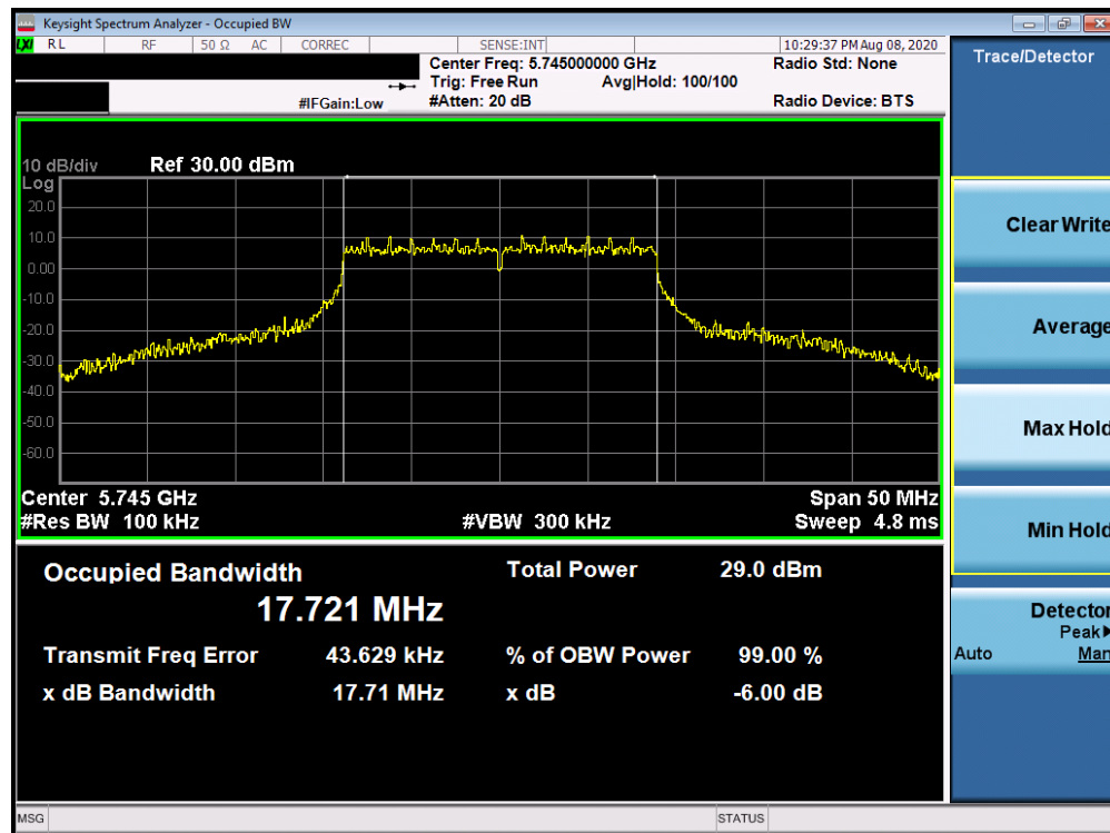
Plot 7-61. 6dB Bandwidth Plot Antenna 2b (20MHz BW 802.11n (UNII Band 3) – Ch. 149)
