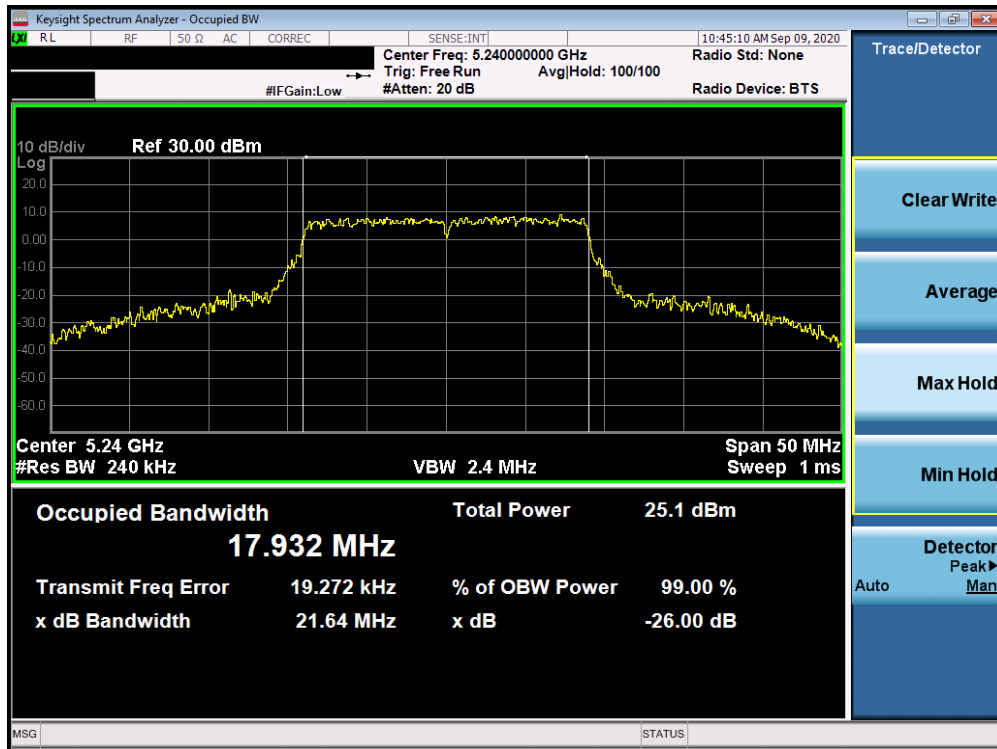
Plot 7-43. 26dB Bandwidth Plot Antenna 1b (20MHz BW 802.11n (UNII Band 1) – Ch. 48)
