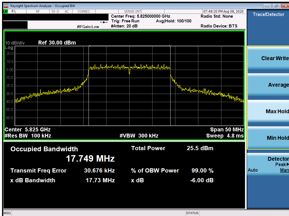
Plot 7-69. 6dB Bandwidth Plot Antenna 2a (20MHz BW 802.11n (UNII Band 3) – Ch. 165)
