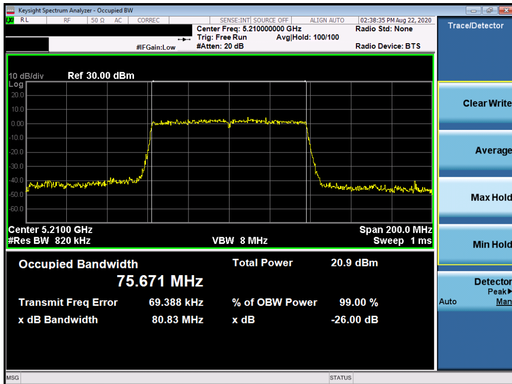
Plot 7-6. 26dB Bandwidth Plot Antenna 2b (80MHz BW 802.11ac (UNII Band 1) – Ch. 42)
