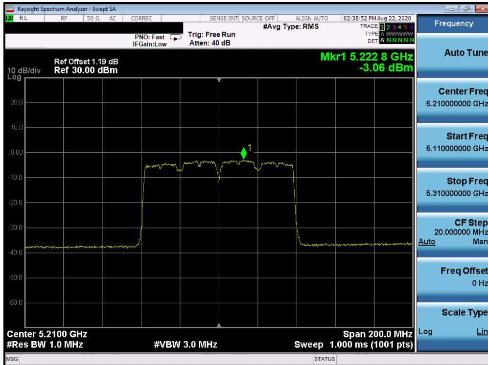
Plot 7-88. Power Spectral Density Plot Antenna 2b (80MHz BW 802.11ac (UNII Band 1) – Ch. 42)
