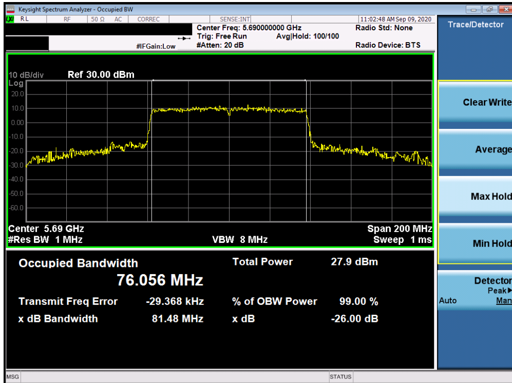
Plot 7-60. 26dB Bandwidth Plot Antenna 1b (80MHz BW 802.11ac (UNII Band 2C) – Ch. 138)
