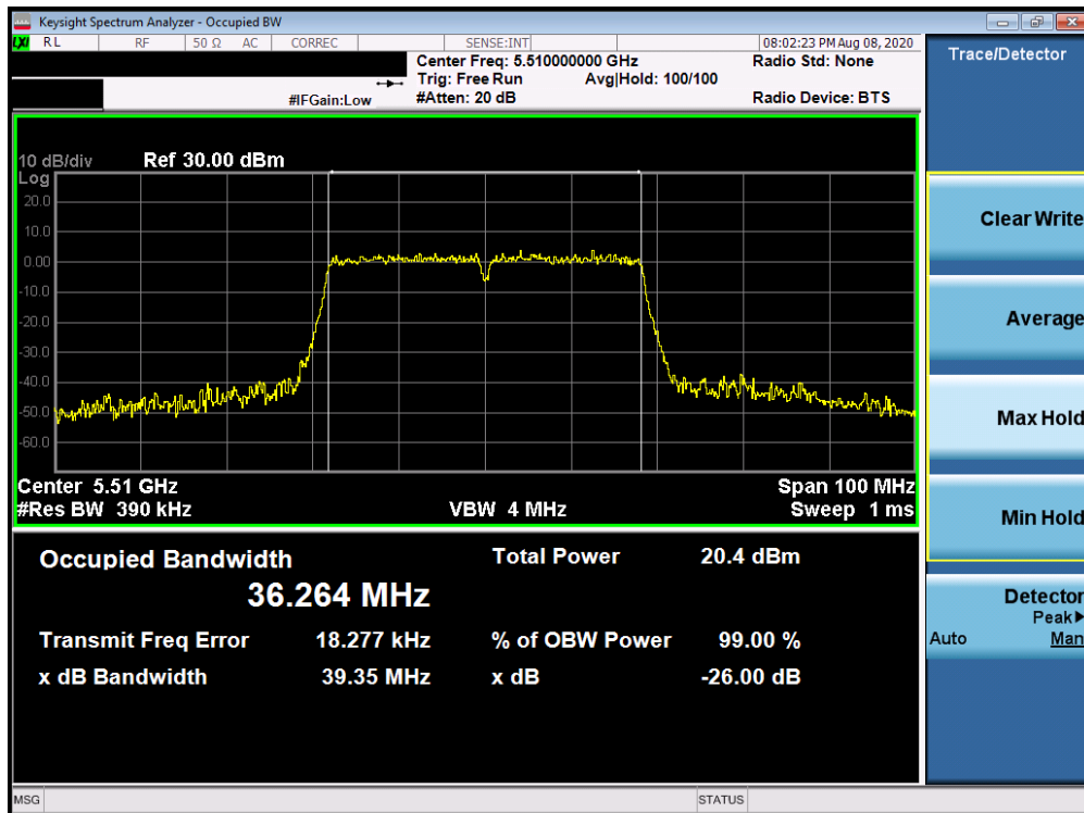
Plot 7-36. 26dB Bandwidth Plot Antenna 2a (40MHz BW 802.11n (UNII Band 2C) – Ch. 102)
