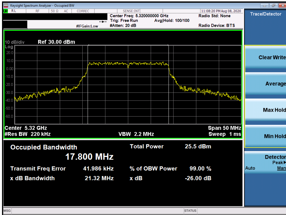
Plot 7-49. 26dB Bandwidth Plot Antenna 1b (20MHz BW 802.11n (UNII Band 2A) – Ch. 64)
