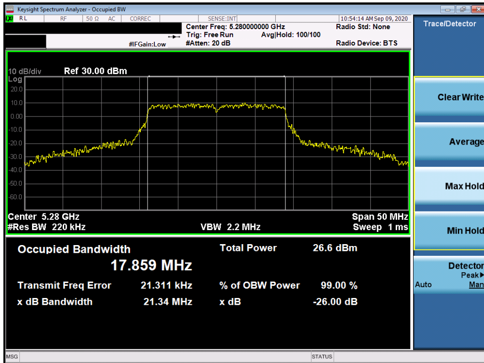
Plot 7-48. 26dB Bandwidth Plot Antenna 1b (20MHz BW 802.11n (UNII Band 2A) – Ch. 56)
