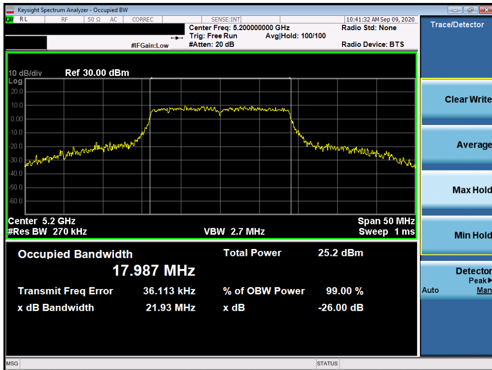
Plot 7-42. 26dB Bandwidth Plot Antenna 1b (20MHz BW 802.11n (UNII Band 1) – Ch. 40)
