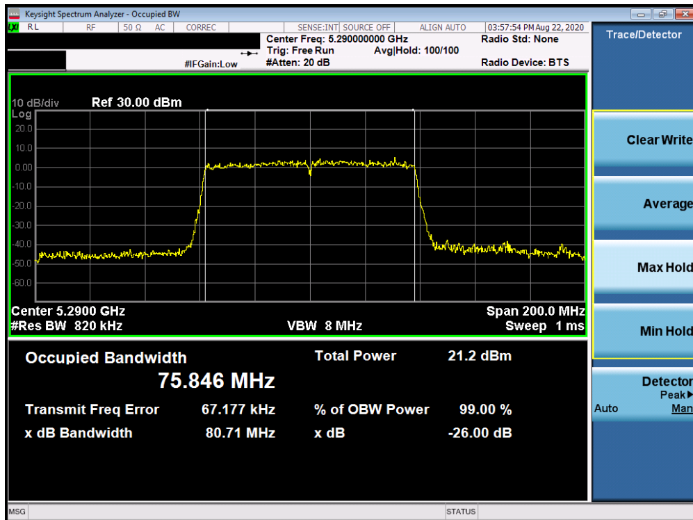
Plot 7-52. 26dB Bandwidth Plot Antenna 1b (80MHz BW 802.11ac (UNII Band 2A) – Ch. 58)
