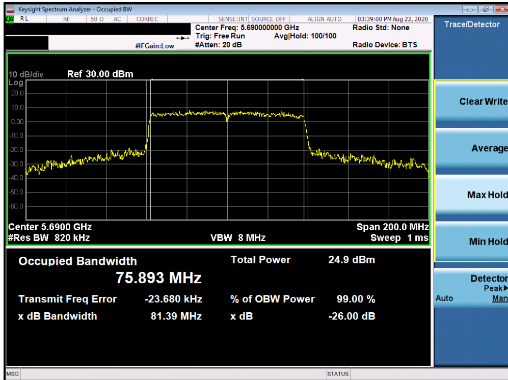
Plot 7-40. 26dB Bandwidth Plot Antenna 2a (80MHz BW 802.11ac (UNII Band 2C) – Ch. 138)
