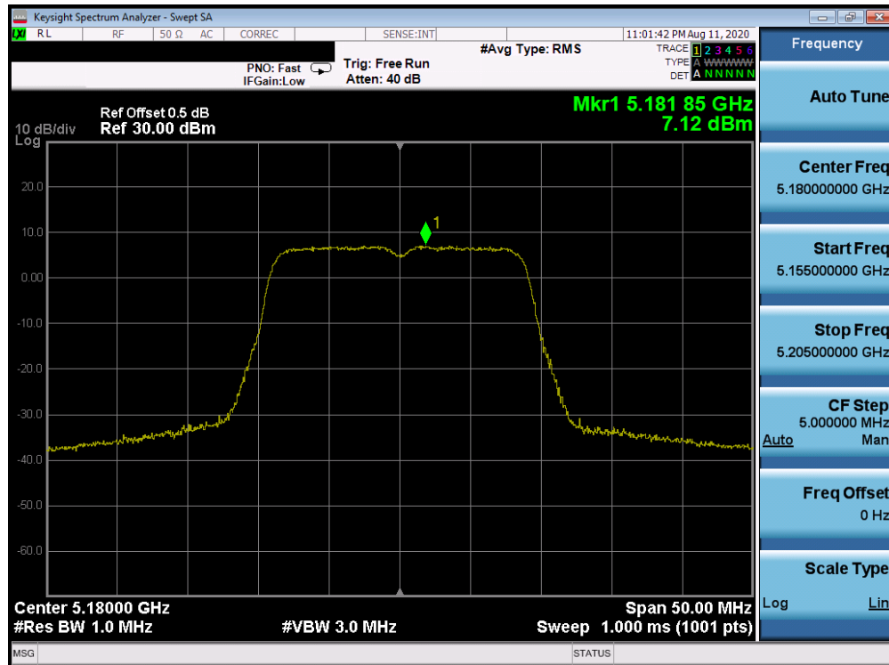
Plot 7-79. Power Spectral Density Plot Antenna 2b (20MHz BW 802.11n (UNII Band 1) – Ch. 36)
