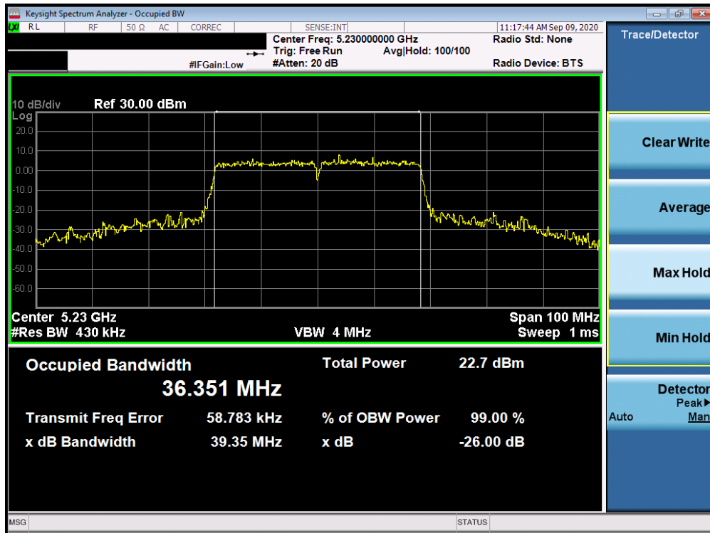
Plot 7-5. 26dB Bandwidth Plot Antenna 2b (40MHz BW 802.11n (UNII Band 1) – Ch. 46)
