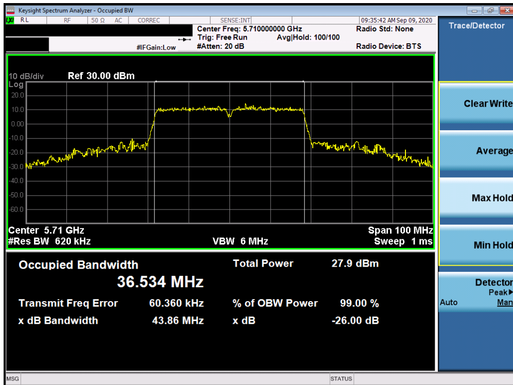
Plot 7-18. 26dB Bandwidth Plot Antenna 2b (40MHz BW 802.11n (UNII Band 2C) – Ch. 142)
