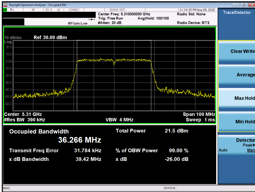
Plot 7-51. 26dB Bandwidth Plot Antenna 1b (40MHz BW 802.11n (UNII Band 2A) – Ch. 62)
