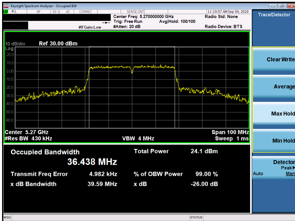
Plot 7-10. 26dB Bandwidth Plot Antenna 2b (40MHz BW 802.11n (UNII Band 2A) – Ch. 54)
