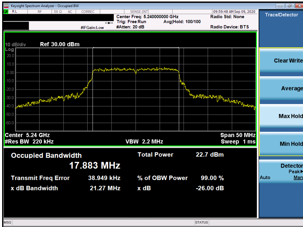
Plot 7-23. 26dB Bandwidth Plot Antenna 2a (20MHz BW 802.11n (UNII Band 1) – Ch. 48)
