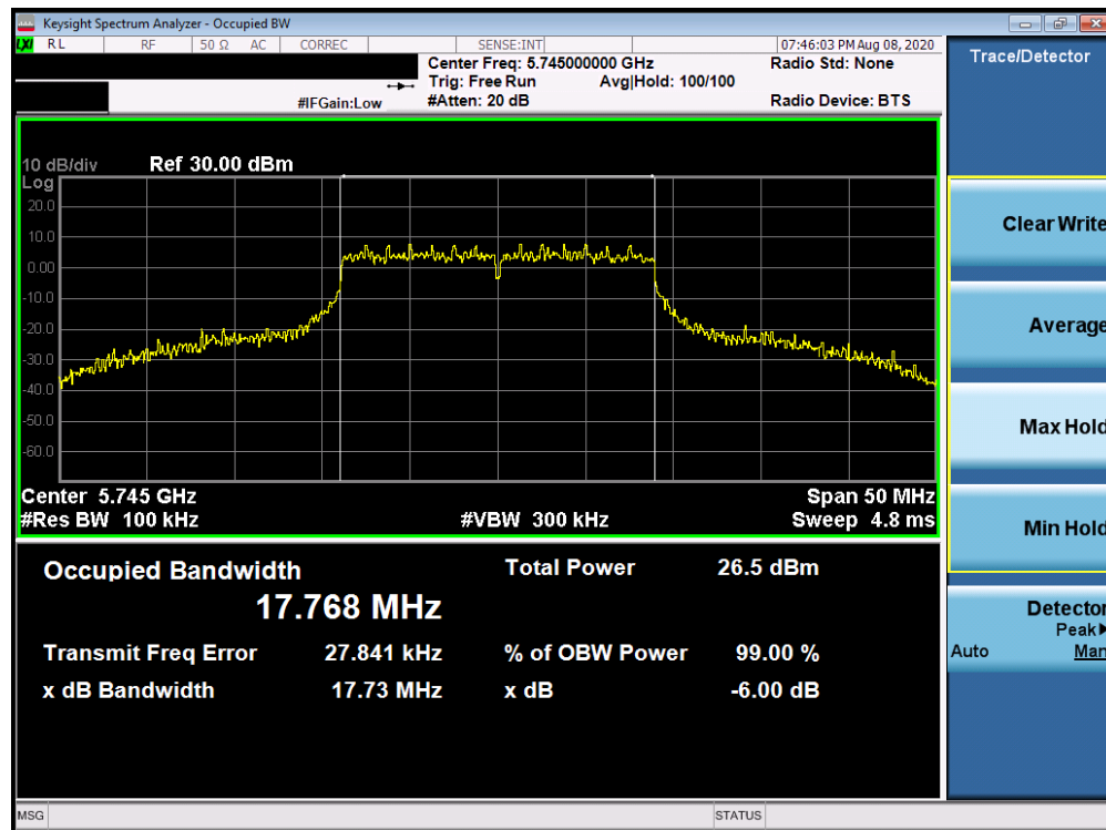
Plot 7-67. 6dB Bandwidth Plot Antenna 2a (20MHz BW 802.11n (UNII Band 3) – Ch. 149)
