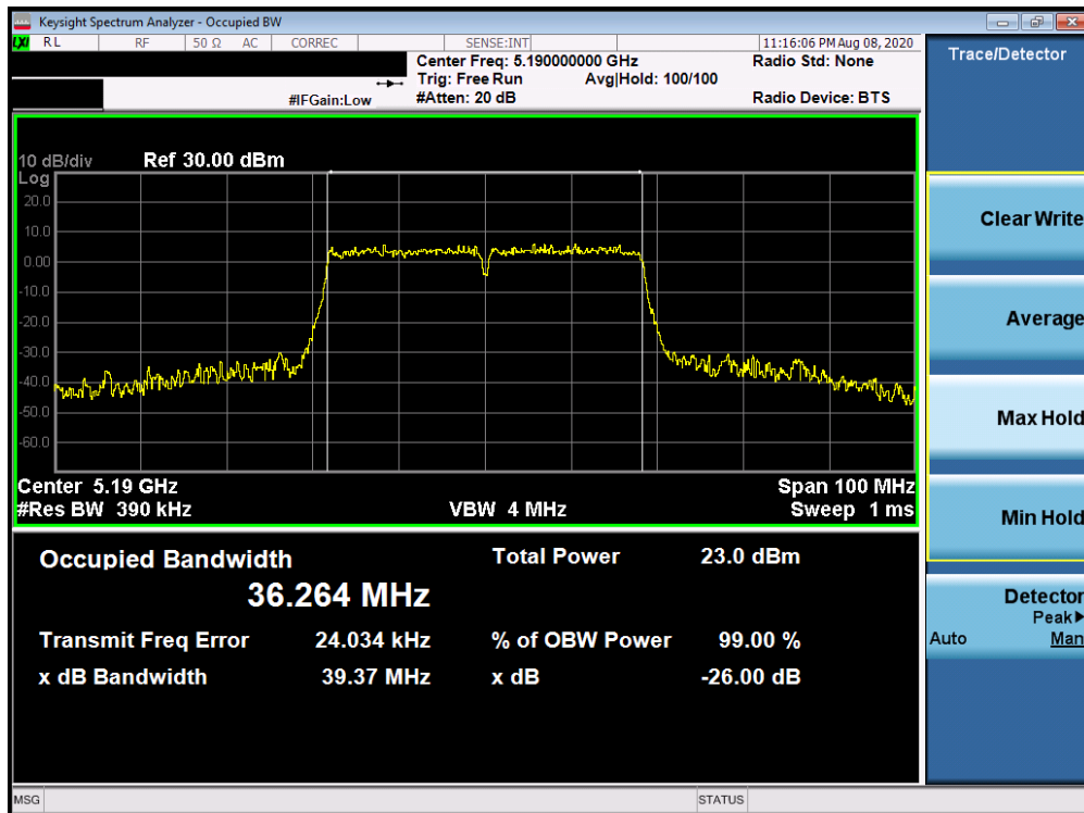
Plot 7-44. 26dB Bandwidth Plot Antenna 1b (40MHz BW 802.11n (UNII Band 1) – Ch. 38)
