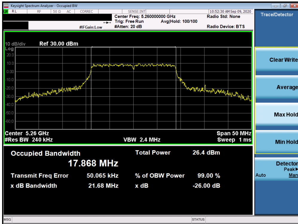
Plot 7-47. 26dB Bandwidth Plot Antenna 1b (20MHz BW 802.11n (UNII Band 2A) – Ch. 52)
