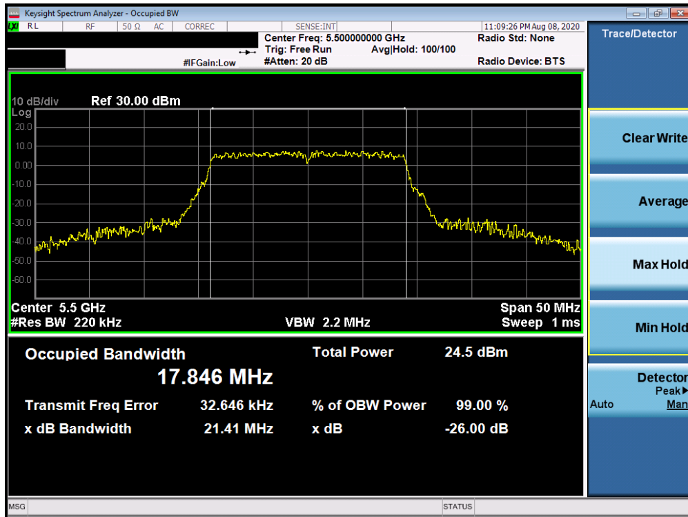
Plot 7-53. 26dB Bandwidth Plot Antenna 1b (20MHz BW 802.11n (UNII Band 2C) – Ch. 100)
