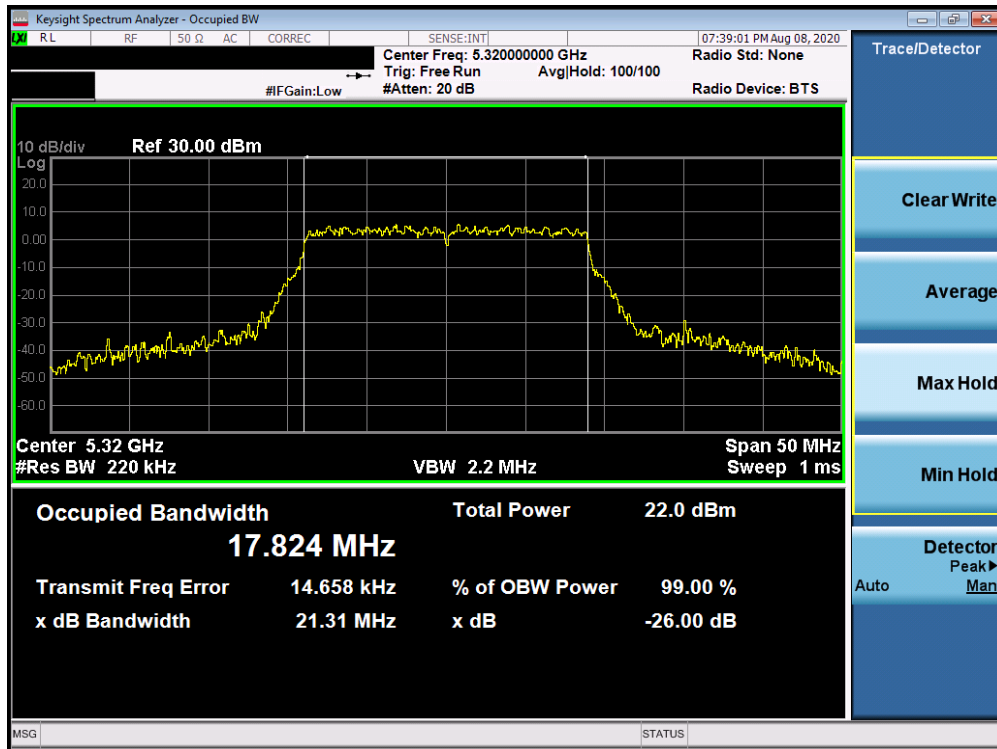
Plot 7-29. 26dB Bandwidth Plot Antenna 2a (20MHz BW 802.11n (UNII Band 2A) – Ch. 64)
