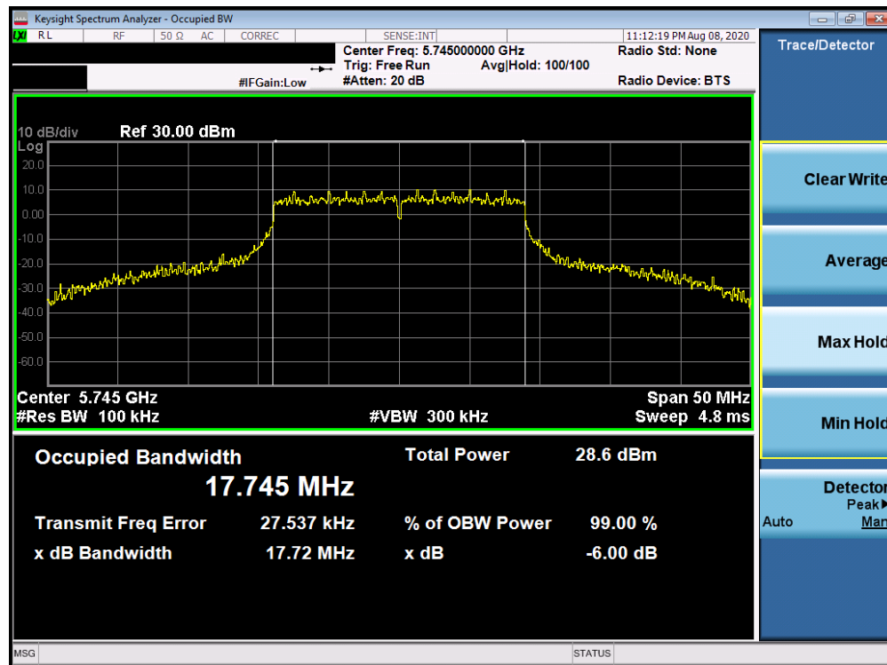
Plot 7-73. 6dB Bandwidth Plot Antenna 1b (20MHz BW 802.11n (UNII Band 3) – Ch. 149)
