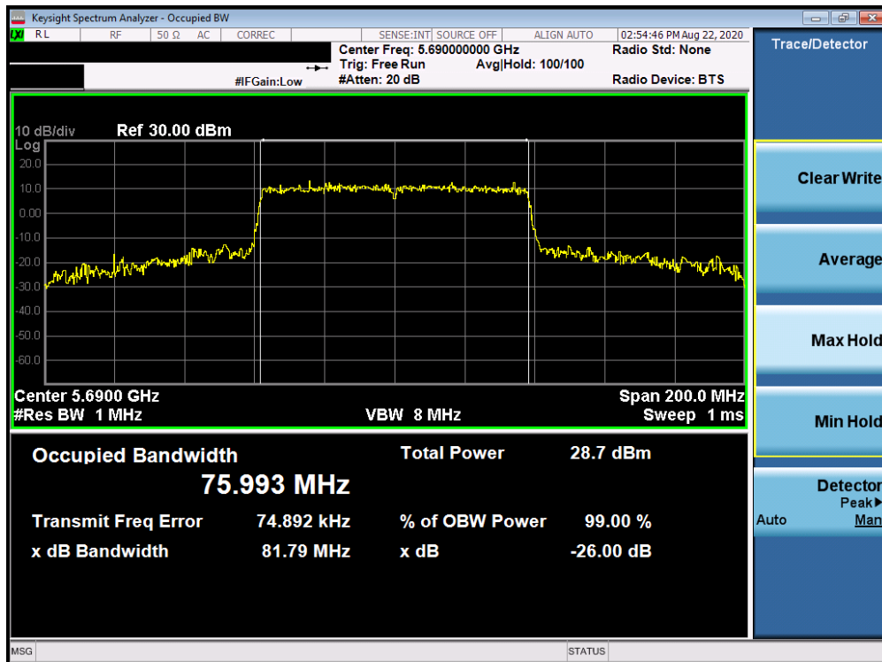
Plot 7-20. 26dB Bandwidth Plot Antenna 2b (80MHz BW 802.11ac (UNII Band 2C) – Ch. 138)
