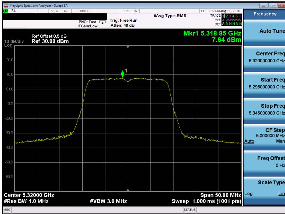
Plot 7-91. Power Spectral Density Plot Antenna 2b (20MHz BW 802.11n (UNII Band 2A) – Ch. 64)
