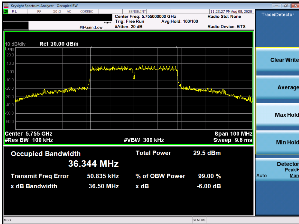
Plot 7-76. 6dB Bandwidth Plot Antenna 1b (40MHz BW 802.11n (UNII Band 3) – Ch. 151)
