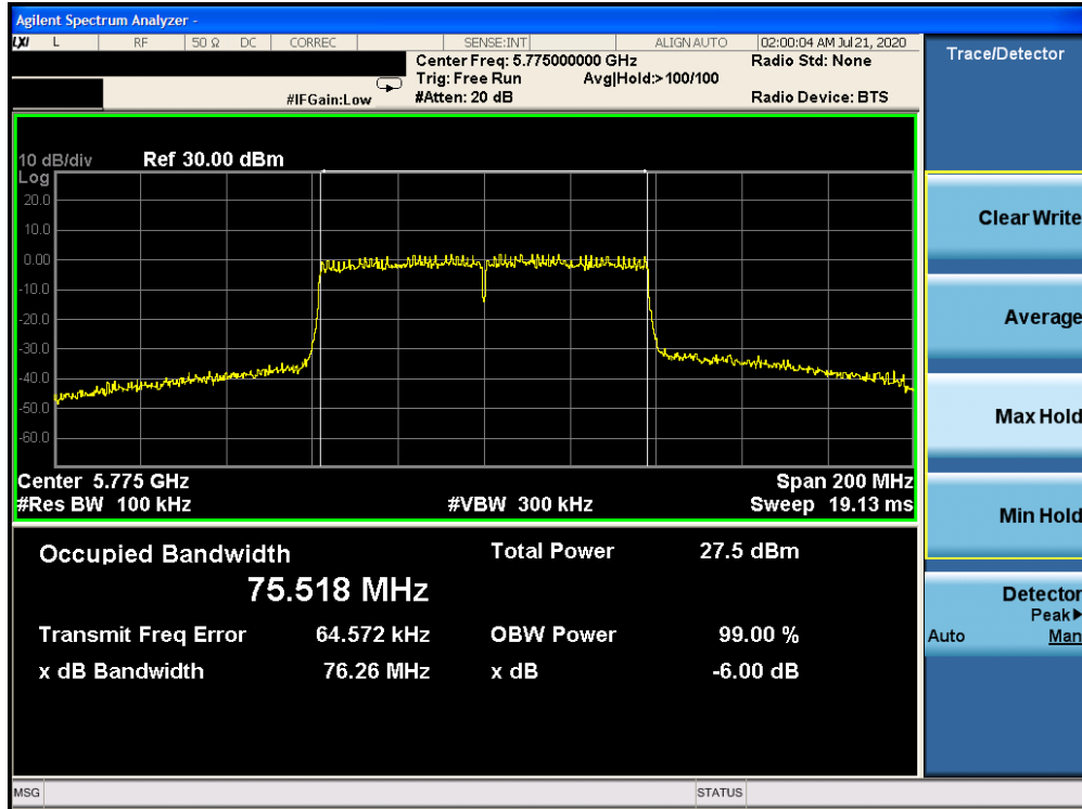
Plot 7-66. 6dB Bandwidth Plot Antenna 2b (80MHz BW 802.11ac (UNII Band 3) – Ch. 155)
