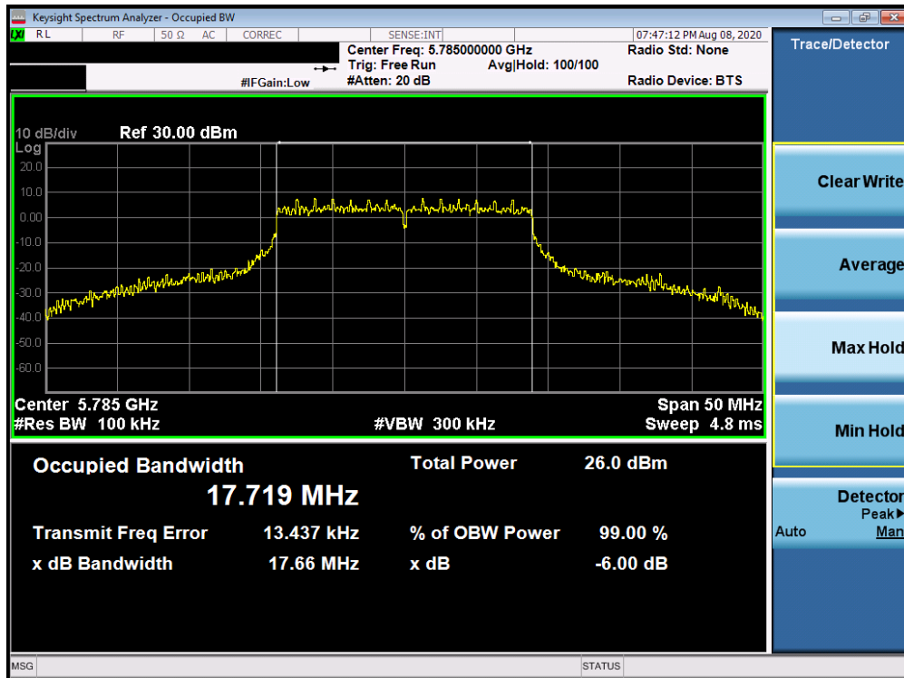
Plot 7-68. 6dB Bandwidth Plot Antenna 2a (20MHz BW 802.11n (UNII Band 3) – Ch. 157)
