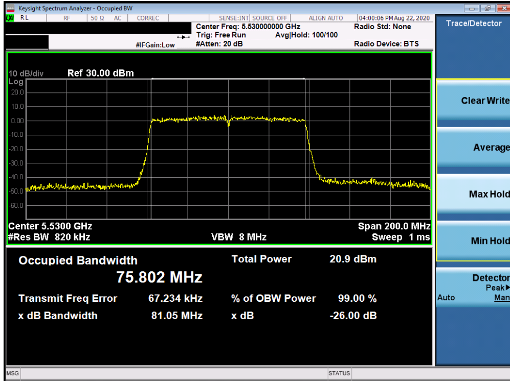
Plot 7-59. 26dB Bandwidth Plot Antenna 1b (80MHz BW 802.11ac (UNII Band 2C) – Ch. 106)
