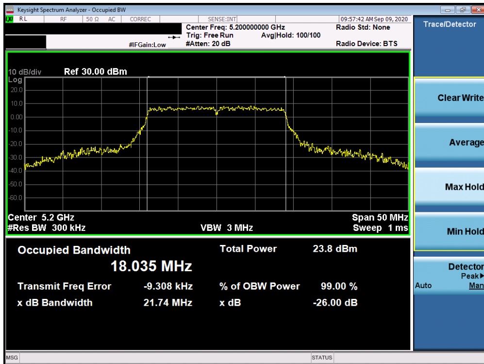
Plot 7-22. 26dB Bandwidth Plot Antenna 2a (20MHz BW 802.11n (UNII Band 1) – Ch. 40)
