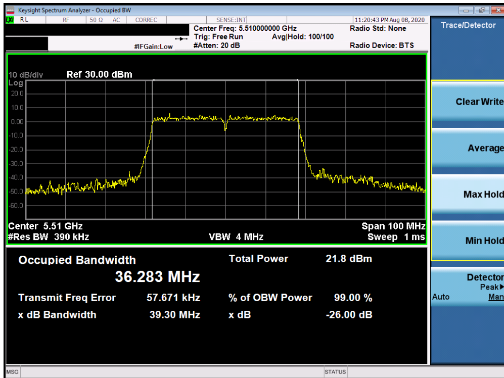
Plot 7-56. 26dB Bandwidth Plot Antenna 1b (40MHz BW 802.11n (UNII Band 2C) – Ch. 102)
