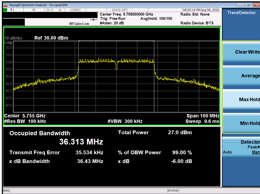
Plot 7-70. 6dB Bandwidth Plot Antenna 2a (40MHz BW 802.11n (UNII Band 3) – Ch. 151)
