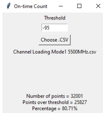
Figure 9-2. 5500MHz - Channel Loading Calculation - Mode 1 (20MHz)
