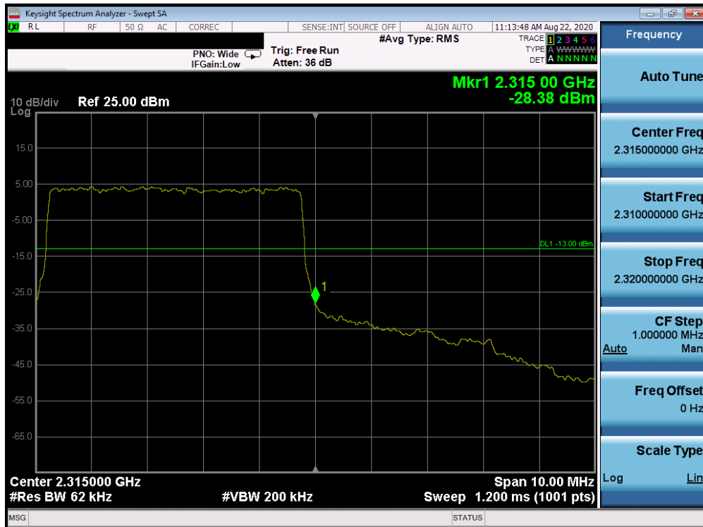
Plot 7-303. Upper Band Edge Plot (Band 30 - 5.0MHz QPSK - Full RB Configuration)
