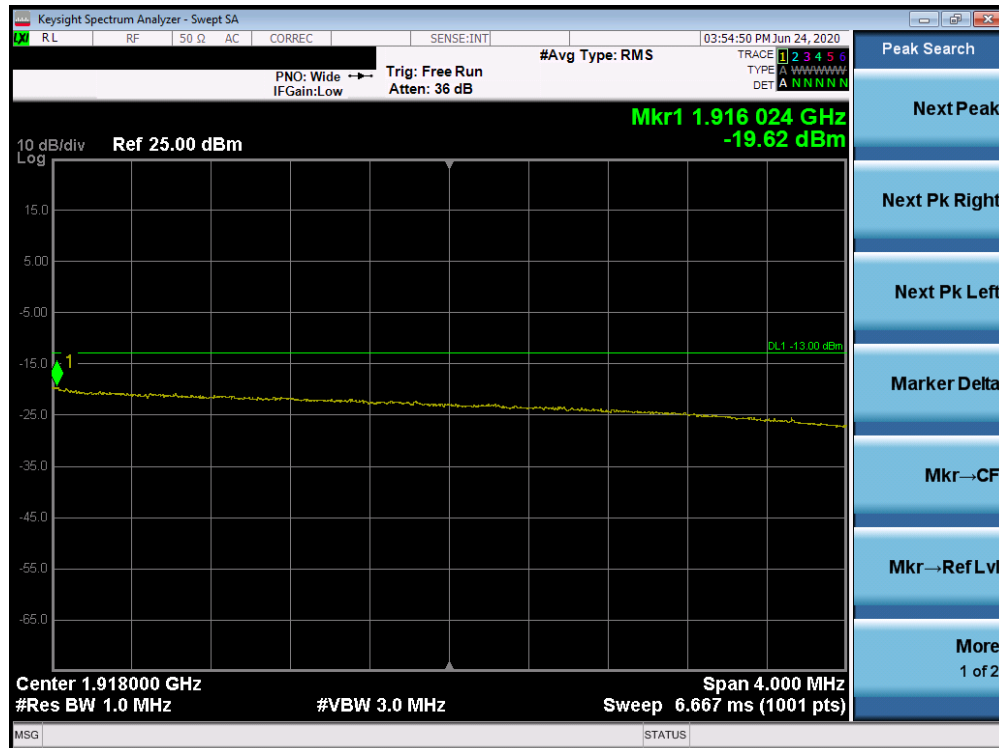
Plot 7-268. Upper Extended Band Edge Plot (Band 25 - 10.0MHz QPSK - Full RB Configuration)
