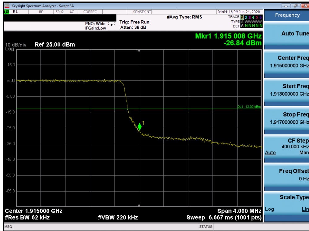
Plot 7-263. Upper Band Edge Plot (Band 25 - 5.0MHz QPSK - Full RB Configuration)
