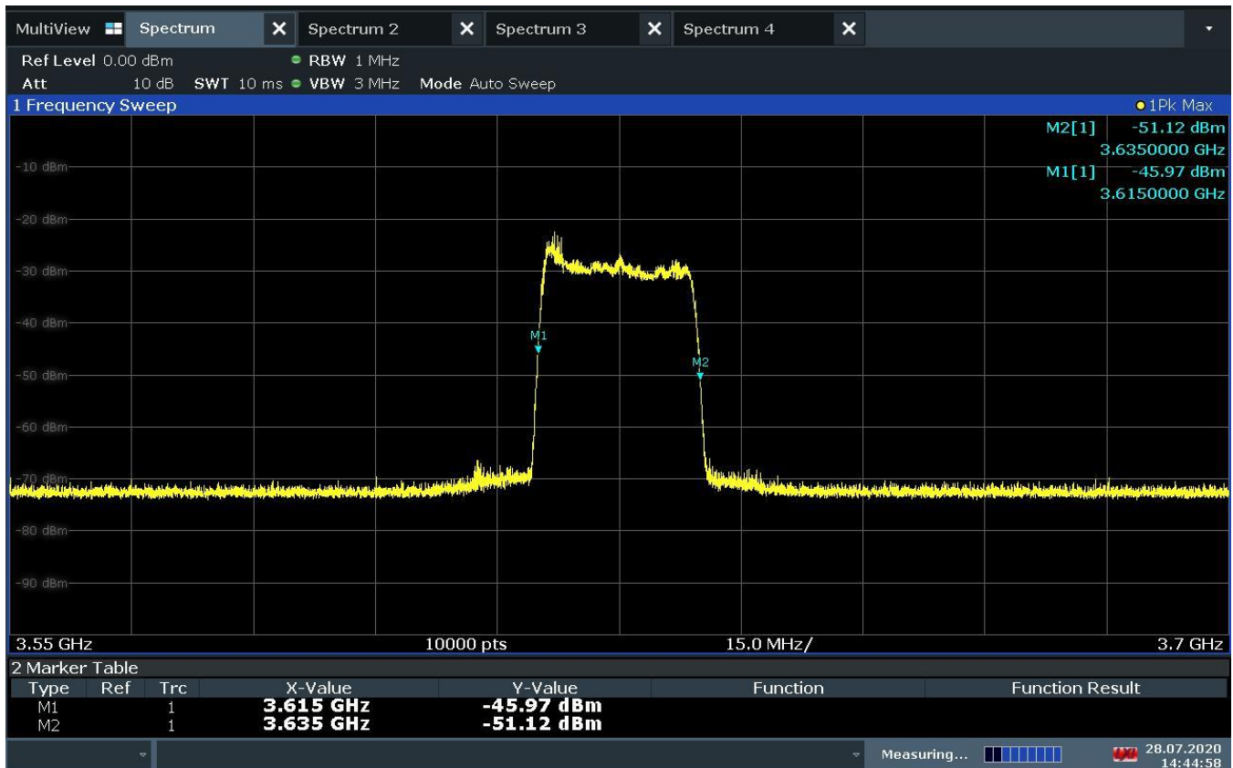
Plot 7-36. Run#1 End User Device Frequency of Operations
