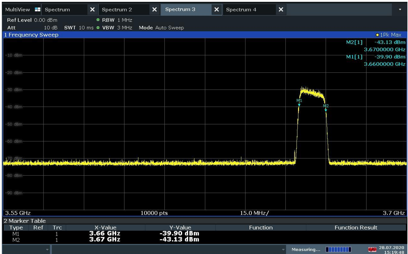
Plot 7-38. Run#2 End User Device Frequency of Operations
