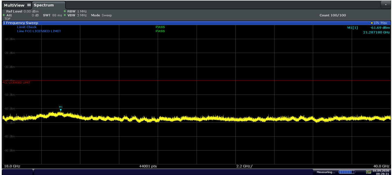
Plot 7-35. Radiated Spurious Plot 18 - 40GHz (Band 48 – Ant. Pol V)
