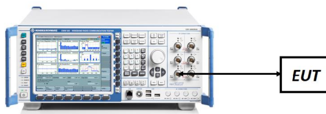
Figure 7-4. ERP/EIRP Measurement Setup
