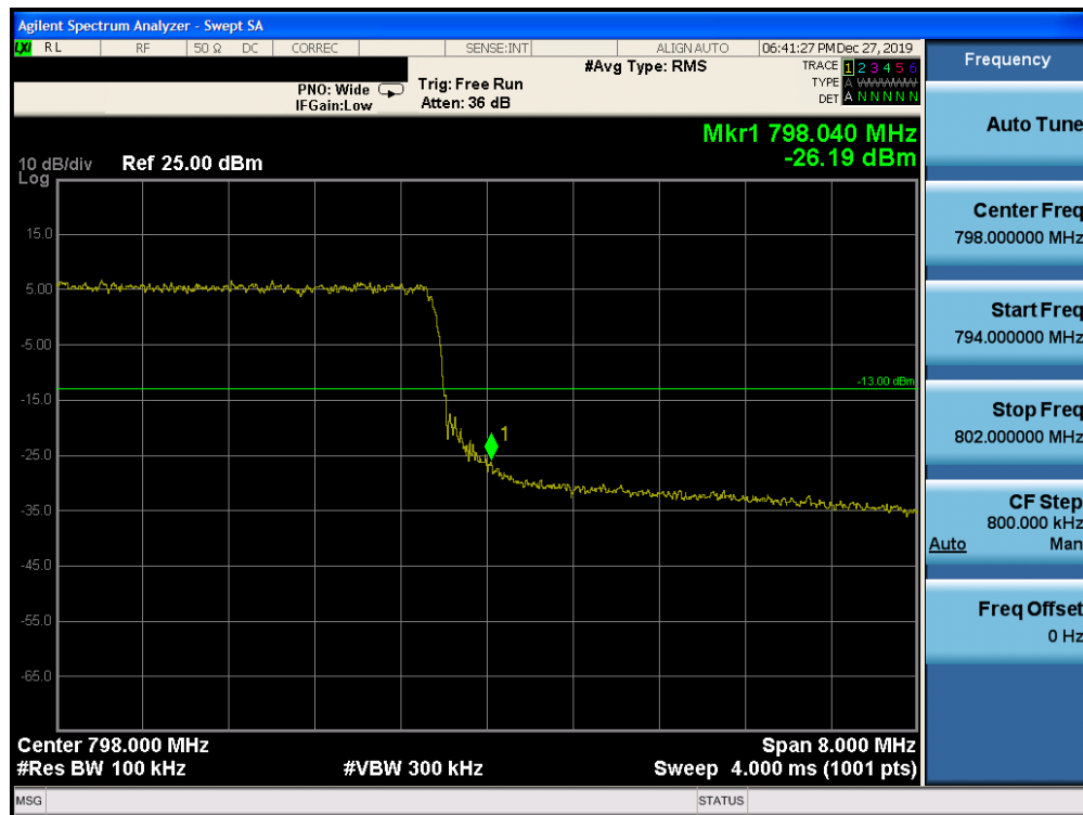
Plot 7-43. Upper Band Edge Plot (LTE Band 14 - 10MHz QPSK)
