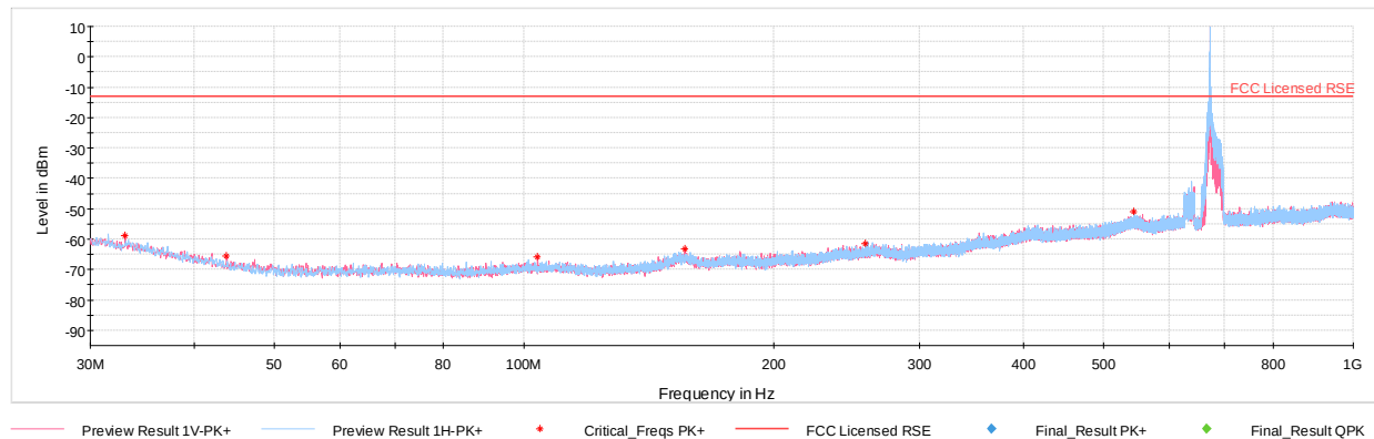
Plot 7-448. Radiated Spurious Plot below 1GHz (Band 71)
