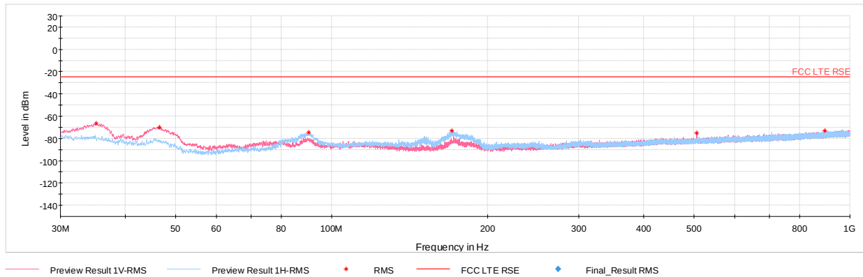
Plot 7-467. Radiated Spurious Plot Below 1GHz
