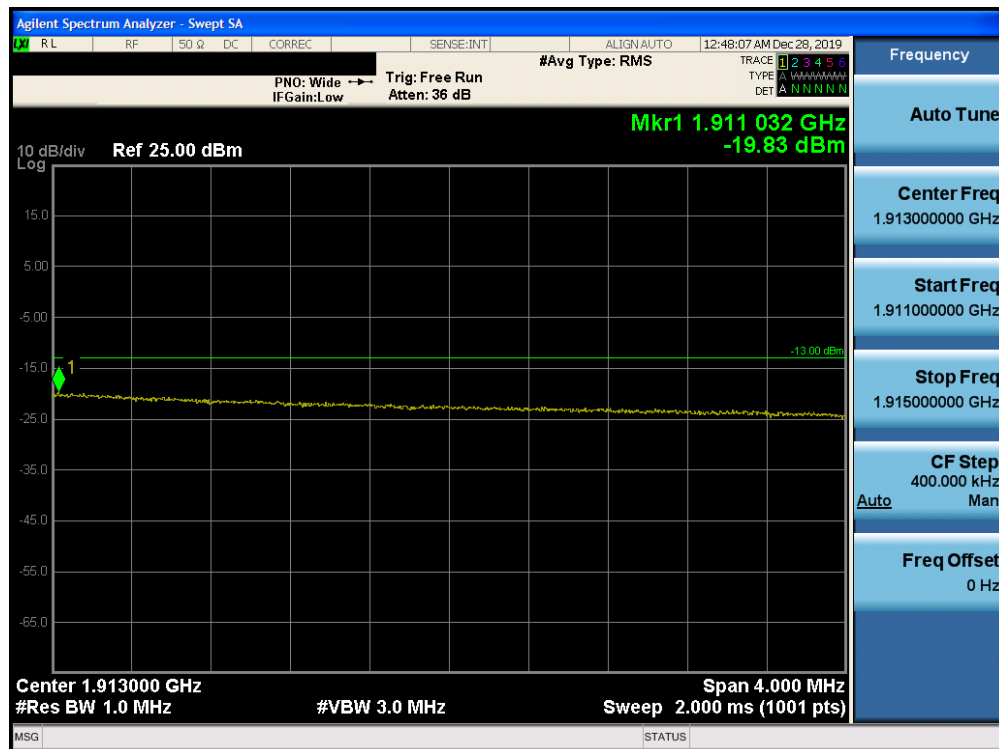
Plot 7-305. Upper Extended Band Edge Plot (Band 2 – 20.0MHz QPSK – RB Size 100)
