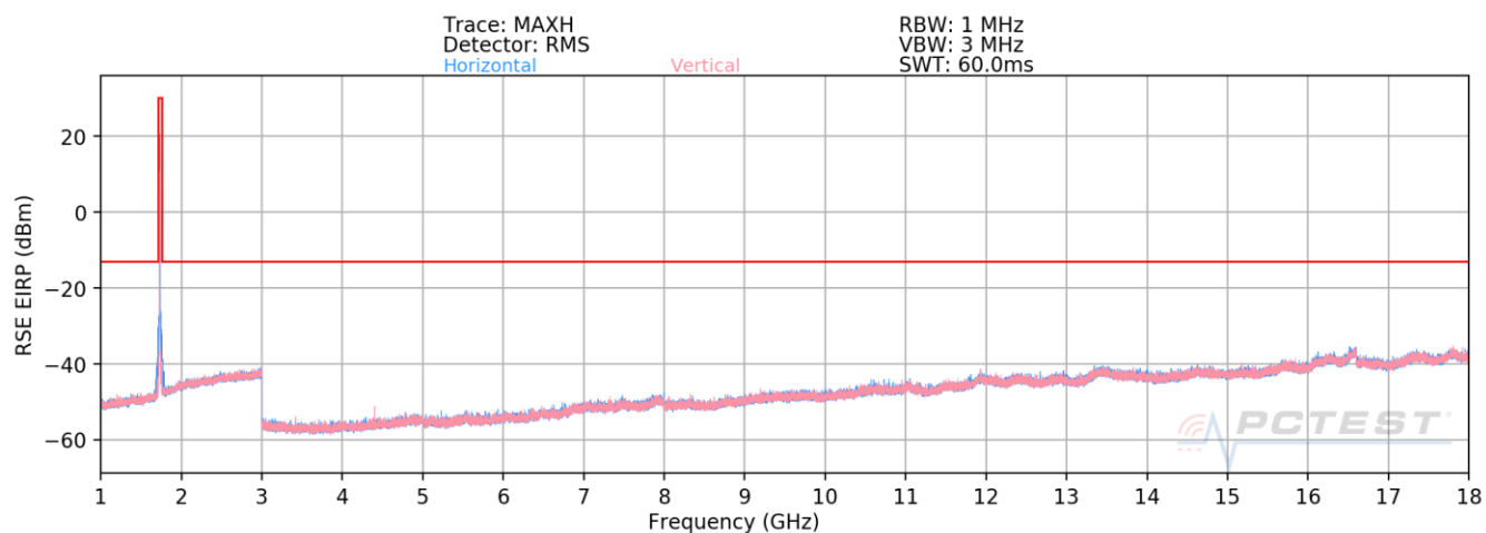
Plot 7-79. Radiated Spurious Plot Above 1GHz (AWS WCDMA Mode)
