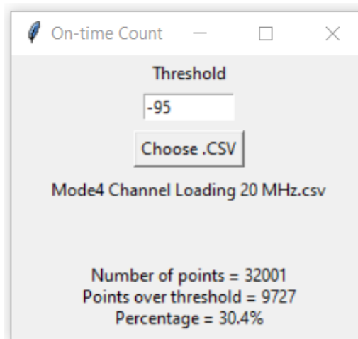
Figure 9-20. 5500MHz - Channel Loading Calculation - Mode 4 (20MHz)
