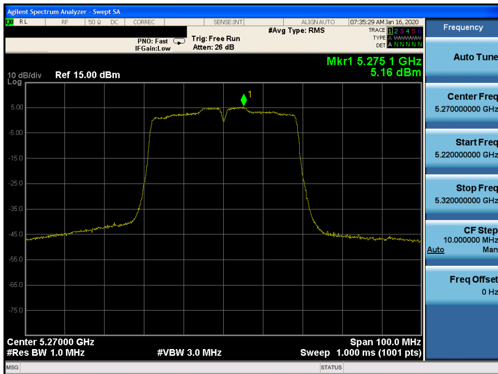
Plot 7-140. Power Spectral Density Plot CDD CORE 1 (40MHz BW 802.11n (UNII Band 2A) – Ch. 54)
