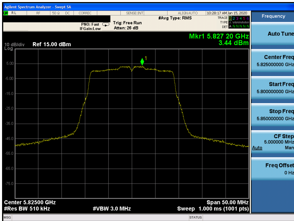
Plot 7-165. Power Spectral Density Plot CDD CORE 0 (20MHz BW 802.11n (UNII Band 3) – Ch. 165)
