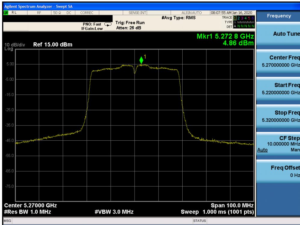
Plot 7-139. Power Spectral Density Plot CDD CORE 0 (40MHz BW 802.11n (UNII Band 2A) – Ch. 54)
