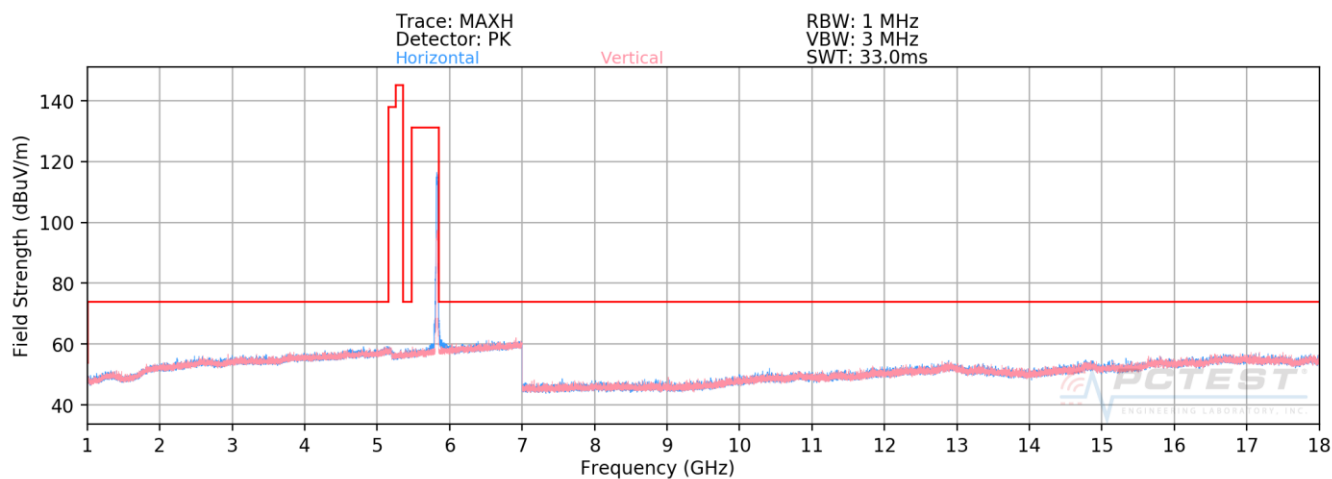
Plot 7-196. Radiated Spurious Plot above 1GHz SISO CORE1 (802.11n – U3 Ch. 165)
