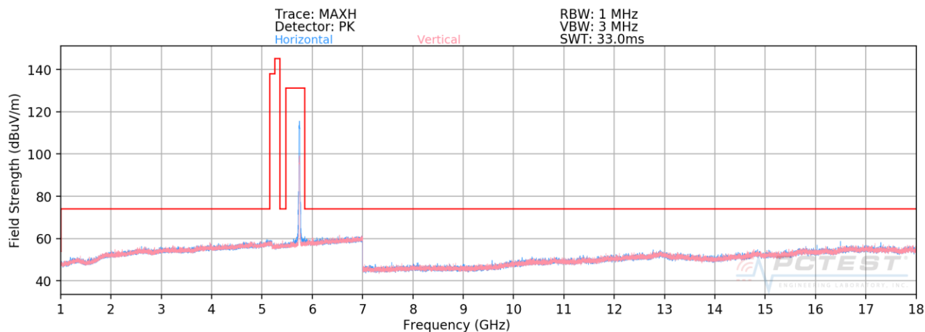
Plot 7-194. Radiated Spurious Plot above 1GHz SISO CORE1 (802.11n – U3 Ch. 149)
