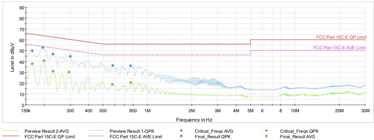
Plot 7-105. Line Conducted Plot with Bluetooth HDR (L1, 4Mbps ePA – Ch.38 with AC/DC Adapter)
