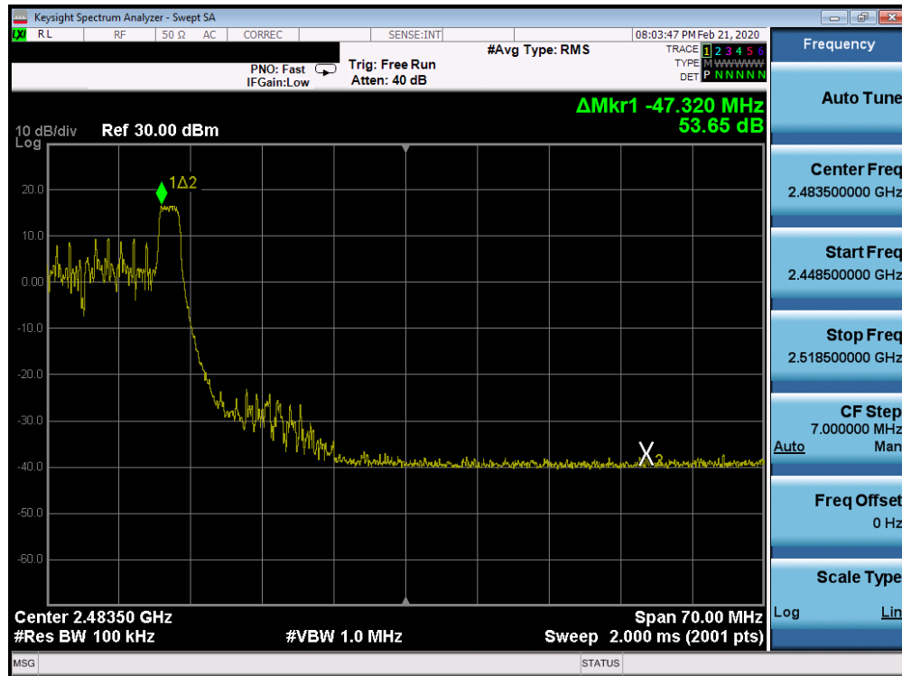
Plot 7-75. Band Edge SISO CORE 0 (802.11ax OFDMA – RU26 Index 8 – Ch. 9)
