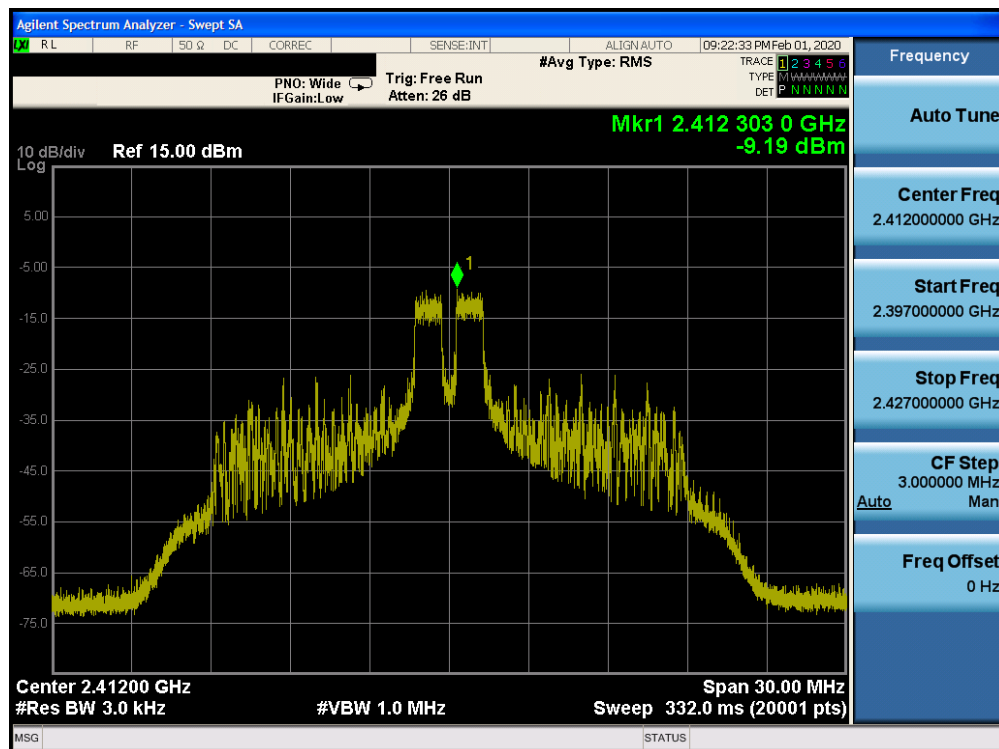
Plot 7-52. Power Spectral Density Plot CDD CORE 1 (802.11ax OFDMA – RU26 Index 4 – Ch. 1)a
