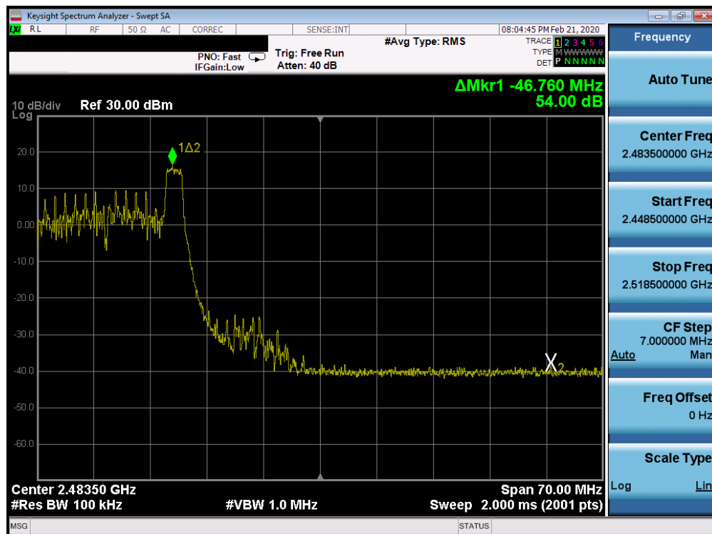
Plot 7-76. Band Edge SISO CORE 0 (802.11ax OFDMA – RU26 Index 8 – Ch. 10)
