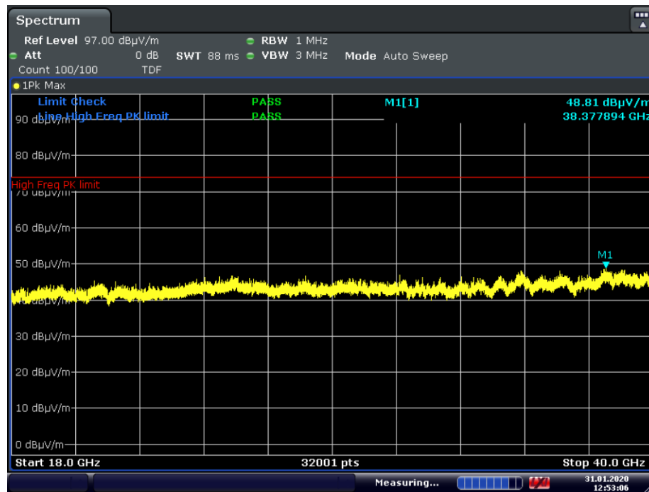
Plot 7-70. Radiated Spurious Plot 18GHz Simultaneous Tx – 40GHz Pol. V
