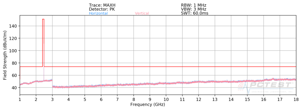
Plot 7-62. Radiated Spurious Plot above 1GHz Ant 2a (BT GFSK ePA – Ch. 78)
