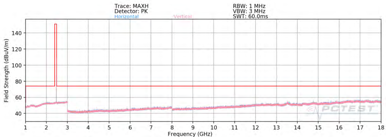
Plot 7-83. Radiated Spurious Plot Above 1GHz Ant 4a (4Mbps, HDR4 ePA – Ch. 75, Ant. Pol. H & V)
