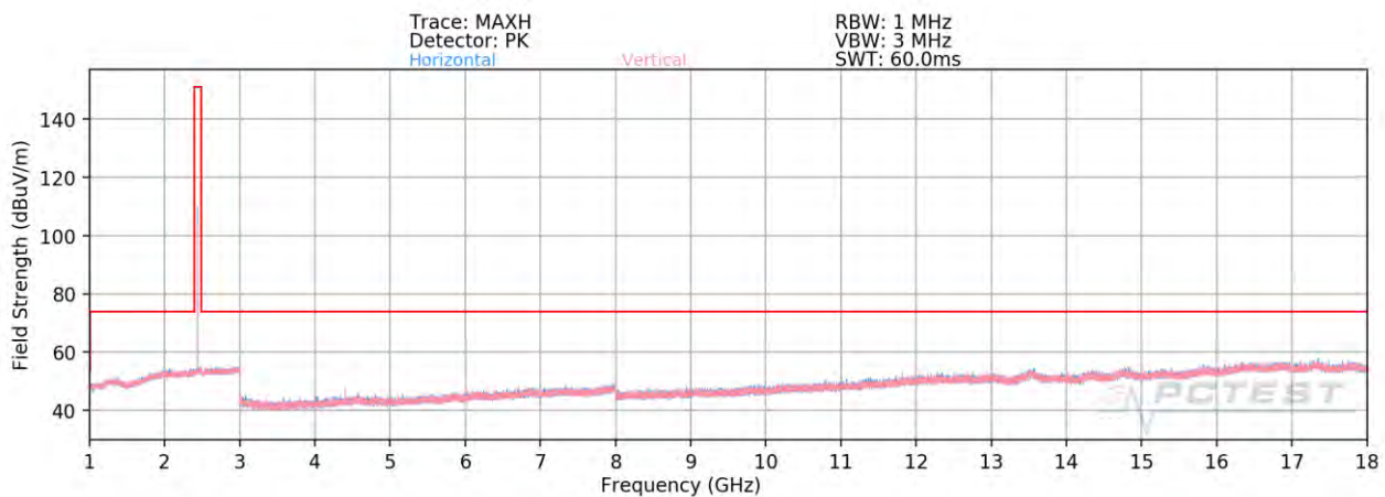
Plot 7-88. Radiated Spurious Plot Above 1GHz TXBF (4Mbps, HDR4 ePA – Ch. 38, Ant. Pol. H & V)
