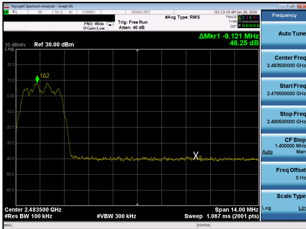
Plot 7-62. Band Edge Plot Ant 4a (Bluetooth (HDR4), ePA – Ch. 75)
