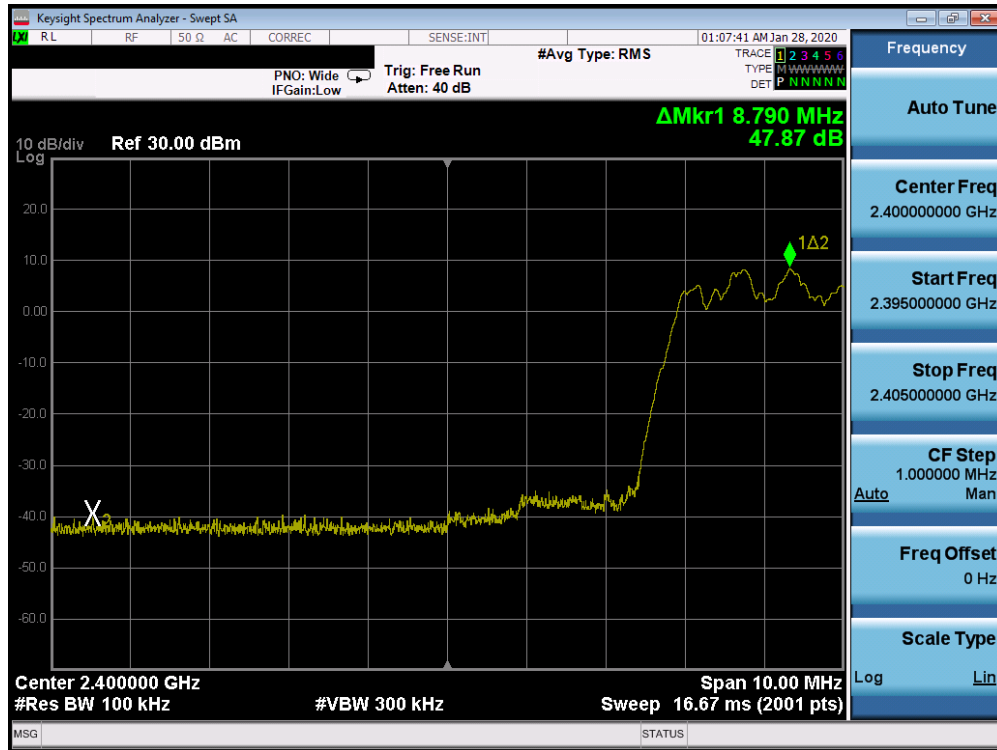
Plot 7-61. Band Edge Plot Ant 4a (Bluetooth (HDR4), ePA – Ch. 1)
