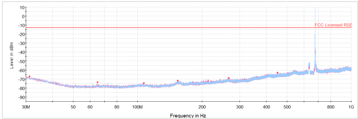
Plot 7-448. Radiated Spurious Plot below 1GHz (Band 71)
