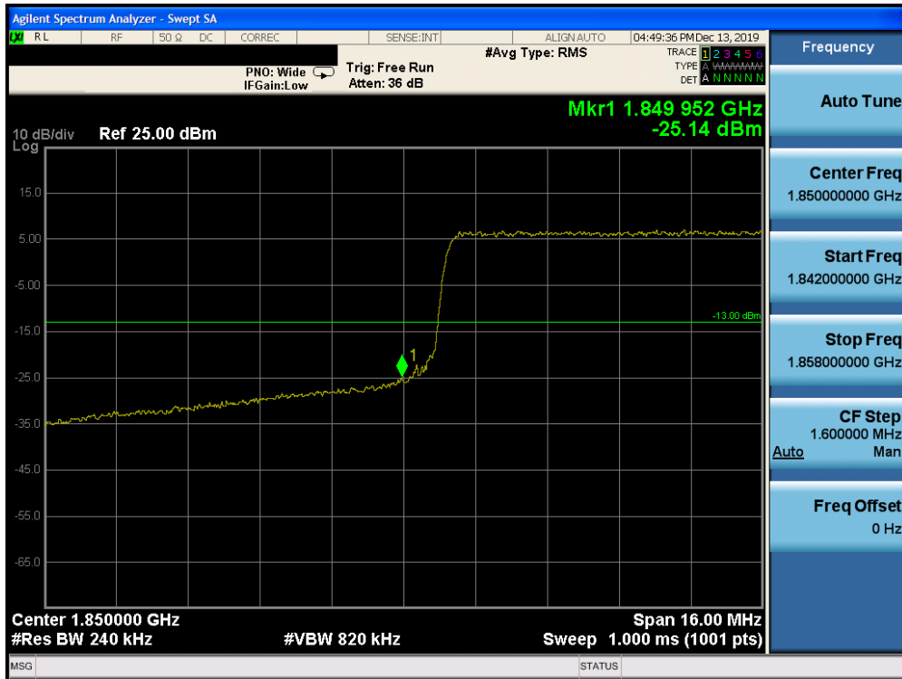
Plot 7-326. Lower Band Edge Plot (Band 25 – 20.0MHz QPSK – RB Size 100)
