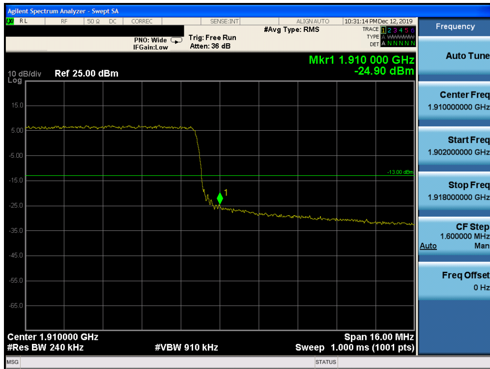
Plot 7-304. Upper Band Edge Plot (Band 2 – 20.0MHz QPSK – RB Size 100)
