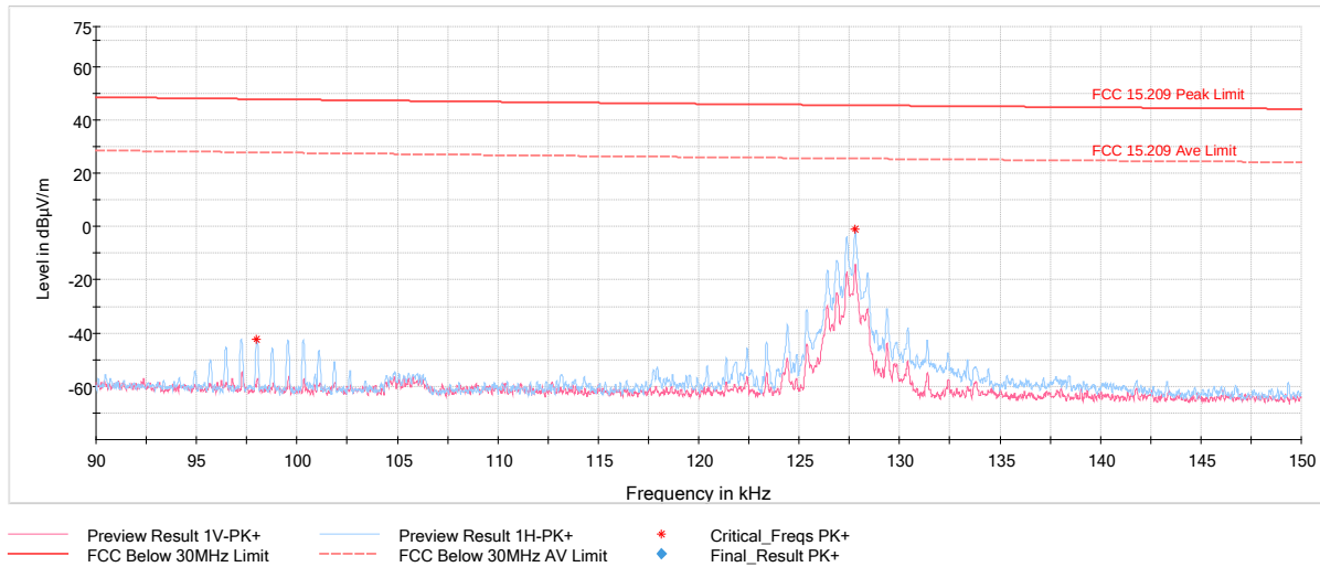
Plot 6-2. Radiated Restricted Lower Band Edge Measurement (Peak)
