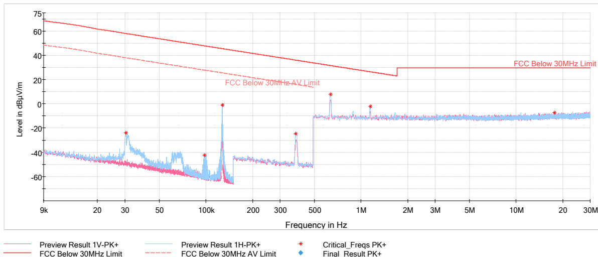
Plot 6-3. Radiated Spurious Plot 9kHz-30MHz with AC/DC Adapter
