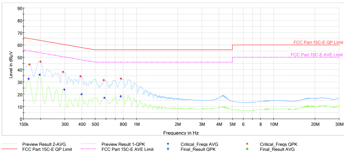
Plot 6-5. Line Conducted Plot (L1, with AC/DC Adapter)
