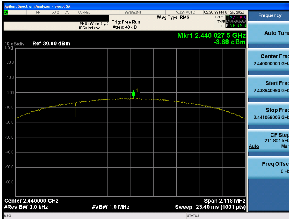
Plot 7-23. Power Spectral Density Plot Ant 4a (Bluetooth (LE), 2Mbps, iPA – Ch. 19)
