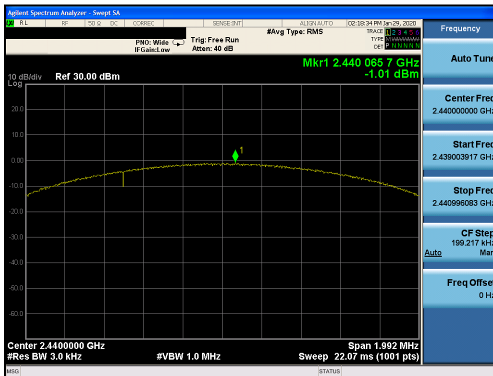
Plot 7-20. Power Spectral Density Plot Ant 4a (Bluetooth (LE), 2Mbps, ePA – Ch. 19)
