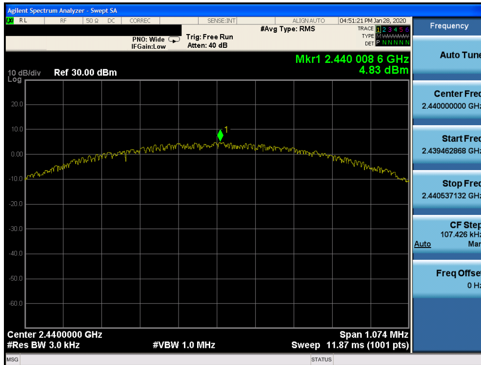
Plot 7-39. Power Spectral Density Plot TxBF Ant 4a (Bluetooth (LE), 1Mbps, ePA – Ch. 19)
