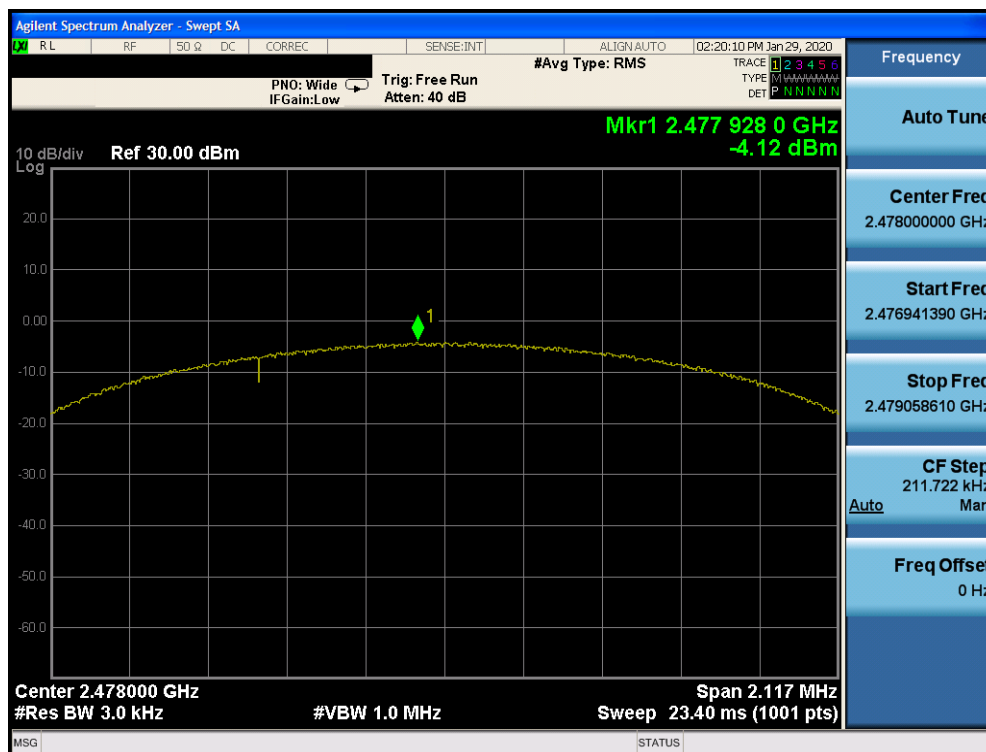
Plot 7-24. Power Spectral Density Plot Ant 4a (Bluetooth (LE), 2Mbps, iPA – Ch. 38)
