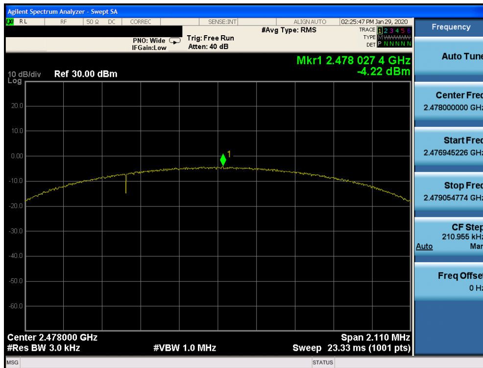
Plot 7-59. Power Spectral Density Plot TxBF Ant 4a (Bluetooth (LE), 2Mbps, iPA – Ch. 38)
