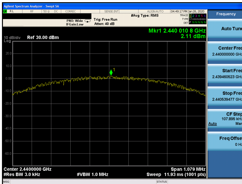
Plot 7-40. Power Spectral Density Plot TxBF Ant 2a (Bluetooth (LE), 1Mbps, ePA – Ch. 19)
