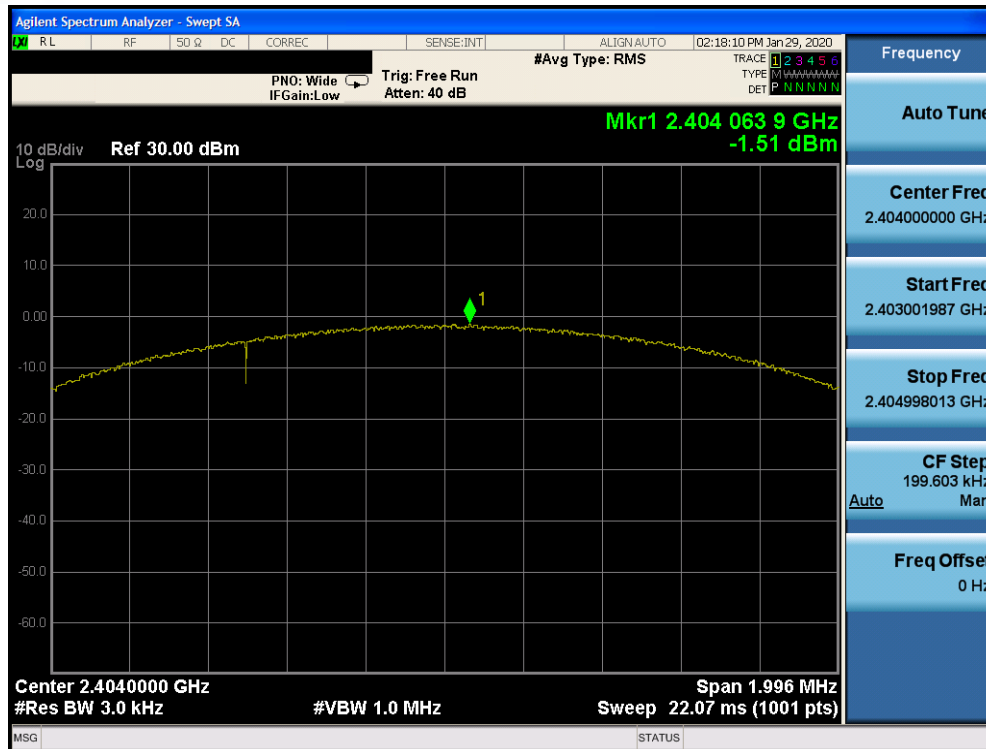
Plot 7-19. Power Spectral Density Plot Ant 4a (Bluetooth (LE), 2Mbps, ePA – Ch. 1)
